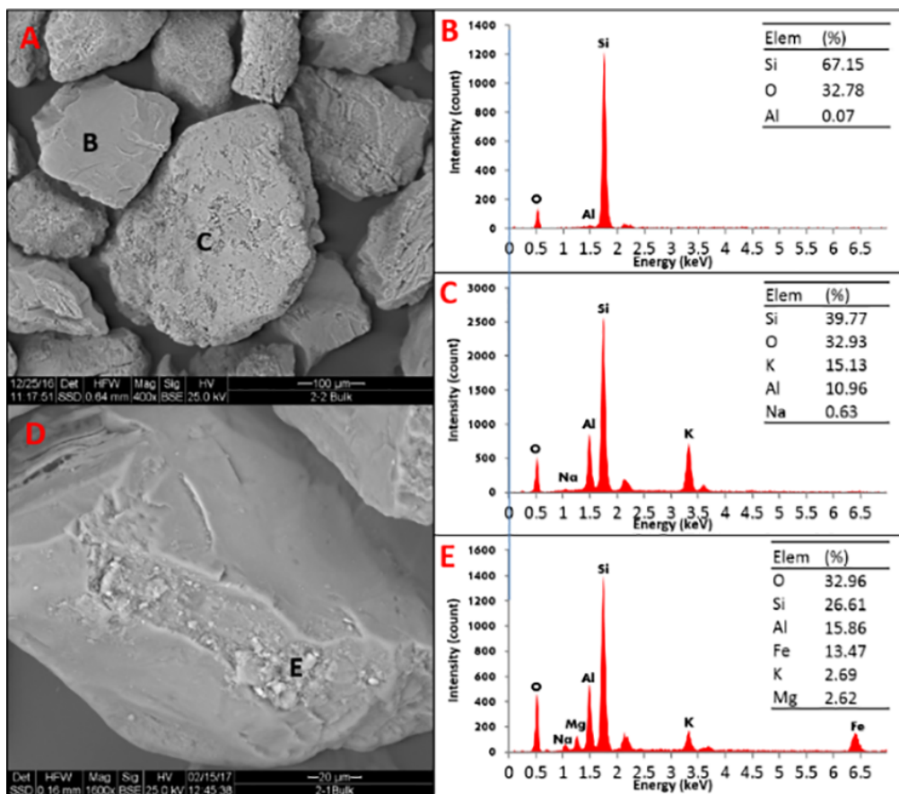
Figure 8. (a) Scanning electron microscopy (SEM) image of an Oceano sand sample. (b) Energy dispersive X-ray spectroscopy (EDS) chemical composition (percentage by mass) of a quartz grain in (a) (the location of the analysis is marked by the black letter “B”). (c) EDS chemical composition of a K-rich feldspar in (a) marked by the black letter “C”. (d) Close-up image of a quartz sand grain with mineral coatings. (e) EDS chemical composition of the mineral coatings in (d) marked by the black letter “E”.
