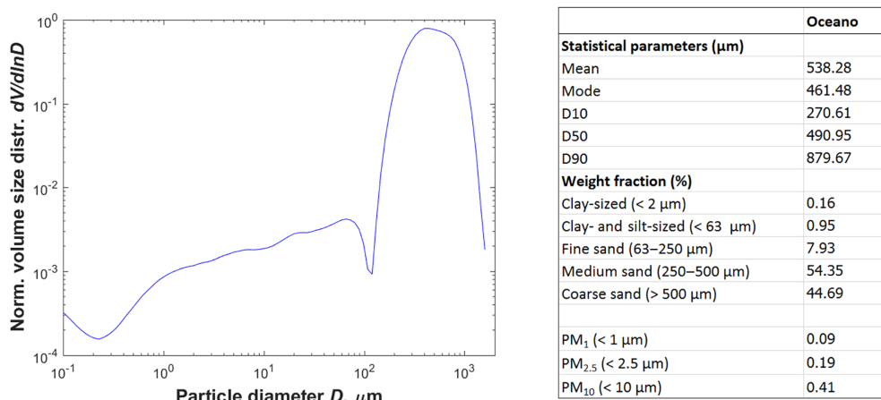
Figure 7. Normalized volume particle size distribution (PSD) of sand samples collected from the Oceano field site. Statistical parameters of the PSD are reported in the table to the right. D10, D50, and D90 refer to cut-off diameters of the 10th, 50th, and 90th percentile of sample grains by mass, respectively. Note that the values are averages of four samples with two collected from the tower location and two from 100 m upwind.
