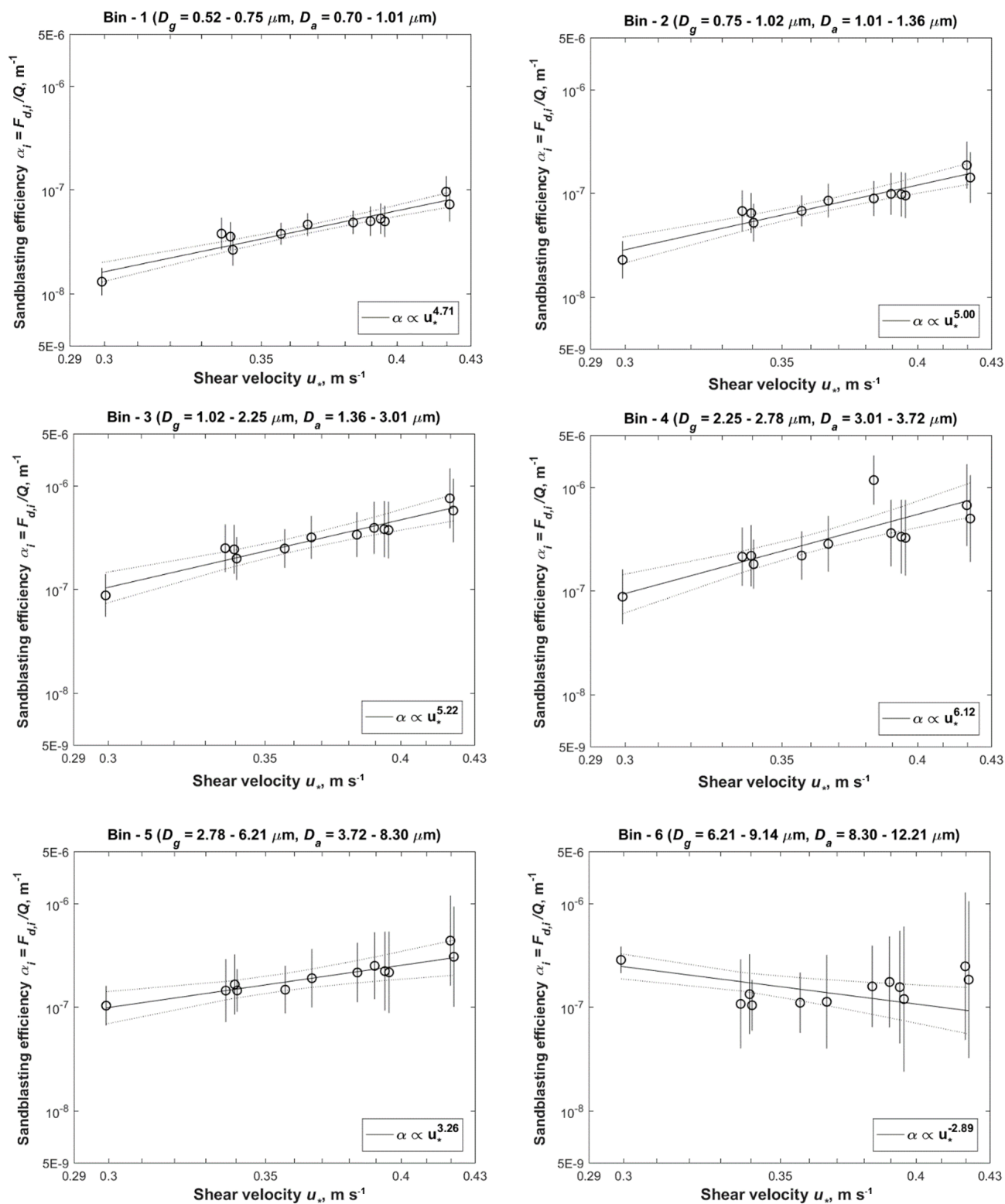
Figure 6. The sandblasting efficiency \alpha_i ( \text{m}^{-1} ) of the six size bins at Oceano as a function of shear velocity. The linear-least-squares fit (black line) indicates that \alpha_i varies as a power law in shear velocity with an exponent of 4.71 \pm 0.97 , 5.00 \pm 1.37 , 5.22 \pm 1.63 , 6.12 \pm 2.11 , 3.26 \pm 1.90 , and -2.89 \pm 1.94 for the six respective size bins. Error bars were obtained by propagating errors from the sensor intercalibration process, the regression used in the gradient method, and the subtraction of the sea-salt deposition flux (see Supplement). The two dotted black lines denote the 95% confidence range of the fit. The geometric and the aerodynamic diameter ranges of the vertical dust mass flux F_{d,i} are noted at the top of each of the six plots, and Q is the total horizontal sand flux integrated over all sand grain sizes (Martin et al., 2018).
