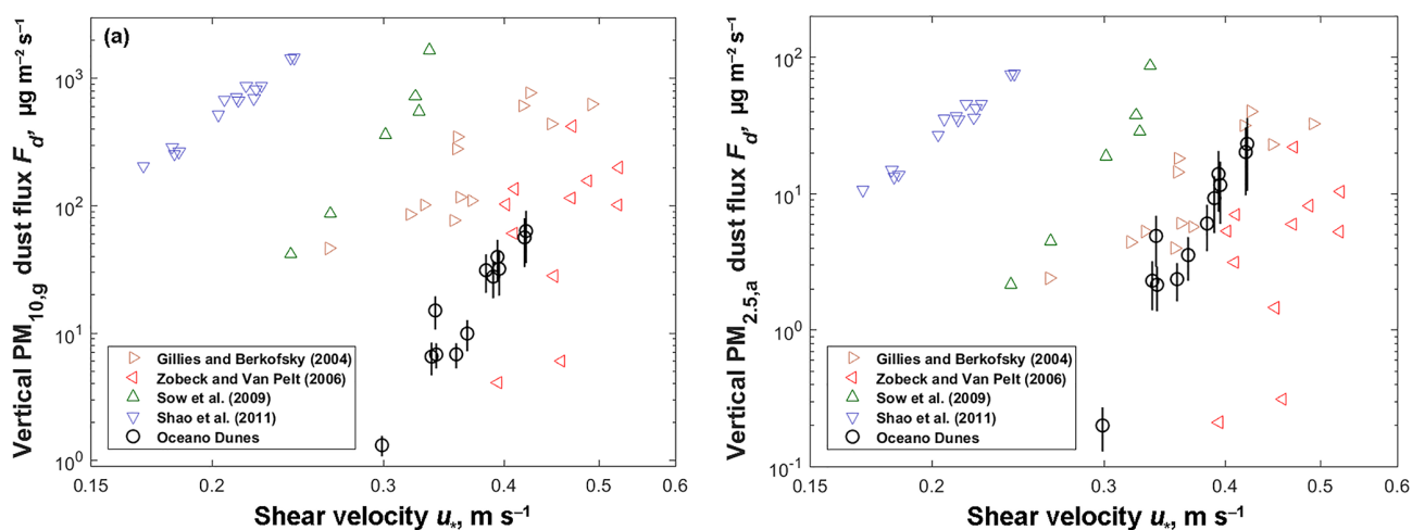
Figure 2. The vertical dust mass flux as a function of shear velocity within (a) the \text{PM}_{10,\text{g}} geometric diameter range and (b) the \text{PM}_{2.5,\text{a}} aerodynamic diameter range. Each of the two plots includes measurements at Oceano (black open circles) and previously published field studies of natural dust emissions from non-sandy soils (open triangles). These latter measurements were compiled in Kok et al. (2014a), which corrected these measurements to the \text{PM}_{10,\text{g}} geometric diameter range following the procedure described in that work. Furthermore, we corrected these measurements to the \text{PM}_{2.5,\text{a}} aerodynamic diameter range assuming that their PSDs follow the prediction of the brittle fragmentation theory generated by aggregate fragmentation (Kok, 2011). Error bars on the Oceano measurements were obtained through error propagation (details in Supplement).
