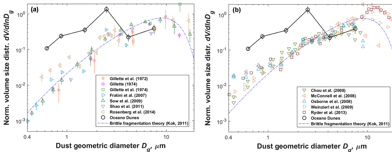
Figure 3. Normalized volume particle size distribution (PSD) of dust at emission as a function of the dust aerosol geometric diameter averaged over all measurements at Oceano (black open circles). Plotted for comparison are measurements compiled by Kok et al. (2017) of (a) the emitted dust PSDs from non-sandy soils in the US (Gillette et al., 1972, 1974; Gillette, 1974), China (Fratini et al., 2007), North Africa (Sow et al., 2009; Rosenberg et al., 2014), and Australia (Shao et al., 2011) and (b) in situ aircraft measurements of dust-dominated PSDs close to the Saharan source regions. Note that these measurements are normalized using the procedure described in Kok (2011) and Kok et al. (2017), which differs somewhat from the procedure used for the Oceano data (see Sect. 2). Also plotted for comparison is the brittle fragmentation theory (dashed–dotted blue lines) on the PSD of emitted dust generated by aggregate fragmentation (Kok, 2011). Error bars on the Oceano measurements were obtained through error propagation (details in Supplement).
