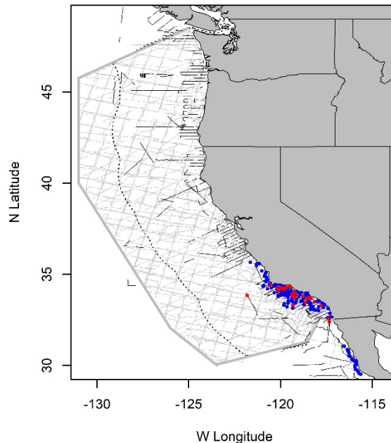
Figure 1. Long-beaked common dolphin sightings based on shipboard surveys off California, Oregon, and Washington, 1991-2018 (Barlow 2016, Henry et al. 2020). Dashed line represents U.S. EEZ, thin lines indicate completed transect effort (gray = 1991-2014, black = 2018). Sightings from the 2018 survey are shown in red.
