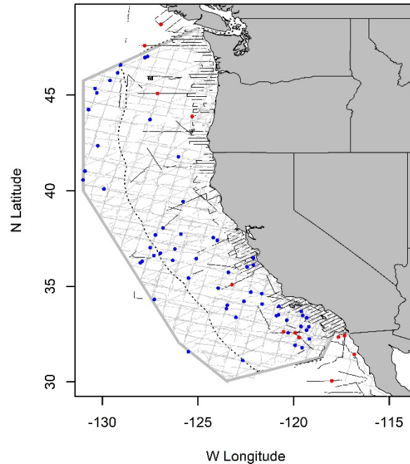
Figure 1. Cuvier's beaked whale sightings based on shipboard surveys off California, Oregon, and Washington, 1991-2018. Dashed line represents U.S. EEZ, thin lines indicate completed transect effort (gray = 1991-2014, black = 2018). Sightings from the 2018 survey are shown in red.
