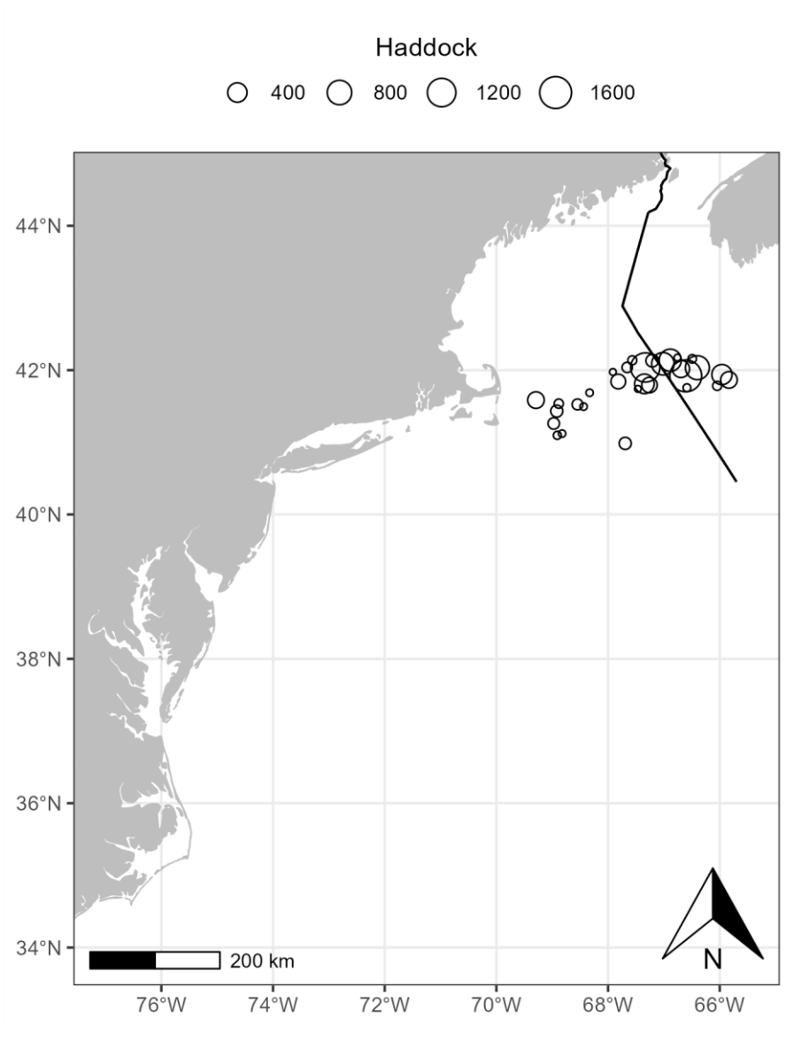
Figure 6: Total number of haddock per tow from the Northeast Fisheries Science Center's Spring Bottom Trawl Survey, May 09, 2023-May 23, 2023.
