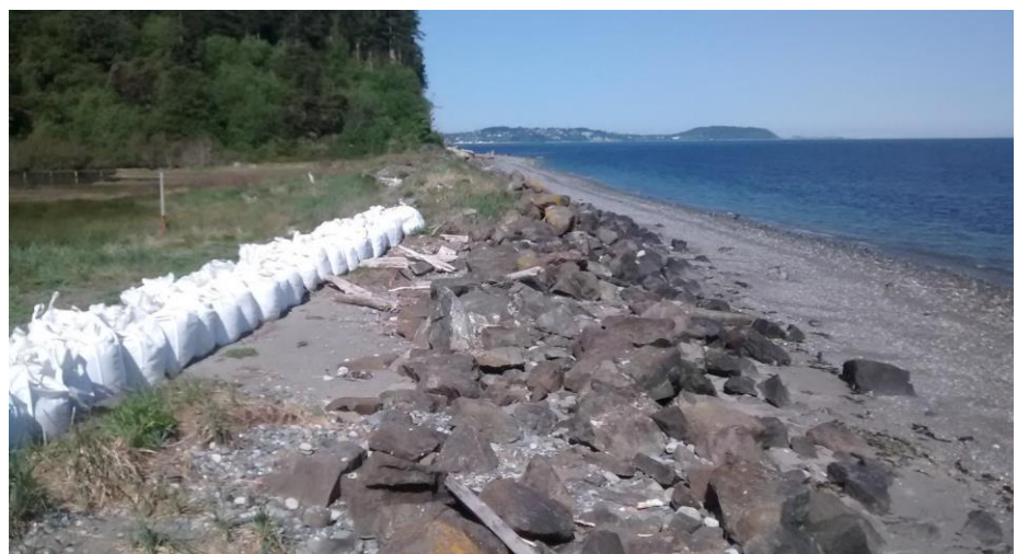
Figure 7. A failing rip-rap structure near Fort Flagler is supplemented with an additional placement of quasi-temporary sandbags to reduce backshore flooding. May 2015 photo by Ian Miller, Washington Sea Grant.
