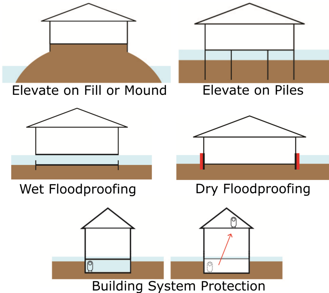
Figure 12. Illustration of accommodation techniques for new and retrofitted structures. Source: Inventory of Adaptive Strategies . Used with permission of the New York City Department of City Planning. All rights reserved.
