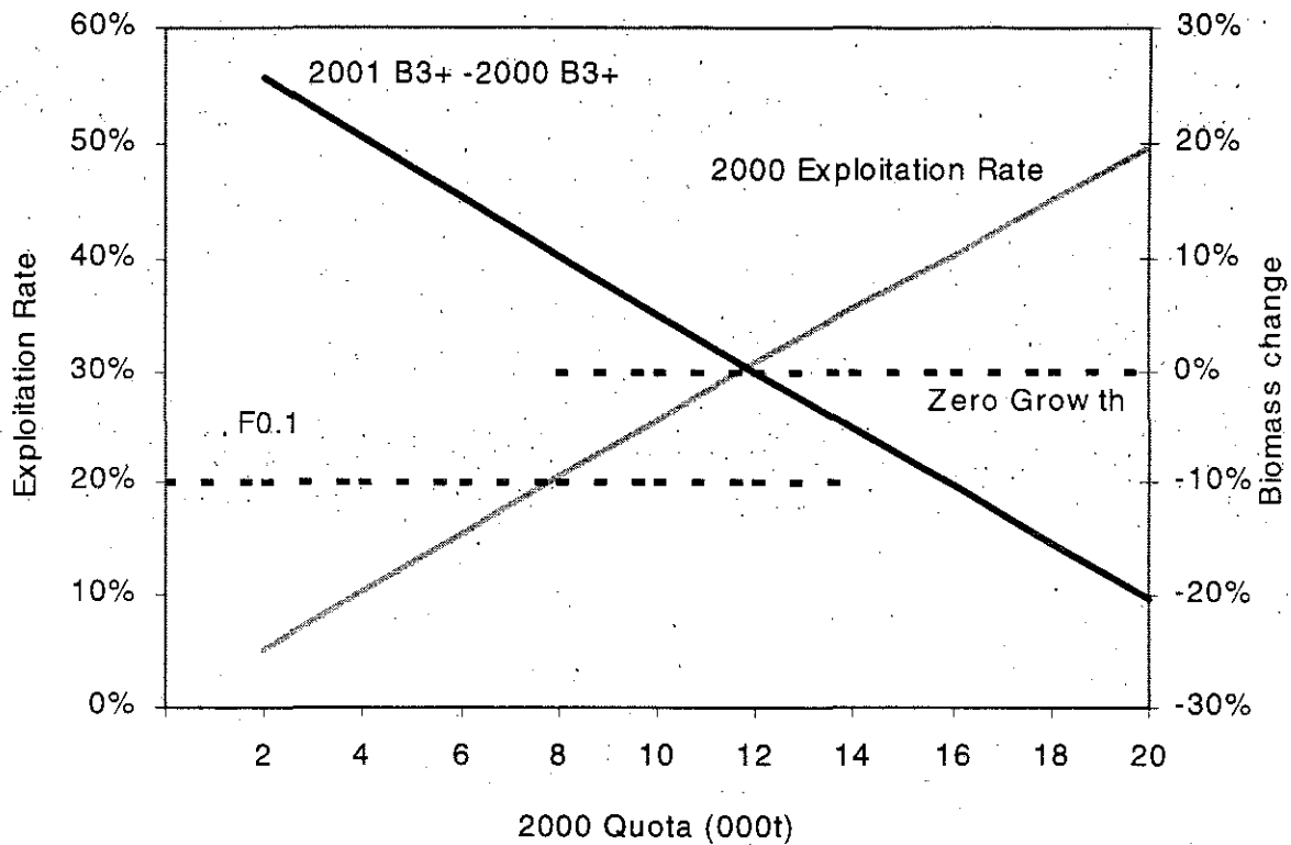
Figure 18. Implications of various 2000 quotas (combined Canada and USA) on exploitation rate and change in the 3+ population biomass of Georges Bank yellowtail flounder from 2000 to 2001.
