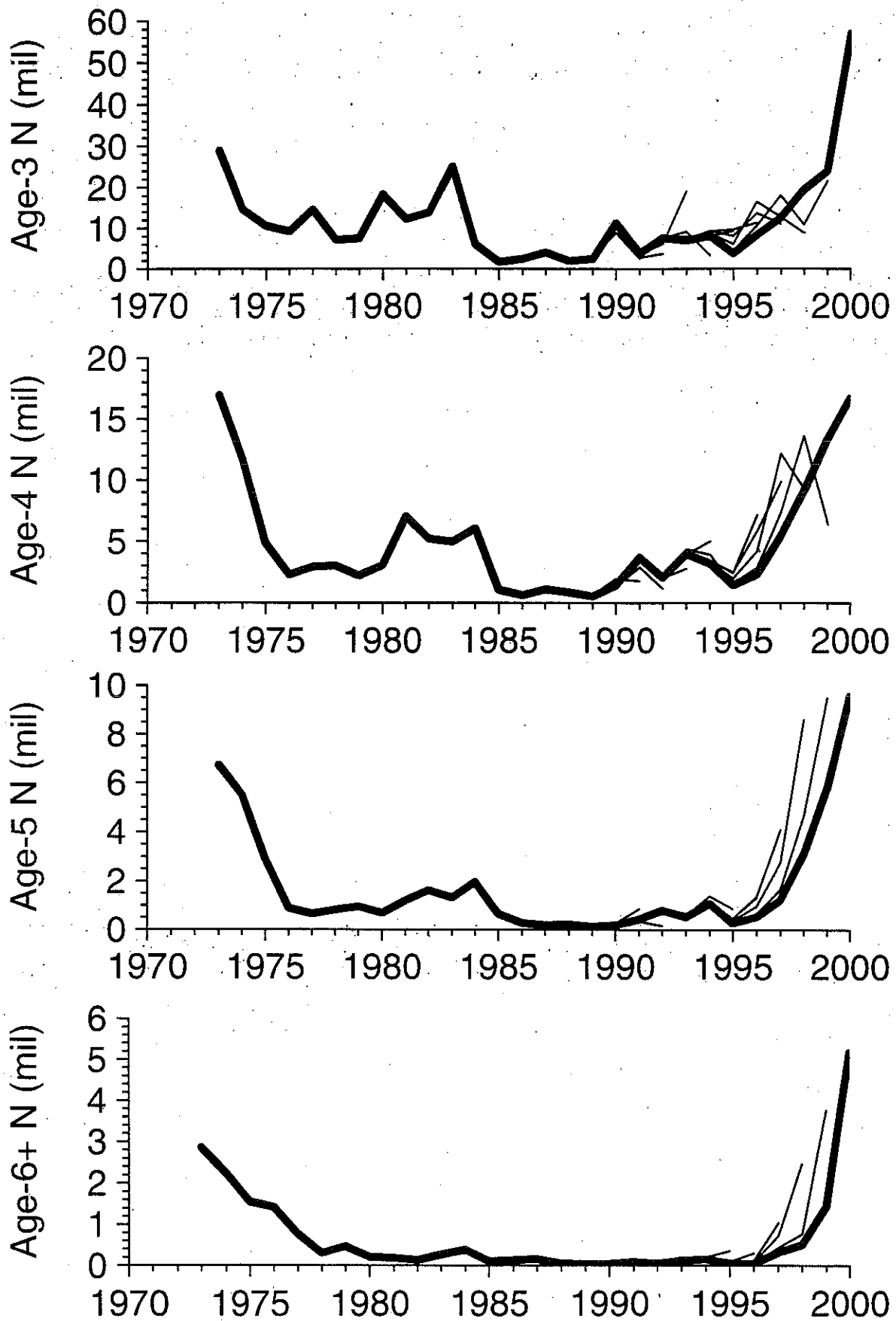
Figure 16 (cont.). Retrospective analysis of Georges Bank yellowtail flounder VPA calibration.
