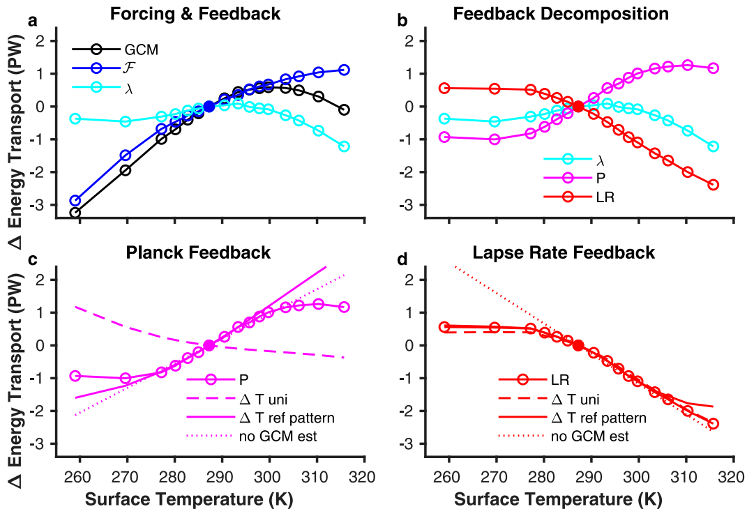
FIG. 4. (a) Change in vertically integrated northward energy transport at 50^{\circ}\text{N} with forcing (blue) and feedback (cyan) components. (b) Decomposition of the feedback-related energy transport into Planck (magenta) and lapse rate (red) feedback components. (c) Planck feedback computed using the climate-state-dependent temperature change (magenta circles), a uniform temperature change (magenta dashed), the reference temperature change pattern with varied amplitude (magenta solid), and a temperature change pattern from a moist energy balance model (magenta dotted). (d) Lapse rate feedback computed using the climate-state dependent temperature change (red circles), a uniform temperature change (red dashed), the reference temperature change pattern with varied amplitude (magenta solid), and a moist adiabatic temperature change with uniform surface warming (red dotted).
