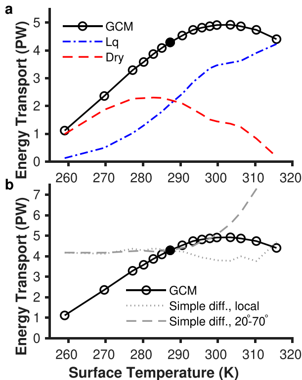
FIG. 1. (a) Vertically integrated northward energy transport at 50^\circ\text{N} for GCM simulations (black) indicated by their global-mean surface temperature, with latent energy (blue) and dry static energy (red) transport components. (b) Evaluation of the constant-diffusivity simple diffusive closure, (5), using the mean moist static energy gradients at the lowest atmospheric level and local 50^\circ\text{N} gradients (gray dotted line) or a bulk extratropical difference between 20^\circ and 70^\circ (gray dashed line).
