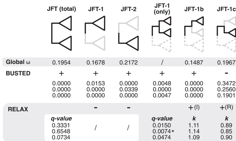
Fig. 4. —Summary of global dN/dS , BUSTED, and RELAX results using HyPhy. Global dN/dS values shown for each focal clade. FDR-corrected P -values ( q -values) are shown for the three subsets in both BUSTED and RELAX tests. For RELAX tests, q -values shown are the same given the FDR-correction was only for two tests (JFT-1 vs. JFT-1, JFT-1b vs. JFT-1c); for example, q -values in the white box are the same for both JFT-1 versus JFT-2 and JFT-2 versus JFT-1. For significant RELAX tests ( q -value < 0.05 ) (in gray), k parameters are shown. For k > 1 , selection strength has been intensified, and for k < 1 , selection strength has been relaxed. I = intensification of selection. R = relaxation of selection. (*) indicates RELAX tests run on Datamonkey server v2 (accessed January 2021; Weaver et al. 2018). Slashes indicate no data shown. Uncorrected P -values and k parameters for all RELAX tests are shown in supplementary table S5, Supplementary Material online.
