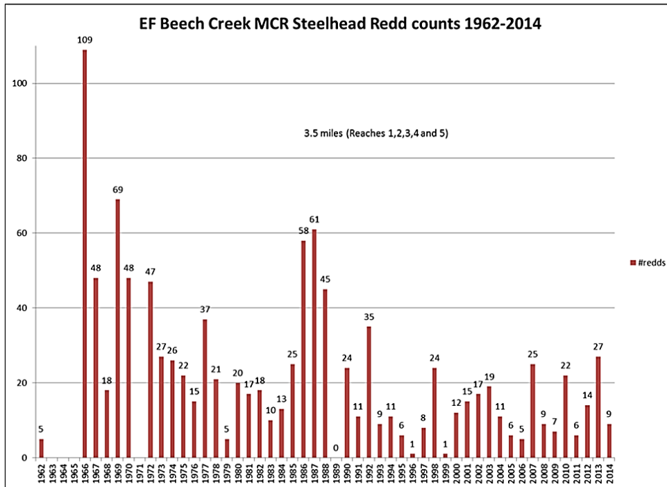
Figure 5. Number of MCR steelhead redds counted within East Fork Beech Creek ODFW index reaches 1962 to 2014.
