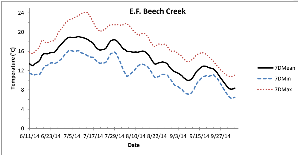
Figure 3. Graph of water temperature data from 6/11/2014 to 10/5/2014 in East Fork Beech Creek
