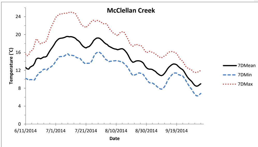
Figure 2. Graph of water temperature data from 6/11/2014 to 10/5/2014 in McClellan Creek.
