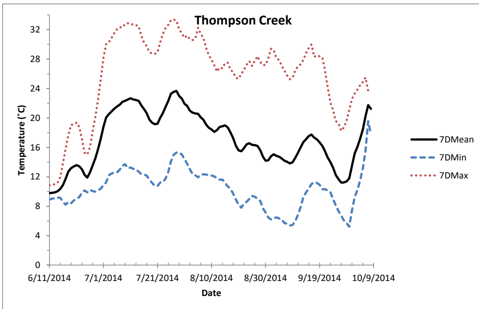
Figure 4. Graph of water temperature data from 6/11/2014 to 10/8/2014 in Thompson Creek.
