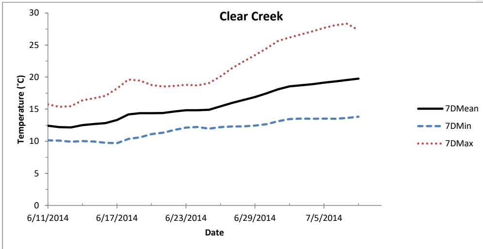
Figure 1. Graph of water temperature data from 6/11/2014 to 7/8/2014 in Clear Creek.
