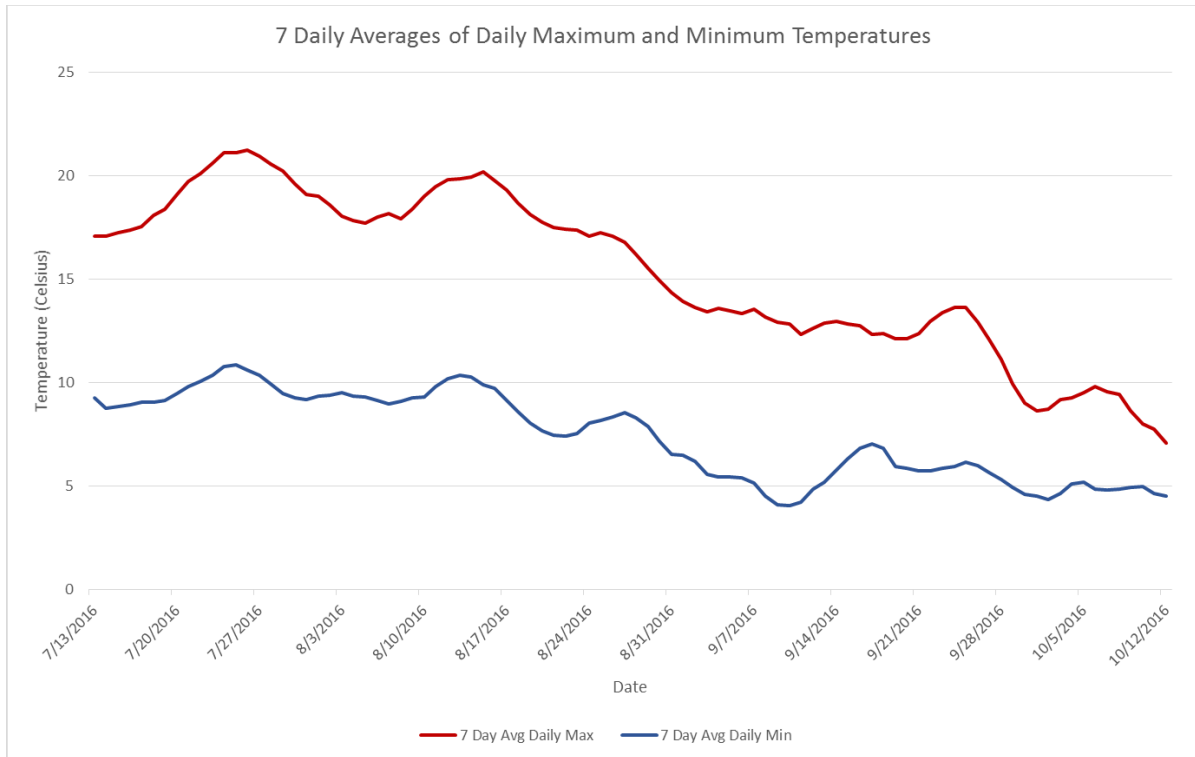
Figure 2. Graph of water temperature data from 7/13/2016 to 10/12/2016 in Dark Canyon Creek.
