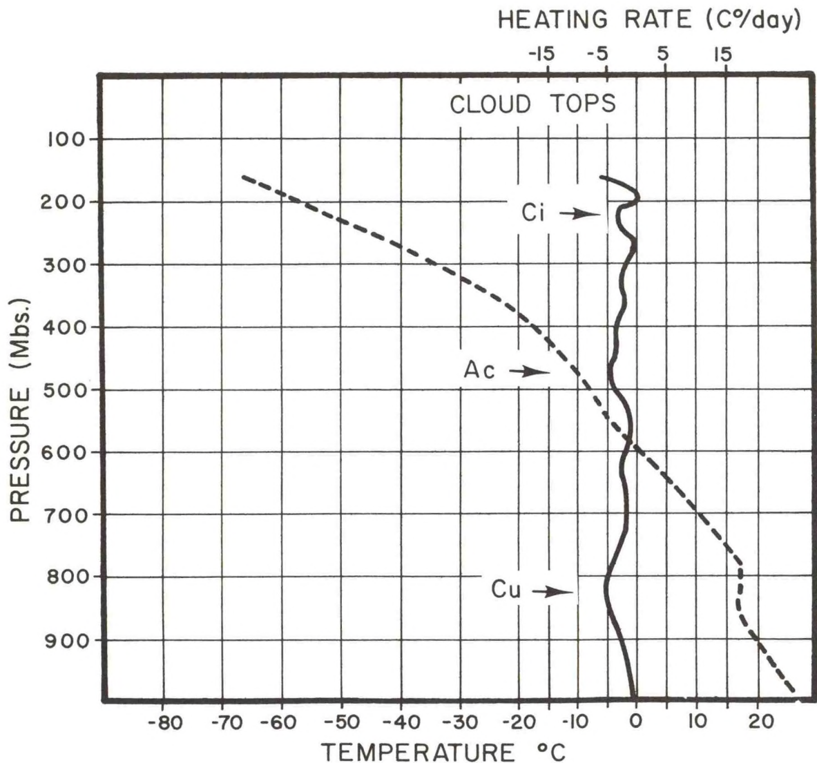
Figure 11.--IR radiometersonde run on the Rockaway June 23, 1969.
