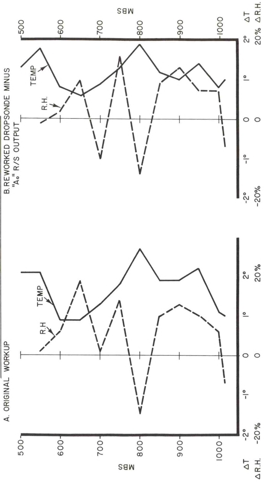
Figure 5. Comparison between sample rawinsonde and dropsonde data.
