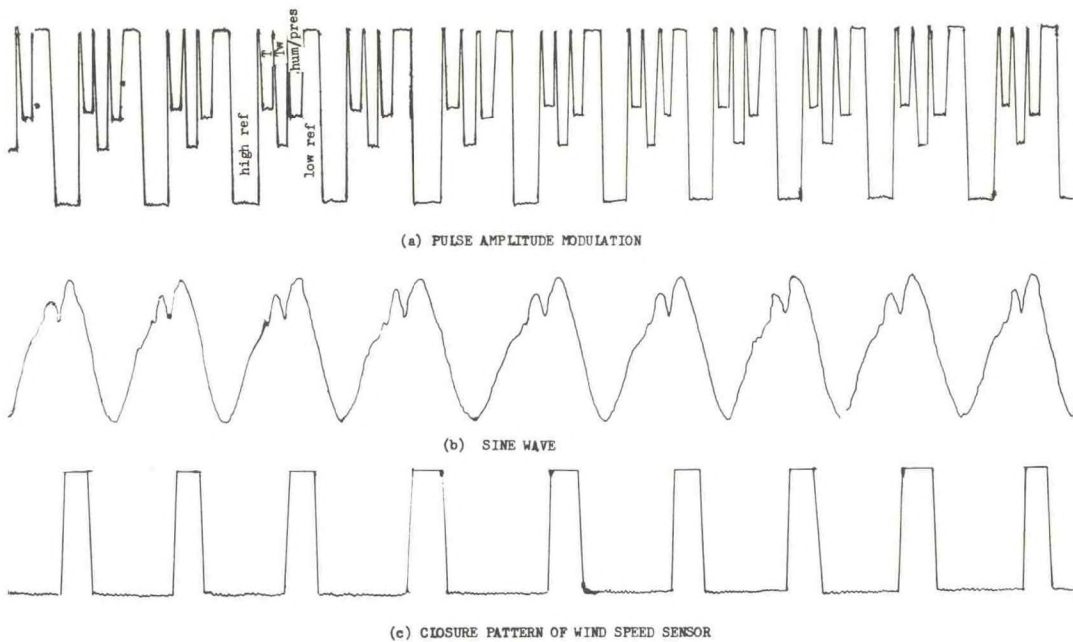
Figure 17.--Typical analog output of BLIP data.
