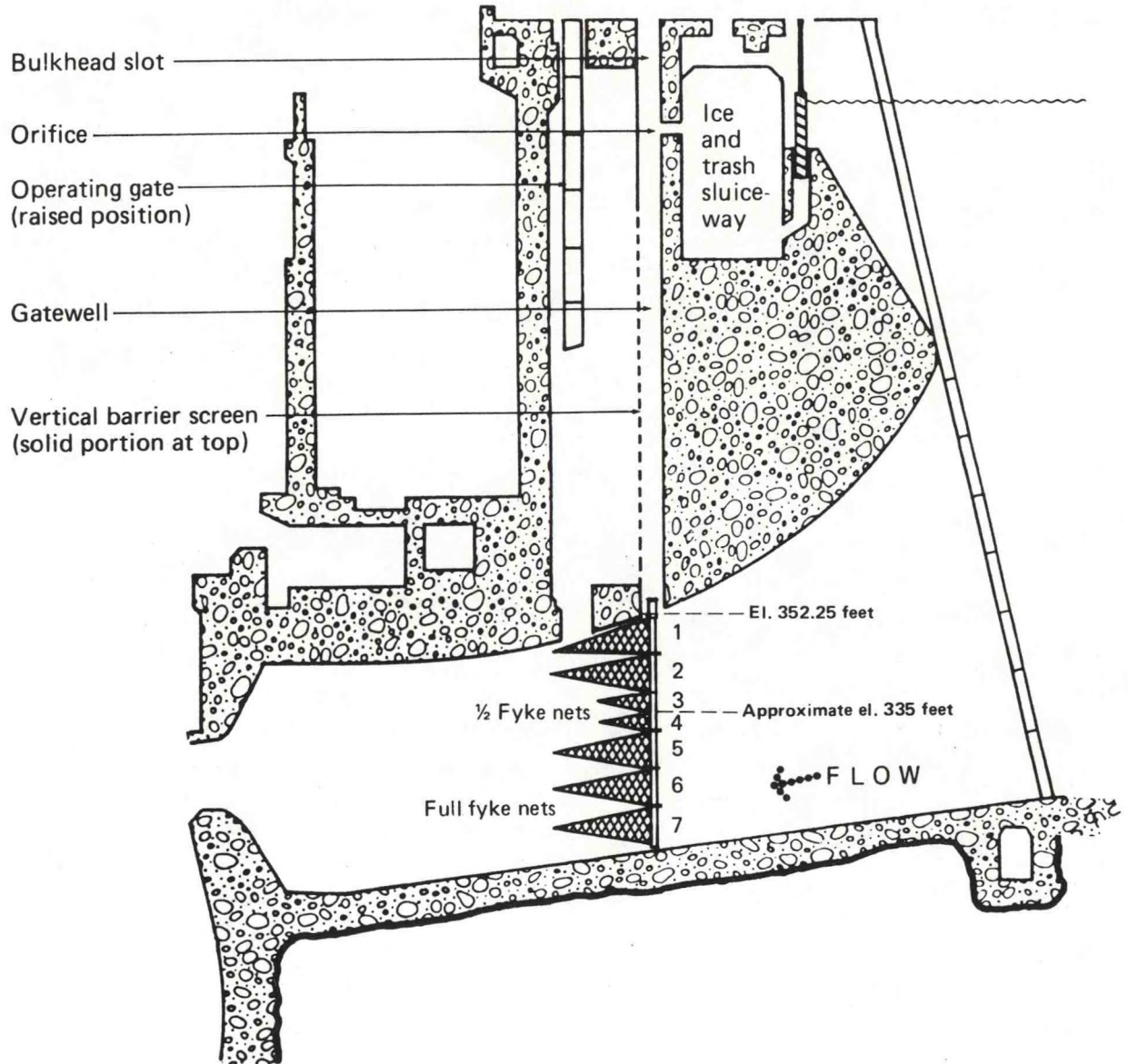
Figure 3.--Cross-section of a turbine intake at Ice Harbor Dam with a vertical distribution frame and fyke nets, 1987.
