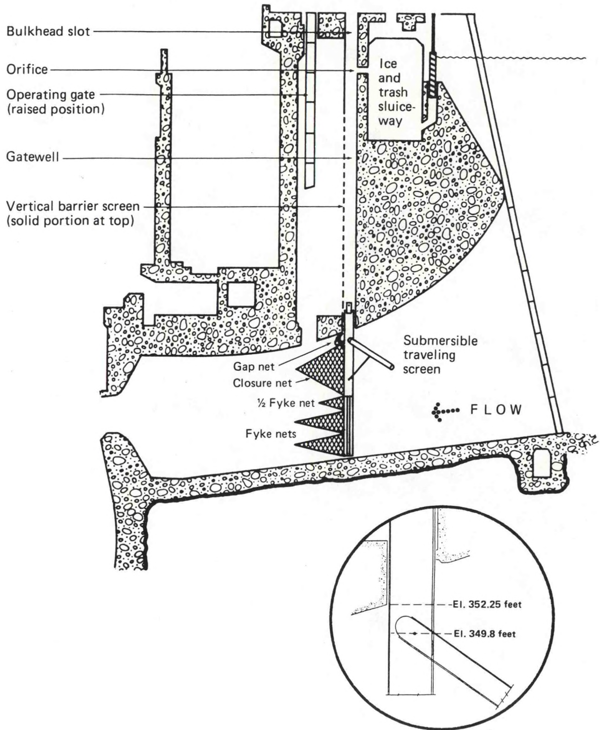
Figure 2.--Cross-section of a turbine intake with a submersible traveling screen and attached nets at Ice Harbor Dam, 1987.
