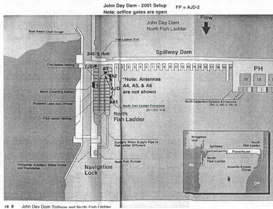
Appendix Figure A3. The Dalles Dam South and West ladder entrances (above) and John Day Dam North ladder (below).
