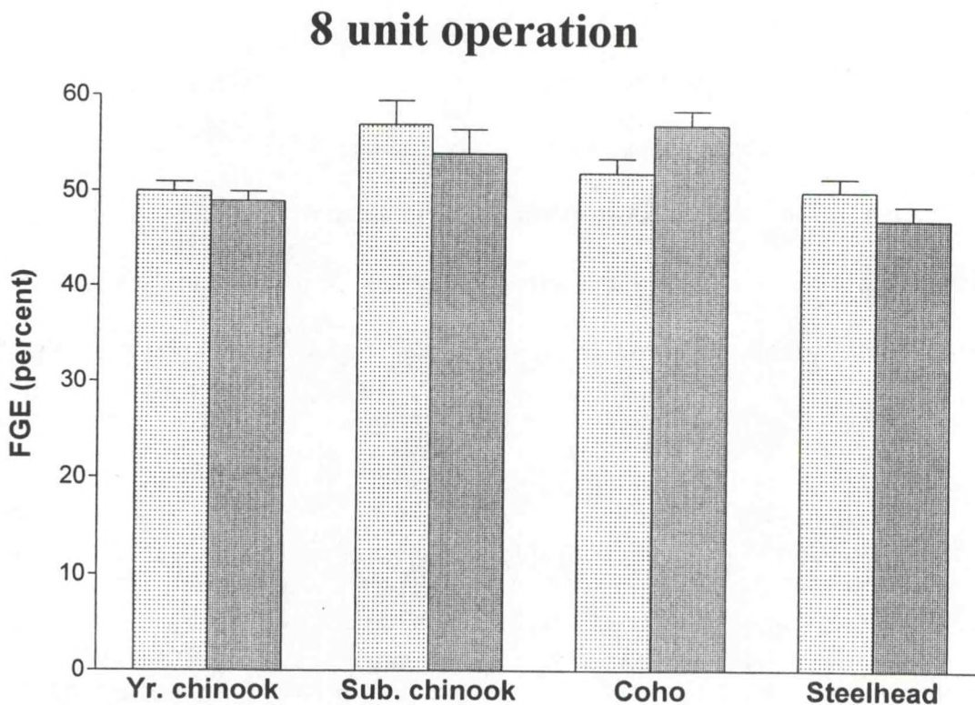
Figure 4. Mean Fish Guidance Efficiency (FGE) and standard errors in gatewells with and without turbine intake extensions (TIES) for four and six unit operation combined and eight unit operation at Bonneville Dam Second Powerhouse in spring 1993 (* denotes significant difference between TIE and non-TIE, \alpha = 0.05 ).
