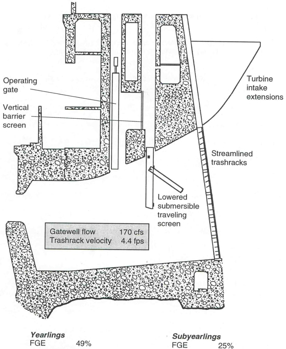
Figure 6. Cross-section of turbine intake at Bonneville Dam Second Powerhouse showing permanent modifications and resulting Fish Guiding Efficiency (FGE) values (in Unit 15) for yearling chinook (in spring) and subyearling chinook salmon (in summer).
