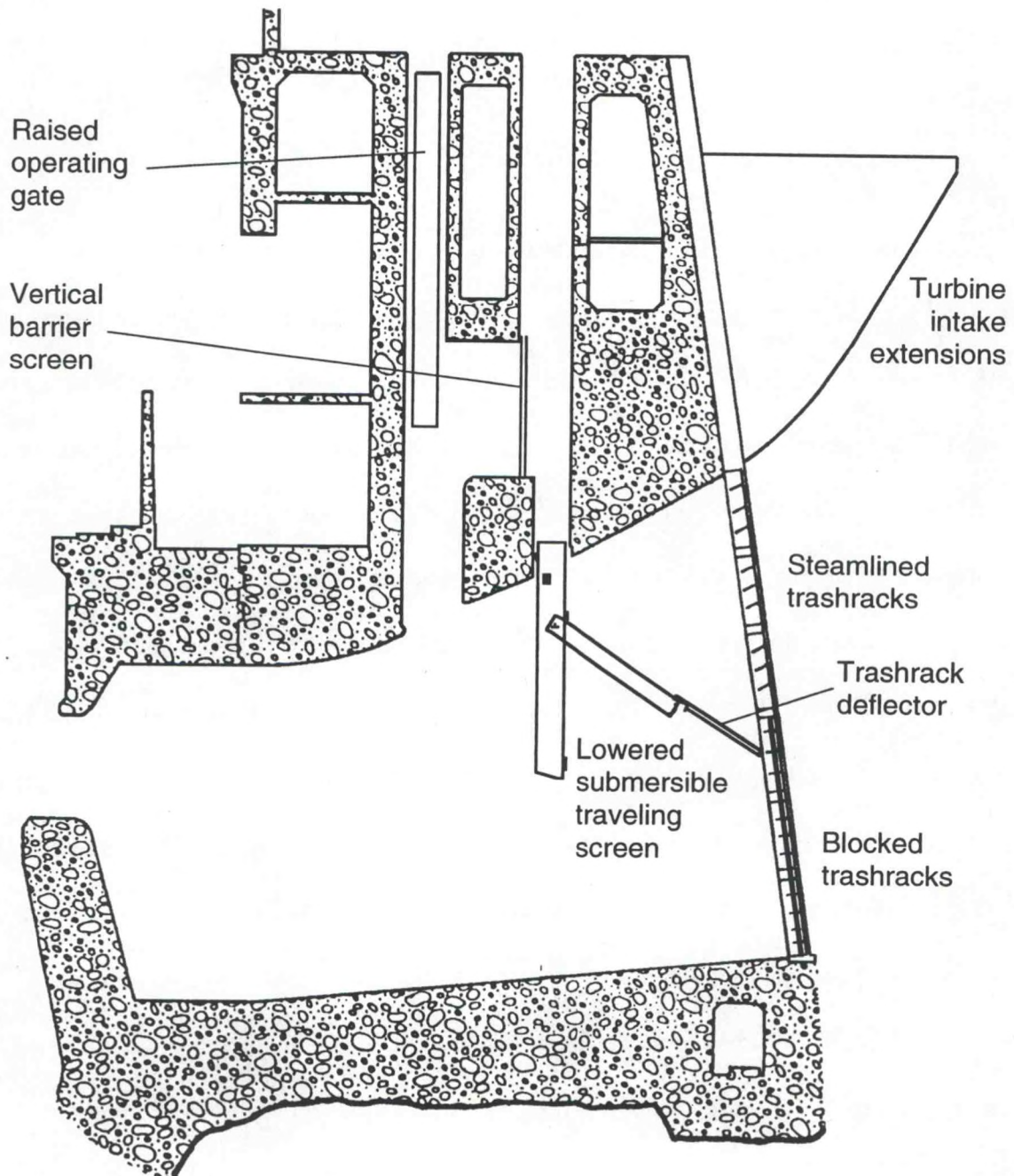
Figure 2. Cross-section of turbine intake at Bonneville Dam Second Powerhouse showing structural modifications tested from 1984 to 1989 to improve Fish Guiding Efficiency (FGE).
