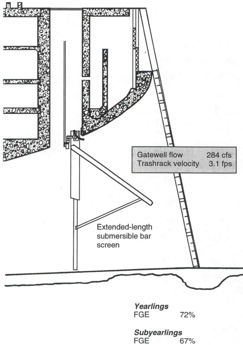
Figure 9. Cross-section of turbine intake at Bonneville Dam First Powerhouse showing extended length submersible bar screen and no operating gate, tested in 1998, with resulting Fish Guiding Efficiency (FGE) results for yearling and subyearling chinook salmon.
