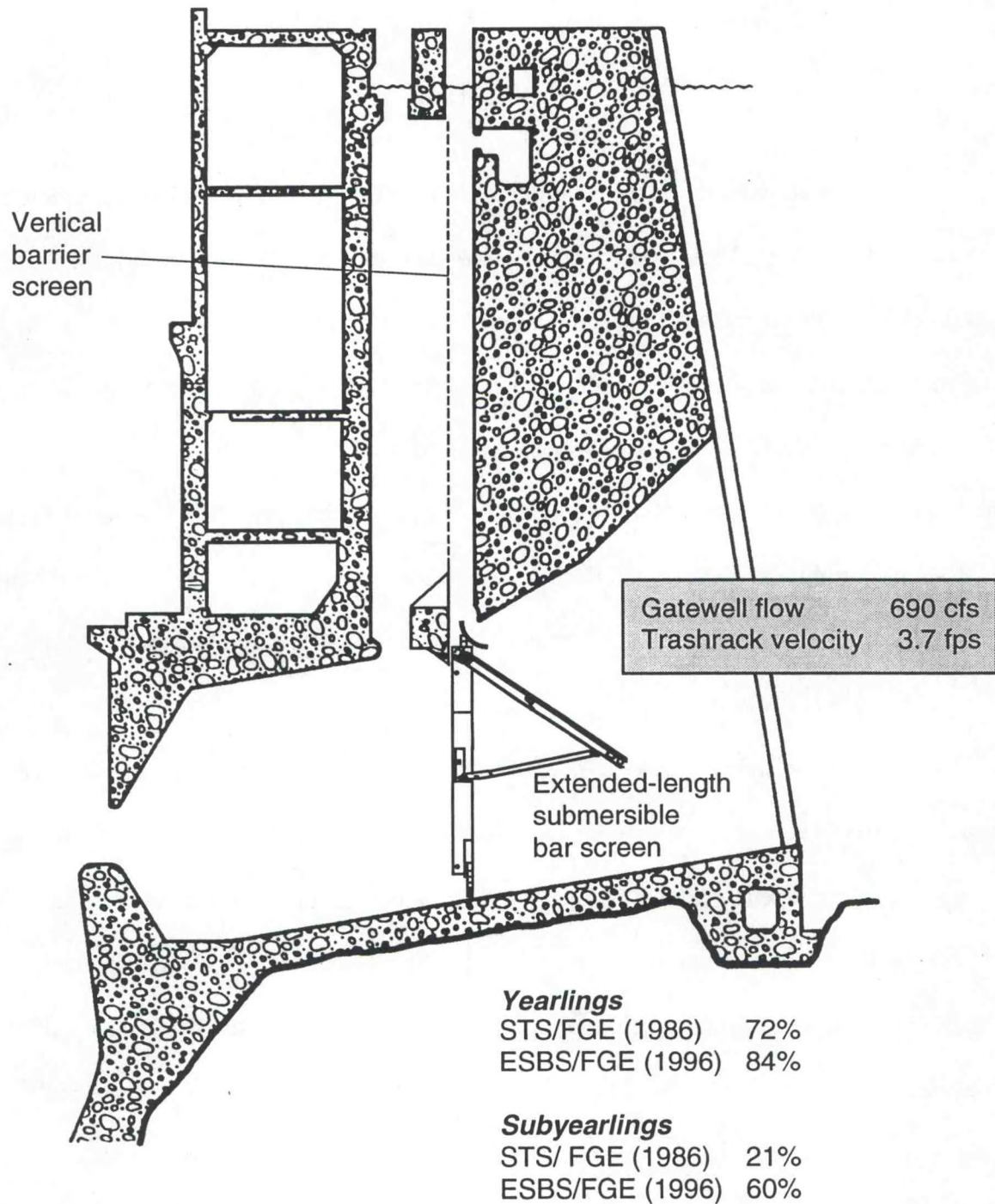
Figure 10. Cross-section of turbine intake at John Day Dam showing extended- length bar screen tested in 1996 with resulting Fish Guiding Efficiency (FGE) values for yearling and subyearling chinook salmon (including results from 1986 testing with submersible traveling screen).
