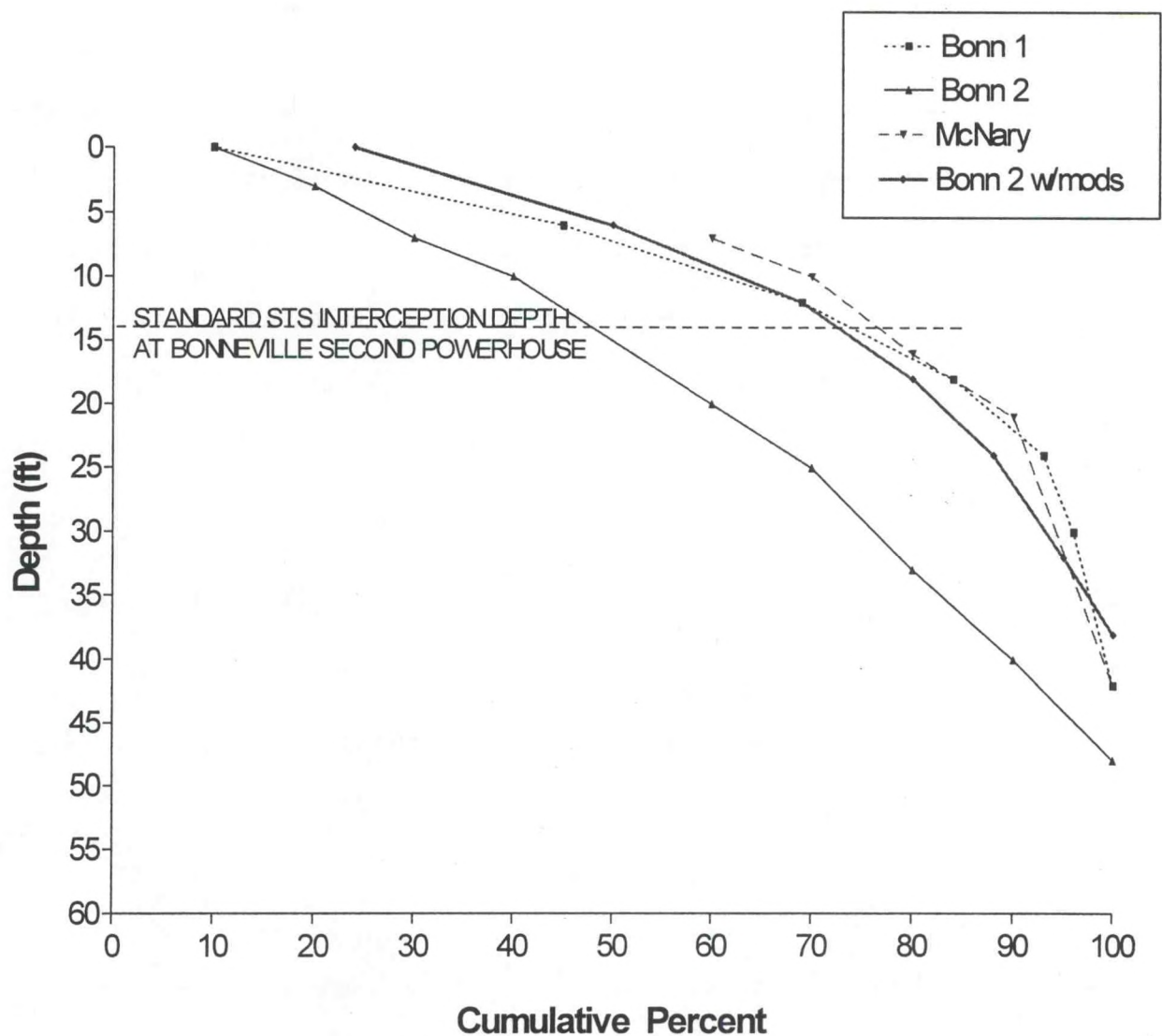
Figure 7. Vertical distribution of yearling chinook salmon (cumulative percent) in intakes at Bonneville Dam First Powerhouse, Second Powerhouse (with and without modifications), and McNary Dam.
