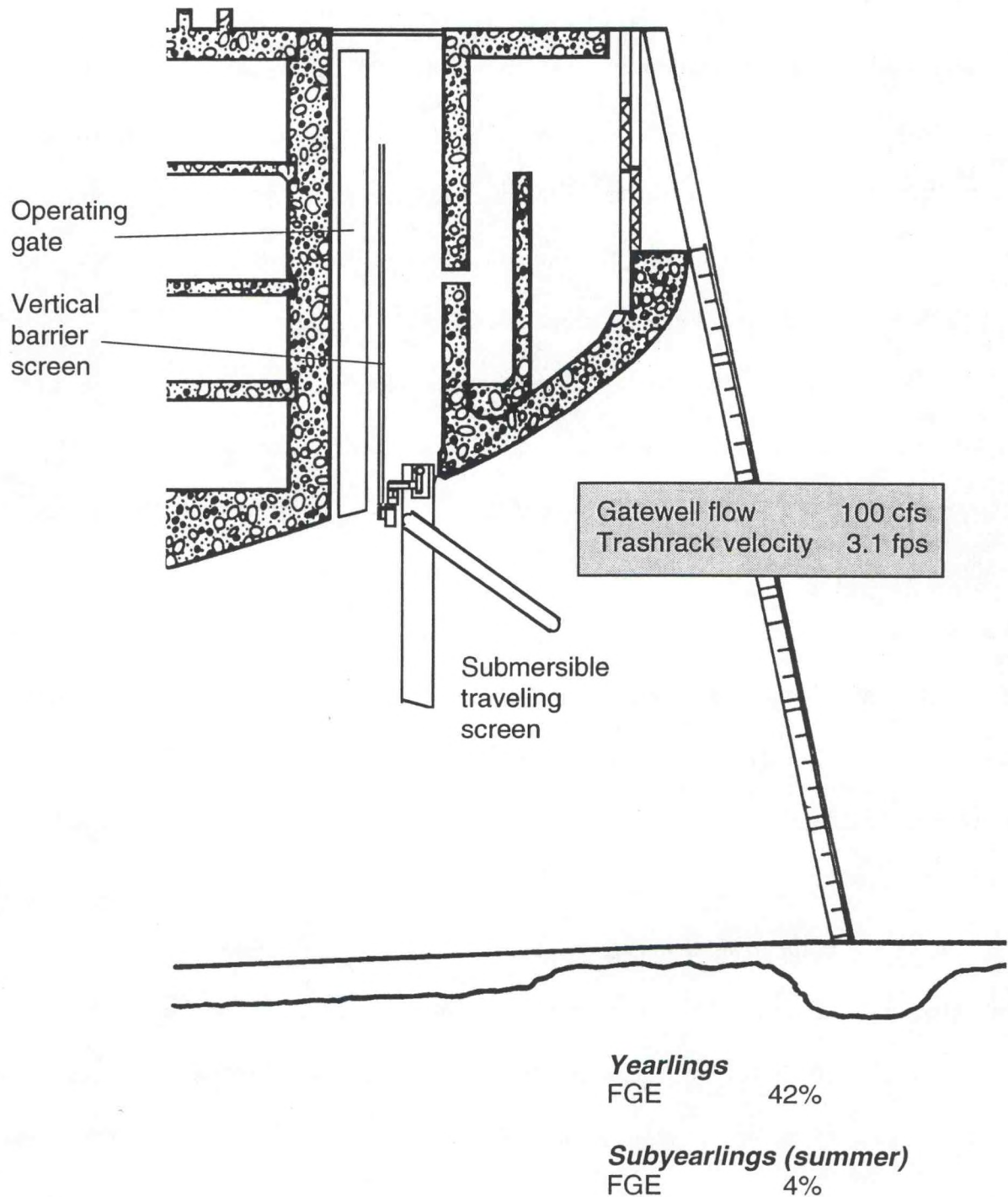
Figure 8. Cross-section of turbine intake at Bonneville Dam First Powerhouse showing fish bypass system and 1989 Fish Guiding Efficiency (FGE) results.
