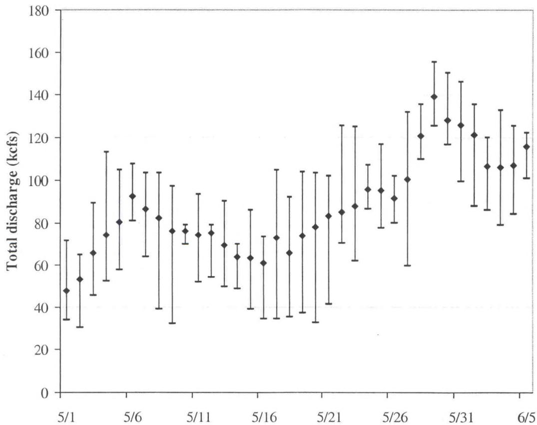
Figure 4. Average daily total project discharge at Ice Harbor Dam during the 2004 spillway passage survival study (whisker bars represent the range of operations for each day).
