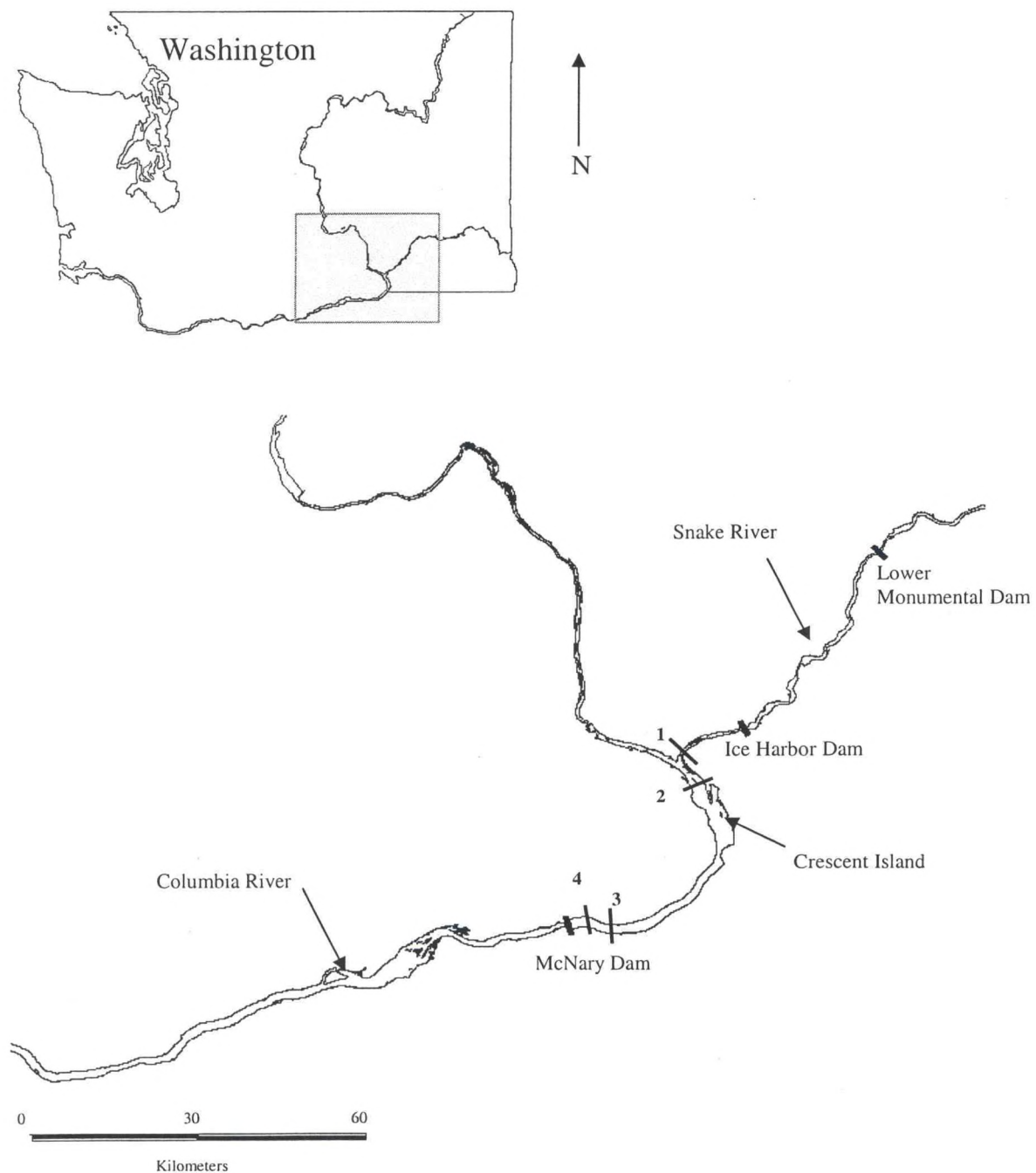
Figure 1. Study area showing location of radiotelemetry transects used for estimating survival at Ice Harbor Dam, 2007. (Note: 1 = Mouth of the Snake River at Sacajawea Park, WA, rkm 523; 2 = Columbia Bank, WA, rkm 518; 3 = McNary Beach, OR, rkm 477 ;4 = McNary Dam Forebay, rkm 472.)
