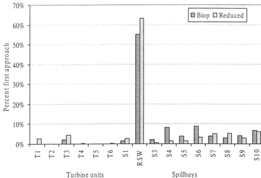
Figure 6. Approach patterns for radio-tagged, river-run subyearling Chinook salmon in the forebay of Ice Harbor Dam, 2007.
