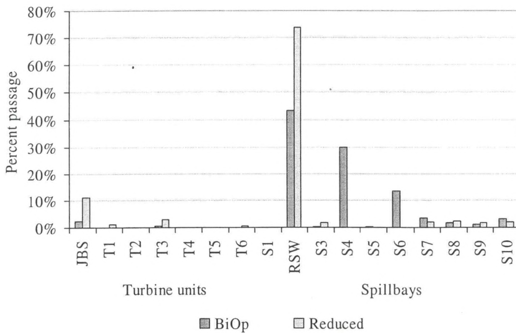
Figure 8. Individual passage route distribution for radio-tagged, river-run subyearling Chinook salmon during spill testing at Ice Harbor Dam, 2007.
