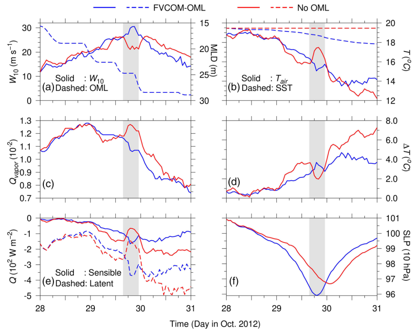
Figure 9. Time series of the 10-m wind speed (solid lines in a) and mixed layer depth (dashed line in a), 2-m air temperature (solid lines in b) and sea surface temperature (dashed lines in b), vapor ratio (c), sea air temperature difference (d), latent heat flux (dashed lines in e) and sensible heat flux (solid lines in e), and sea level pressure (f) at a selected location (shown in Figure 7) over the period from 0000 UTC 28 October to 2100 UTC 31 October. The results of the case with OML are shown in blue and the case without OML in red.
