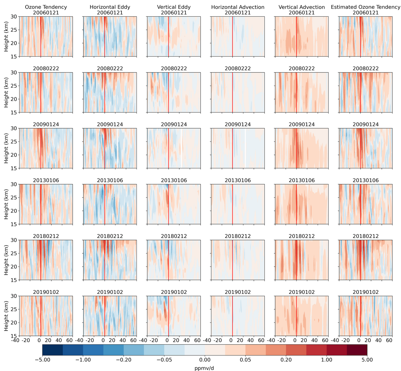
Figure 11. Same as Fig. 8 for ozone tendency, horizontal and vertical component of eddy mixing, horizontal ( -\bar{v}^*x_y ) and vertical ( -\bar{w}^*x_z ) component of mean advection, and the indirect ozone tendency using the right-hand side of Eq. (2). Summing four middle columns leads to the estimated ozone tendency on the sixth column. The vertical axis is the log-pressure height.
