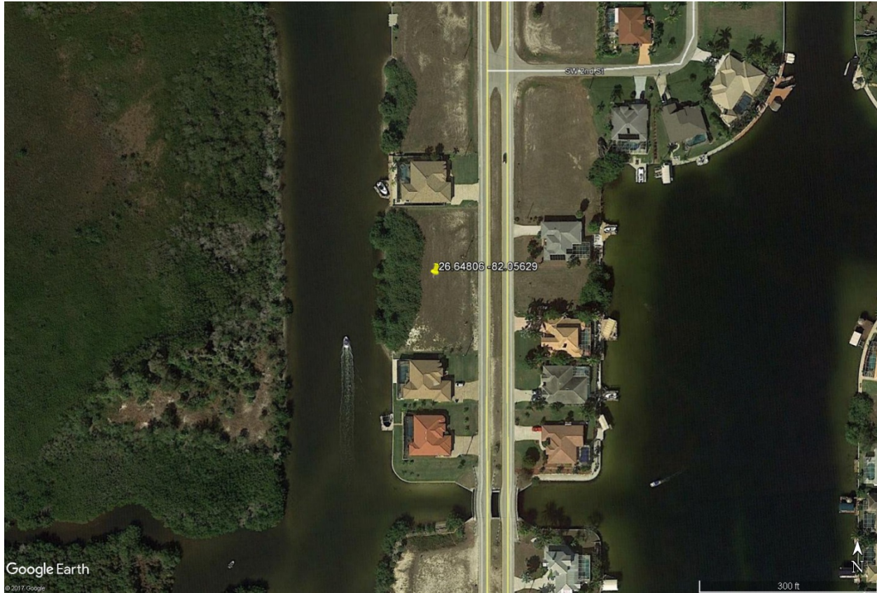
Figure 1. Image showing the Mochrie Seawall project site location in the North Spreader Waterway in Cape Coral, Lee County, Florida (©2016 Google).
