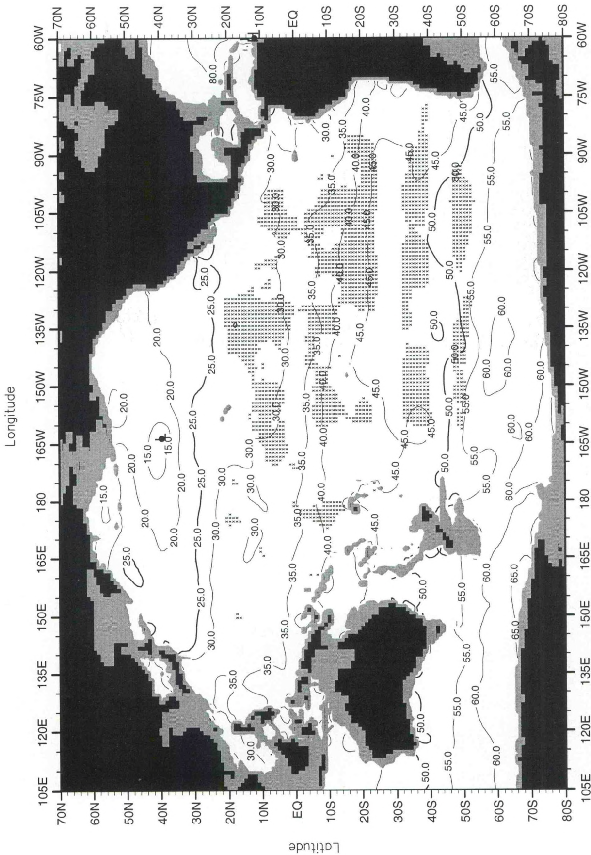
Fig. G13. Annual mean oxygen saturation (%) at 2000 m. depth .
