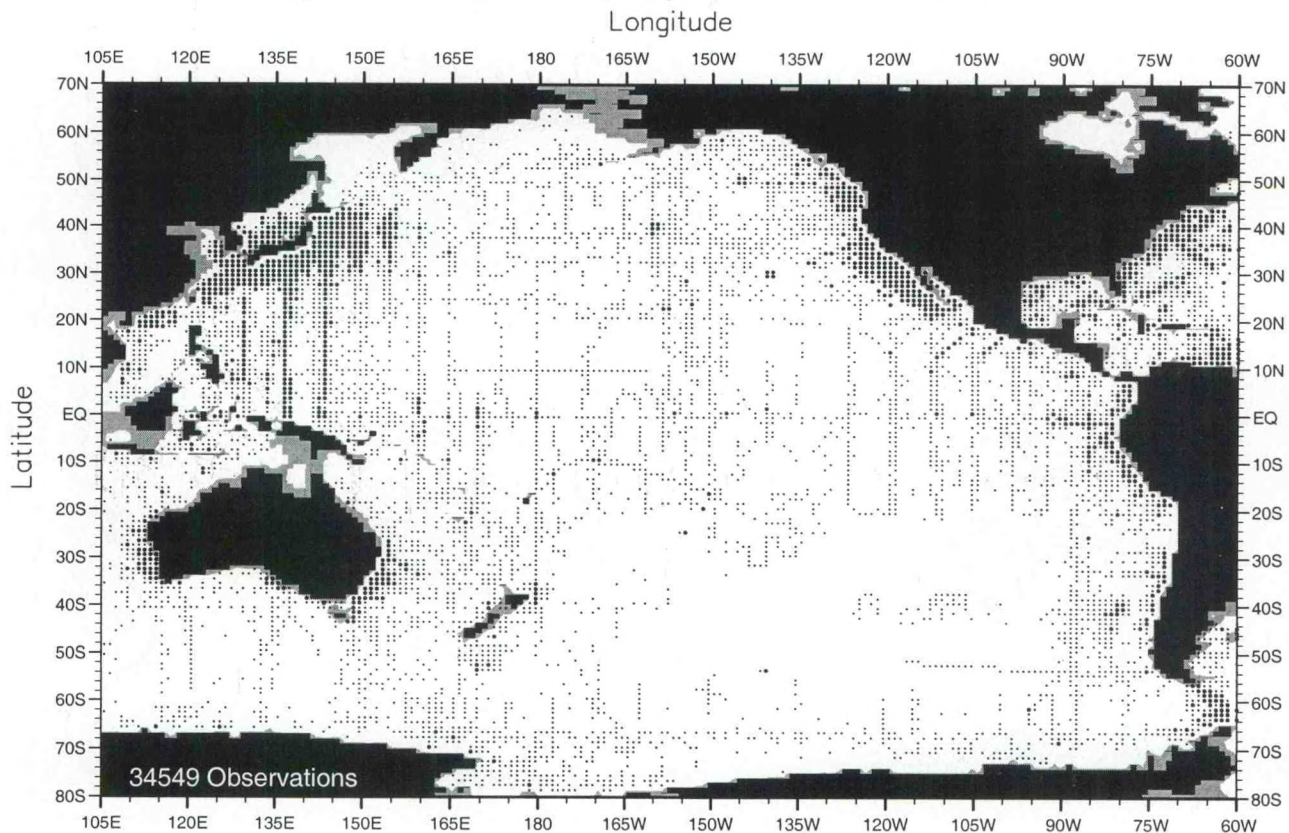
Fig. B2. Winter (Jan.-Mar.) oxygen observations at 75 m. depth .
