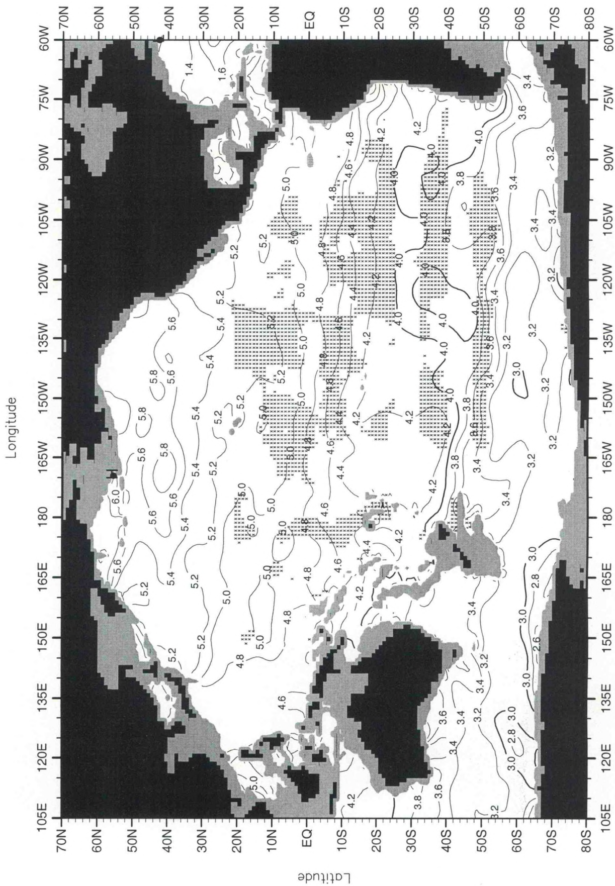
Fig. D14. Annual mean Apparent Oxygen Utilization (ml/l) at 2500 m. depth .
