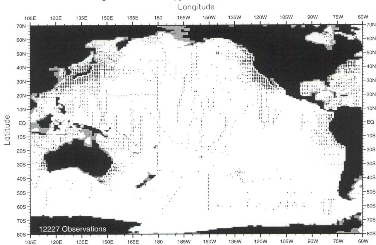
Fig. C20. October oxygen observations at 75 m. depth .
