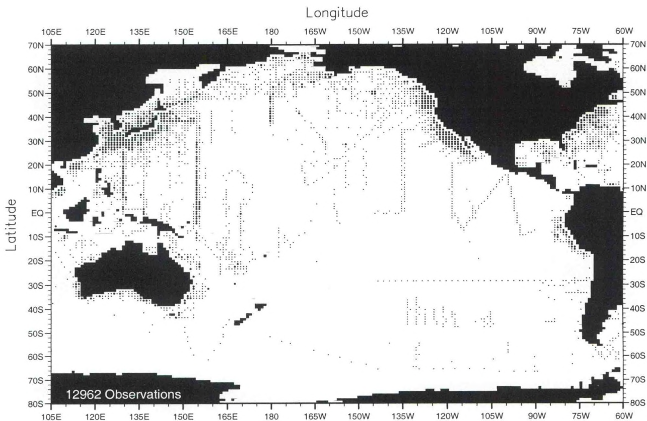
Fig. C11. June oxygen observations at the surface .
