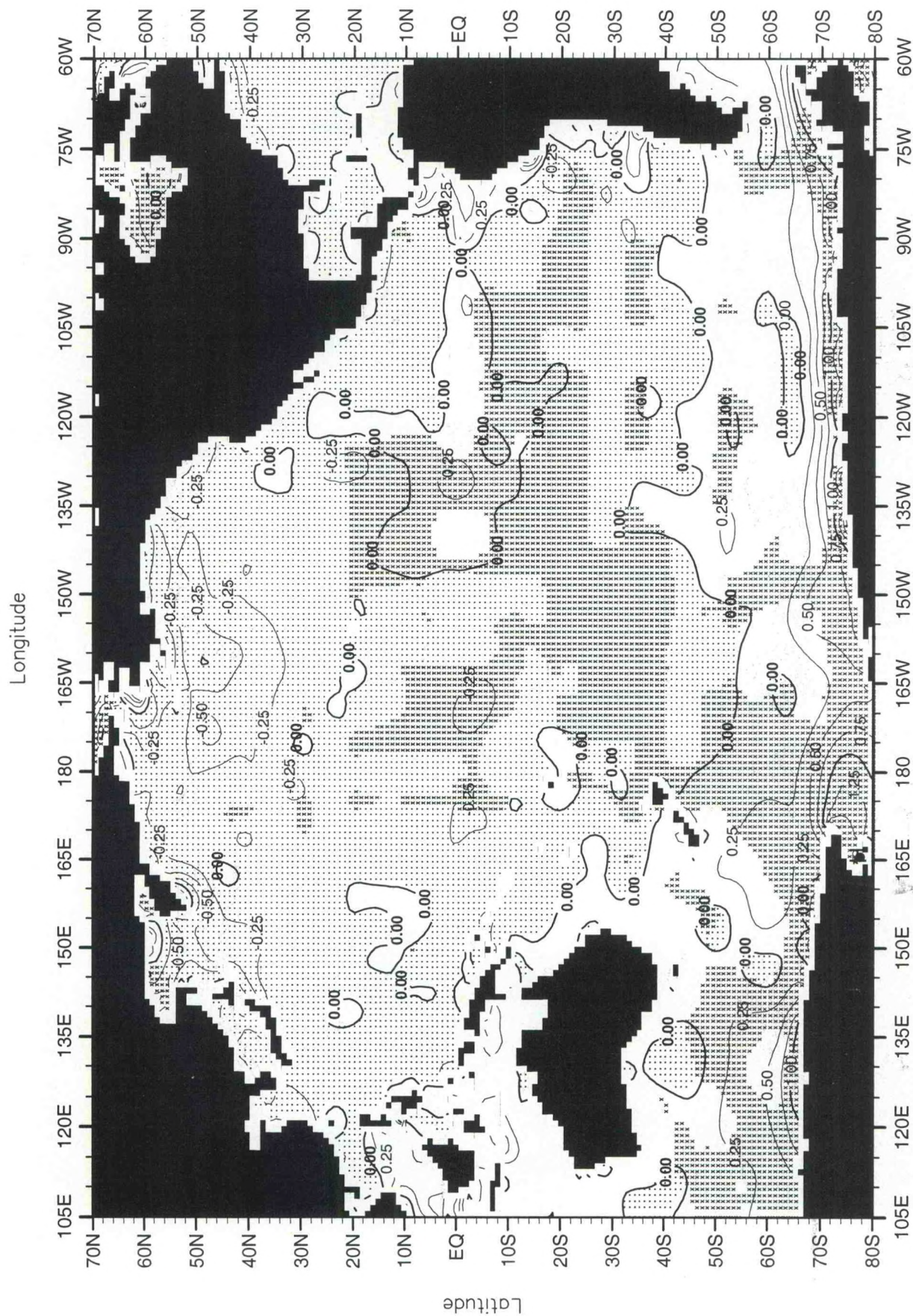
Fig. E5. Spring (Apr.-Jun.) mean Apparent Oxygen Utilization (ml/l) at the surface .
