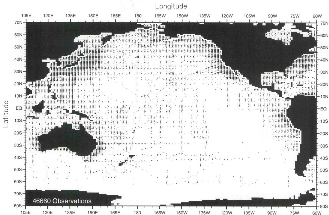
Fig. B9. Summer (Jul.-Sep.) oxygen observations at the surface .
