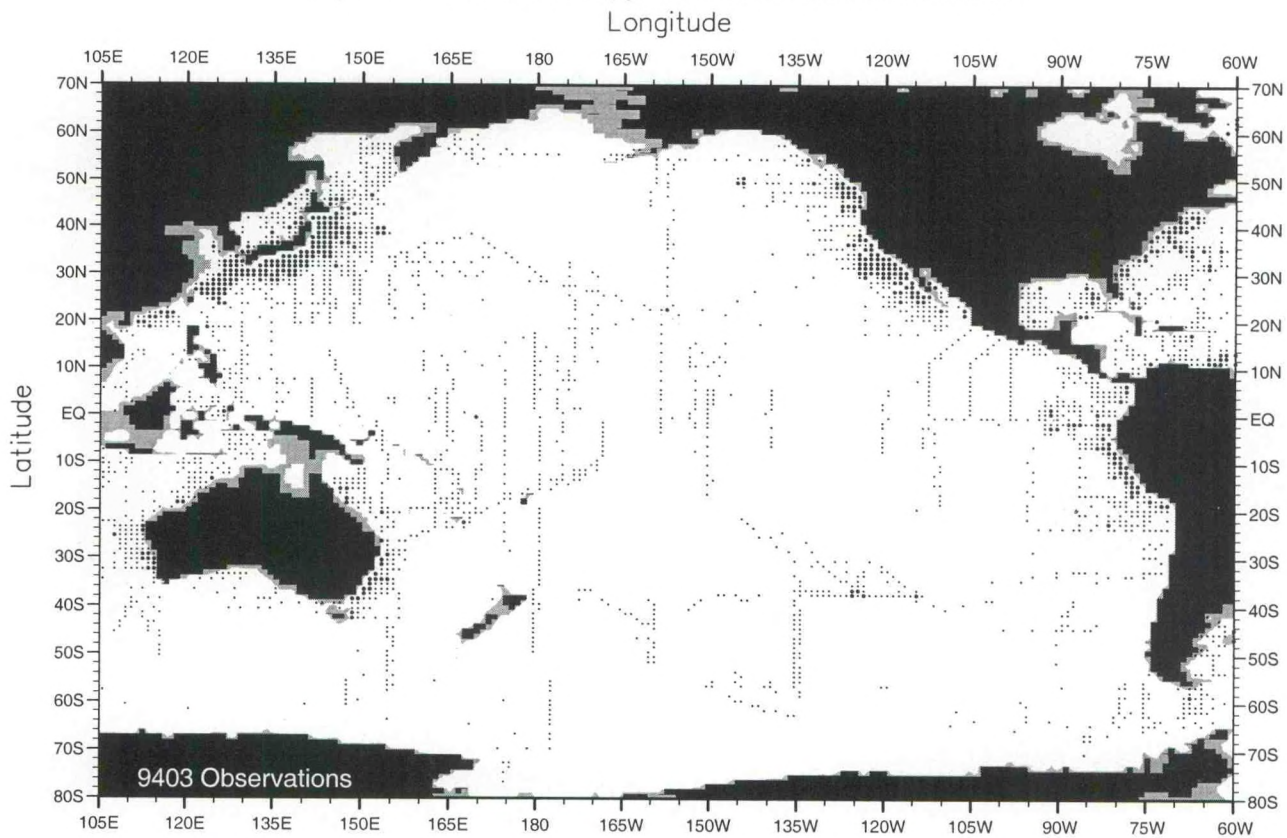
Fig. C22. November oxygen observations at 75 m. depth .
