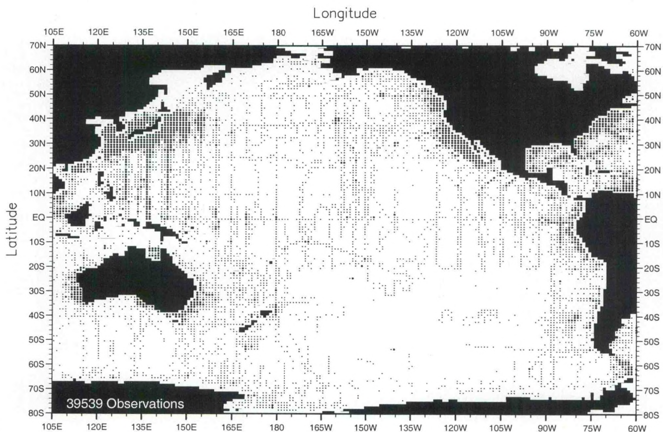
Fig. B1. Winter (Jan.-Mar.) oxygen observations at the surface .
