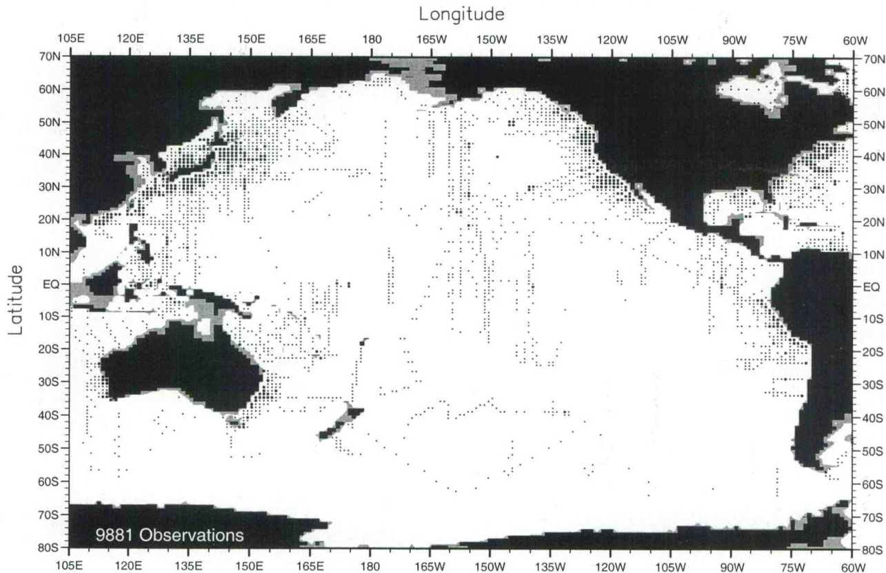
Fig. C18. September oxygen observations at 75 m. depth .
