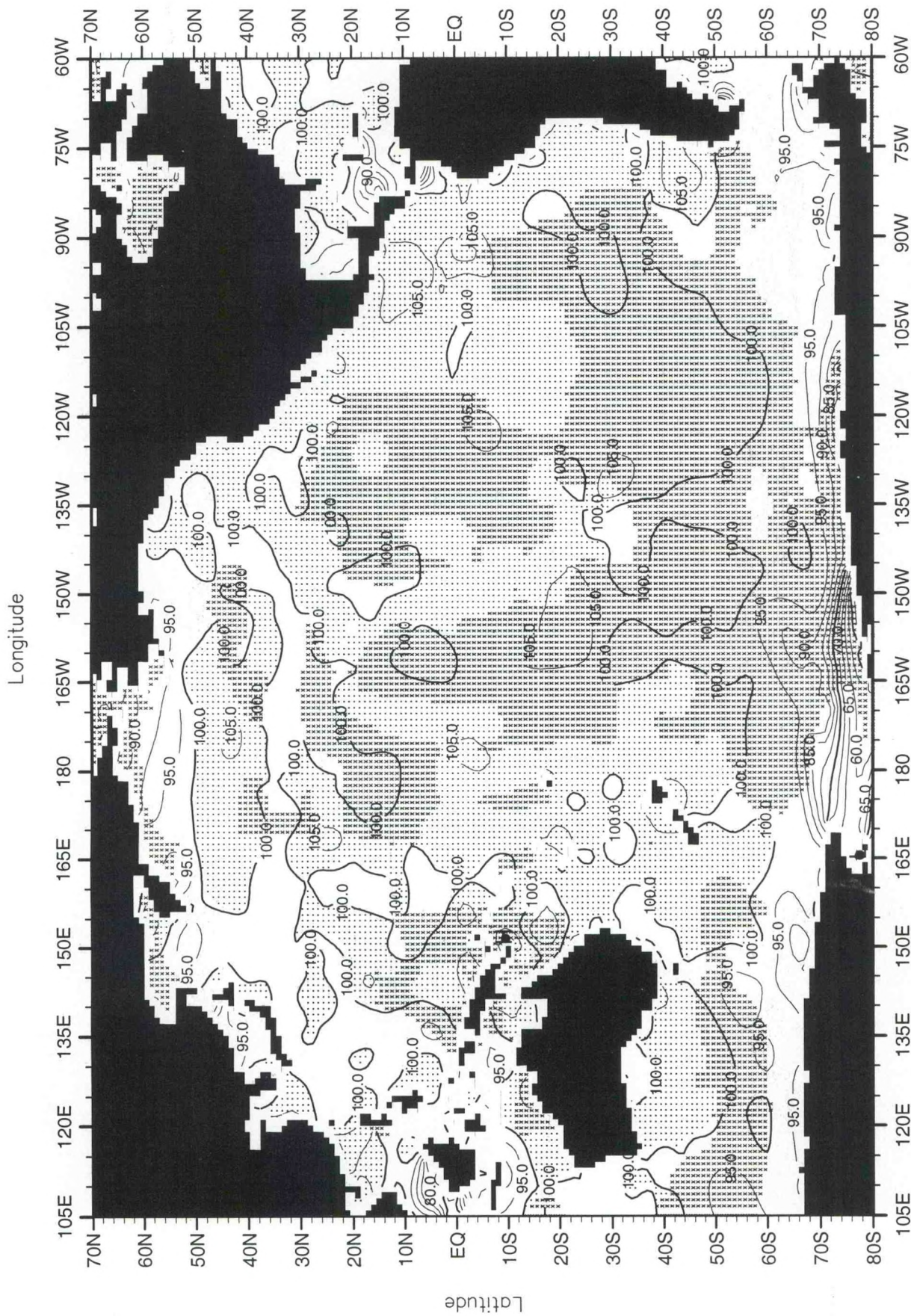
Fig. 15. March mean oxygen saturation (%) at the surface .
