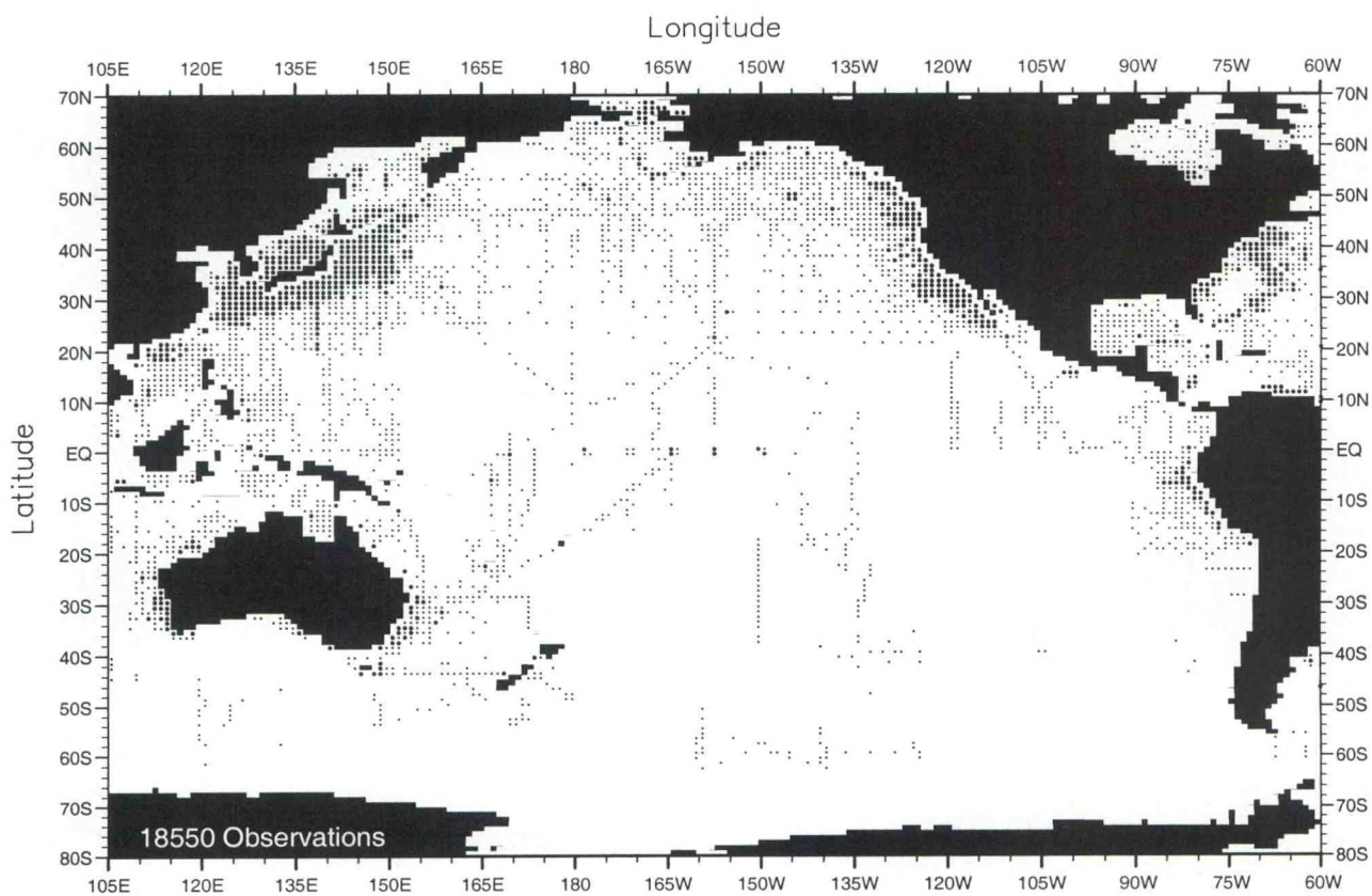
Fig. C15. August oxygen observations at the surface .
