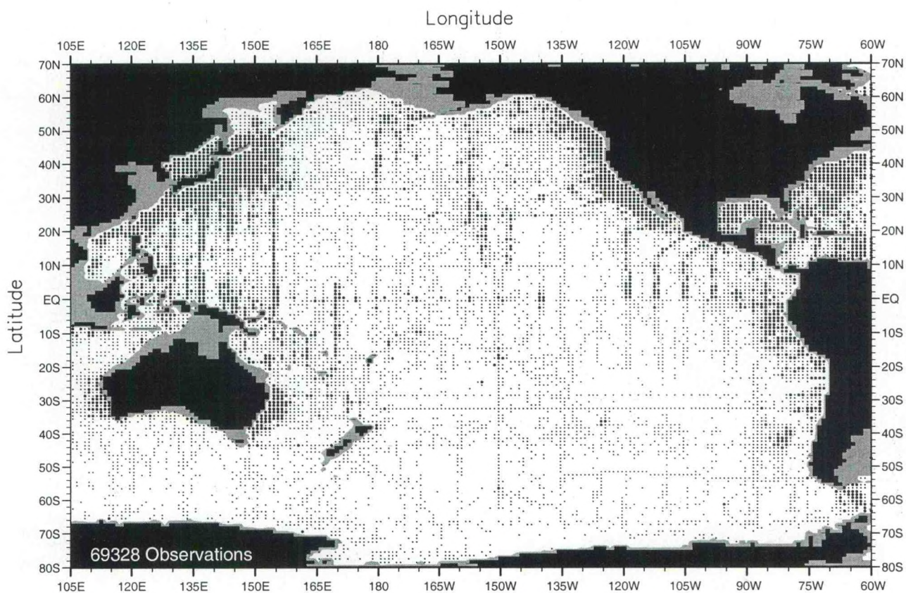
Fig. A9. Annual oxygen observations at 500 m. depth .
