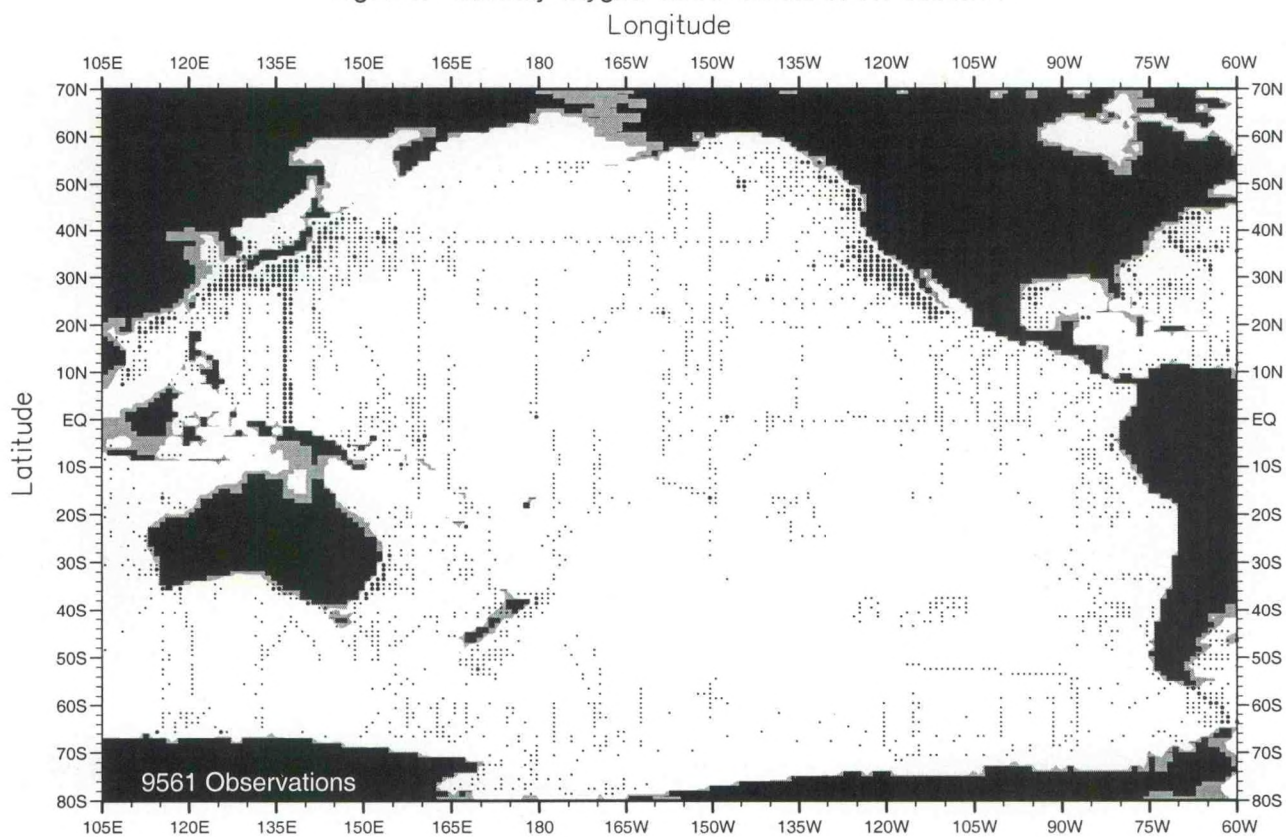
Fig. C2. January oxygen observations at 75 m. depth .
