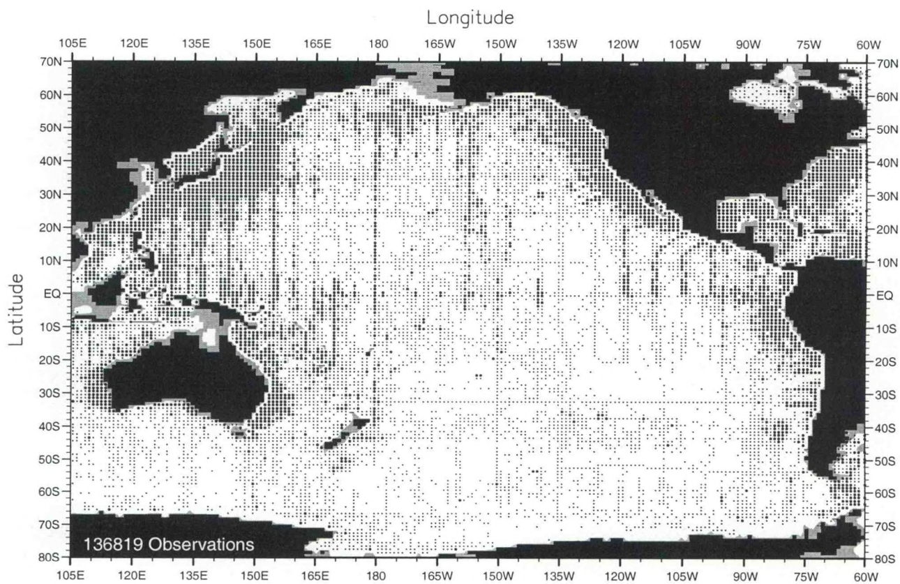
Fig. A3. Annual oxygen observations at 75 m. depth .
