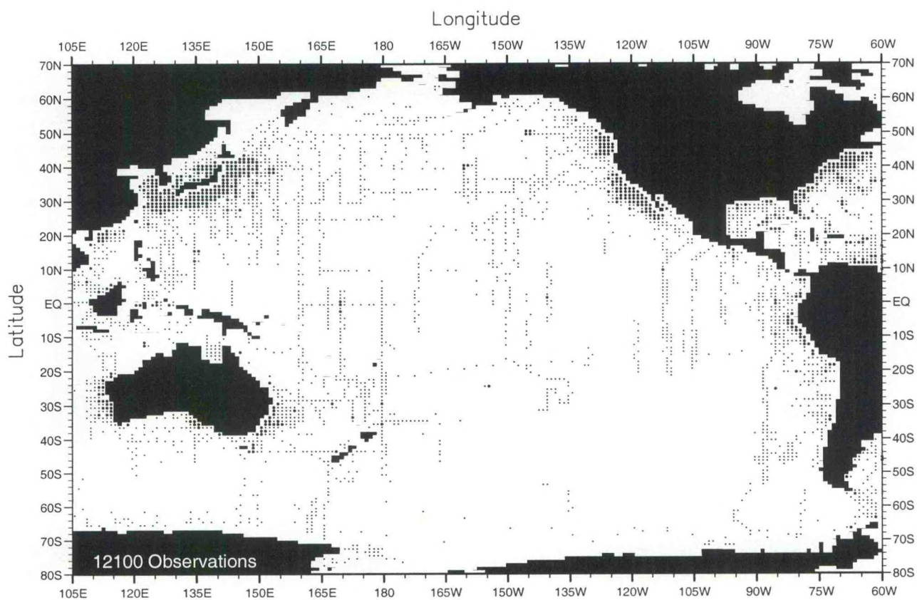
Fig. C5. March oxygen observations at the surface .
