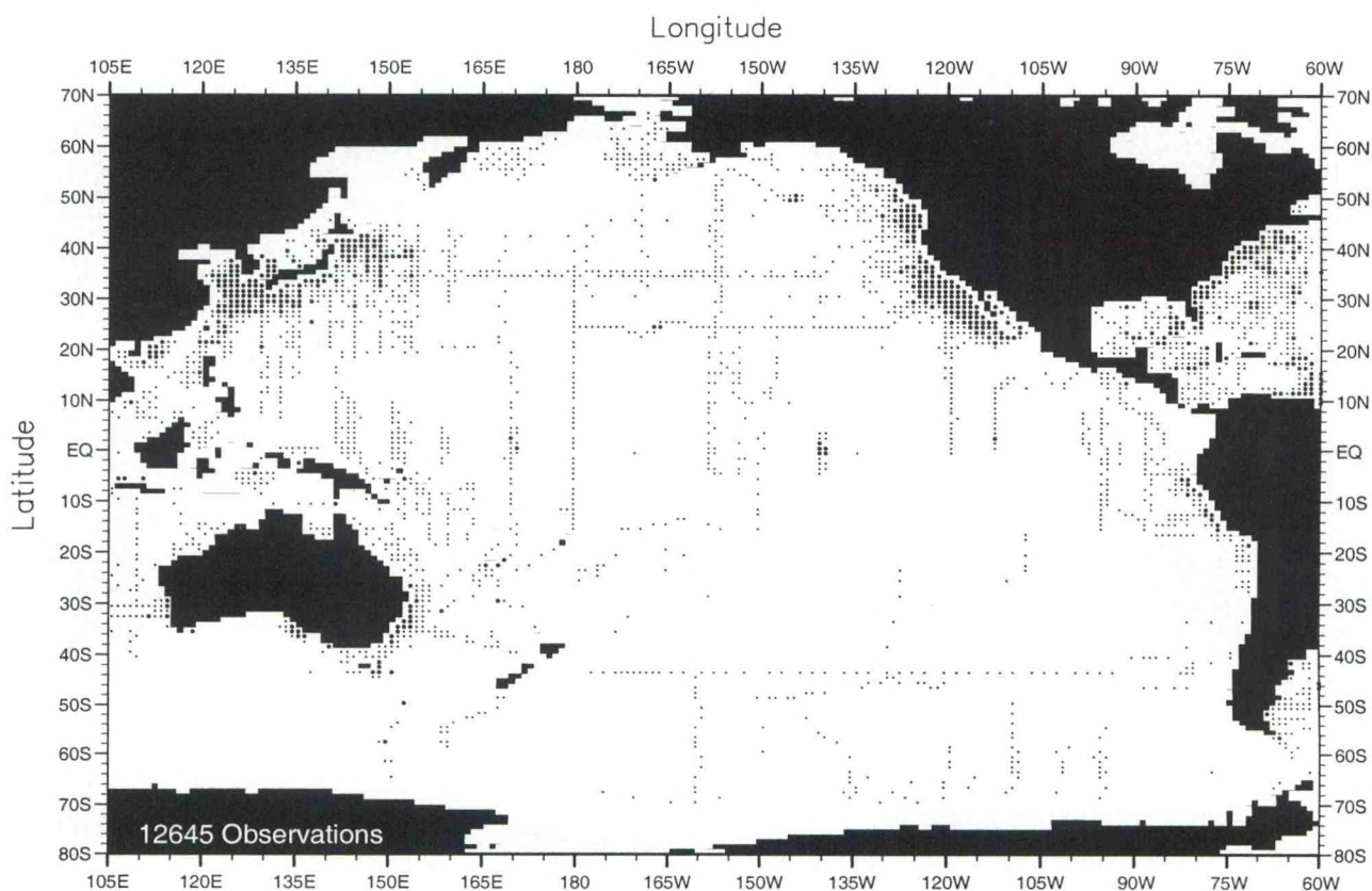
Fig. C7. April oxygen observations at the surface .
