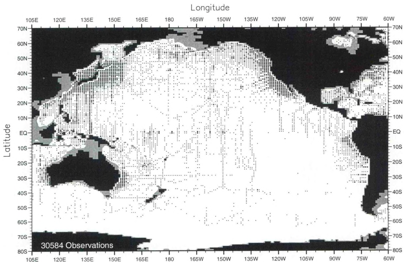
Fig. B11. Summer (Jul.-Sep.) oxygen observations at 150 m. depth .
