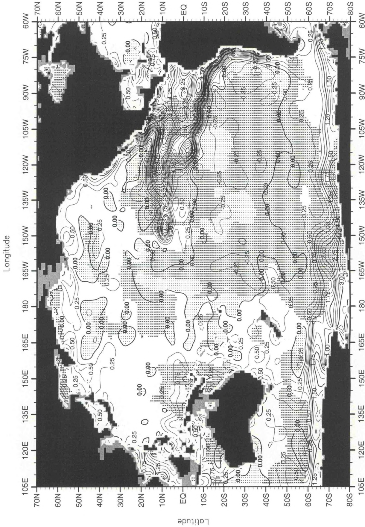
Fig. F6. March mean Apparent Oxygen Utilization (ml/l) at 75 m. depth .
