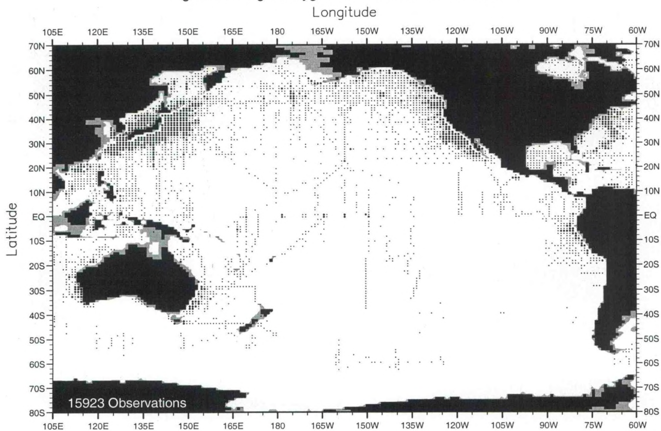
Fig. C16. August oxygen observations at 75 m. depth .
