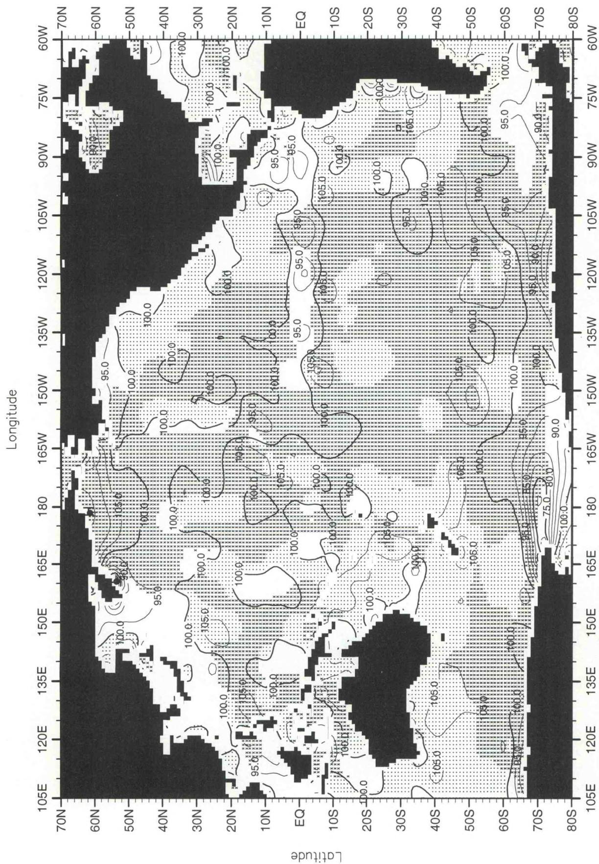
Fig. 123. December mean oxygen saturation (%) at the surface .
