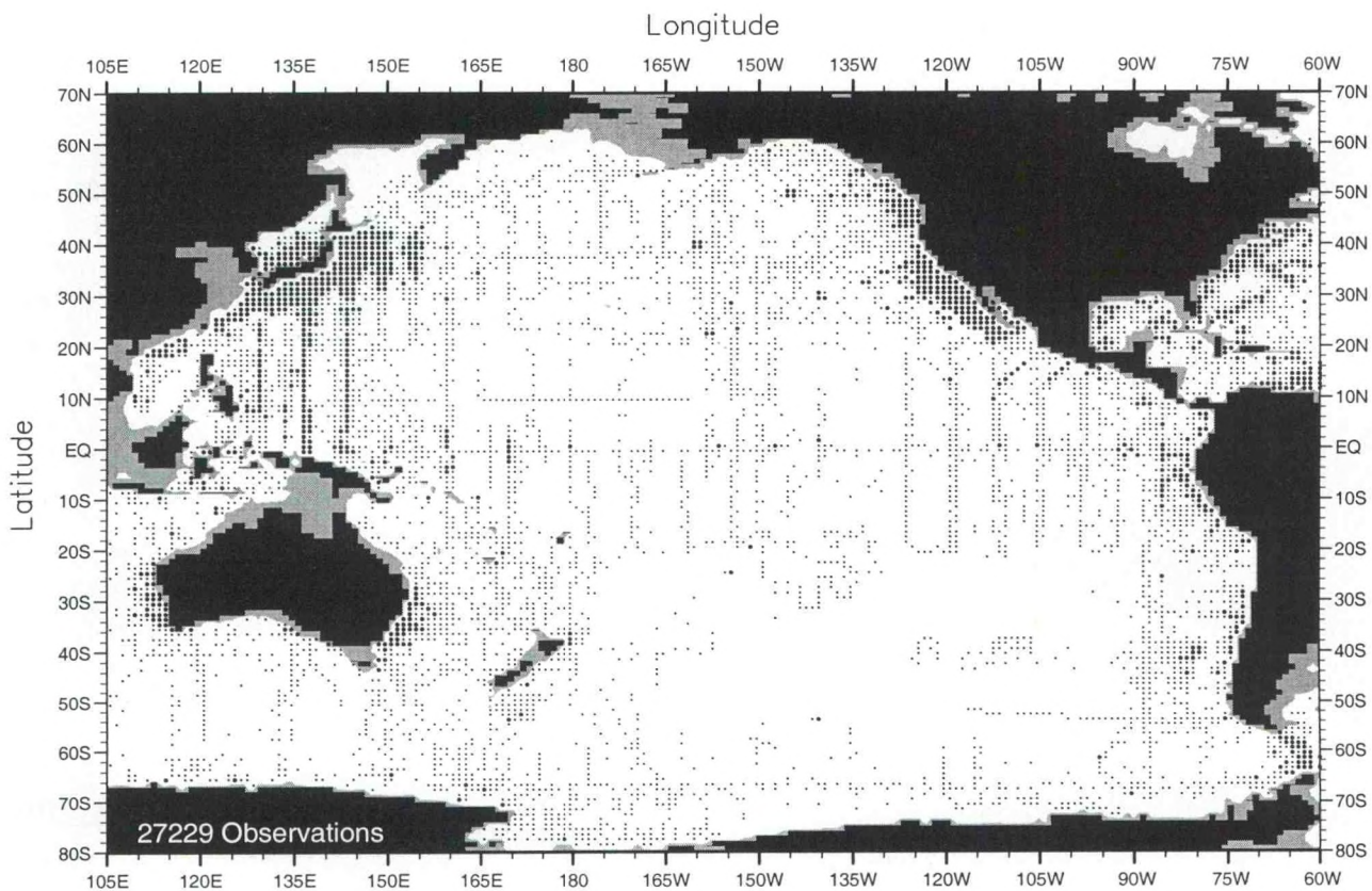
Fig. B3. Winter (Jan.-Mar.) oxygen observations at 150 m. depth .
