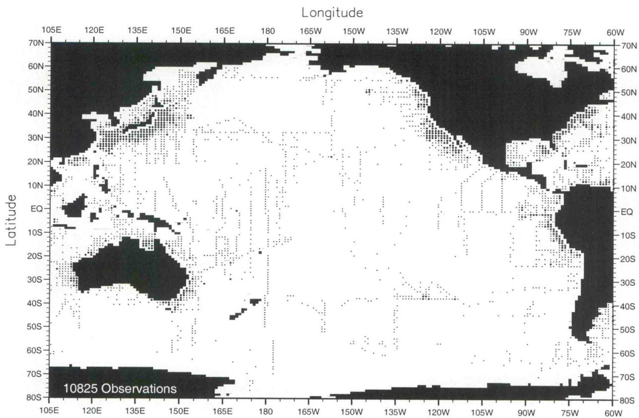
Fig. C21. November oxygen observations at the surface .
