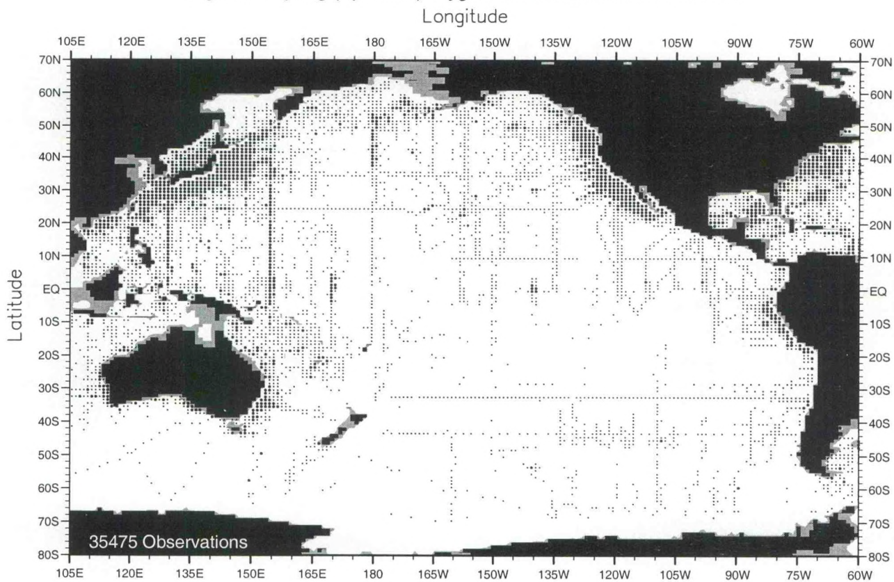
Fig. B6. Spring (Apr.-Jun.) oxygen observations at 75 m. depth .
