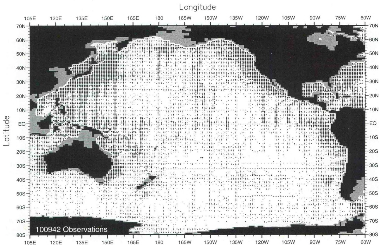
Fig. A7. Annual oxygen observations at 250 m. depth .
