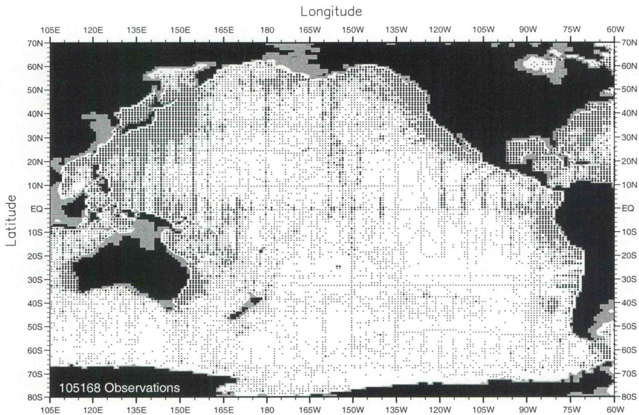
Fig. A5. Annual oxygen observations at 150 m. depth .
