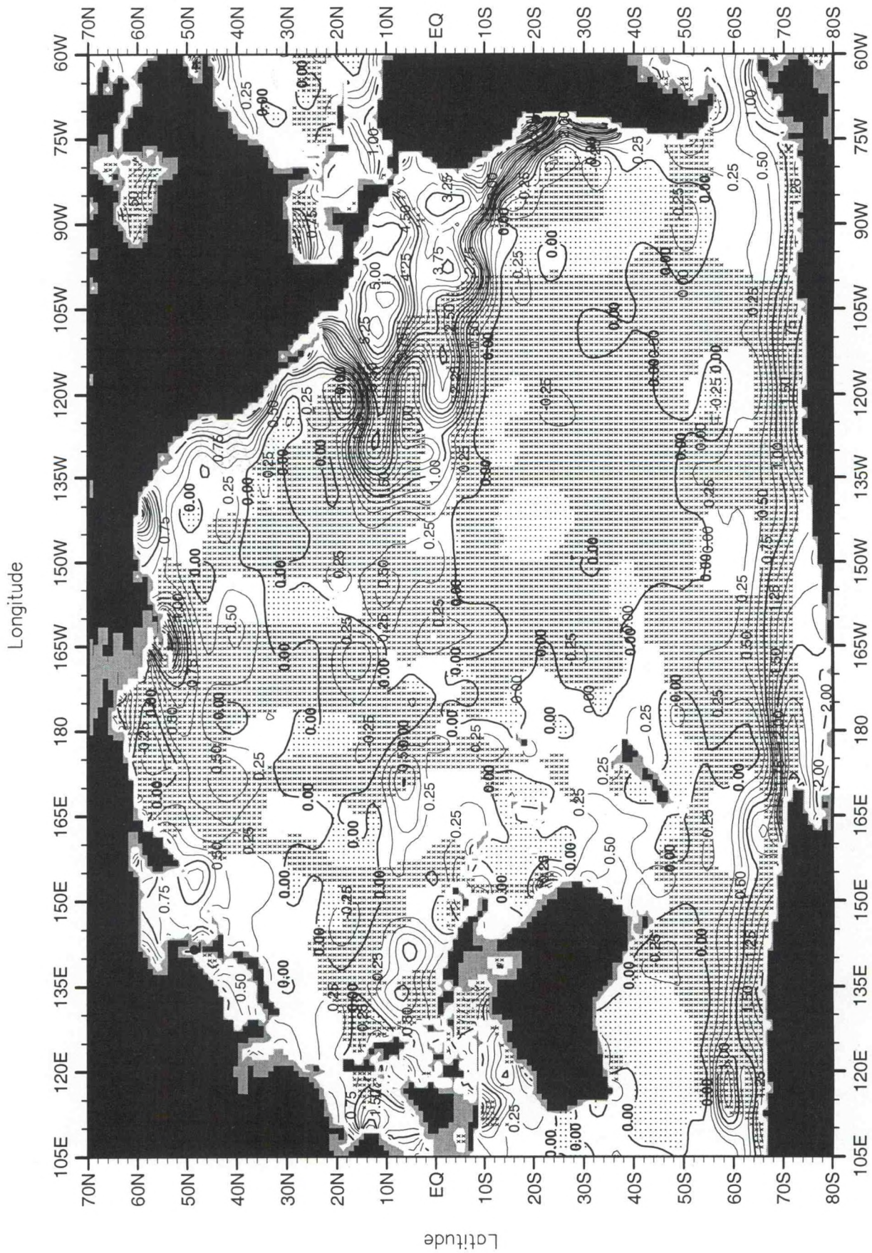
Fig. F24. December mean Apparent Oxygen Utilization (ml/l) at 75 m. depth .
