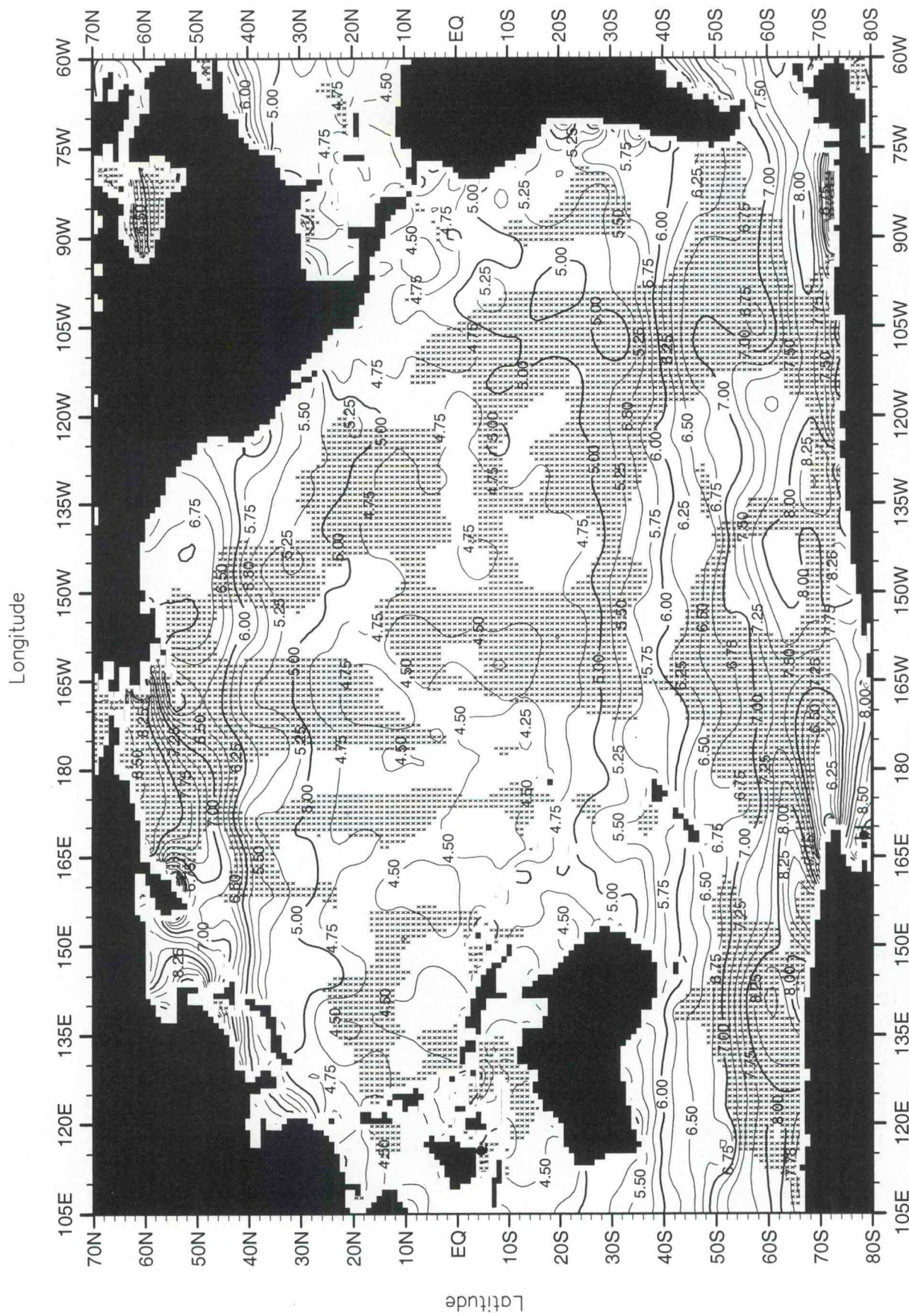
Fig. C47. December mean oxygen (ml/l) at the surface .
