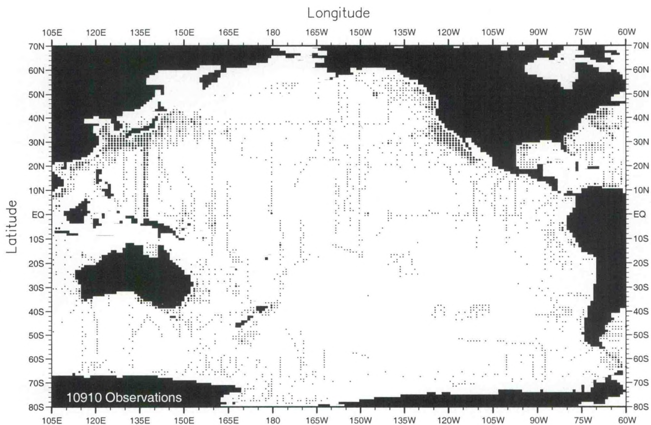
Fig. C1. January oxygen observations at the surface .
