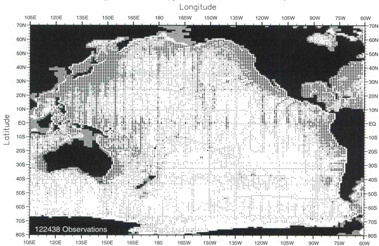
Fig. A4. Annual oxygen observations at 100 m. depth .
