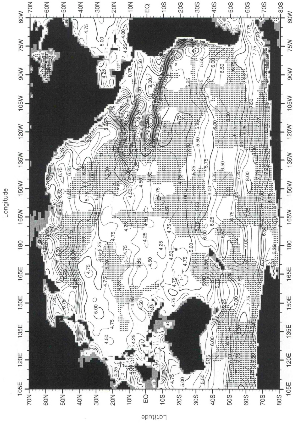
Fig. C46. November mean oxygen (ml/l) at 75 m. depth .
