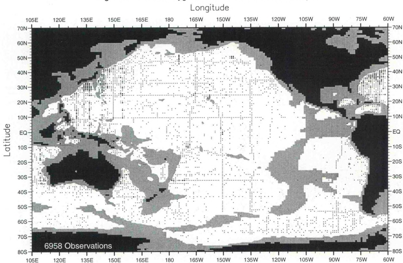
Fig. A16. Annual oxygen observations at 4000 m. depth .
