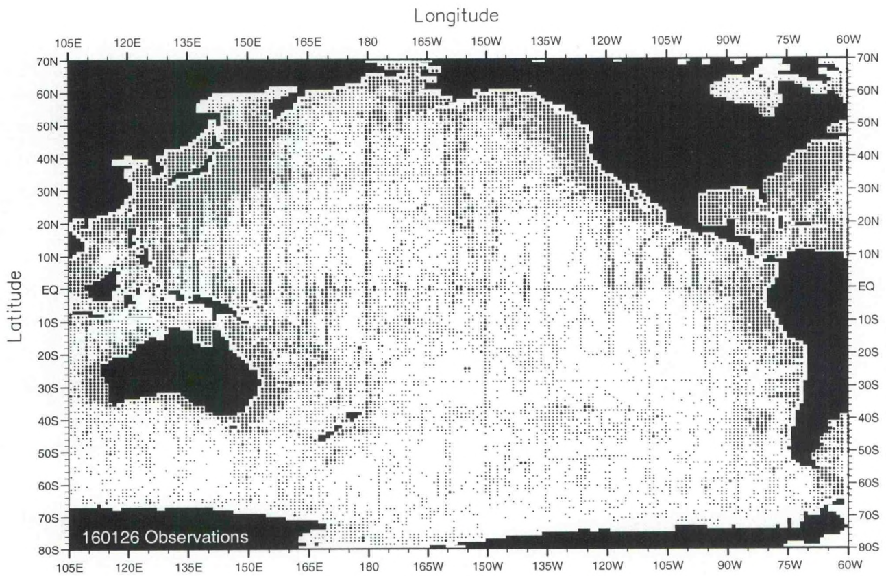
Fig. A1. Annual oxygen observations at the surface .
