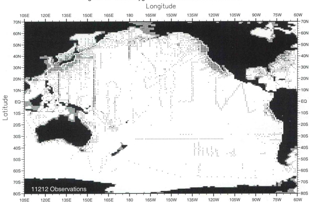
Fig. C12. June oxygen observations at 75 m. depth .
