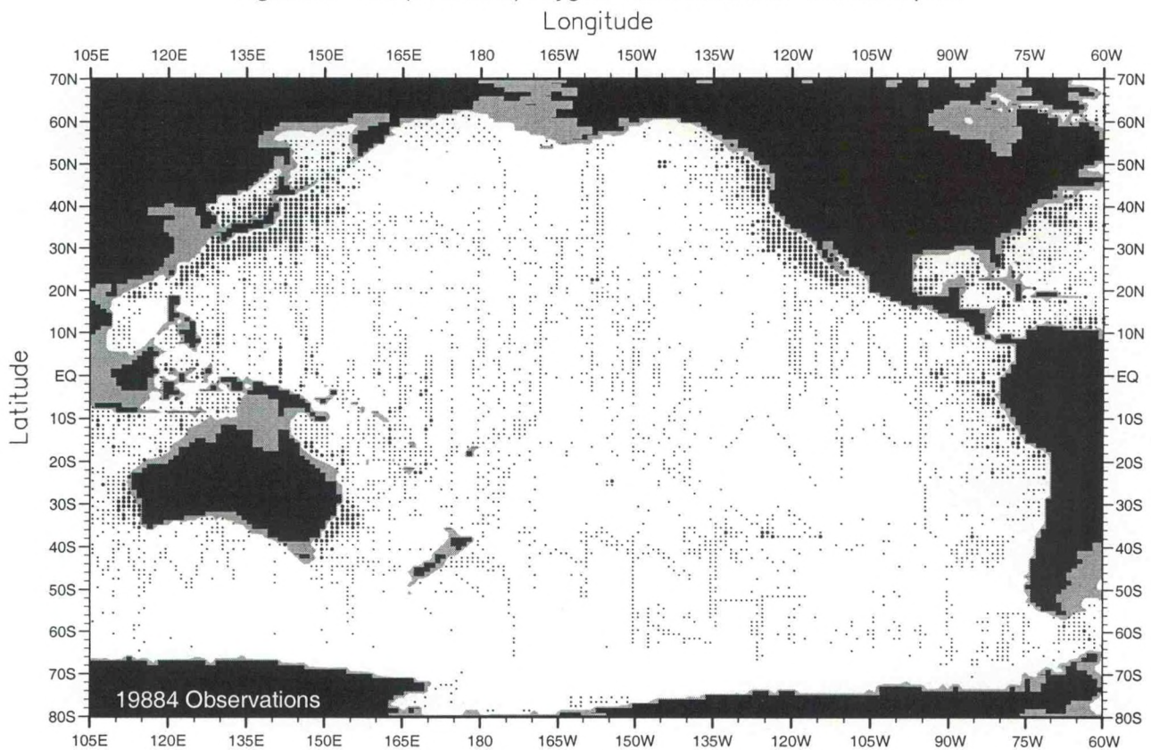
Fig. B16. Fall (Oct.-Dec.) oxygen observations at 250 m. depth .
