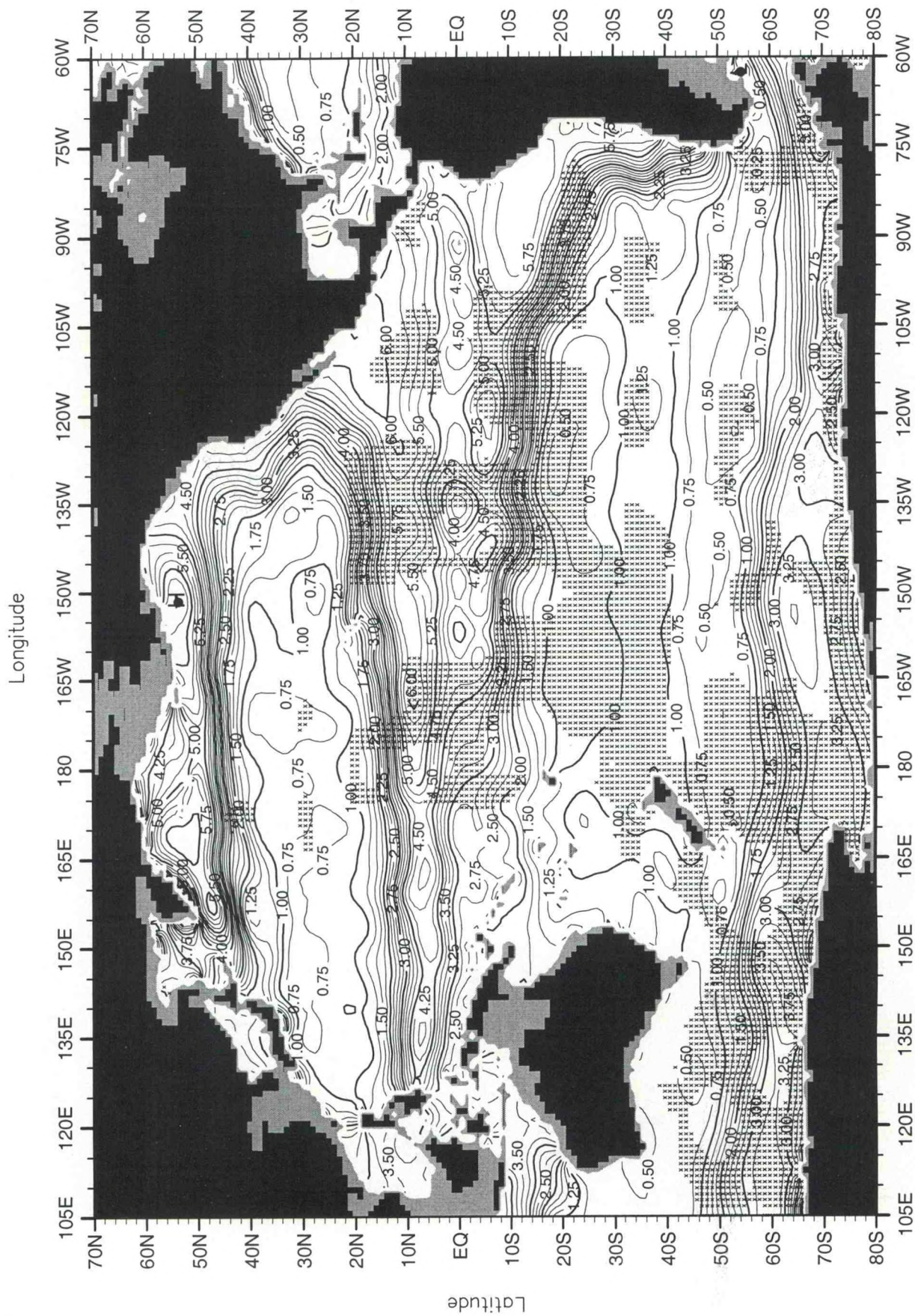
Fig. E8. Spring (Apr.-Jun.) mean Apparent Oxygen Utilization (m/l) at 250 m. depth .
