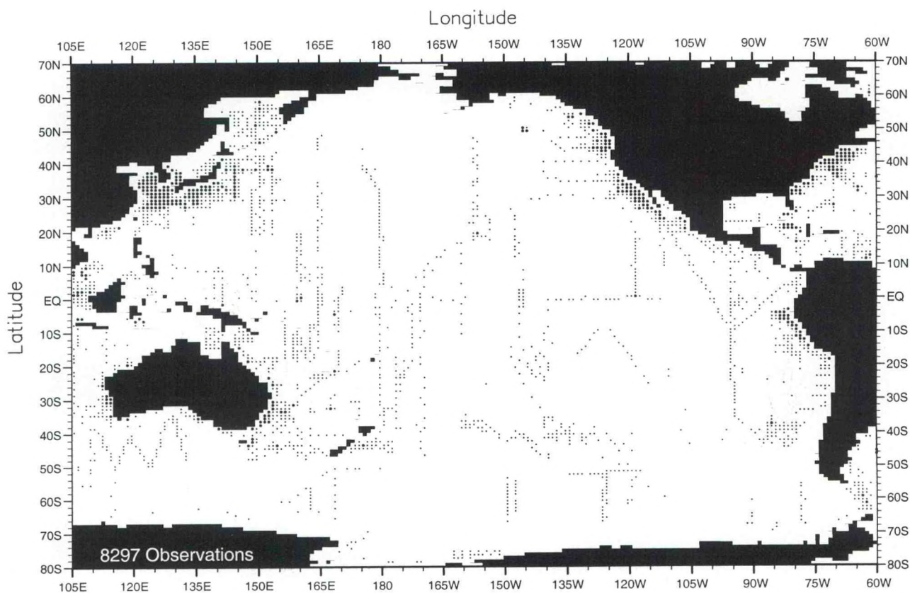
Fig. C23. December oxygen observations at the surface .
