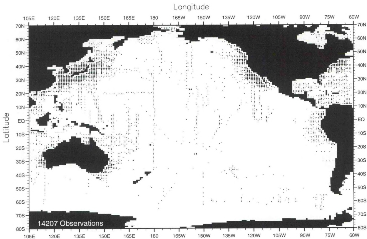
Fig. C19. October oxygen observations at the surface .
