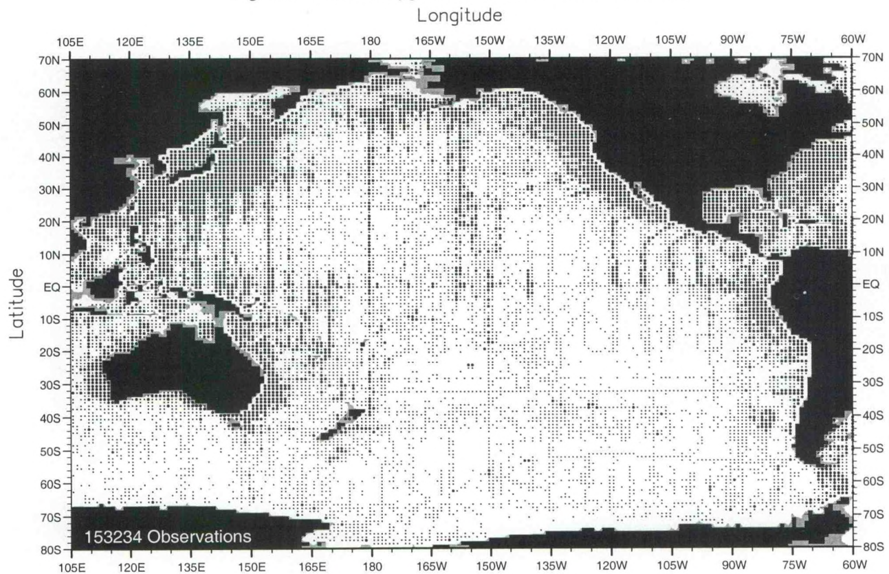
Fig. A2. Annual oxygen observations at 50 m. depth .
