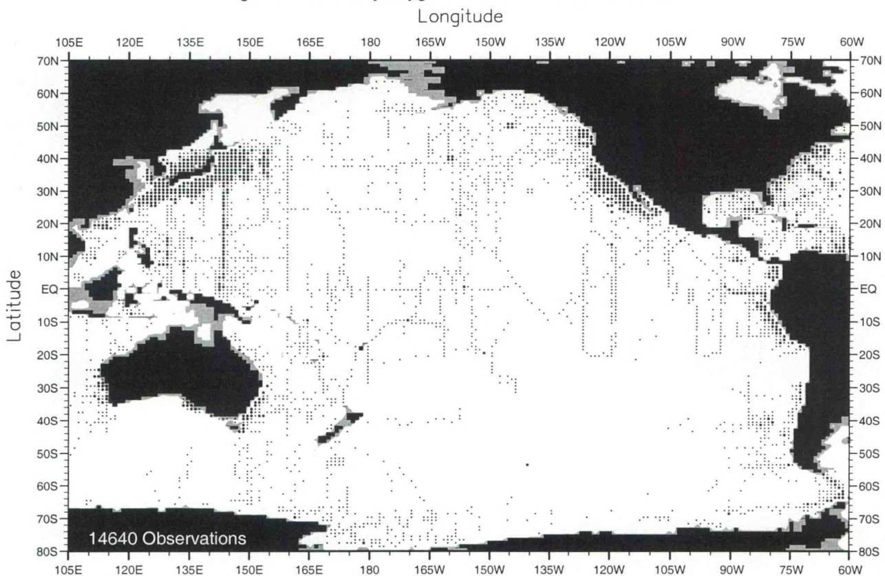
Fig. C4. February oxygen observations at 75 m. depth .
