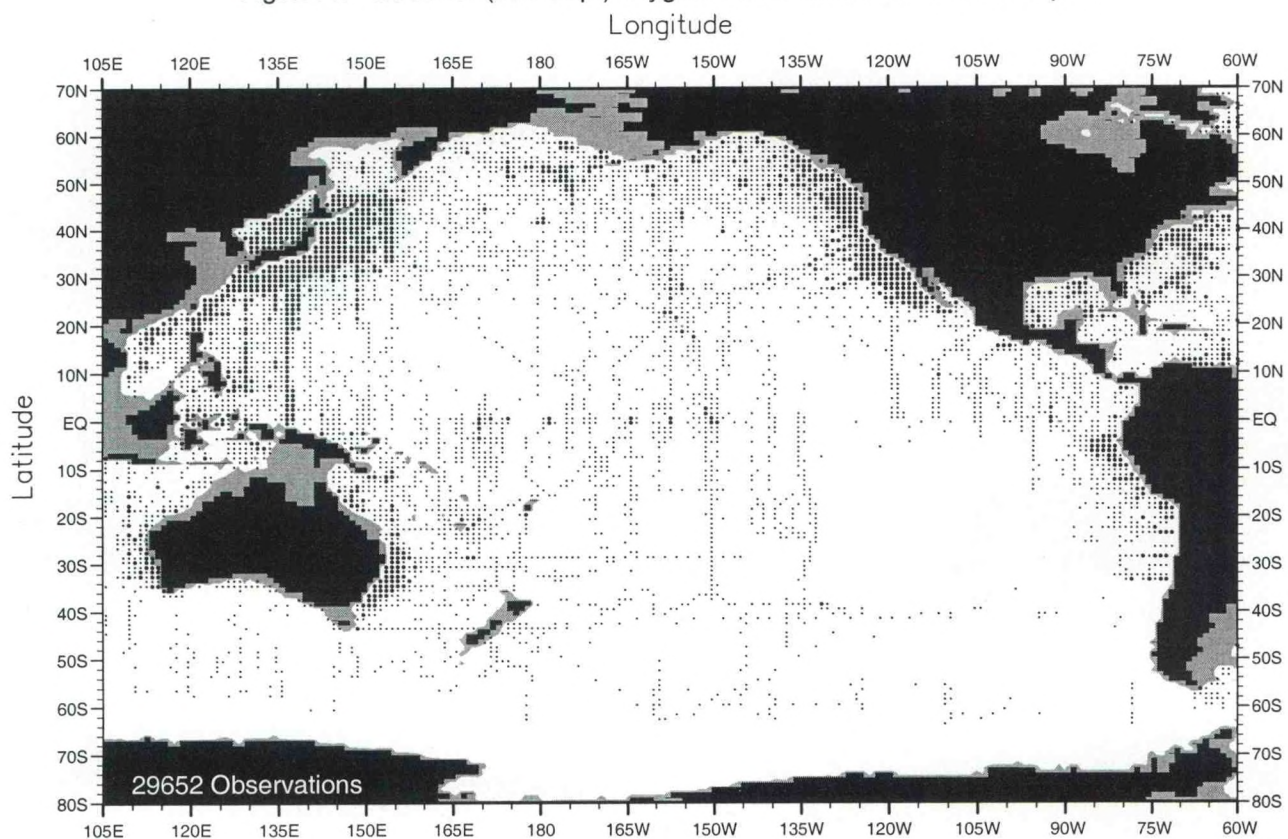
Fig. B12. Summer (Jul.-Sep.) oxygen observations at 250 m. depth .
