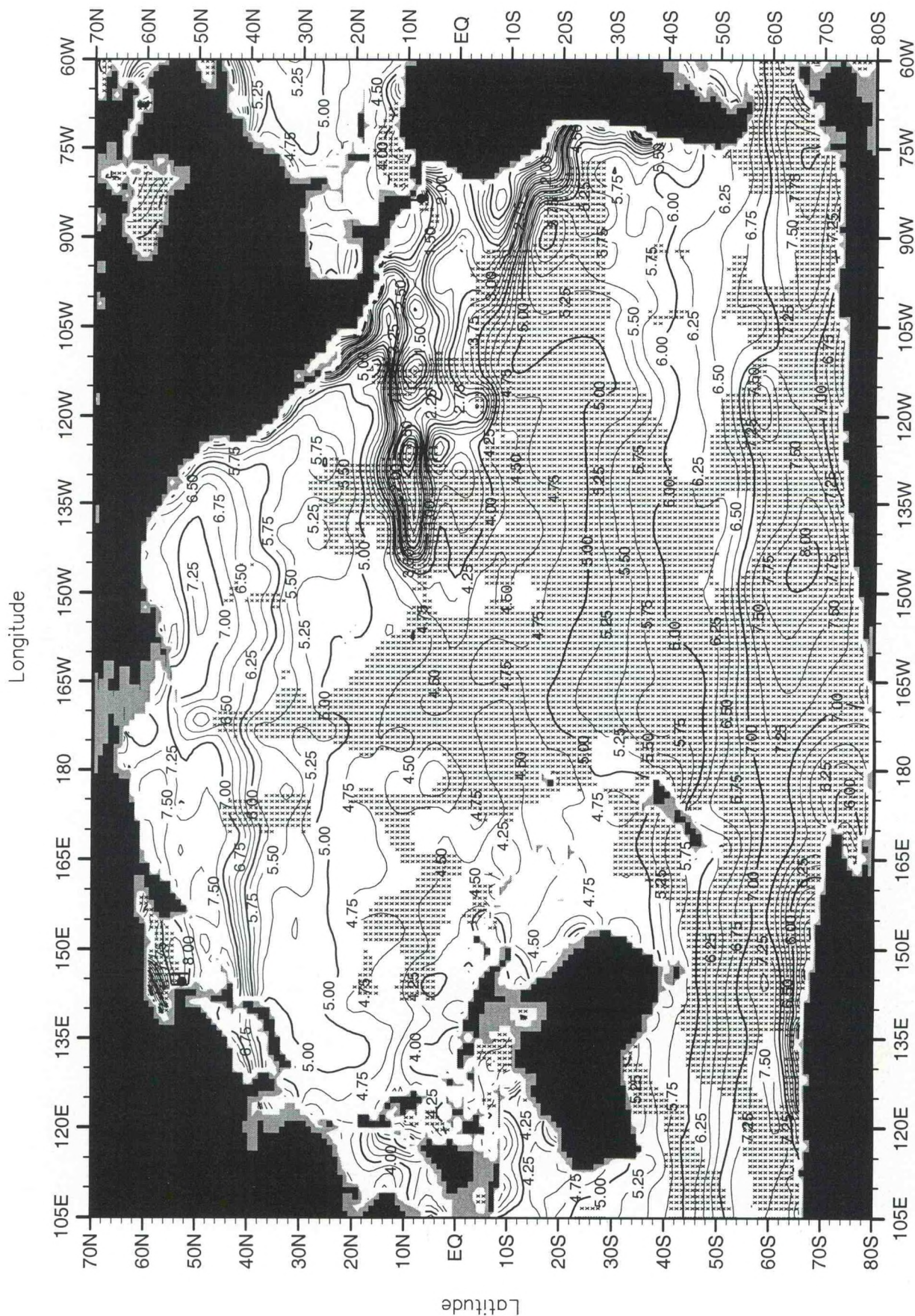
Fig. C34. May mean oxygen (ml/l) at 75 m. depth .
