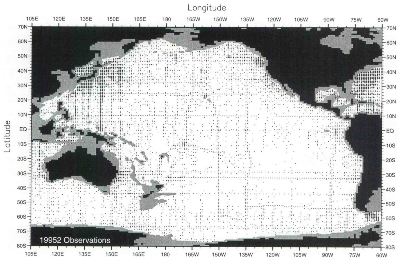
Fig. A13. Annual oxygen observations at 2000 m. depth .
