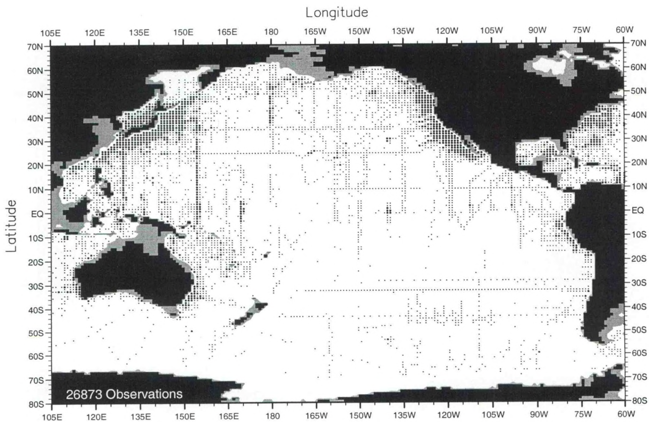
Fig. B7. Spring (Apr.-Jun.) oxygen observations at 150 m. depth .
