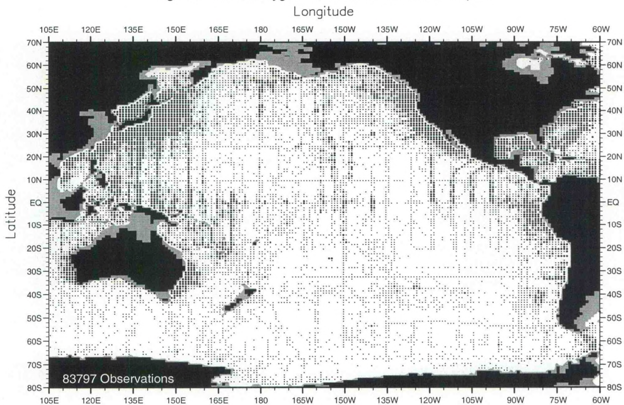
Fig. A6. Annual oxygen observations at 200 m. depth .
