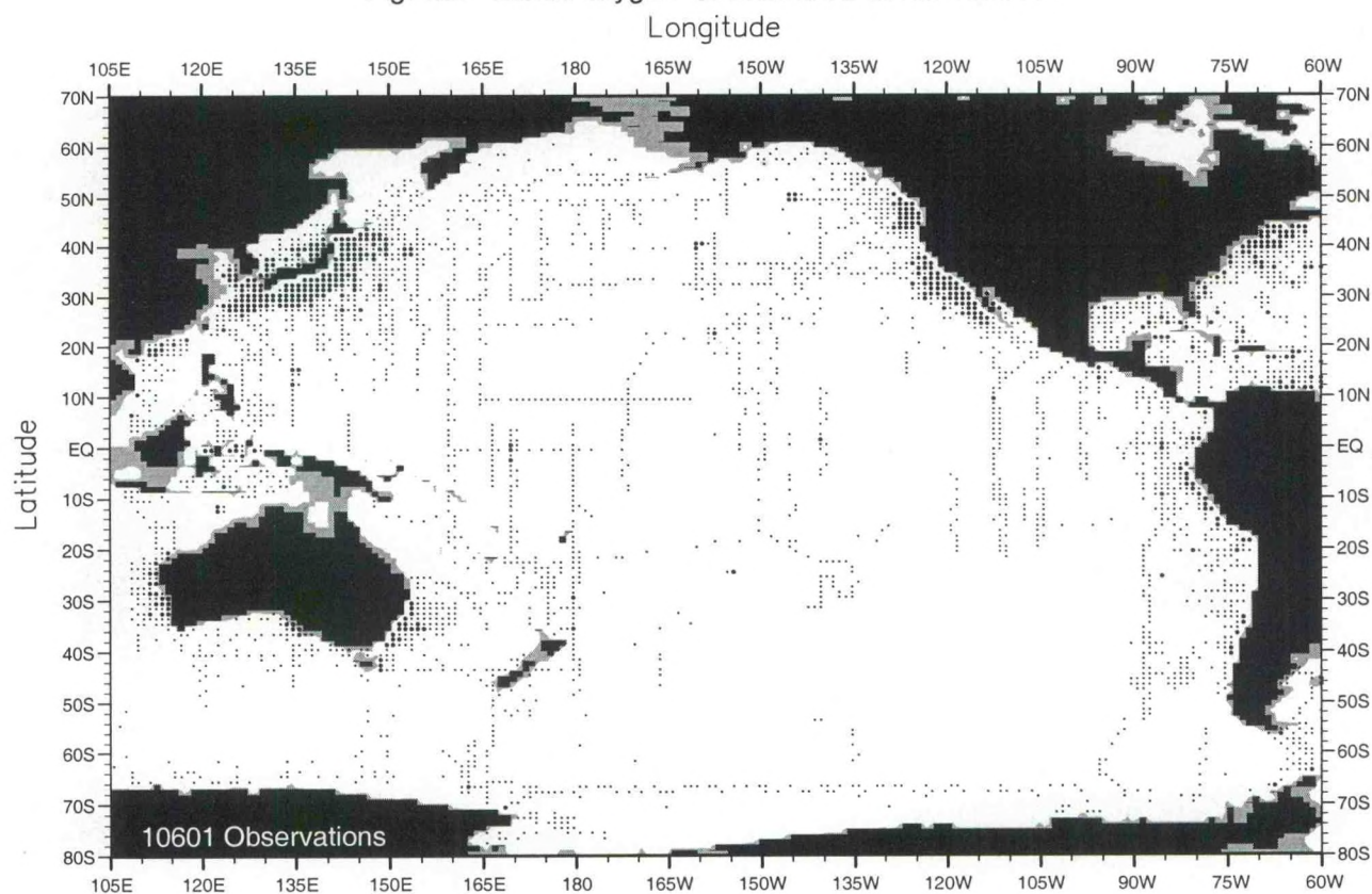
Fig. C6. March oxygen observations at 75 m. depth .
