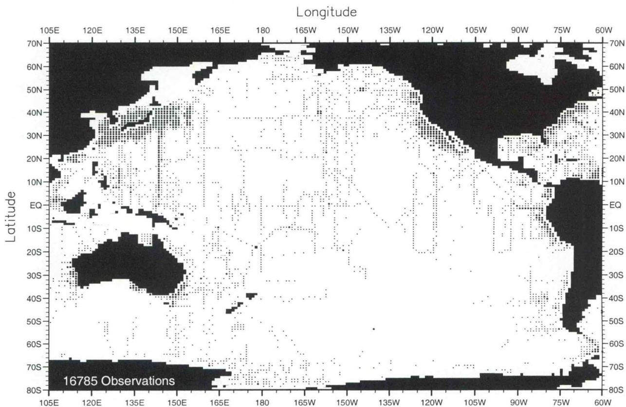
Fig. C3. February oxygen observations at the surface .
