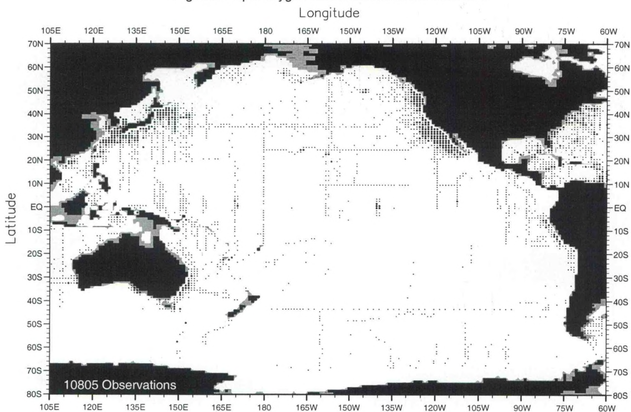
Fig. C8. April oxygen observations at 75 m. depth .
