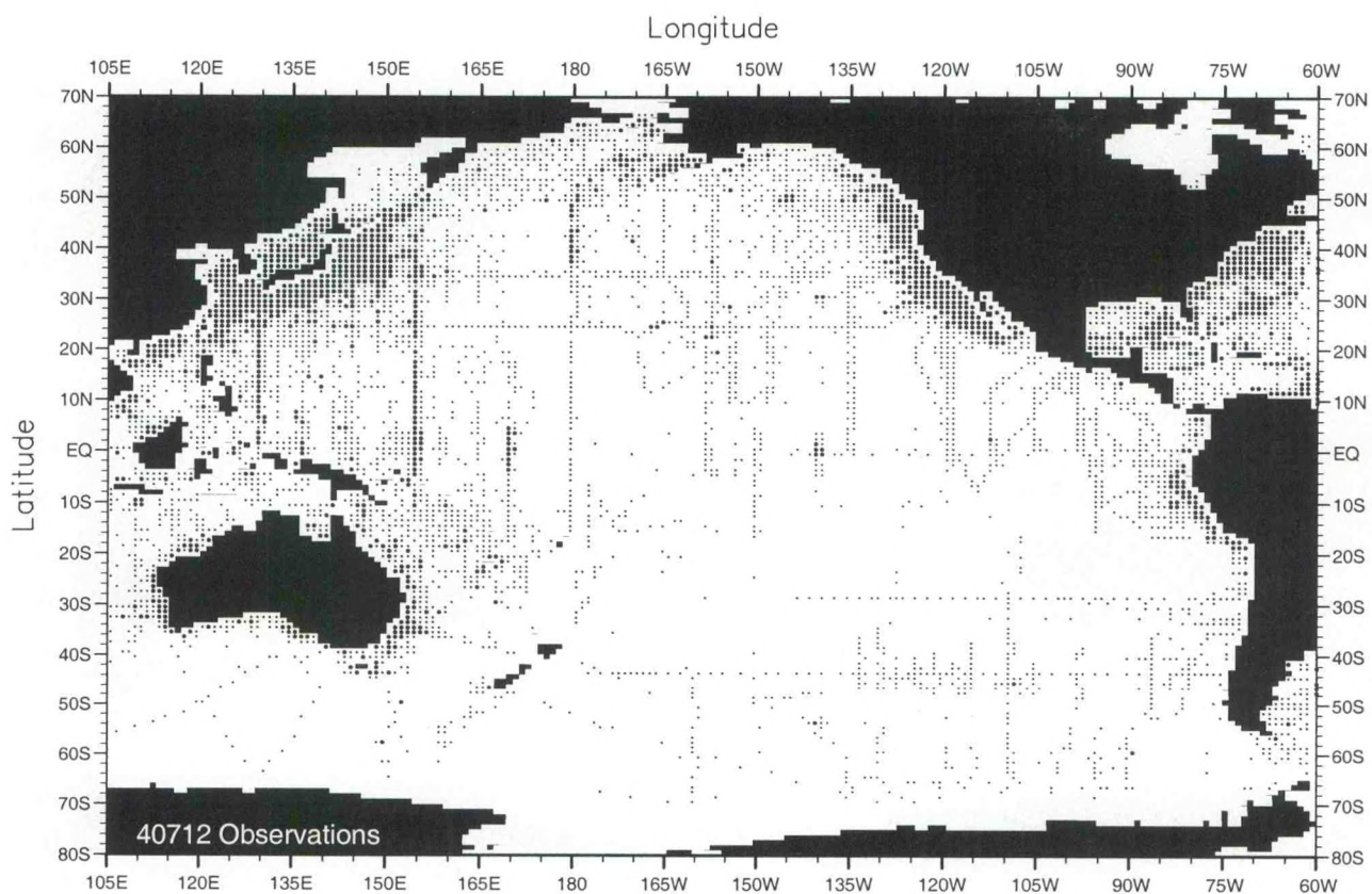
Fig. B5. Spring (Apr.-Jun.) oxygen observations at the surface .
