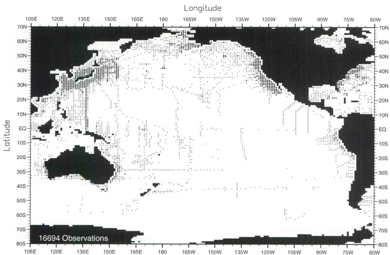
Fig. C13. July oxygen observations at the surface .
