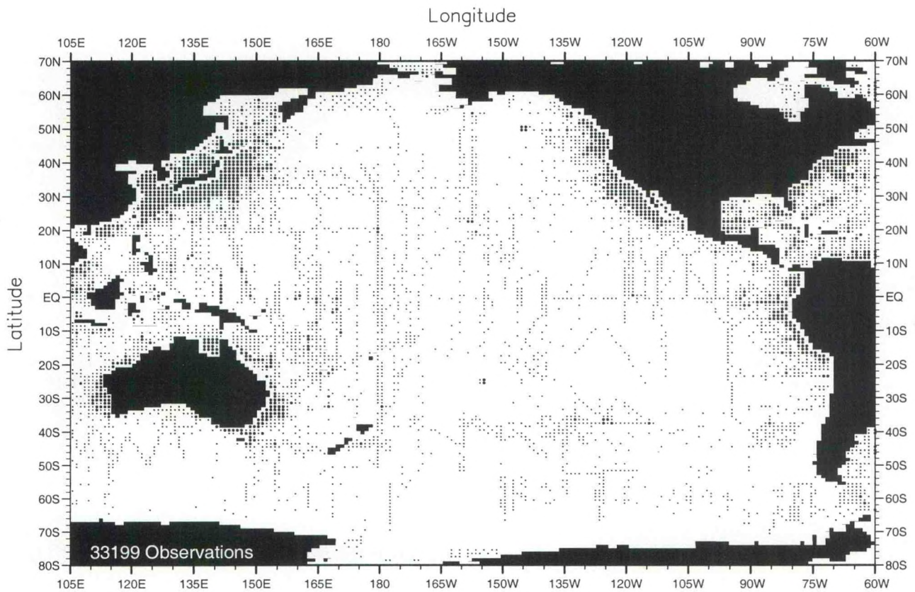
Fig. B13. Fall (Oct.-Dec.) oxygen observations at the surface .
