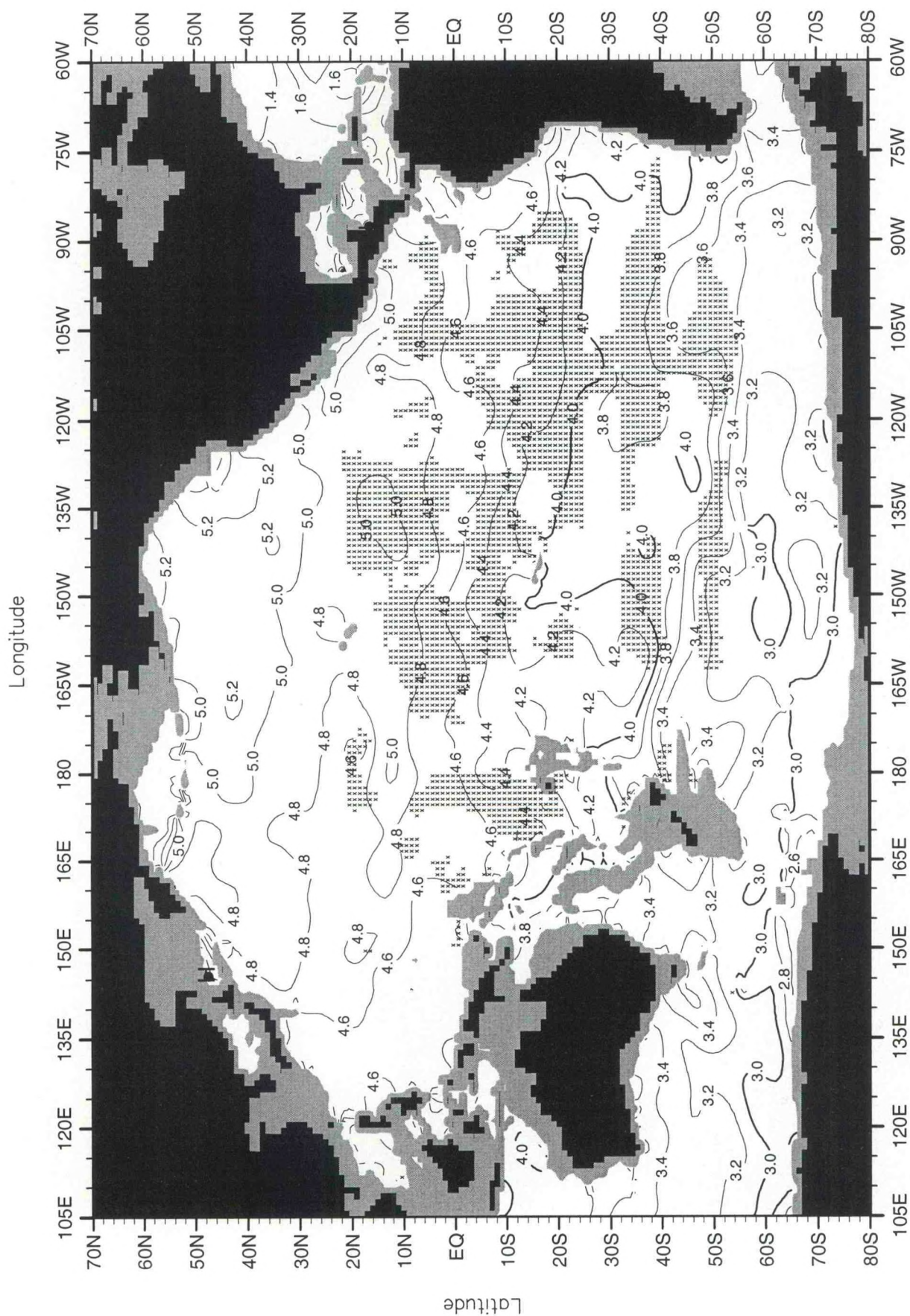
Fig. D15. Annual mean Apparent Oxygen Utilization (ml/l) at 3000 m. depth .
