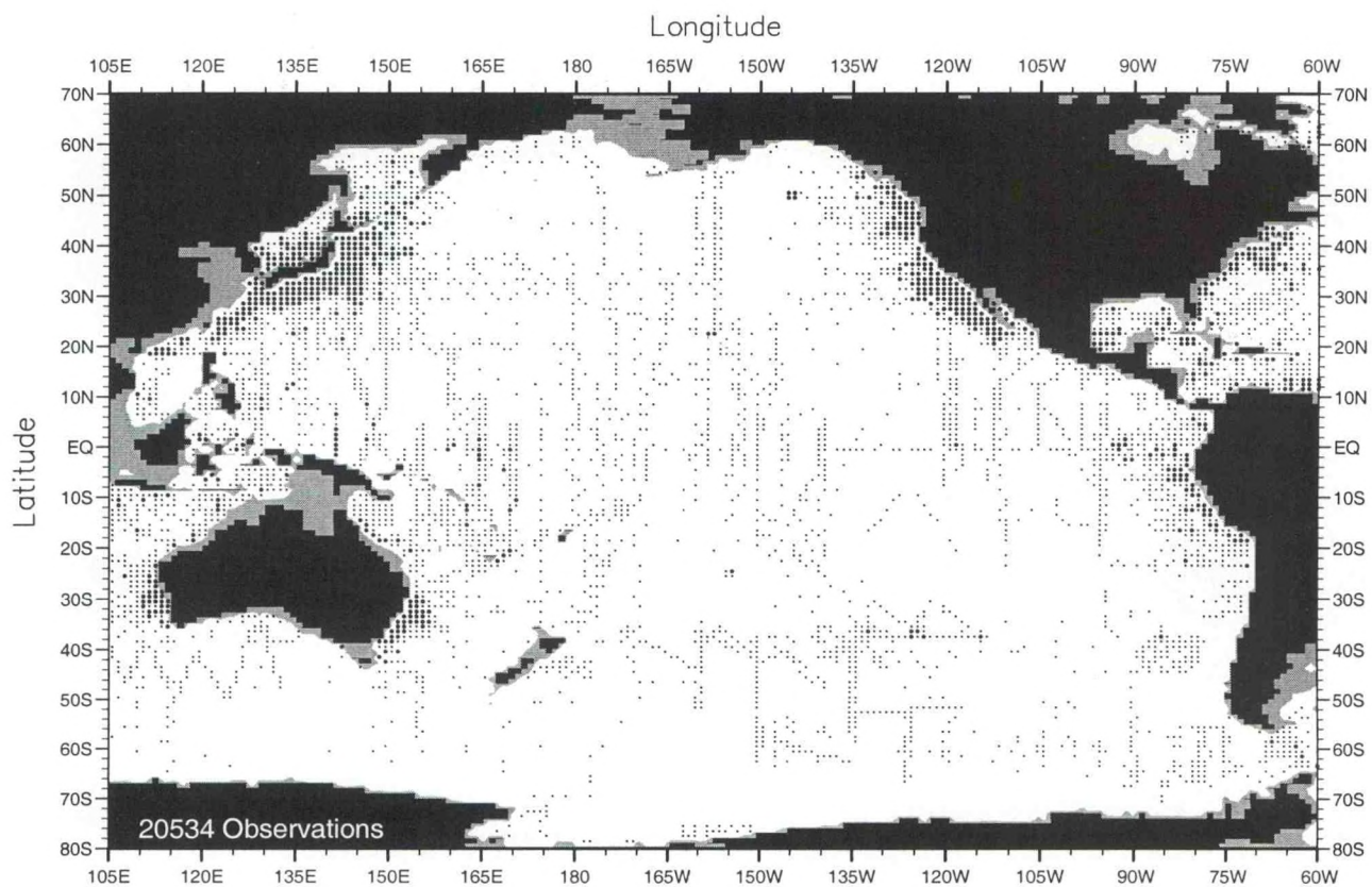
Fig. B15. Fall (Oct.-Dec.) oxygen observations at 150 m. depth .
