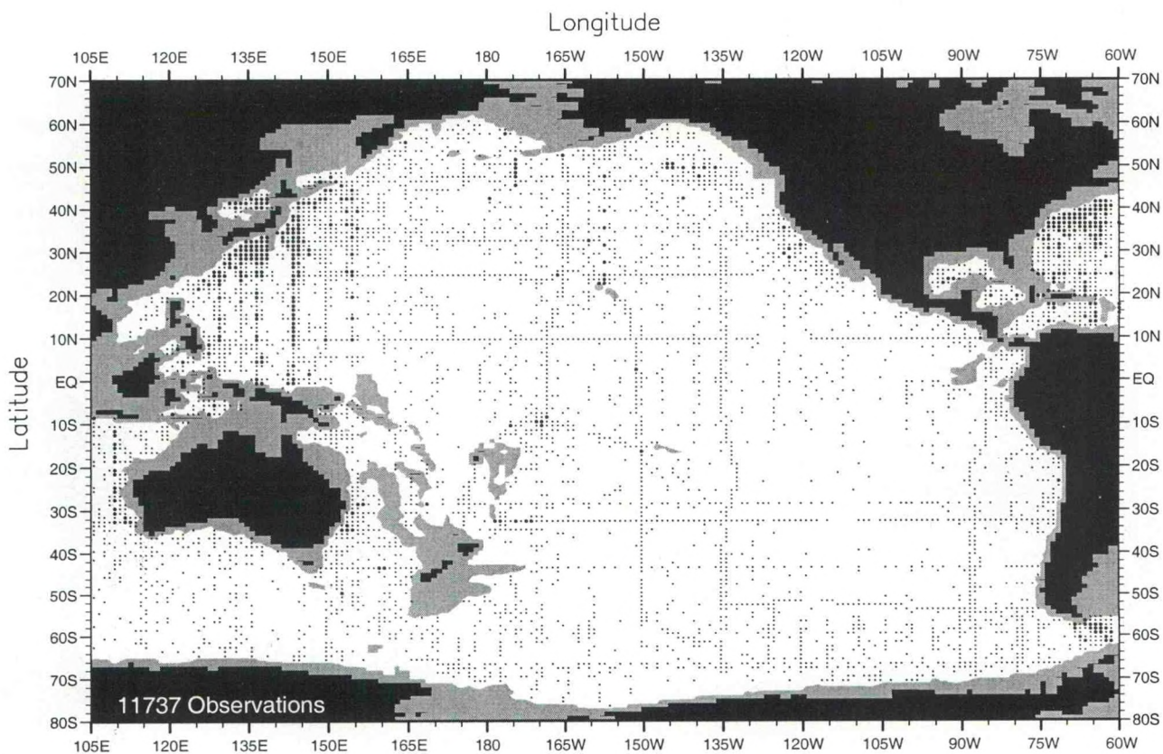
Fig. A15. Annual oxygen observations at 3000 m. depth .
