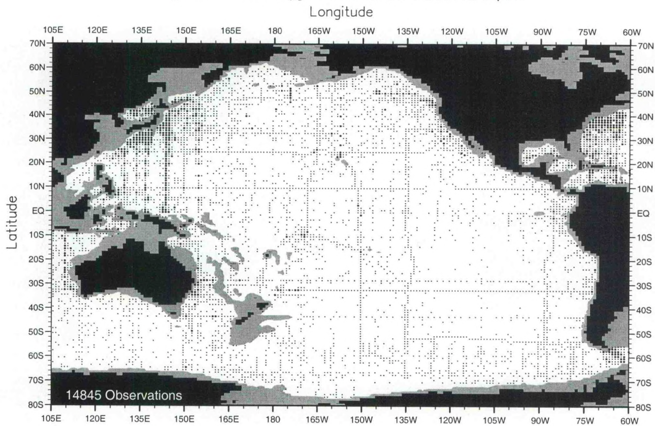
Fig. A14. Annual oxygen observations at 2500 m. depth .
