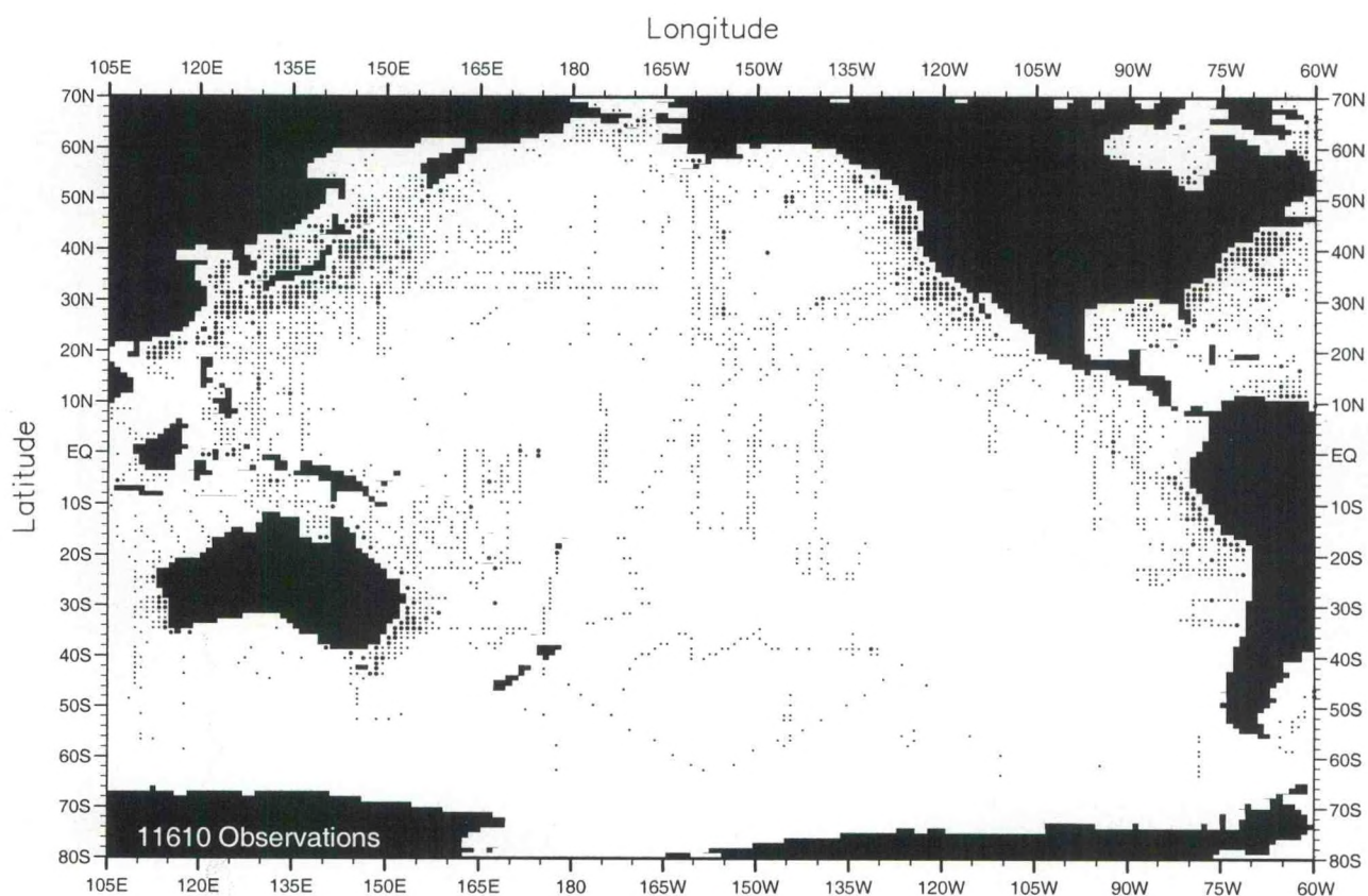
Fig. C17. September oxygen observations at the surface .
