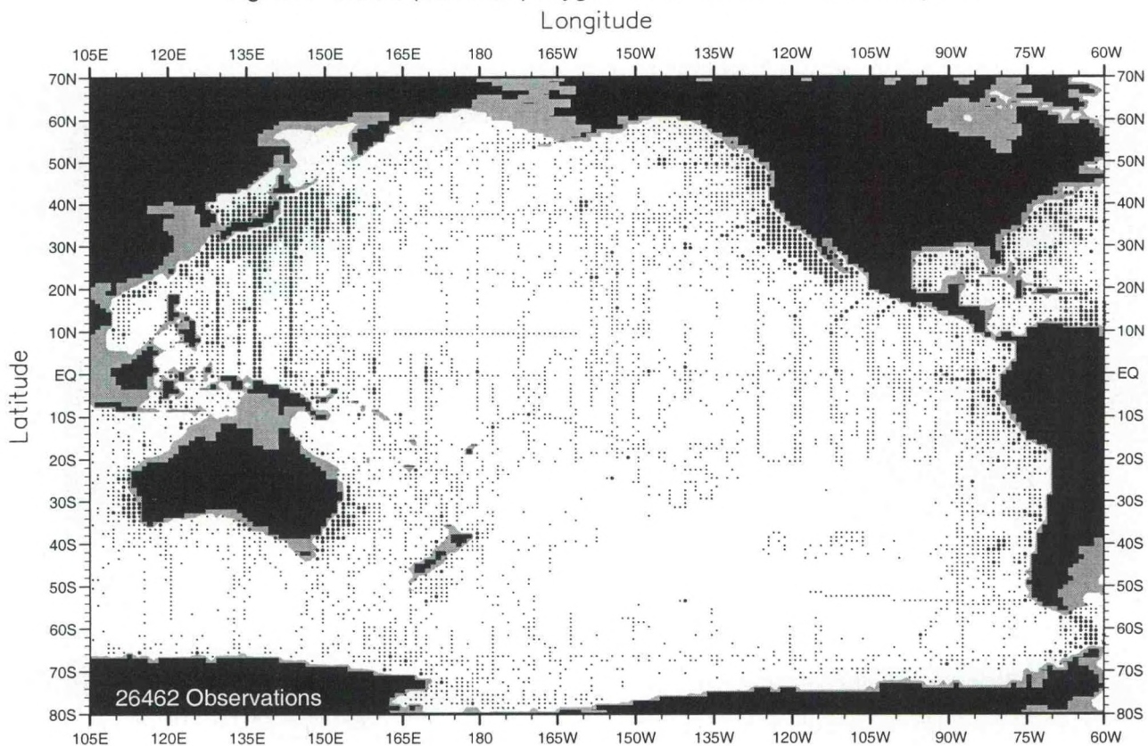
Fig. B4. Winter (Jan.-Mar.) oxygen observations at 250 m. depth .
