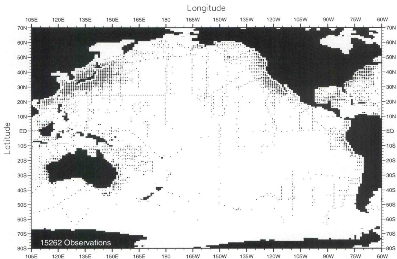
Fig. C9. May oxygen observations at the surface .
