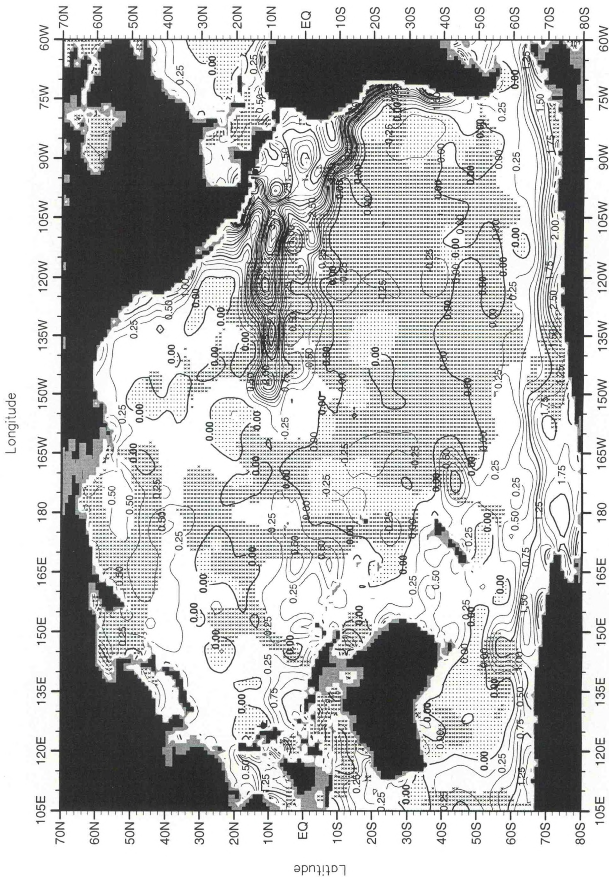
Fig. F2. January mean Apparent Oxygen Utilization (ml/l) at 75 m. depth .
