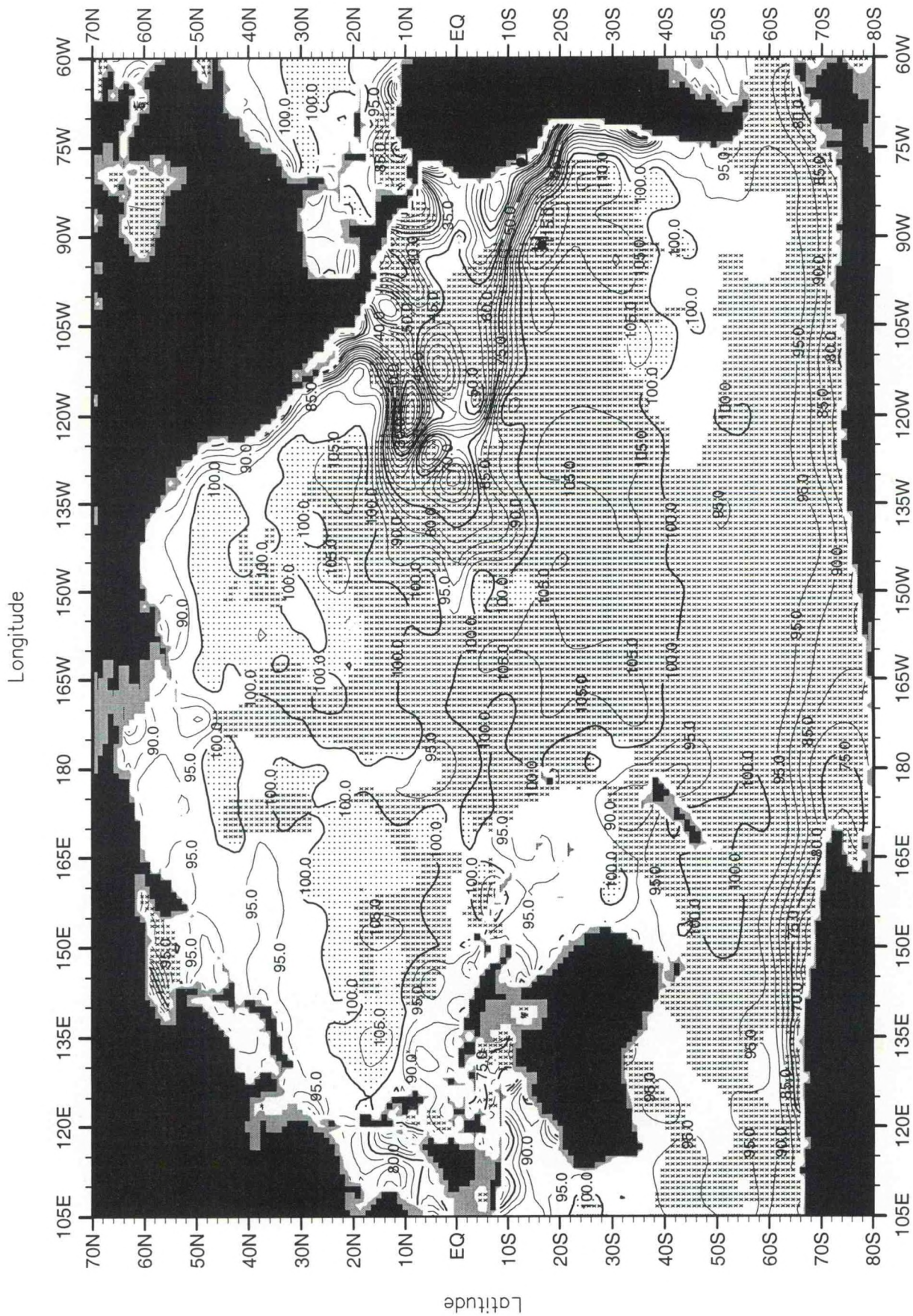
Fig. 110. May mean oxygen saturation (%) at 75 m. depth .
