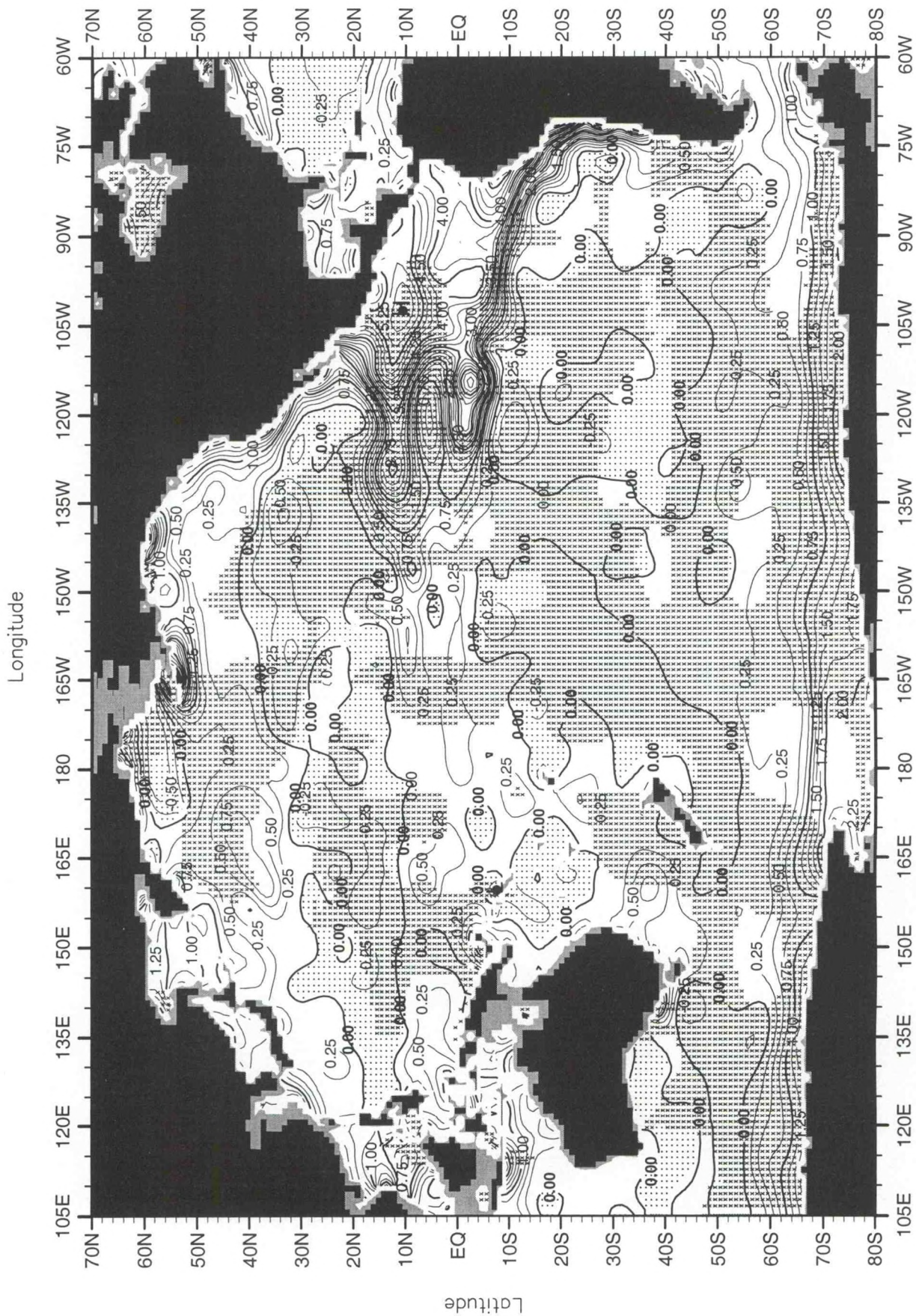
Fig. F22. November mean Apparent Oxygen Utilization (ml/l) at 75 m. depth .
