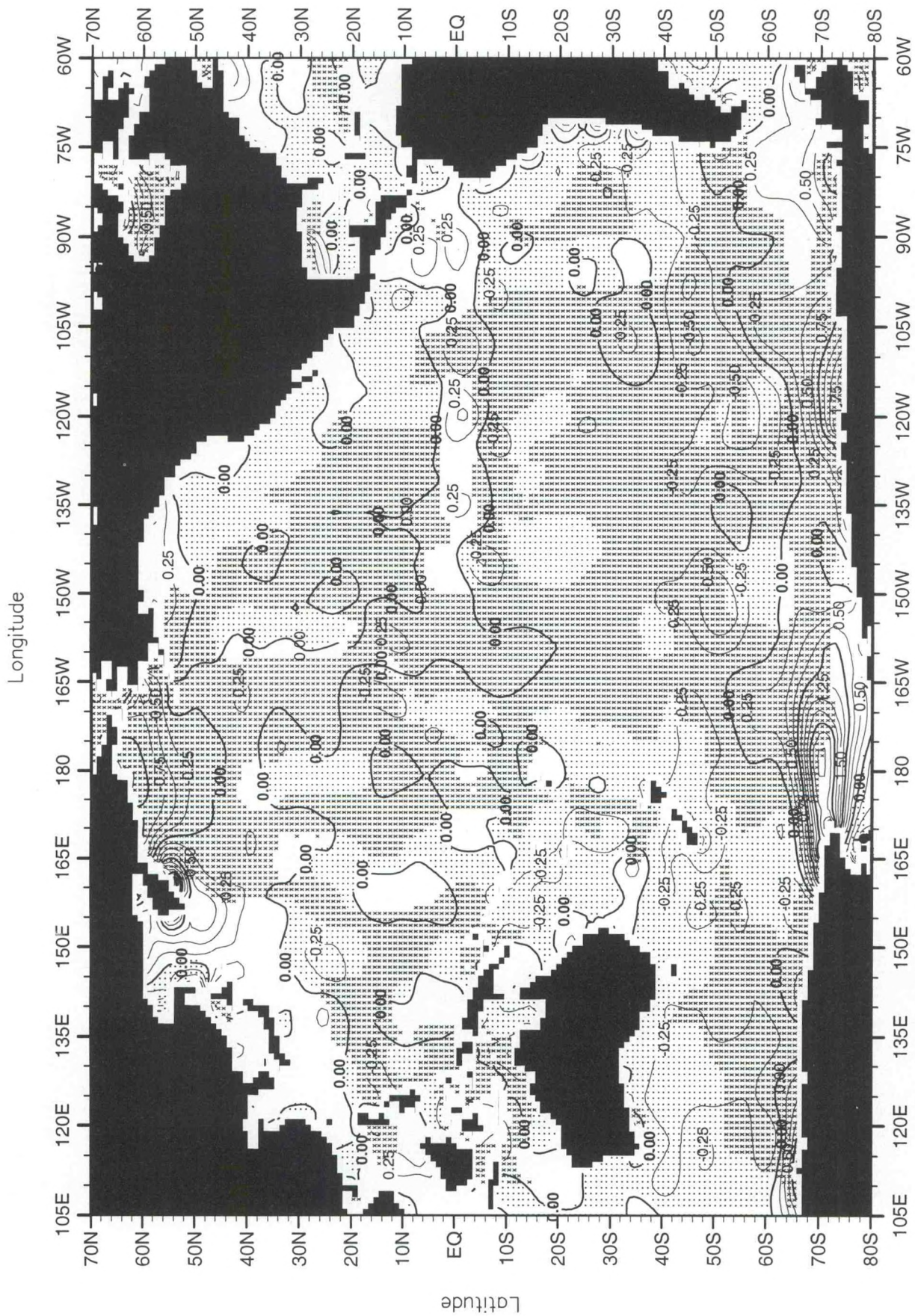
Fig. F23. December mean Apparent Oxygen Utilization (ml/l) at the surface .
