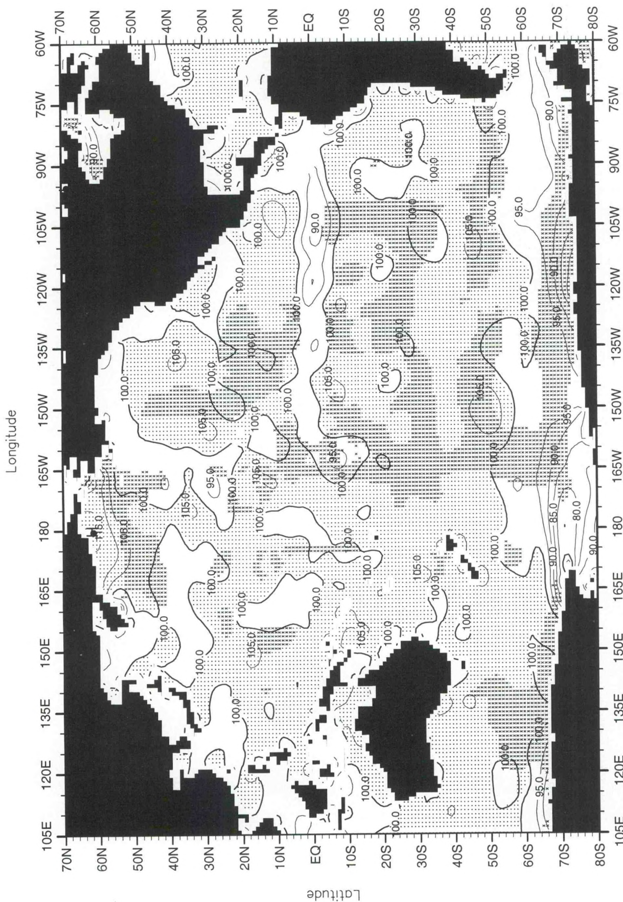
Fig. H13. Fall (Oct.-Dec.) mean oxygen saturation (%) at the surface .
