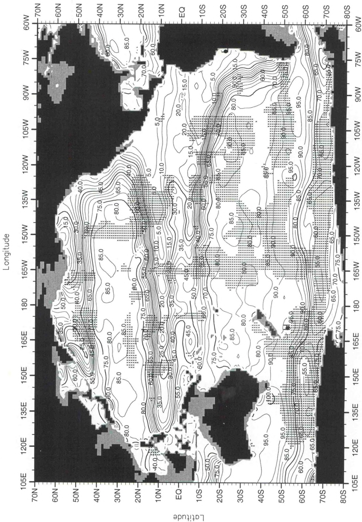
Fig. H16. Fall (Oct.-Dec.) mean oxygen saturation (%) at 250 m. depth .
