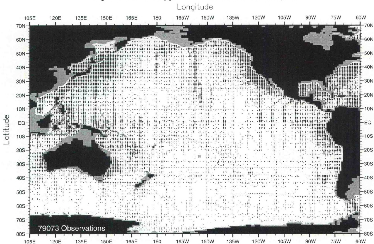
Fig. A8. Annual oxygen observations at 400 m. depth .
