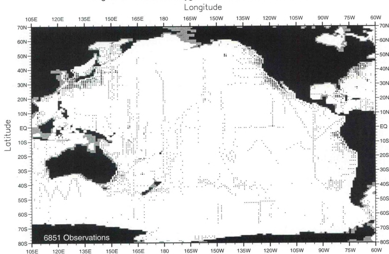
Fig. C24. December oxygen observations at 75 m. depth .
