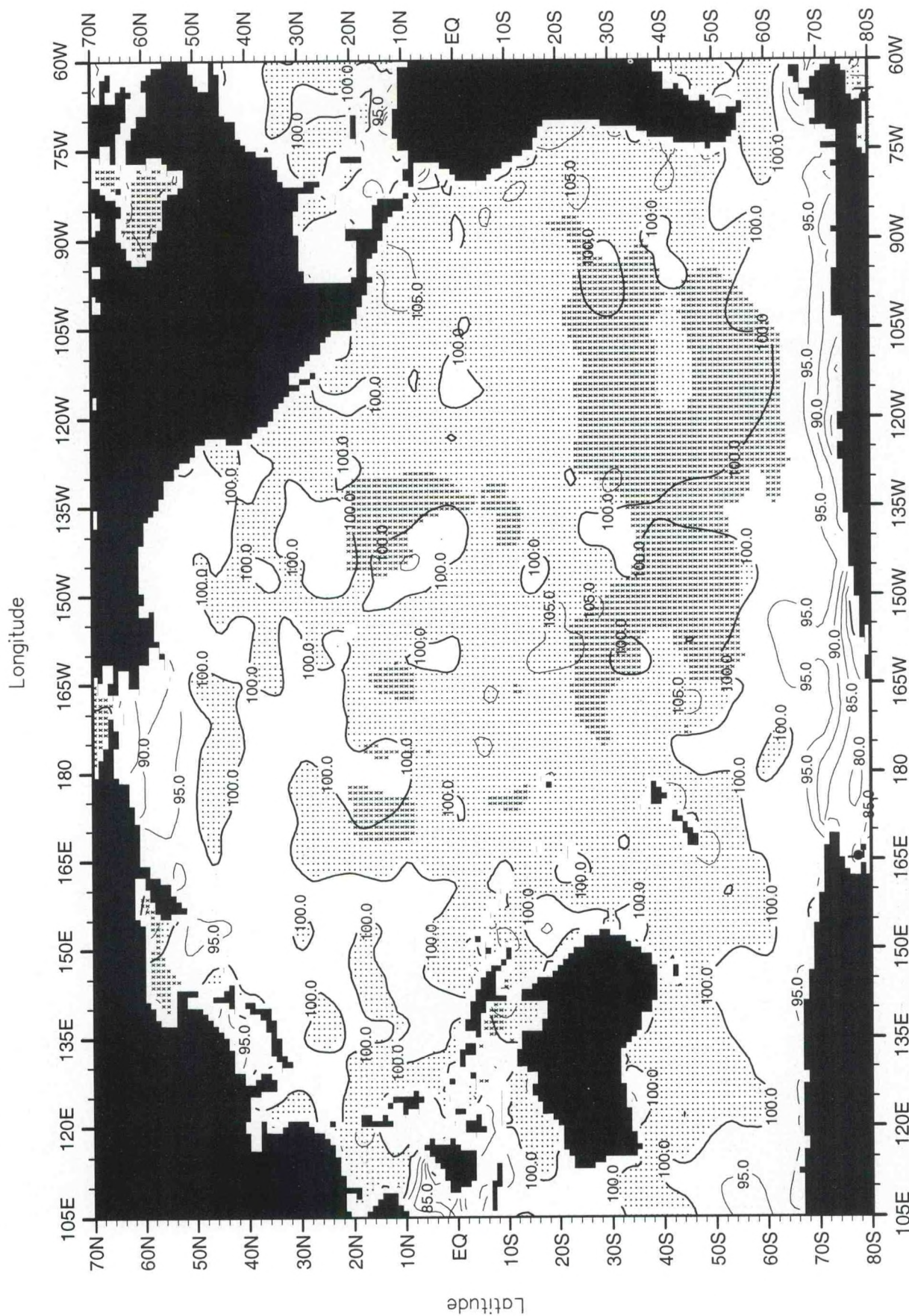
Fig. H1. Winter (Jan.-Mar.) mean oxygen saturation (%) at the surface .
