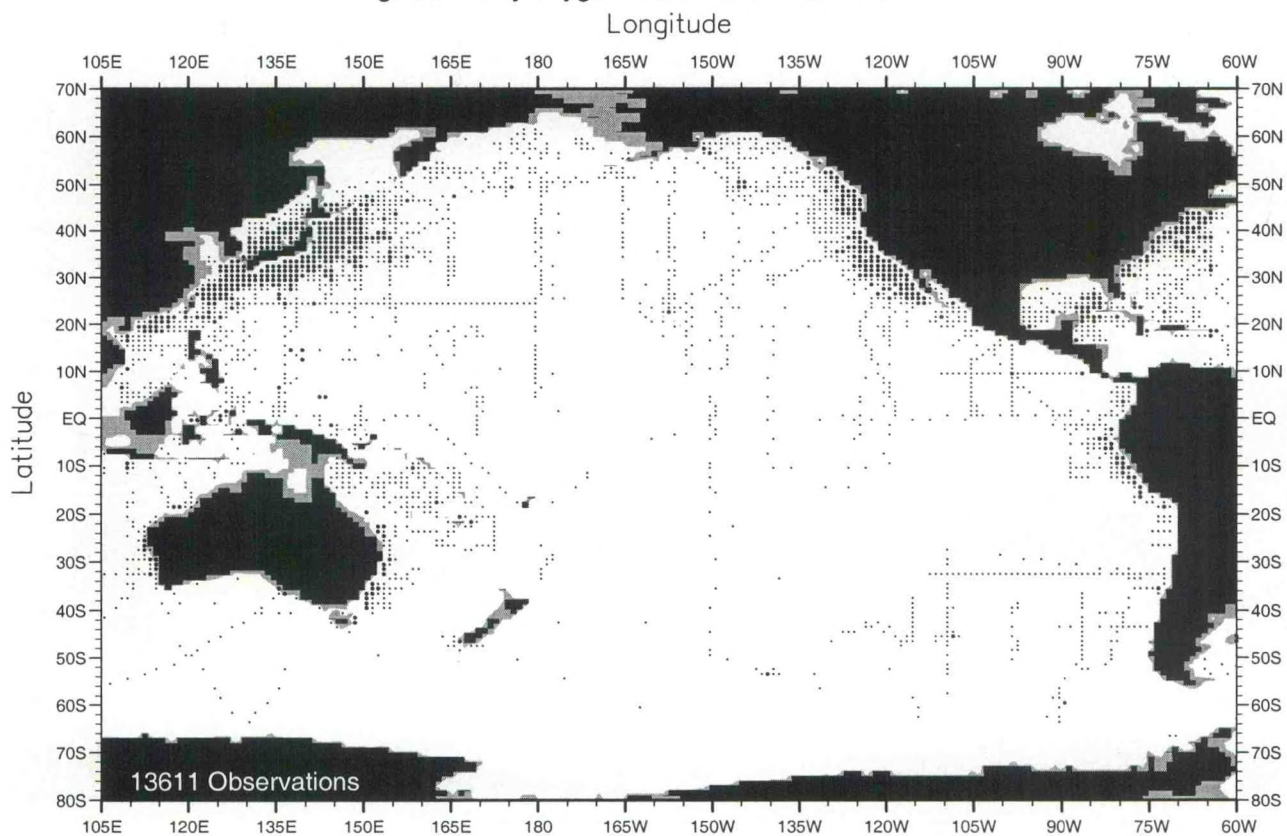
Fig. C10. May oxygen observations at 75 m. depth .
