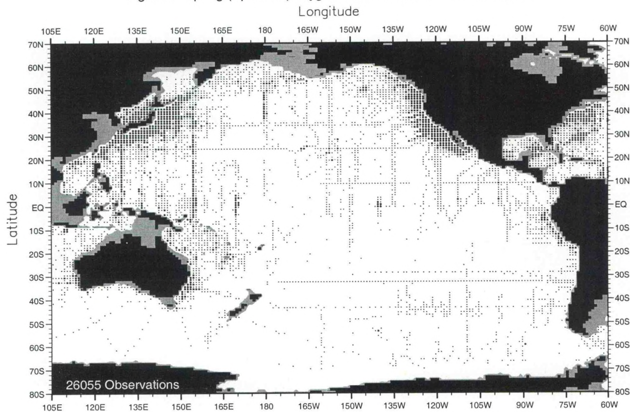
Fig. B8. Spring (Apr.-Jun.) oxygen observations at 250 m. depth .
