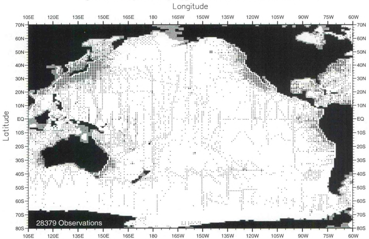
Fig. B14. Fall (Oct.-Dec.) oxygen observations at 75 m. depth .
