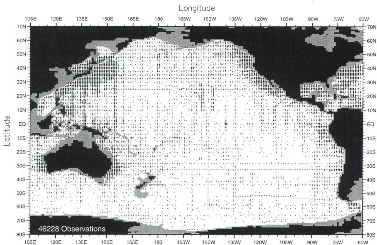
Fig. A11. Annual oxygen observations at 1000 m. depth .
