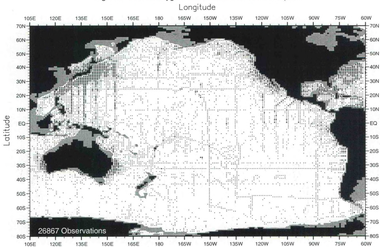
Fig. A10. Annual oxygen observations at 700 m. depth .
