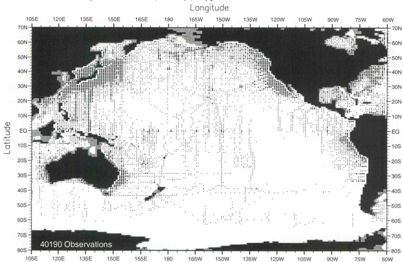
Fig. B10. Summer (Jul.-Sep.) oxygen observations at 75 m. depth .
