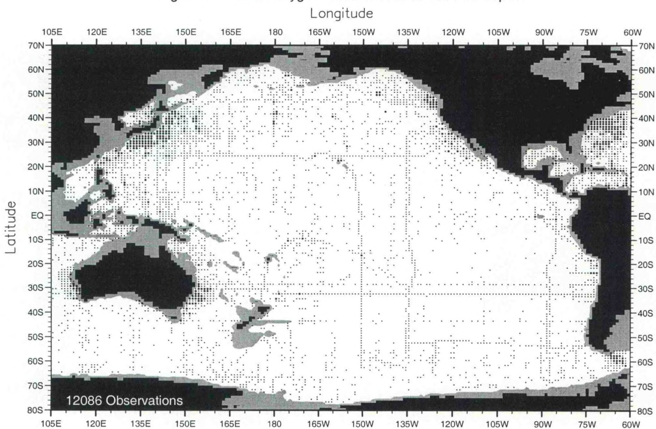
Fig. A12. Annual oxygen observations at 1500 m. depth .
