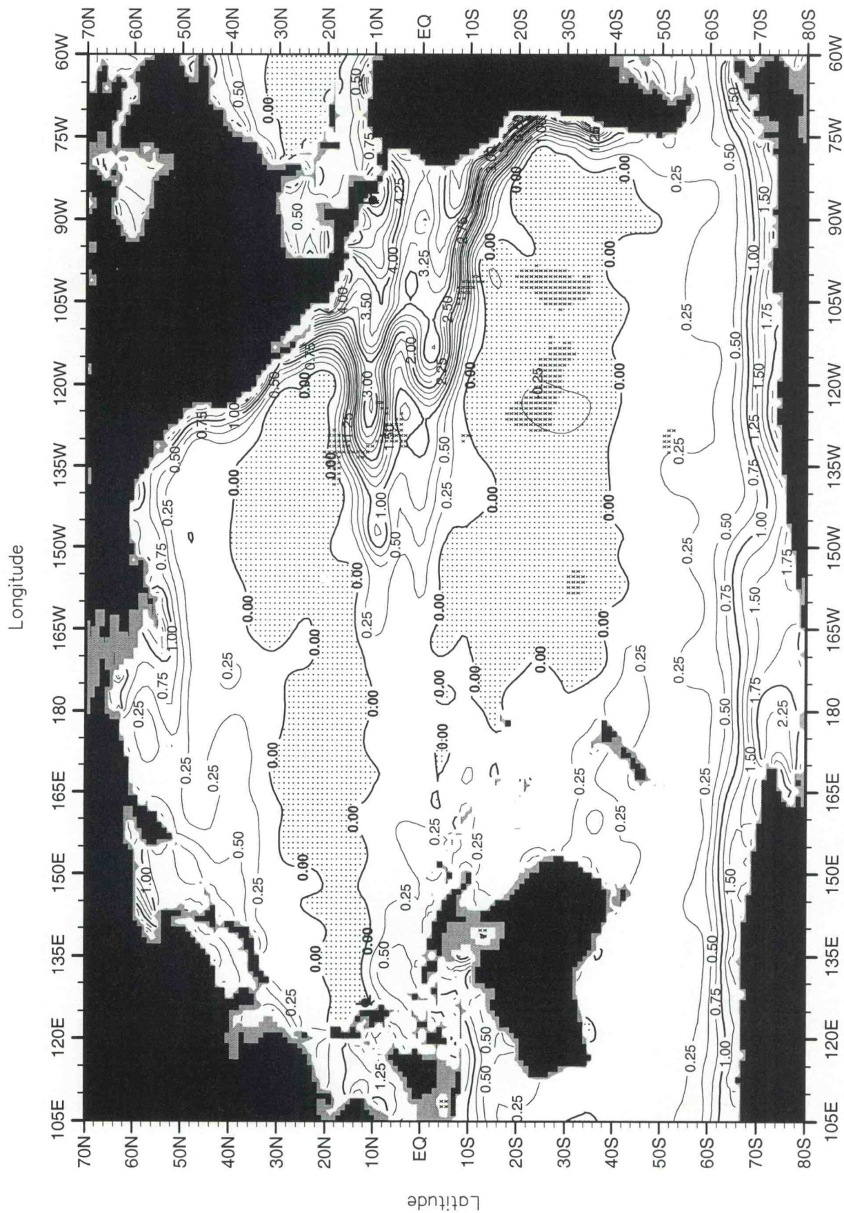
Fig. D3. Annual mean Apparent Oxygen Utilization (ml/l) at 75 m. depth .
