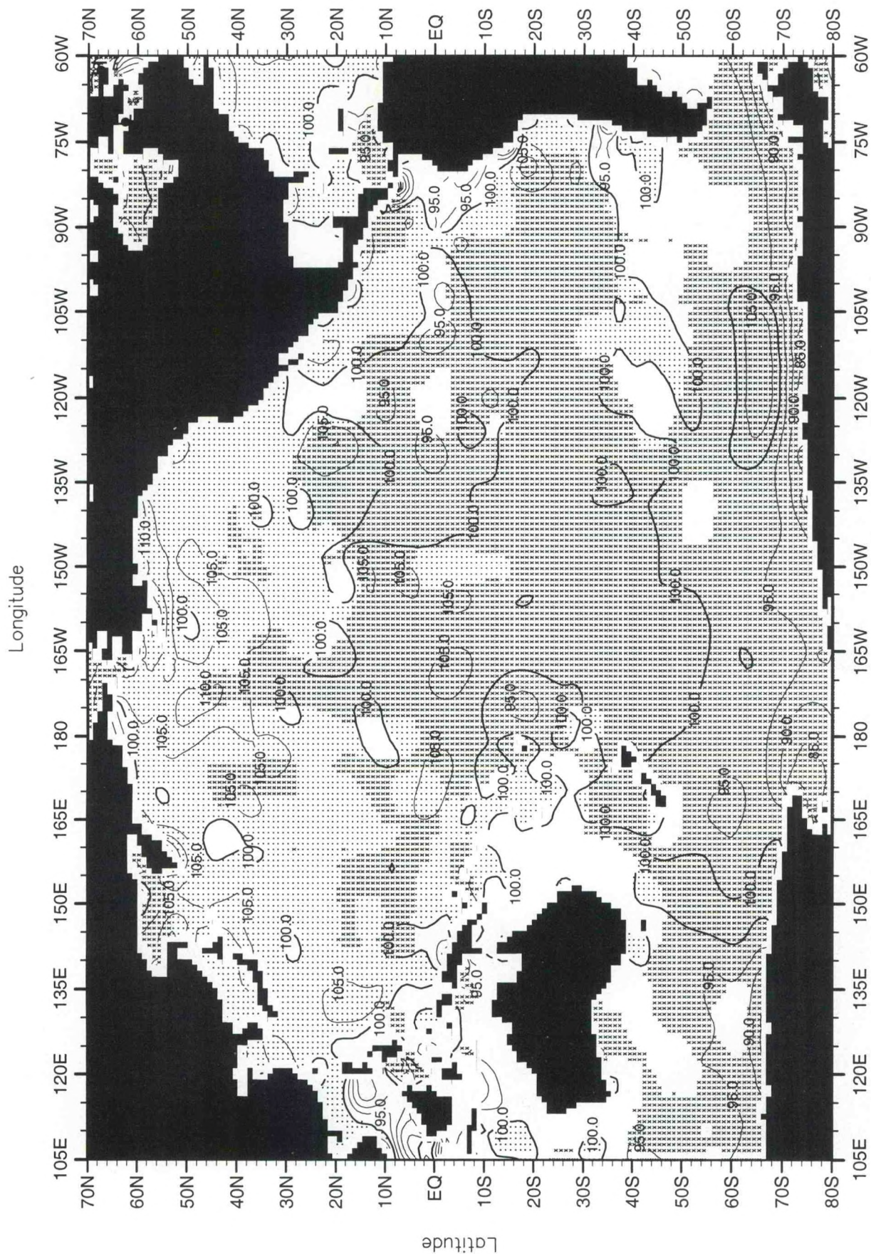
Fig. I9. May mean oxygen saturation (%) at the surface .
