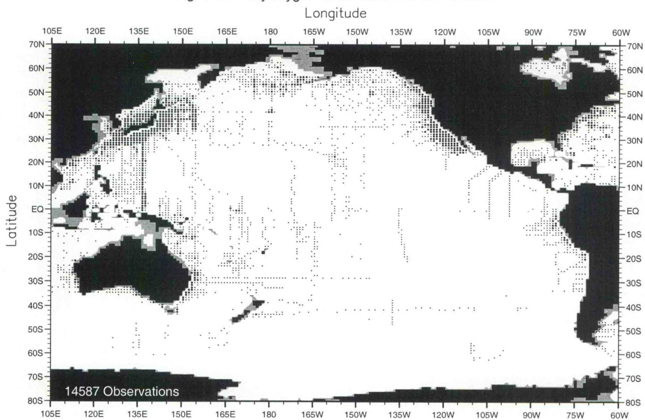
Fig. C14. July oxygen observations at 75 m. depth .
