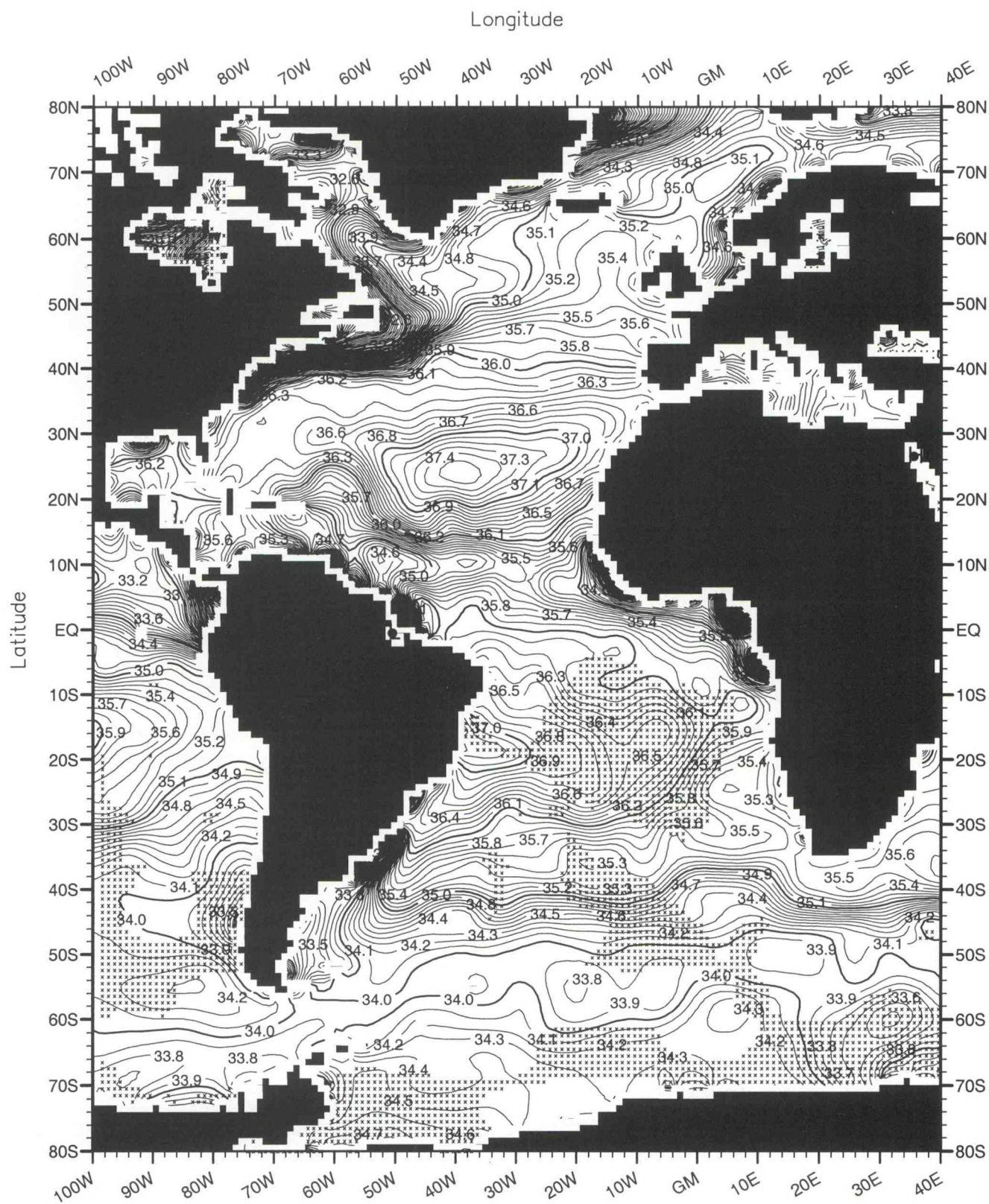
Fig. C65. November mean salinity (PSS) at the surface .
