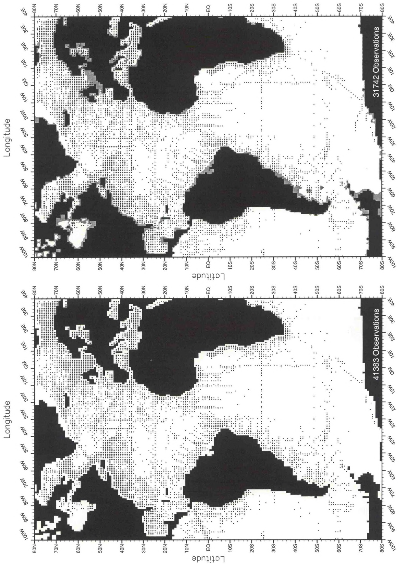
Fig. C19. October salinity observations at the surface .
