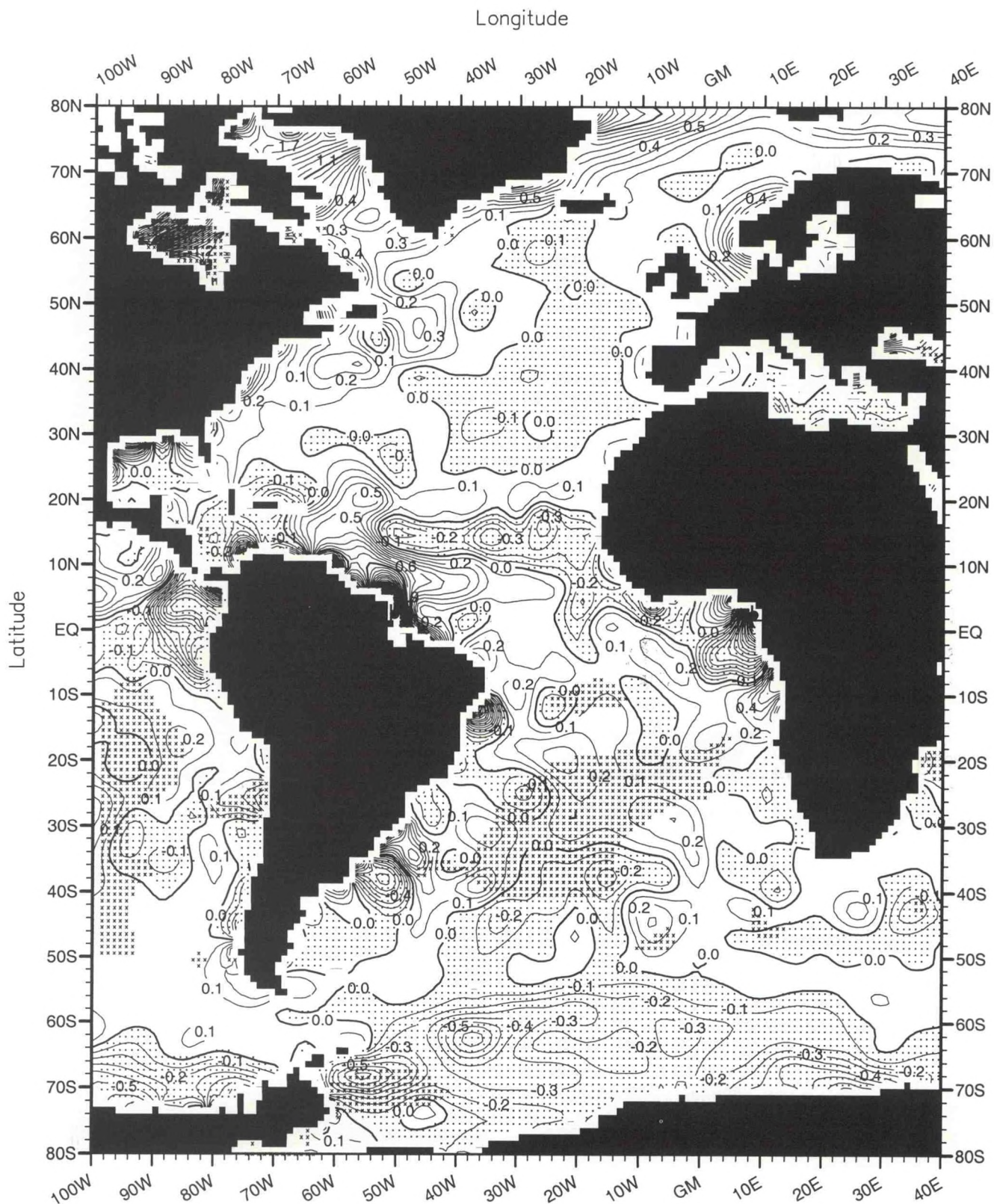
Fig. C26. January minus annual salinity (PSS) at the surface .
