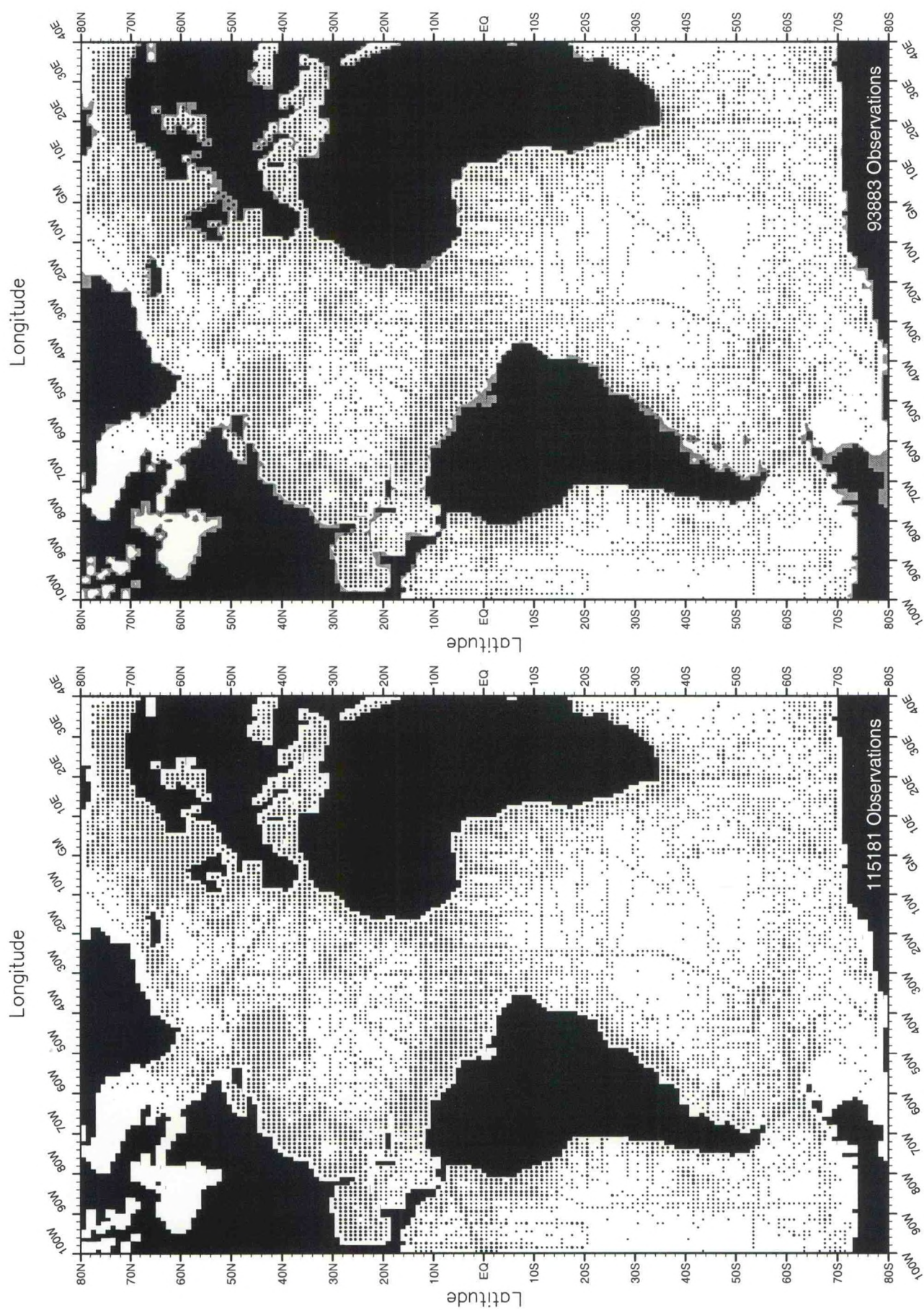
Fig. B1. Winter (Jan.-Mar.) salinity observations at the surface .
