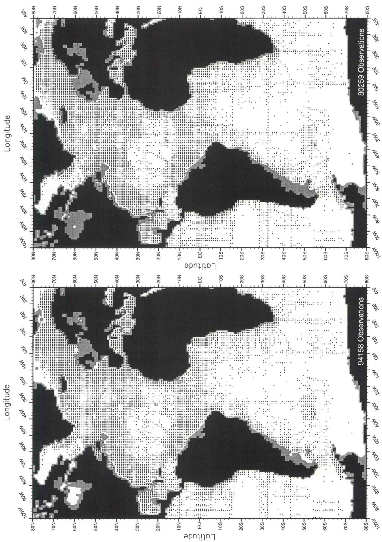
Fig. B11. Spring (Apr.-Jun.) salinity observations at 150 m. depth .
