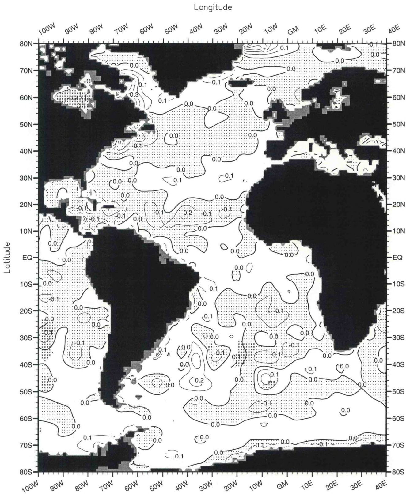
Fig. B30. Winter (Jan.-Mar.) minus annual salinity (PSS) at 75 m. depth . Minimum Value= -0.44 Maximum Value= 1.21 Contour Interval: 0.10
