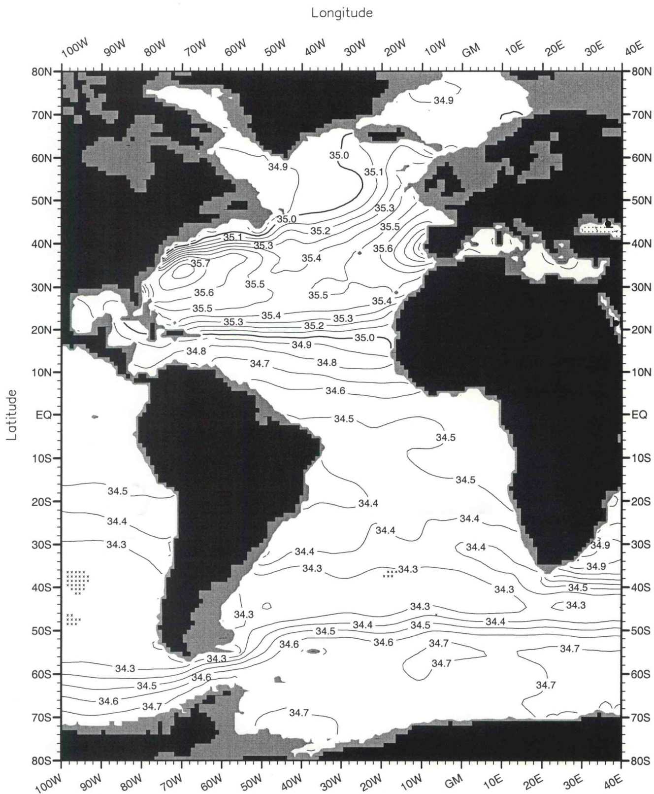
Fig. A26. Annual mean salinity (PSS) at 700 m. depth .
