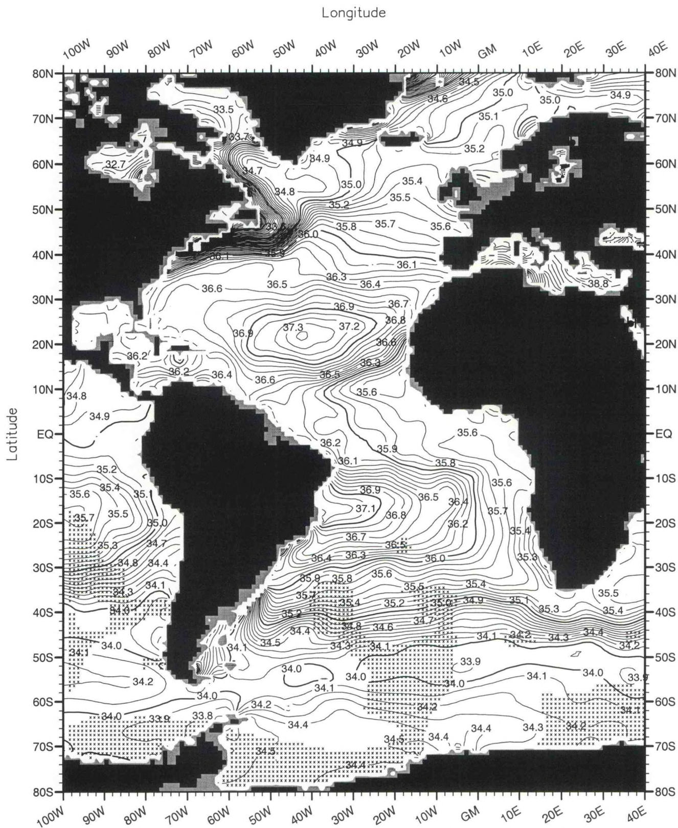
Fig. B53. Summer (Jul.-Sep.) mean salinity (PSS) at 75 m. depth .
