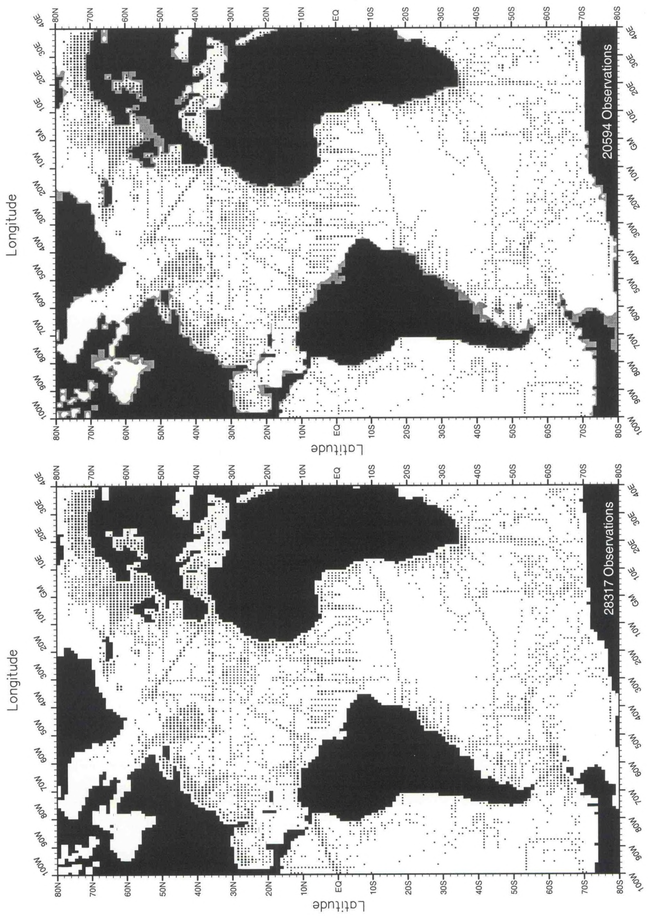
Fig. C1. January salinity observations at the surface .
