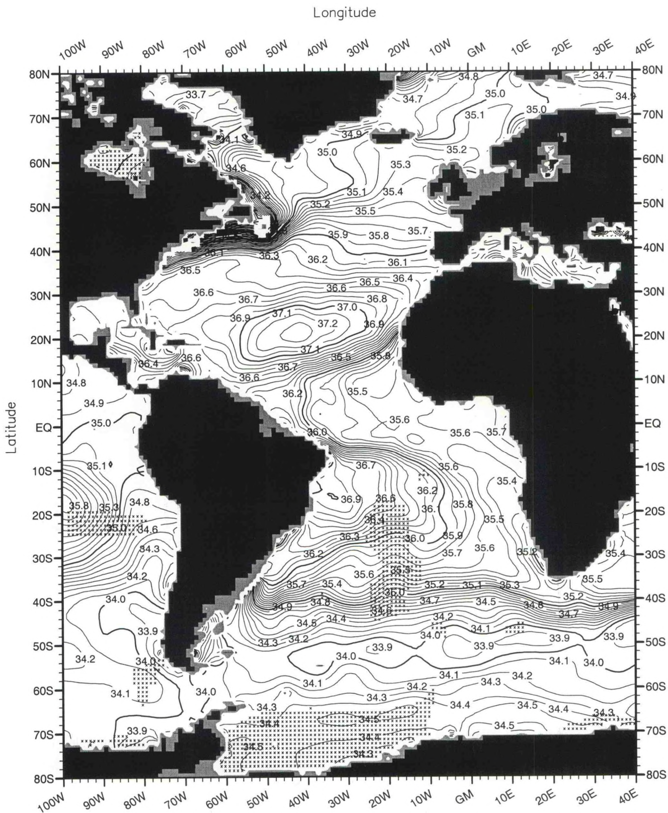
Fig. B43. Spring (Apr.-Jun.) mean salinity (PSS) at 100 m. depth .
