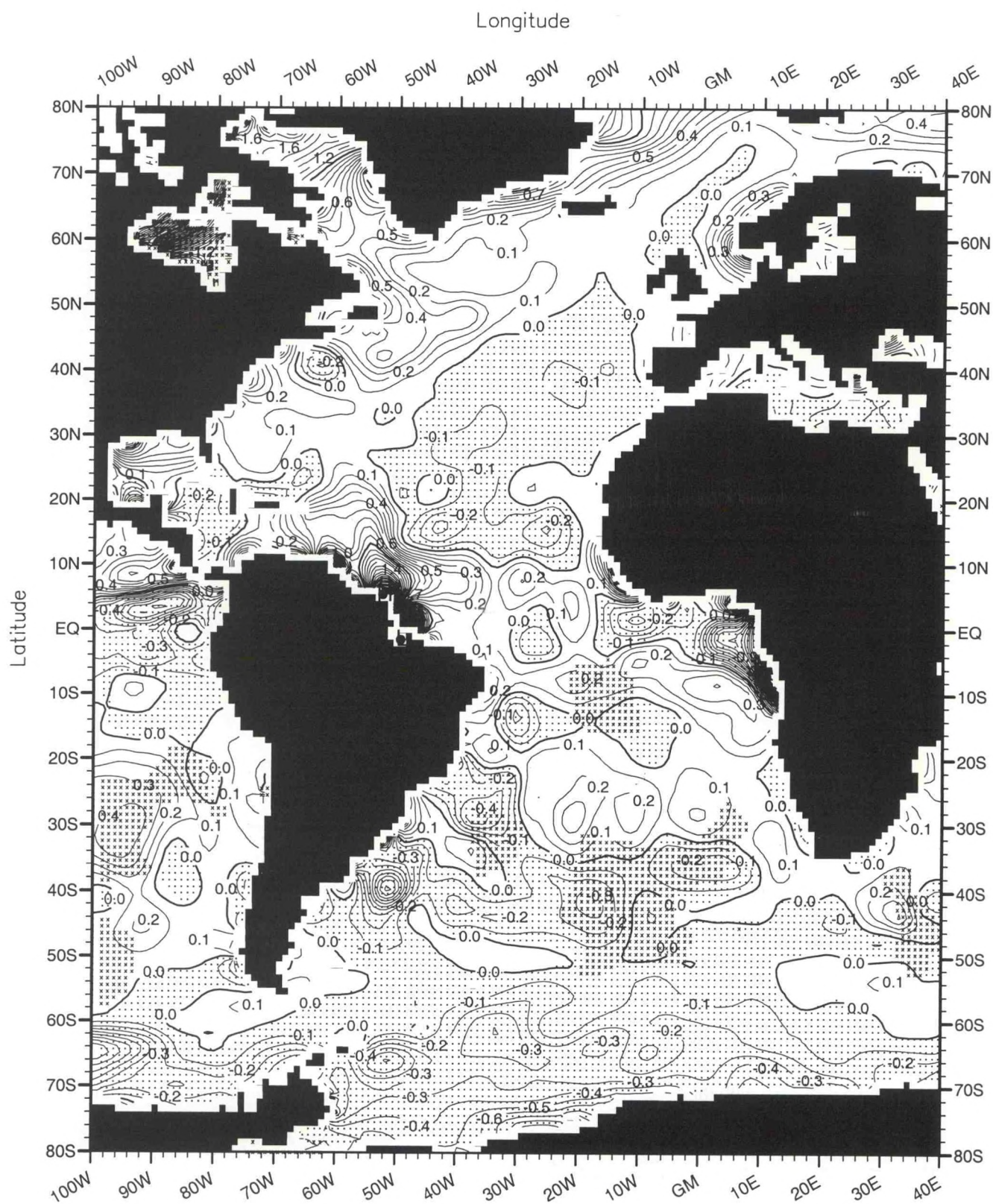
Fig. C30. February minus annual salinity (PSS) at the surface .
