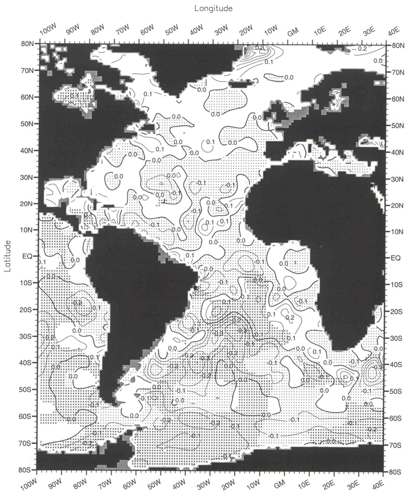
Fig. C48. June minus annual salinity (PSS) at 75 m. depth .
