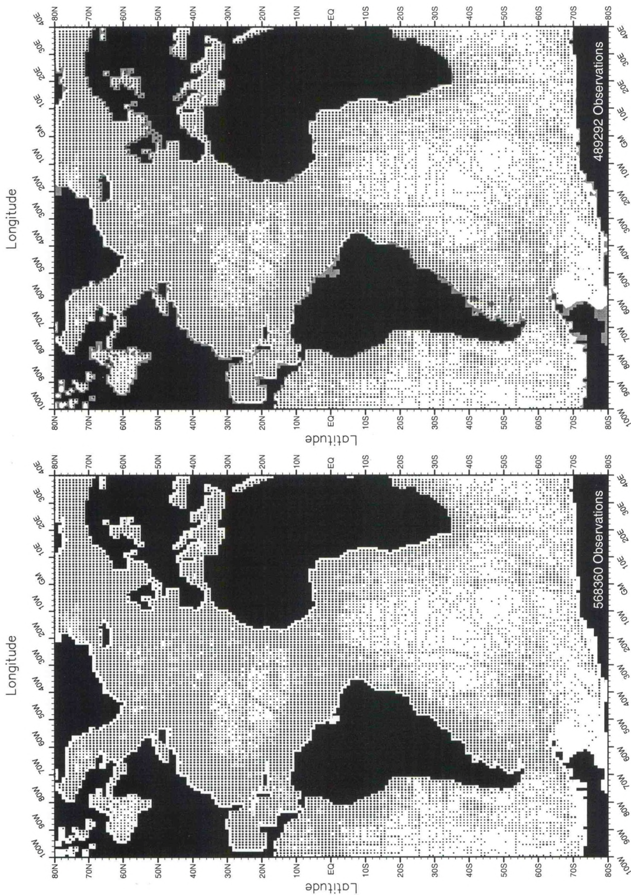
Fig. A1. Annual salinity observations at the surface .
