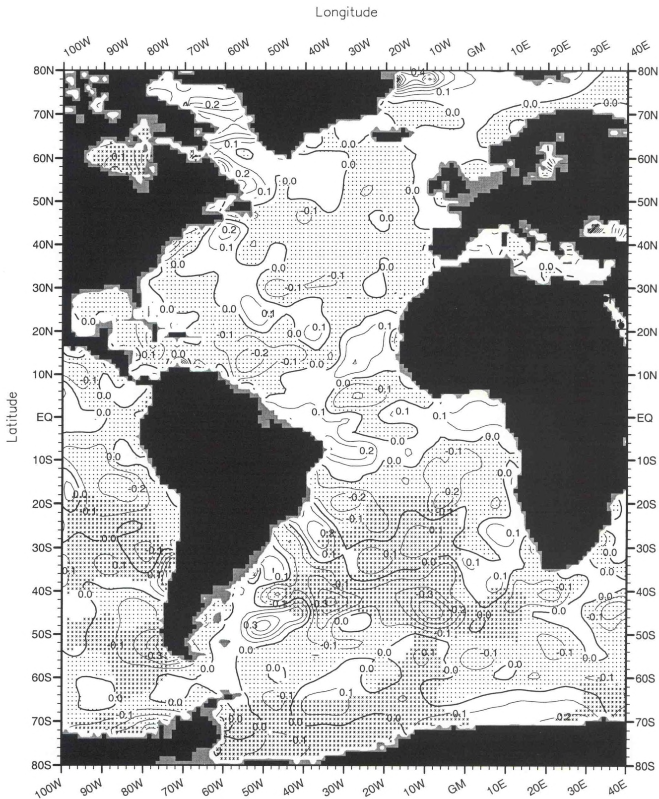
Fig. C40. April minus annual salinity (PSS) at 75 m. depth .
