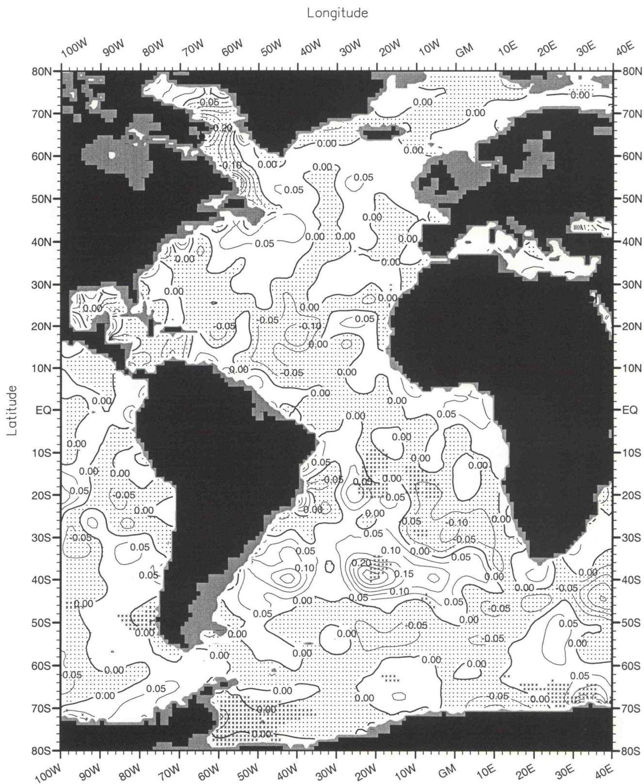
Fig. B72. Fall (Oct.-Dec.) minus annual salinity (PSS) at 250 m. depth .
