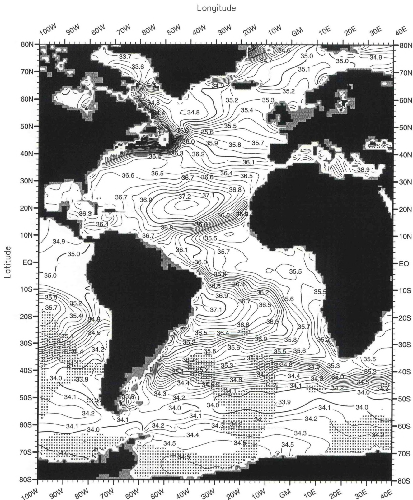
Fig. B55. Summer (Jul.-Sep.) mean salinity (PSS) at 100 m. depth . Minimum Value= 4.32 Maximum Value= 40.72 Contour Interval: 0.10
