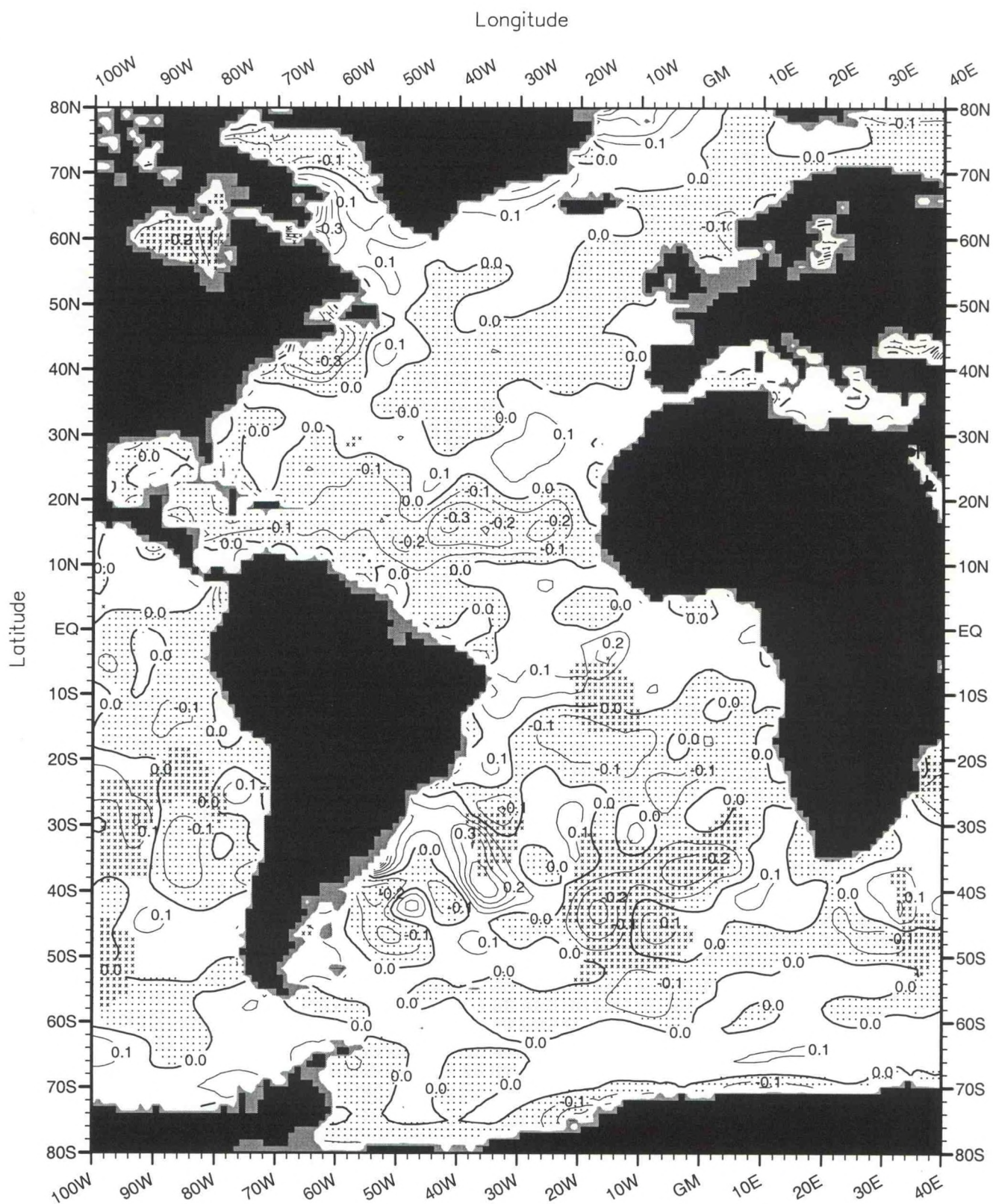
Fig. C32. February minus annual salinity (PSS) at 75 m. depth .
