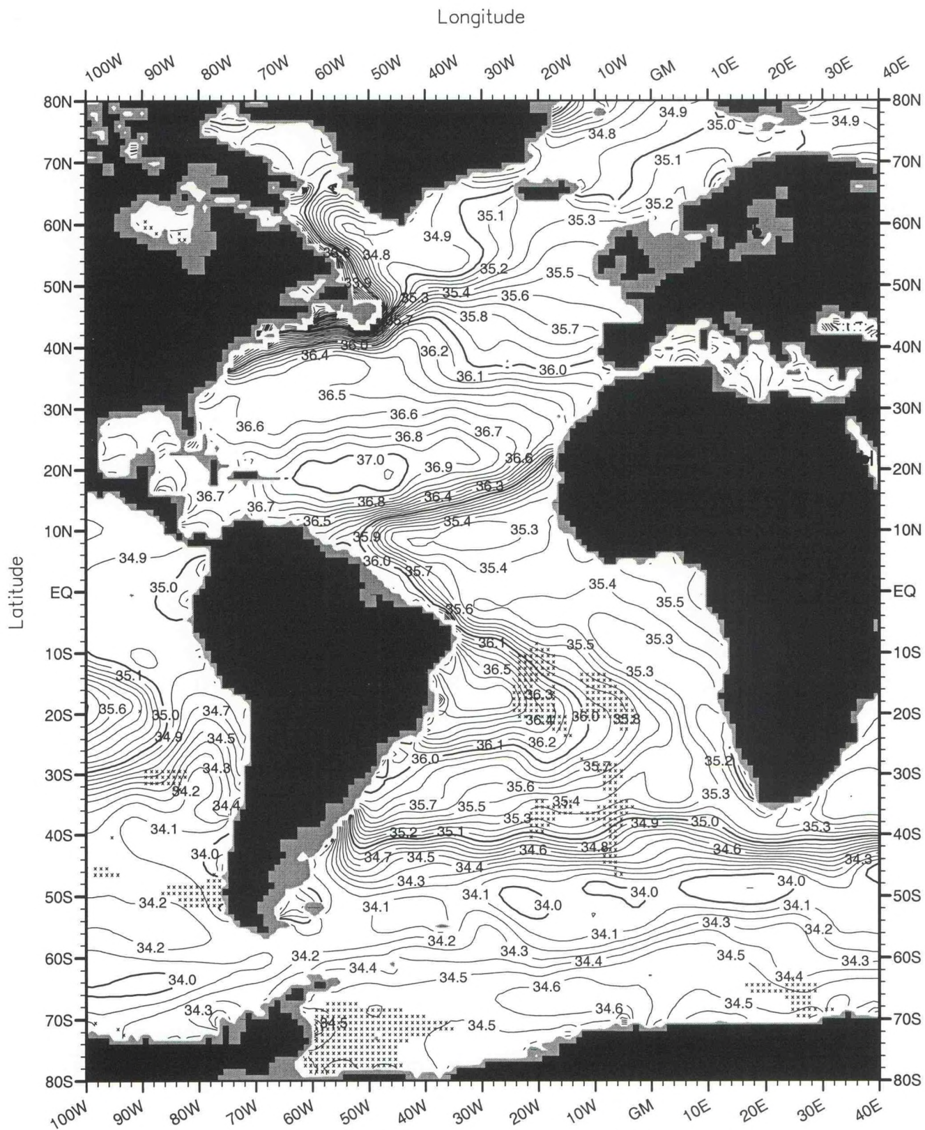
Fig. B69. Fall (Oct.-Dec.) mean salinity (PSS) at 150 m. depth . Minimum Value= 10.65 Maximum Value= 40.56 Contour Interval: 0.10
