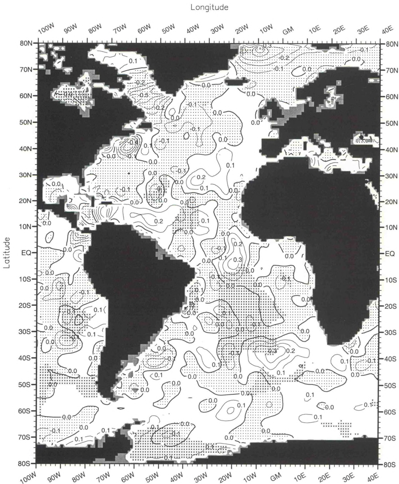
Fig. C72. December minus annual salinity (PSS) at 75 m. depth .
