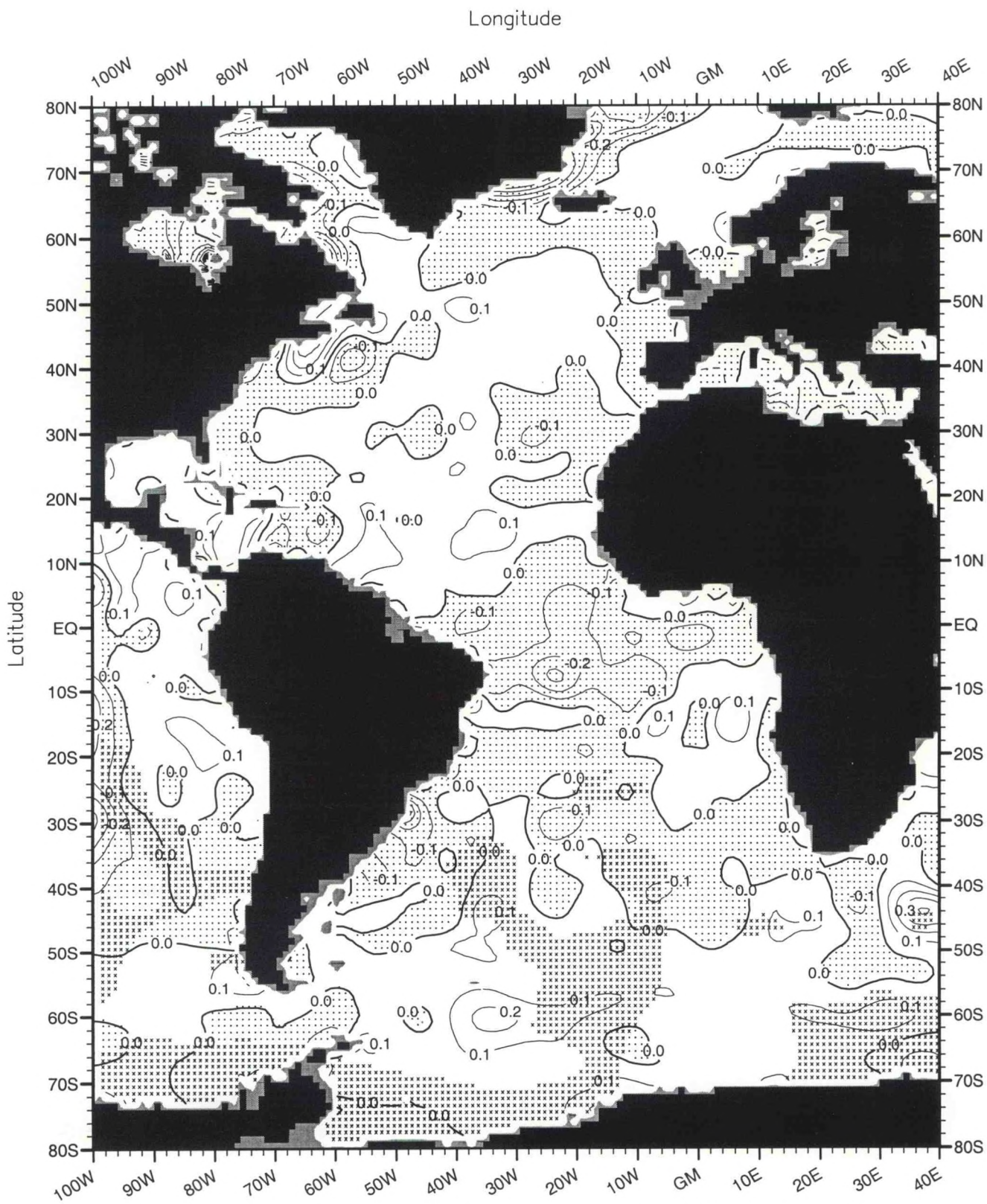
Fig. B52. Summer (Jul.-Sep.) minus annual salinity (PSS) at 50 m. depth . Minimum Value= -4.11 Maximum Value= 1.54 Contour Interval: 0.10
