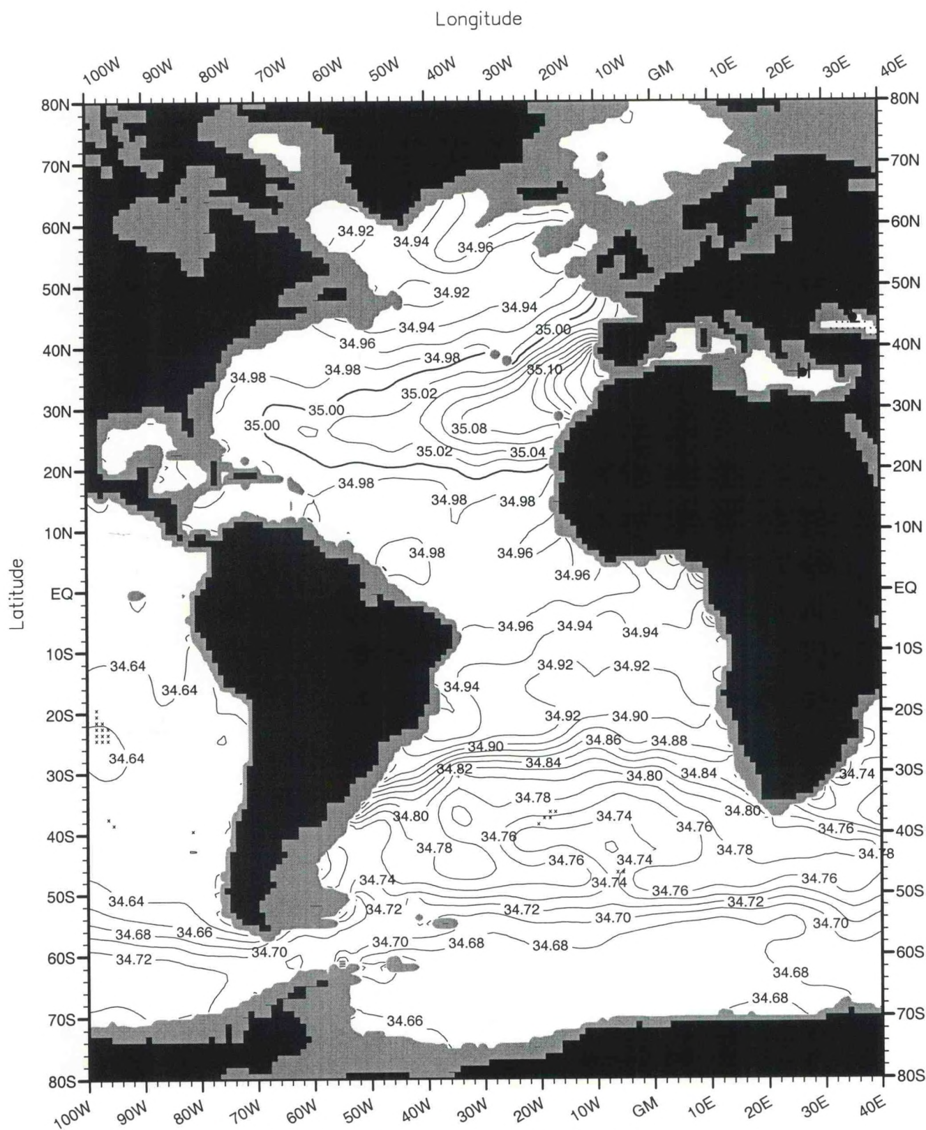
Fig. A29. Annual mean salinity (PSS) at 2000 m. depth .
