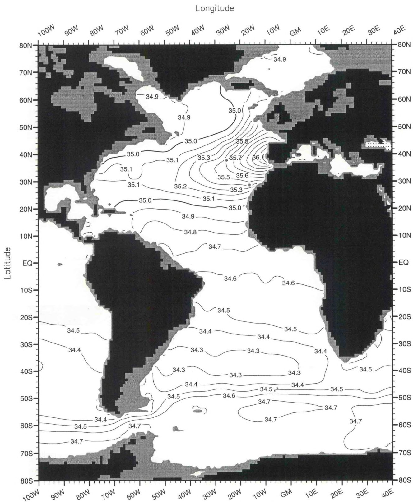
Fig. A27. Annual mean salinity (PSS) at 1000 m. depth .
