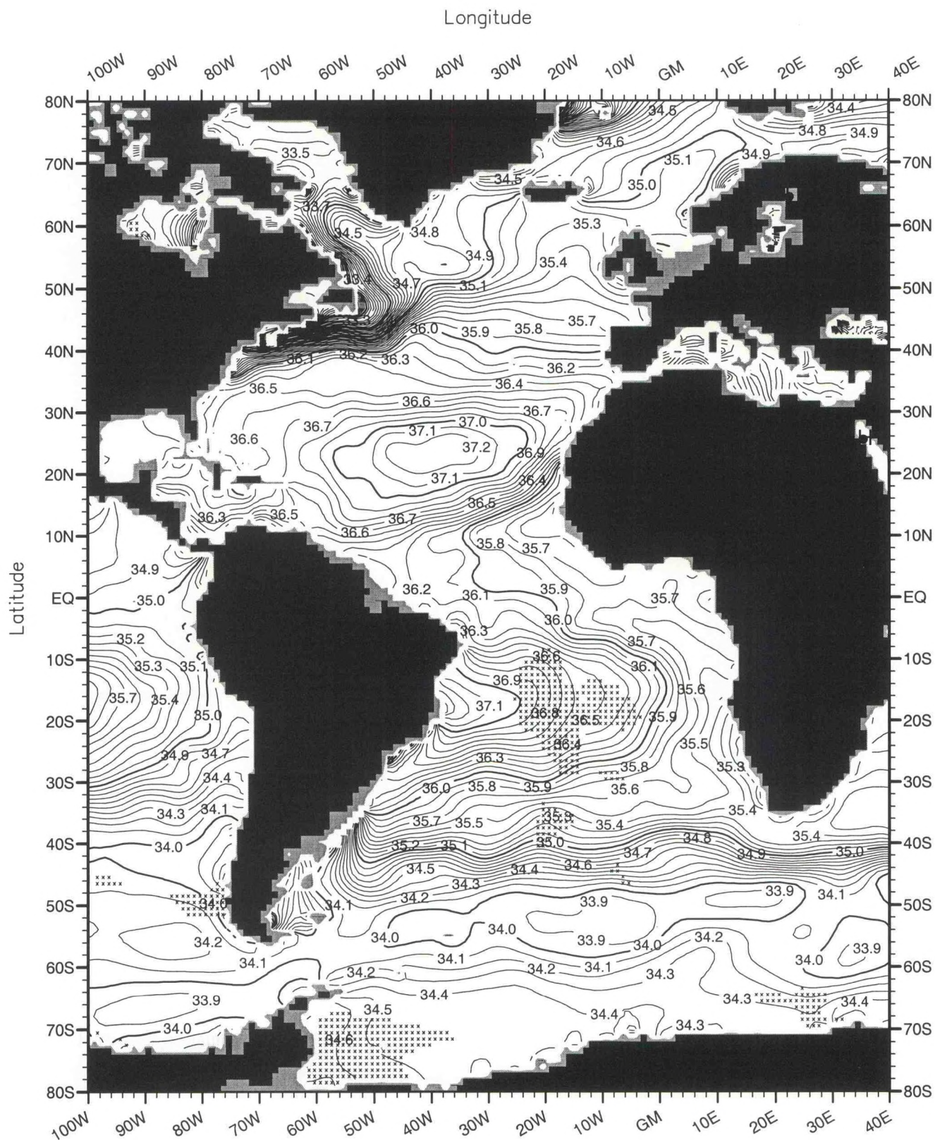
Fig. B65. Fall (Oct.-Dec.) mean salinity (PSS) at 75 m. depth .
