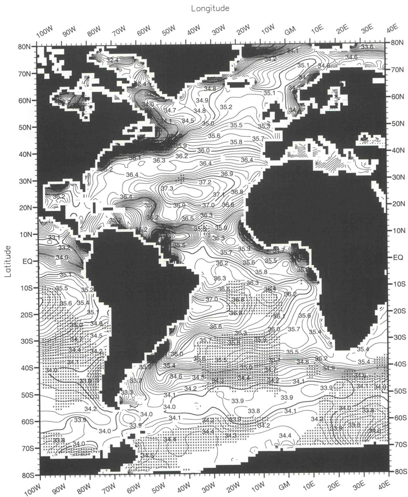
Fig. C61. October mean salinity (PSS) at the surface .
