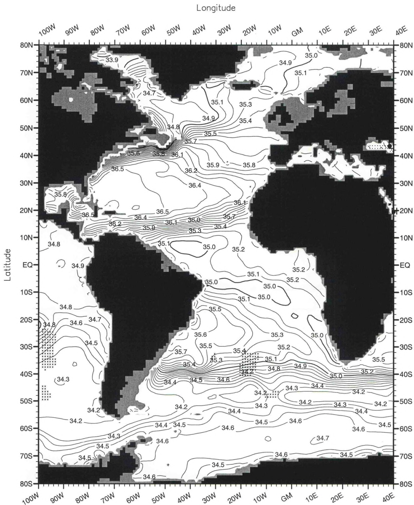
Fig. B35. Winter (Jan.-Mar.) mean salinity (PSS) at 250 m. depth . Minimum Value= 21.34 Maximum Value= 40.58 Contour Interval: 0.10
