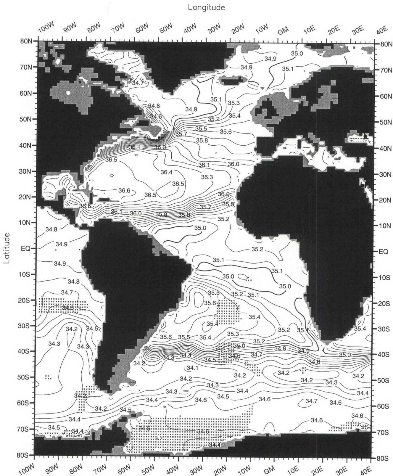
Fig. B47. Spring (Apr.-Jun.) mean salinity (PSS) at 250 m. depth . Minimum Value= 21.33 Maximum Value= 40.83 Contour Interval: 0.10
