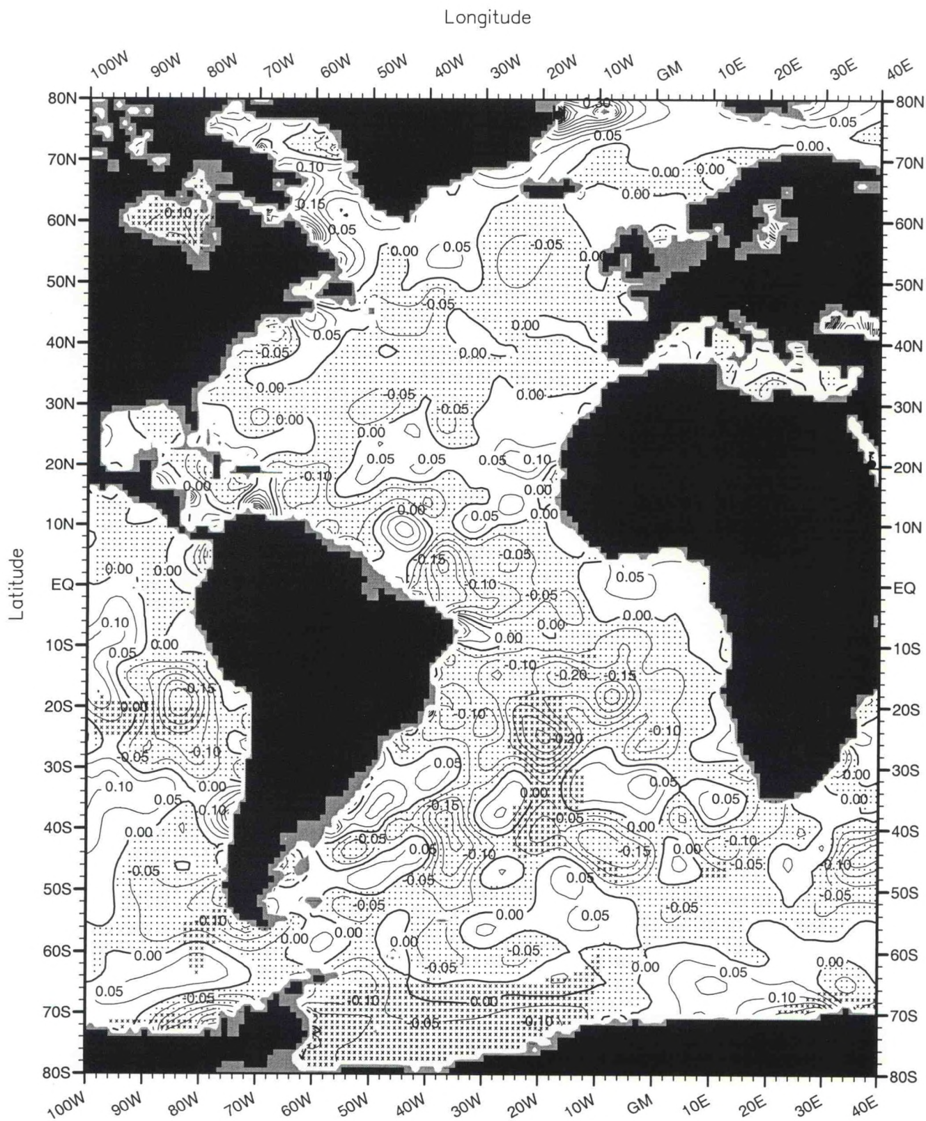
Fig. B44. Spring (Apr.-Jun.) minus annual salinity (PSS) at 100 m. depth . Minimum Value= -0.52 Maximum Value= 0.81 Contour Interval: 0.05
