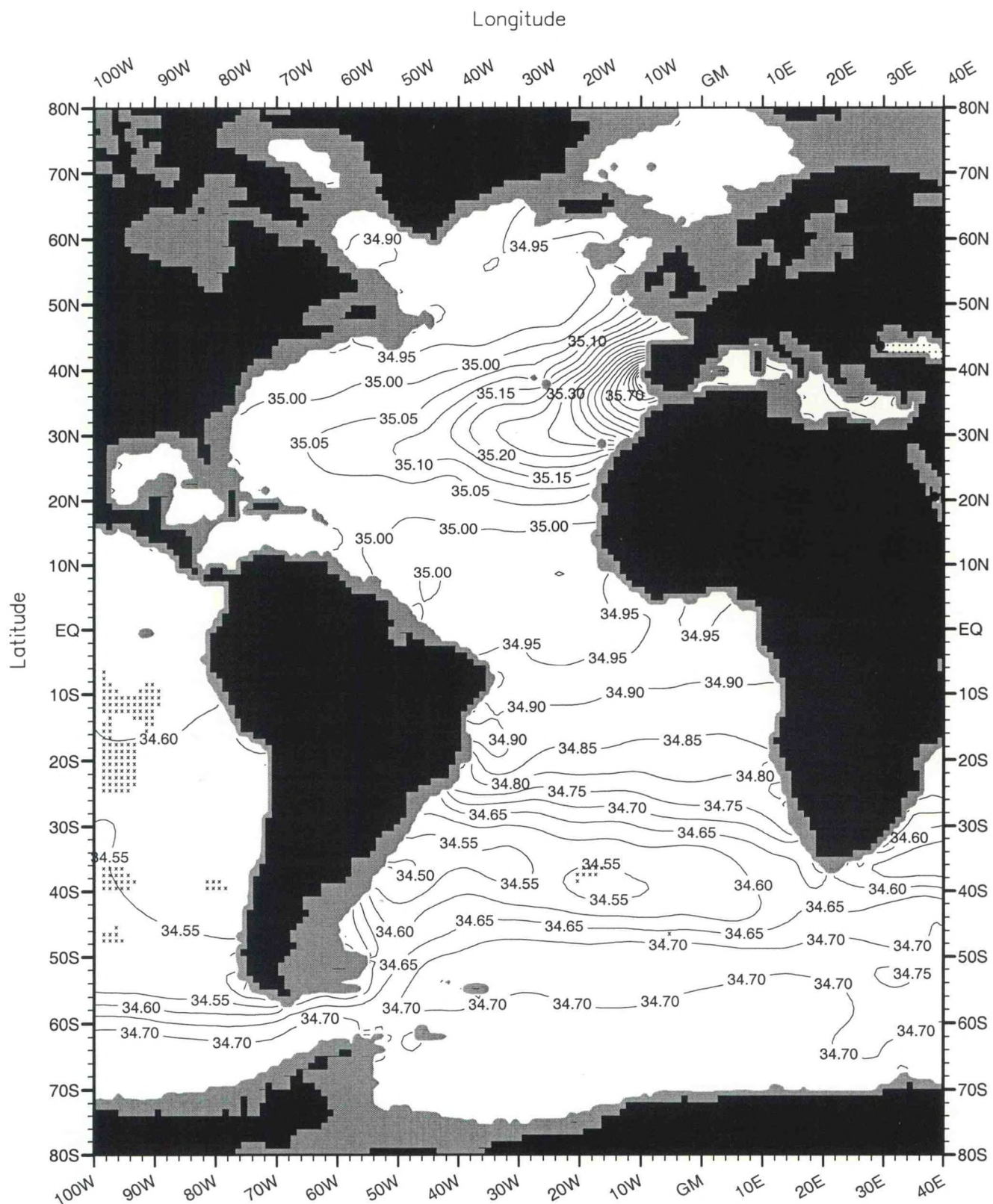
Fig. A28. Annual mean salinity (PSS) at 1500 m. depth .
