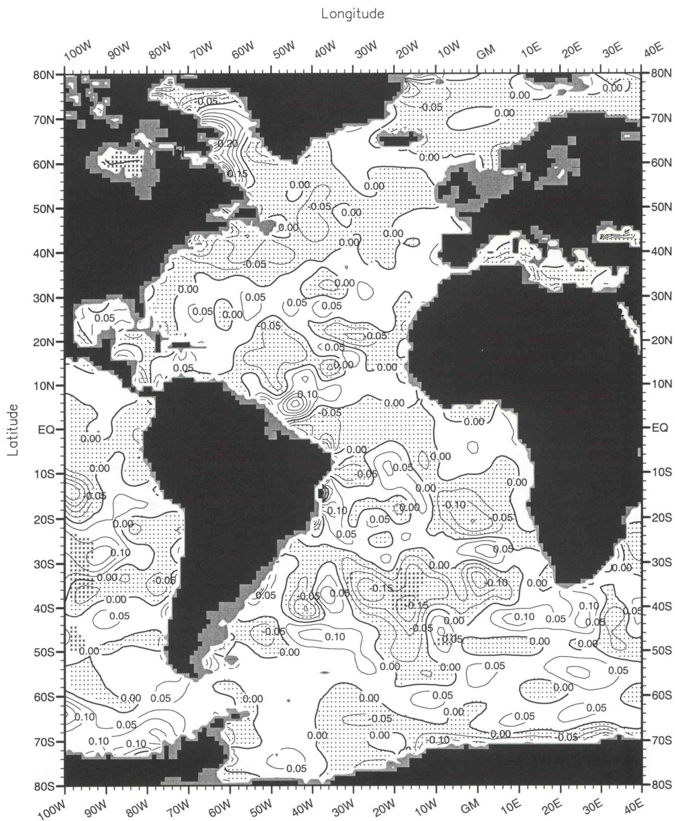
Fig. B34. Winter (Jan.-Mar.) minus annual salinity (PSS) at 150 m. depth . Minimum Value= -0.69 Maximum Value= 0.79 Contour Interval: 0.05
