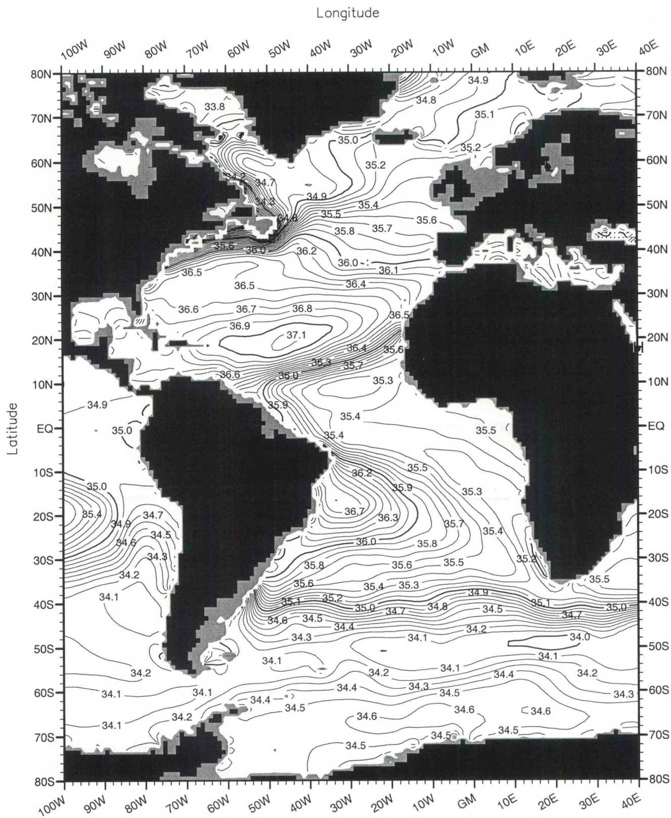
Fig. A21. Annual mean salinity (PSS) at 150 m. depth .
