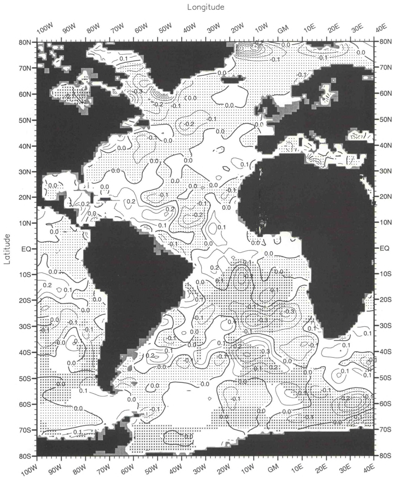
Fig. C68. November minus annual salinity (PSS) at 75 m. depth .
