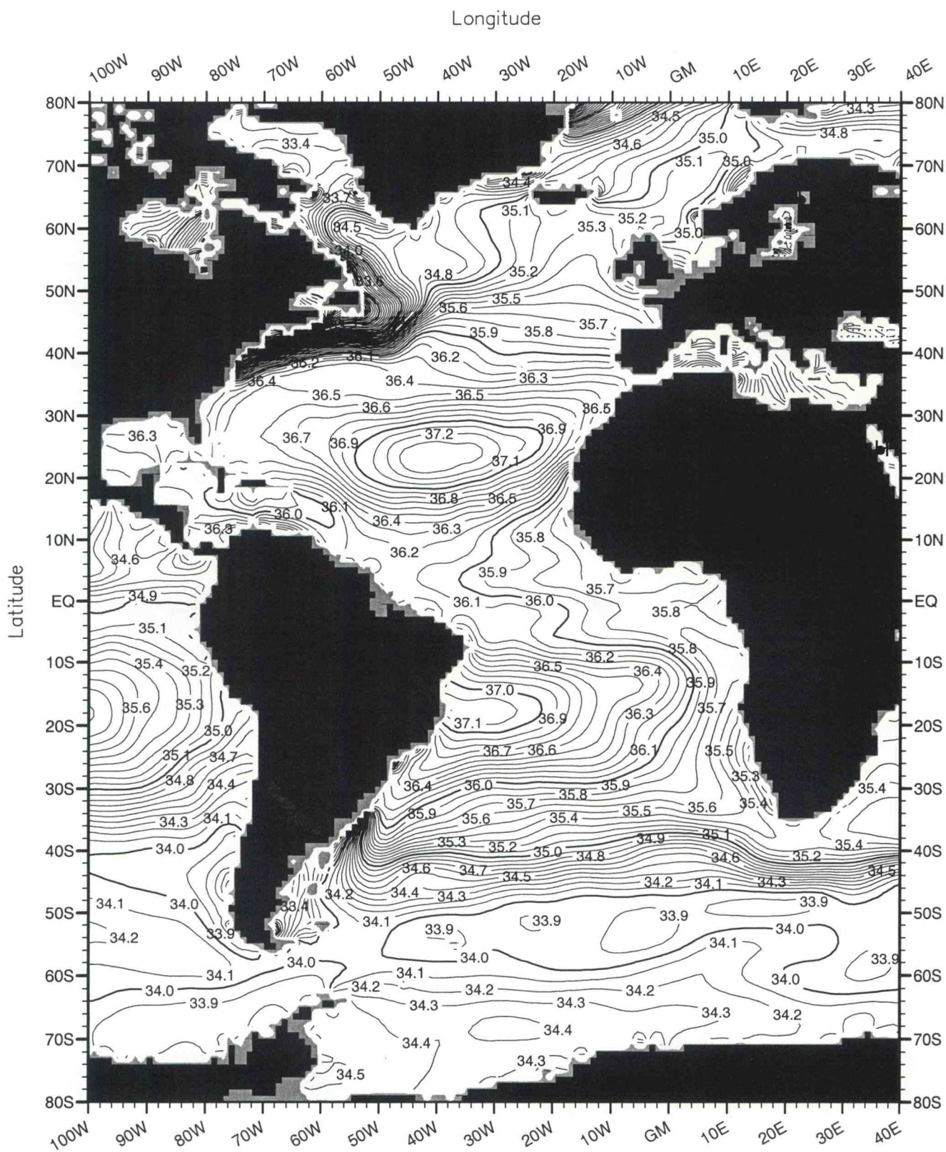
Fig. A18. Annual mean salinity (PSS) at 50 m. depth .
