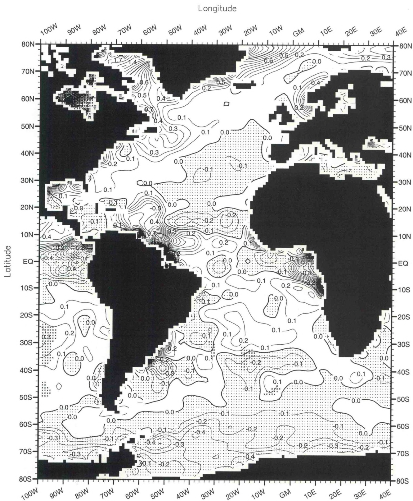
Fig. B26. Winter (Jan.-Mar.) minus annual salinity (PSS) at the surface . Minimum Value= -4.05 Maximum Value= 3.30 Contour Interval: 0.10
