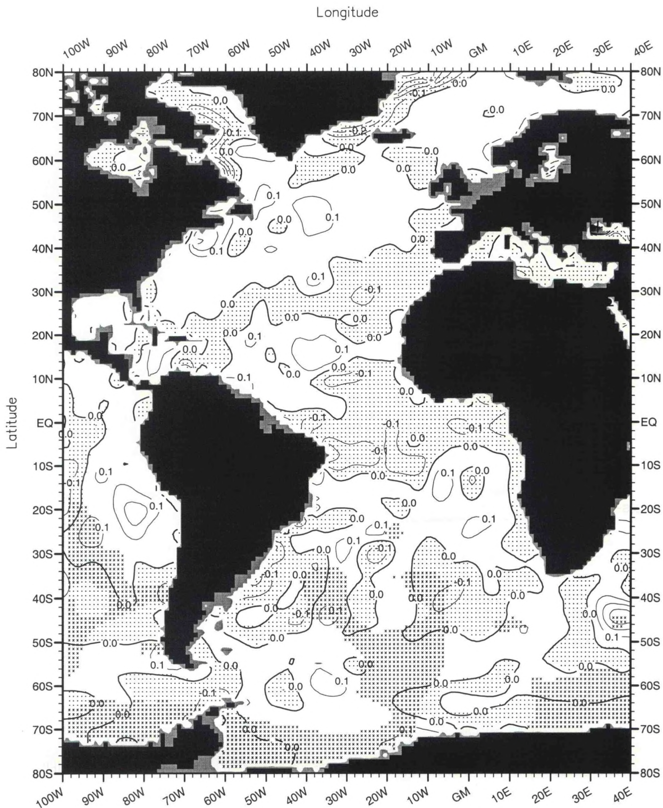
Fig. B54. Summer (Jul.-Sep.) minus annual salinity (PSS) at 75 m. depth . Minimum Value= -4.54 Maximum Value= 0.88 Contour Interval: 0.10
