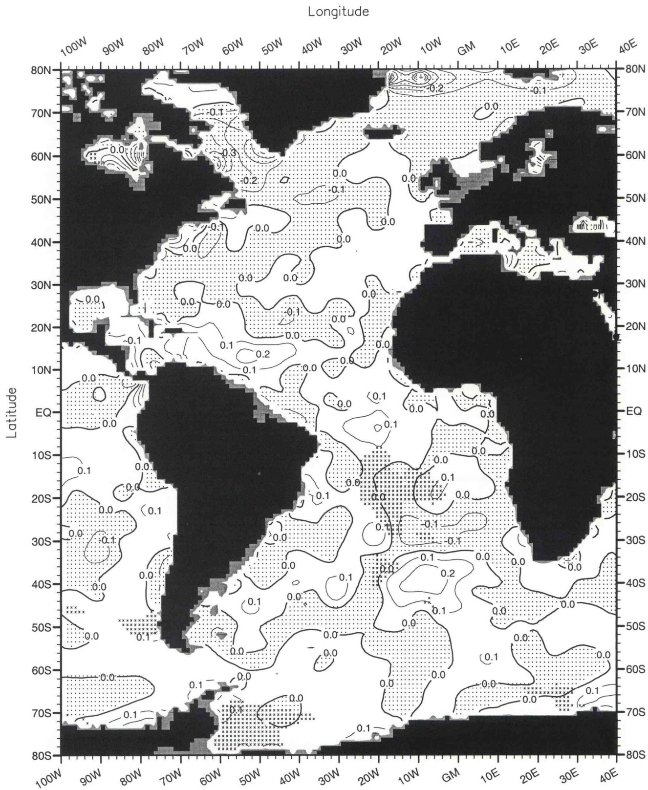
Fig. B66. Fall (Oct.-Dec.) minus annual salinity (PSS) at 75 m. depth . Minimum Value= -1.01 Maximum Value= 1.61 Contour Interval: 0.10
