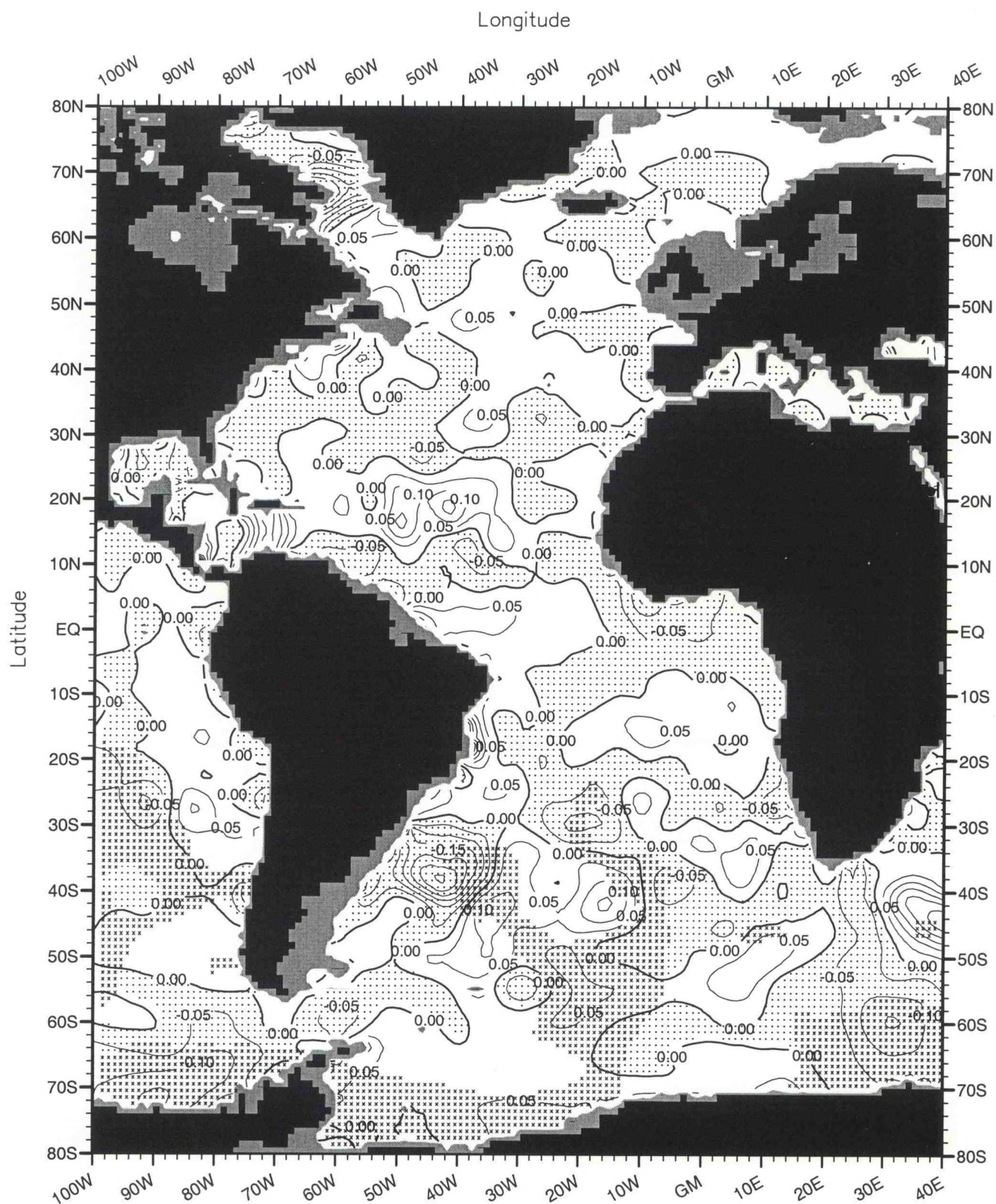
Fig. B60. Summer (Jul.-Sep.) minus annual salinity (PSS) at 250 m. depth . Minimum Value= -0.41 Maximum Value= 0.36 Contour Interval: 0.05
