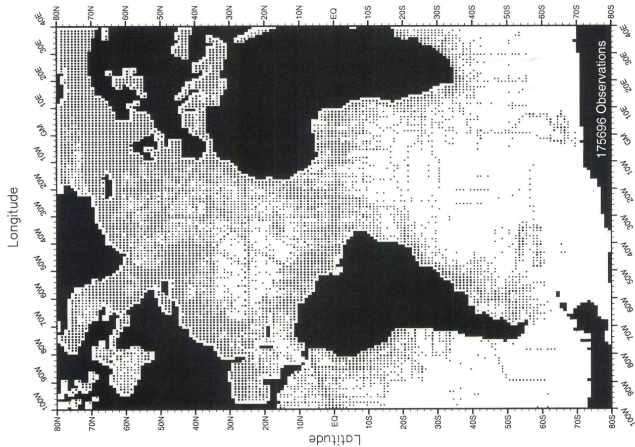
Fig. B13. Summer (Jul.-Sep.) salinity observations at the surface .
