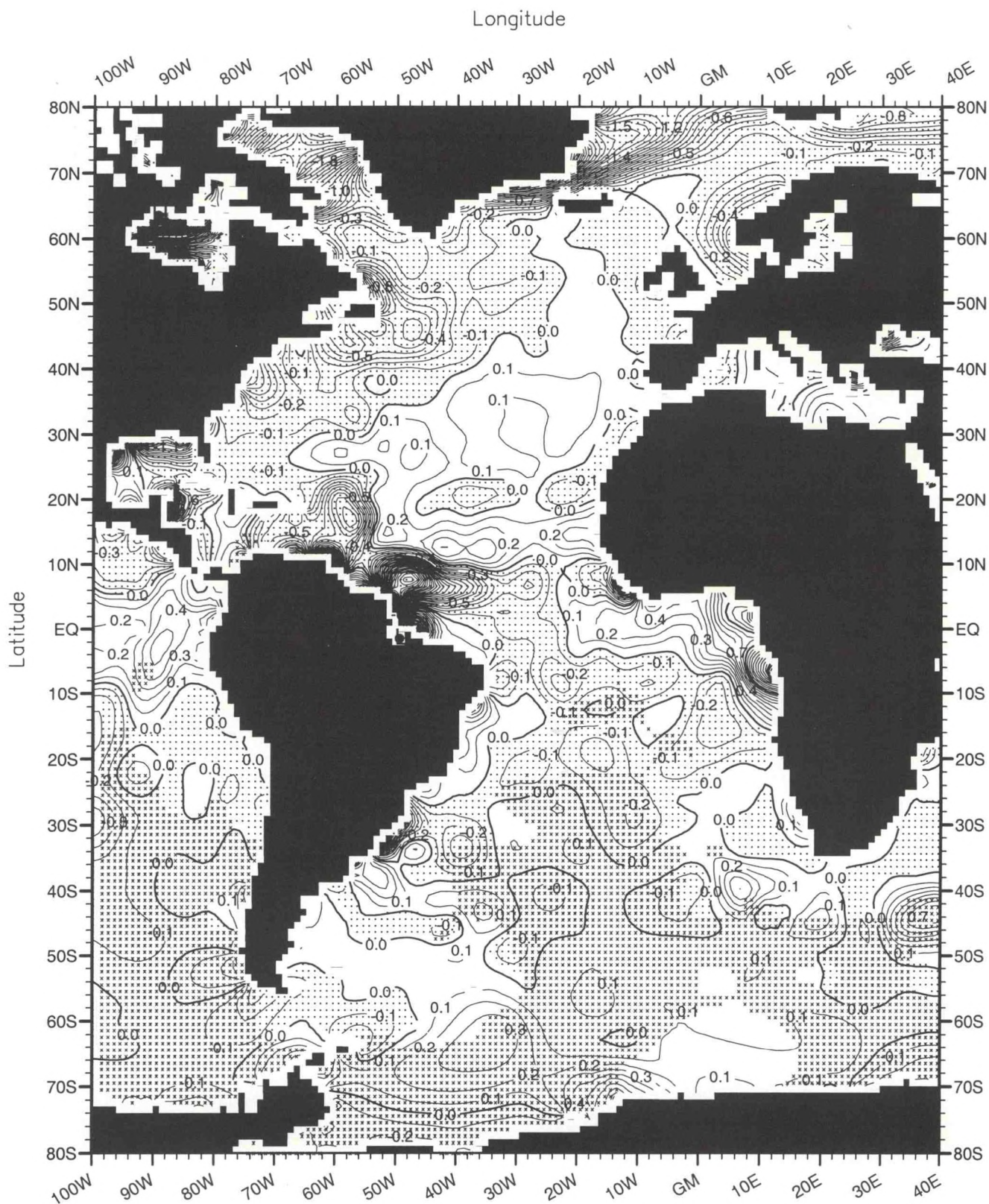
Fig. C54. August minus annual salinity (PSS) at the surface .
