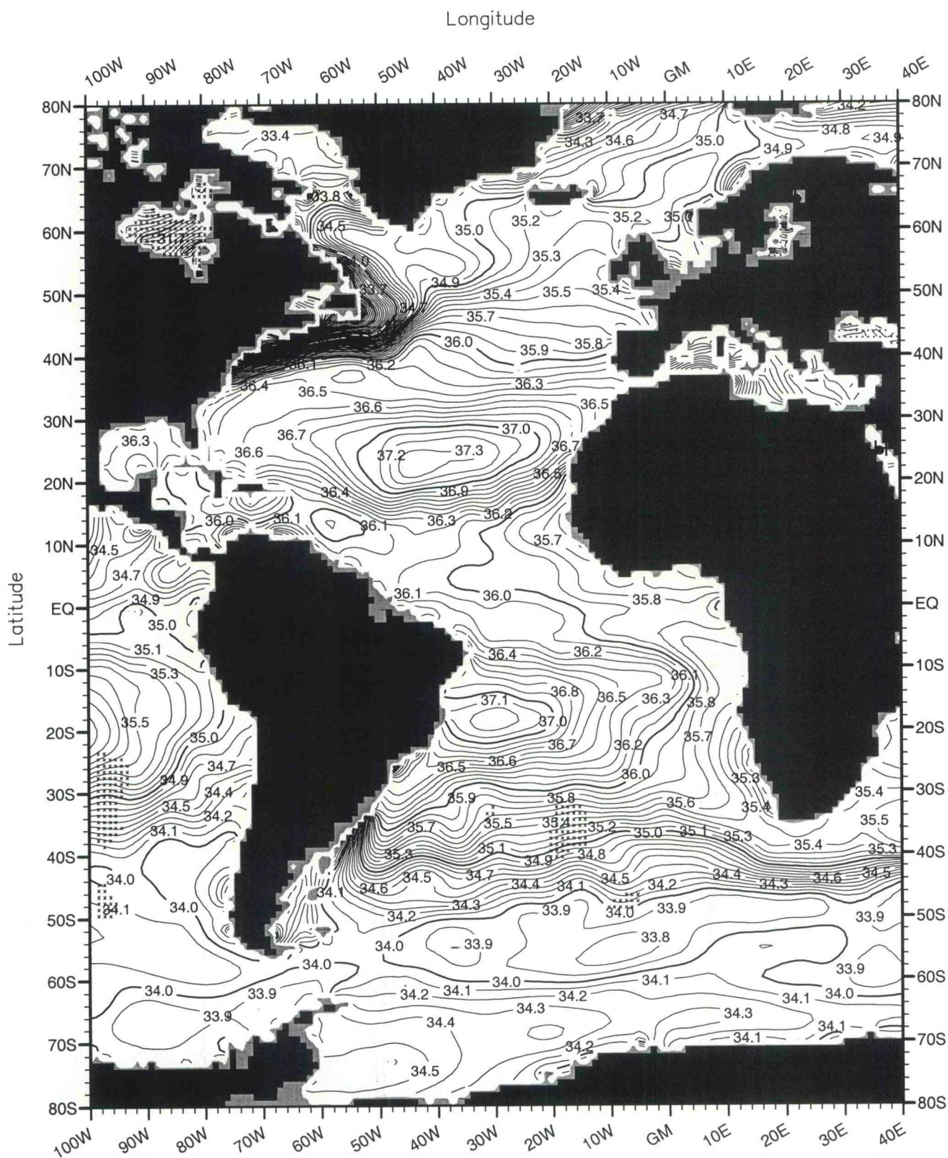
Fig. B27. Winter (Jan.-Mar.) mean salinity (PSS) at 50 m. depth .
