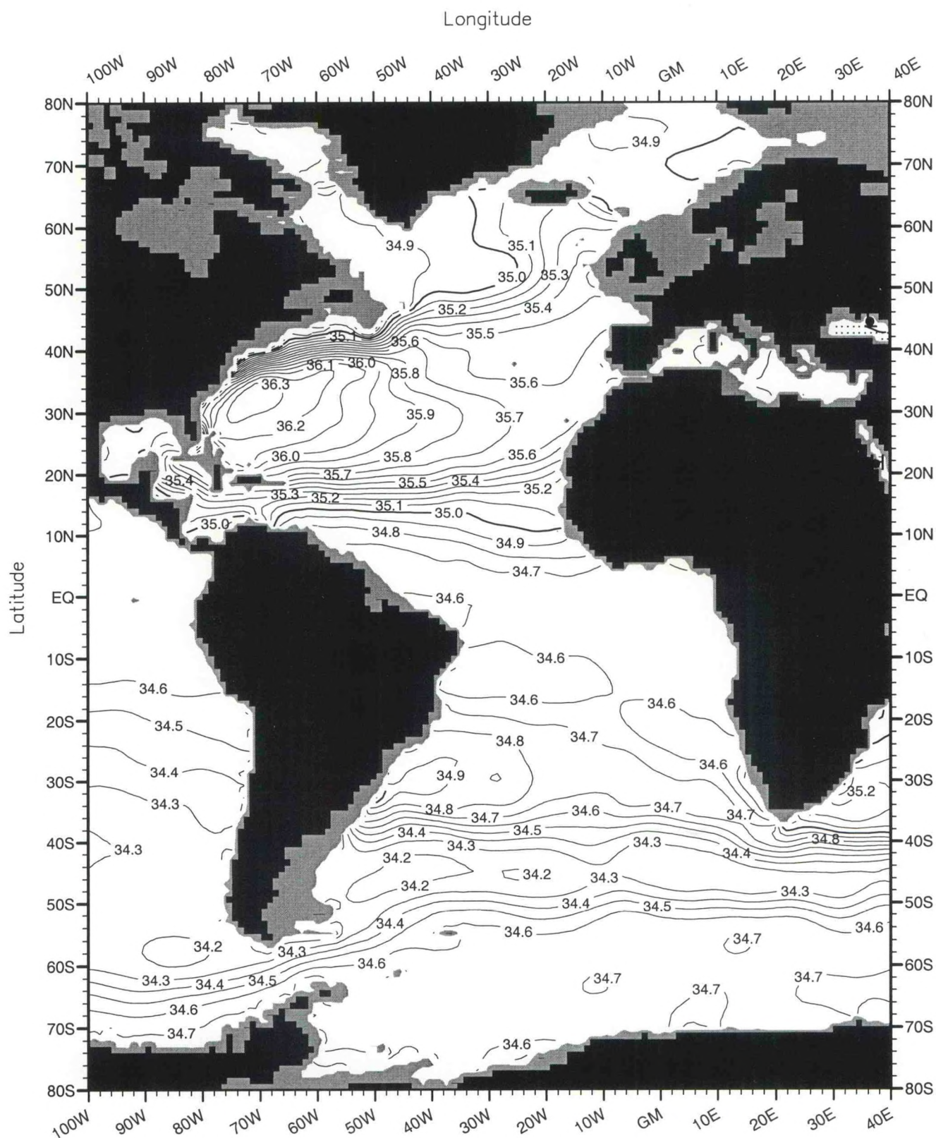
Fig. A25. Annual mean salinity (PSS) at 500 m. depth .
