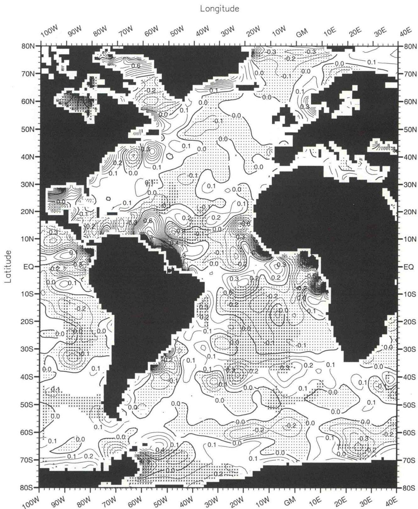
Fig. C70. December minus annual salinity (PSS) at the surface .
