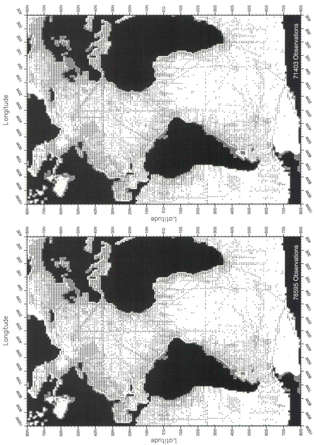
Fig. B21. Fall (Oct.-Dec.) salinity observations at 75 m. depth .
