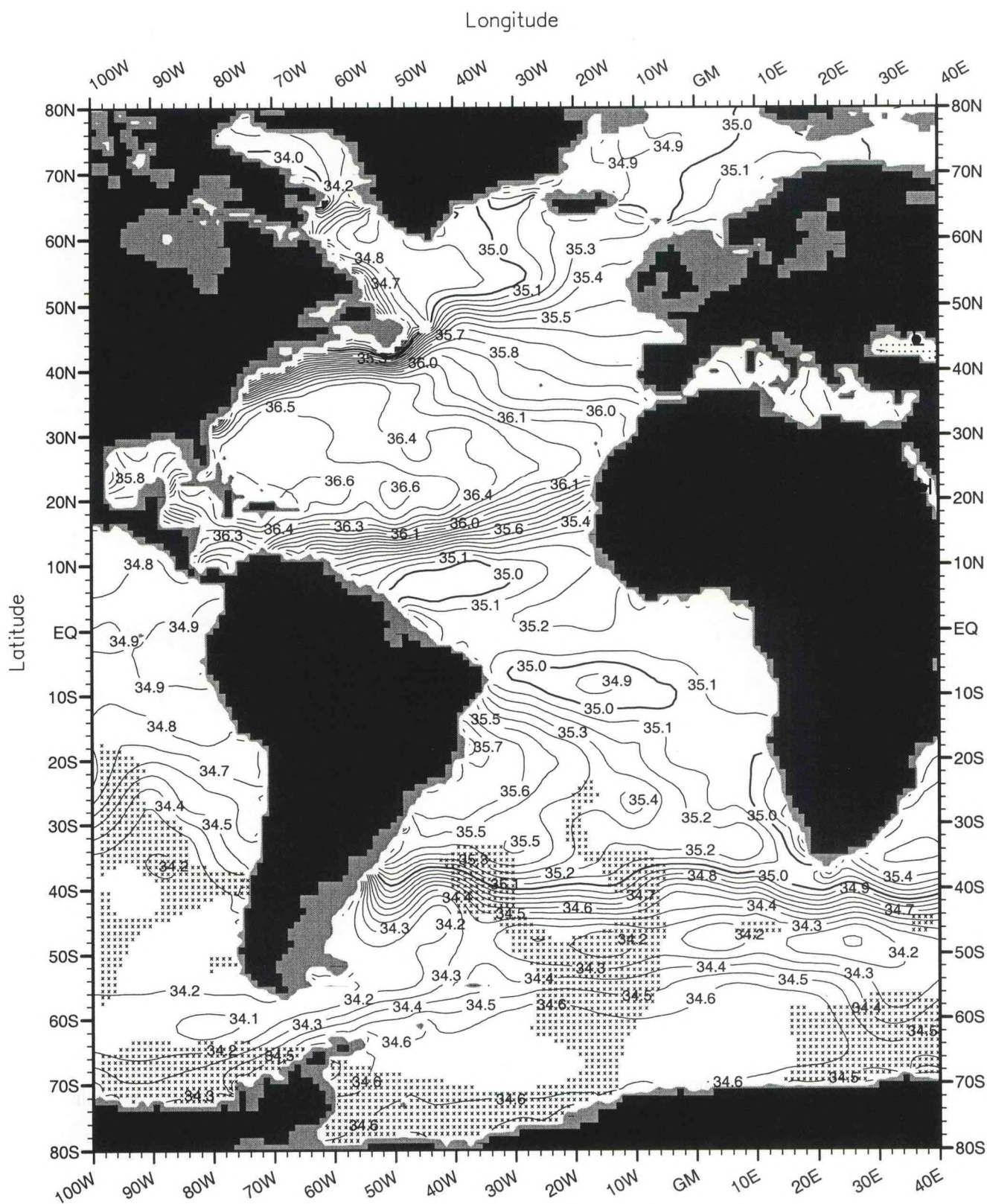
Fig. B59. Summer (Jul.-Sep.) mean salinity (PSS) at 250 m. depth .
