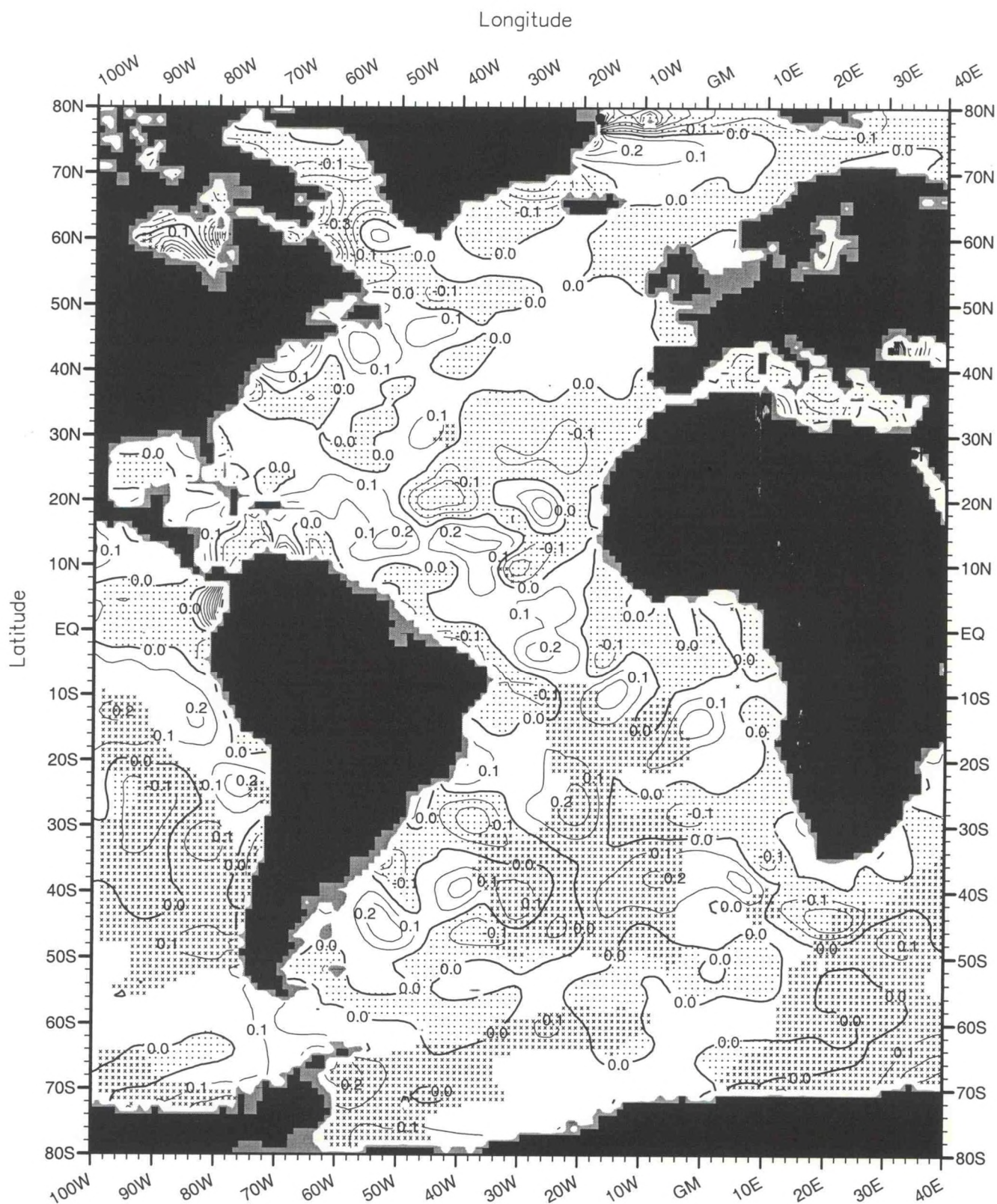
Fig. C64. October minus annual salinity (PSS) at 75 m. depth .
