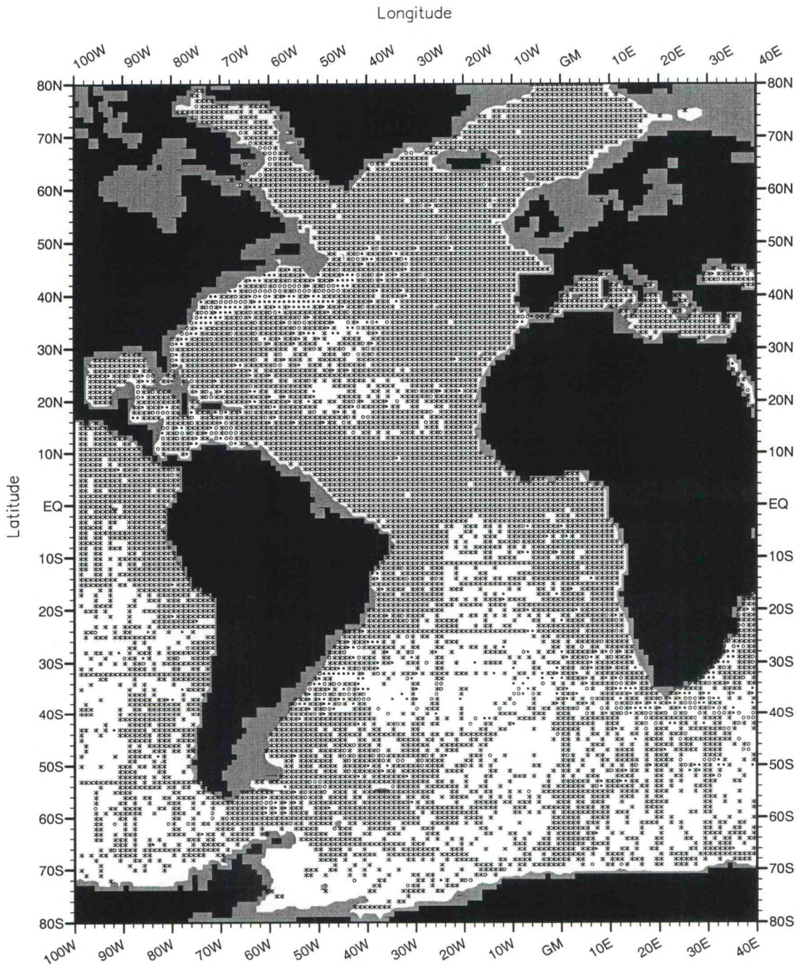
Fig. 4 Annual observed one-degree square salinity mean value minus objectively analyzed mean salinity values (PSS) at 500 meters depth.
