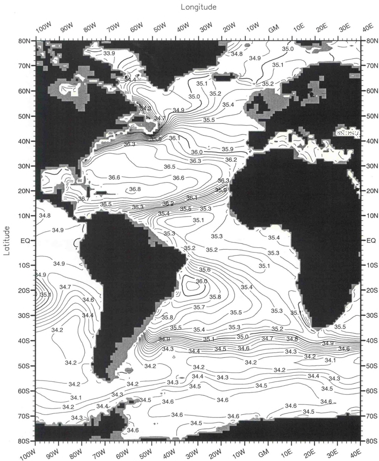
Fig. A22. Annual mean salinity (PSS) at 200 m. depth .
