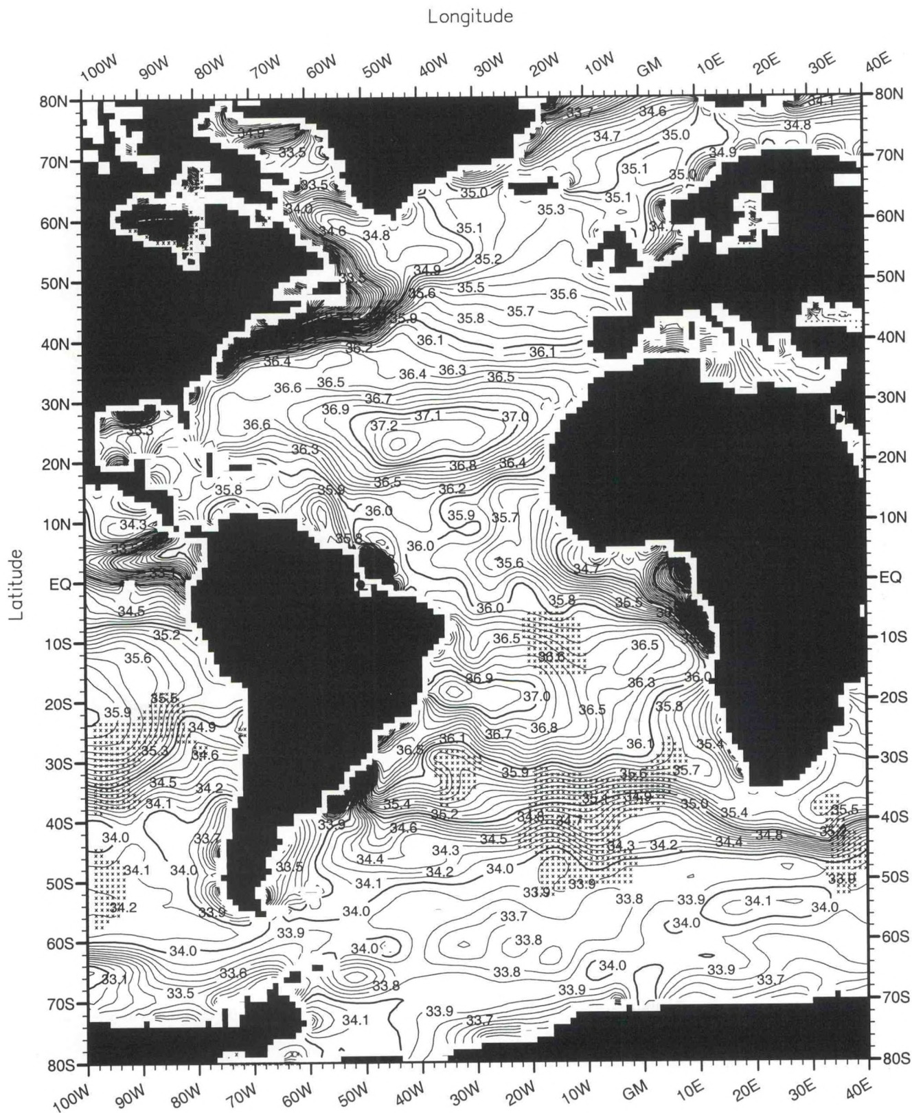
Fig. C29. February mean salinity (PSS) at the surface .
