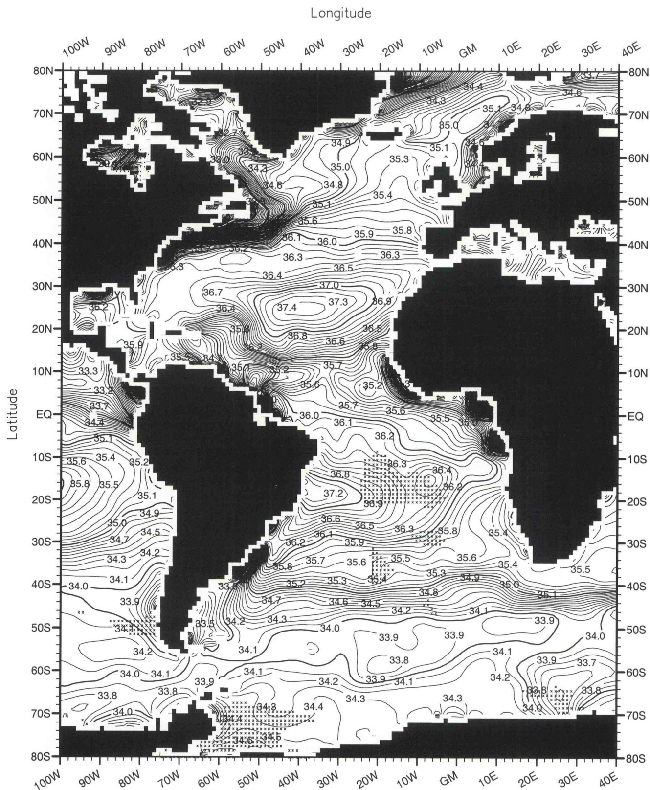
Fig. B61. Fall (Oct.-Dec.) mean salinity (PSS) at the surface .
