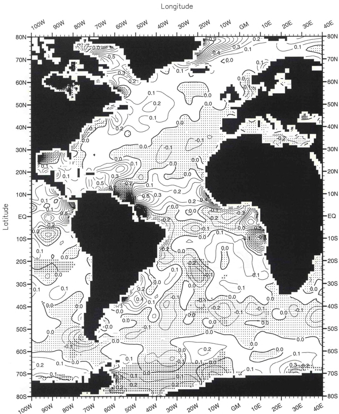
Fig. B38. Spring (Apr.-Jun.) minus annual salinity (PSS) at the surface . Minimum Value= -8.67 Maximum Value= 6.69 Contour Interval: 0.10
