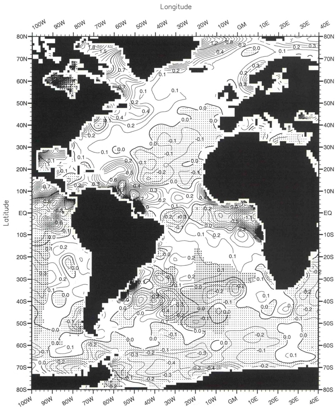
Fig. C34. March minus annual salinity (PSS) at the surface .
