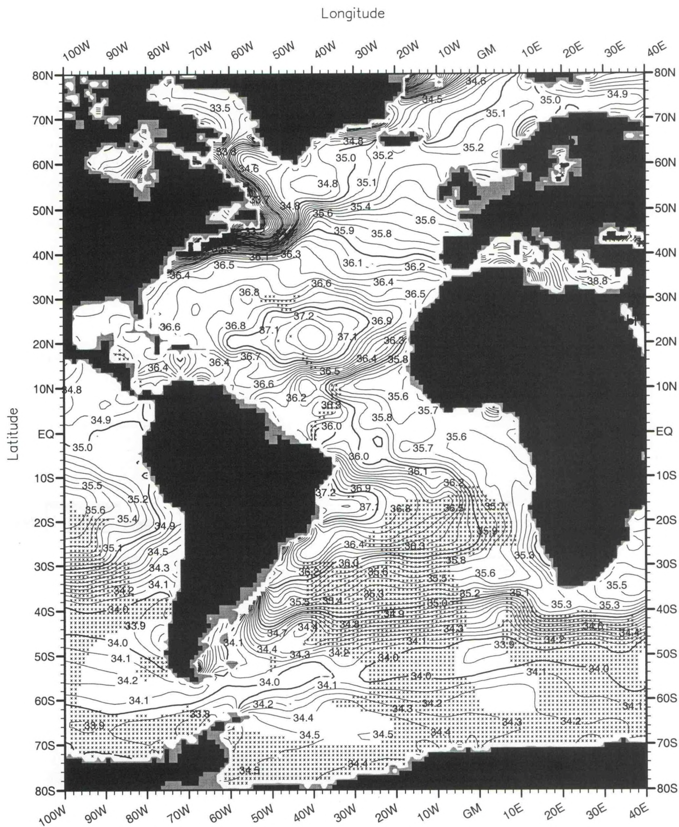
Fig. C59. September mean salinity (PSS) at 75 m. depth .
