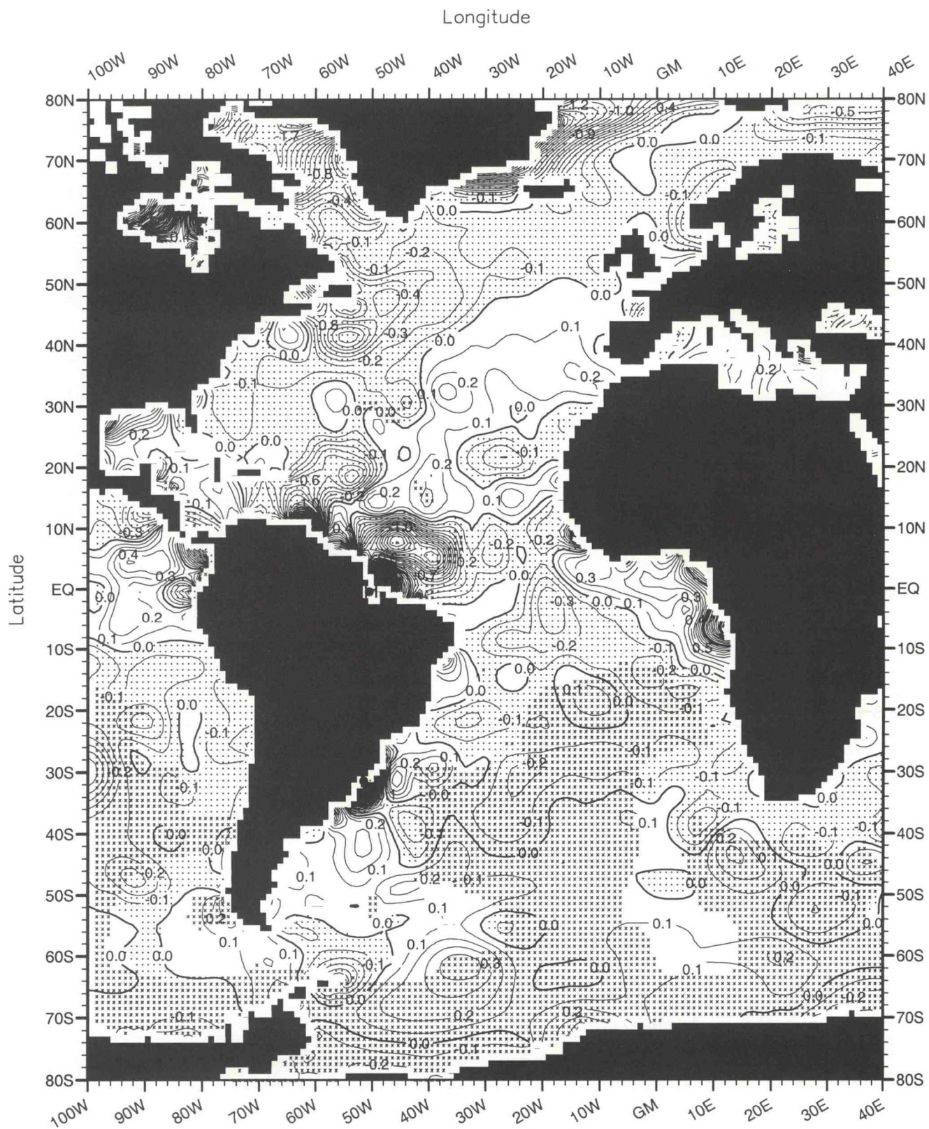
Fig. C58. September minus annual salinity (PSS) at the surface .
