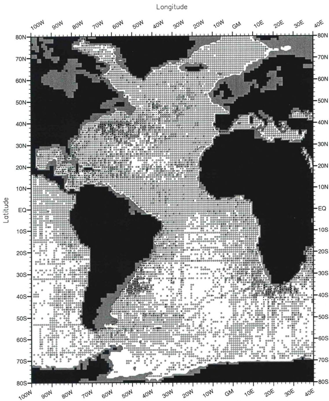
Fig. 1b Annual salinity standard error of the mean (PSS) at 500 meters depth by one-degree squares.
