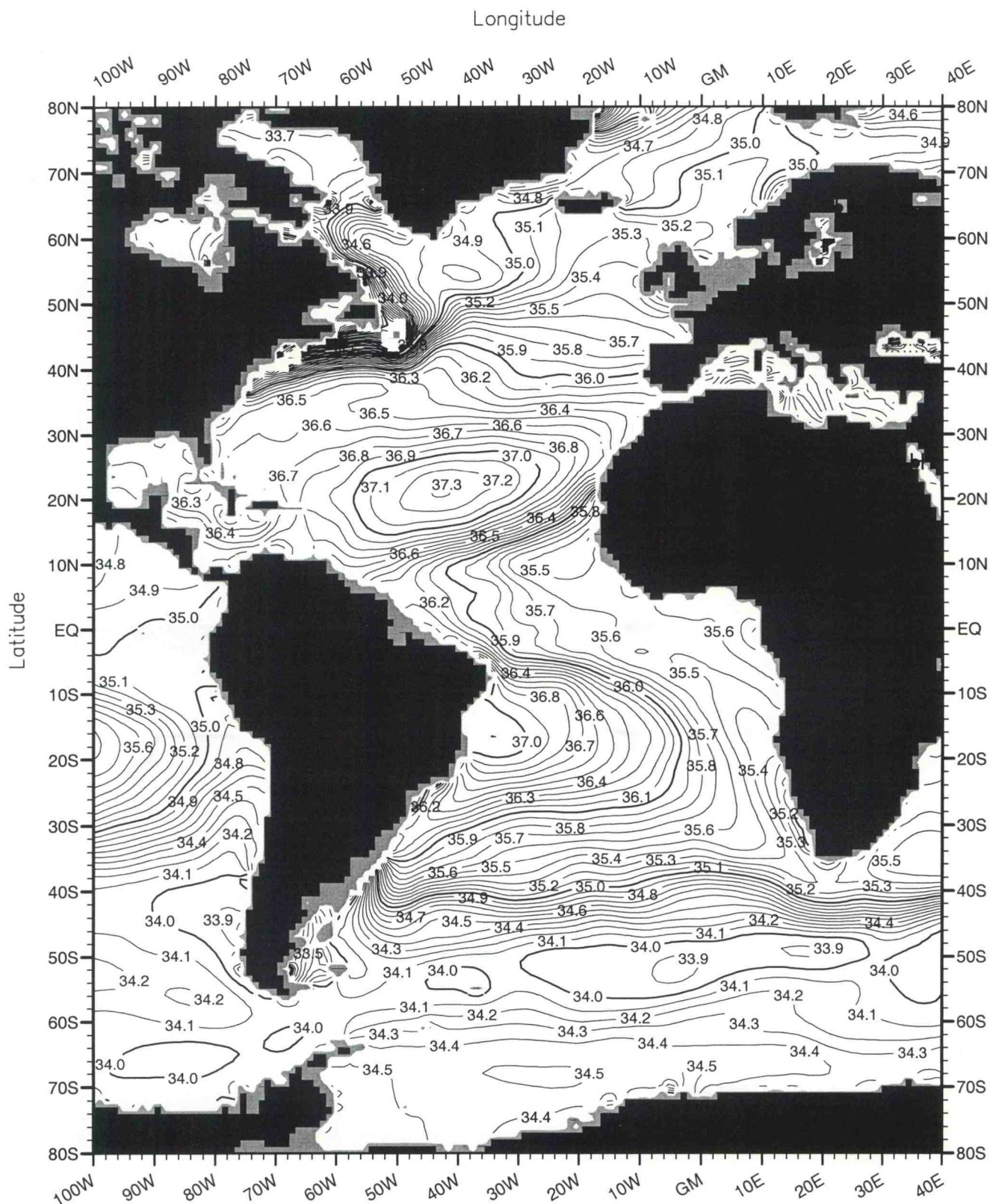
Fig. A20. Annual mean salinity (PSS) at 100 m. depth .
