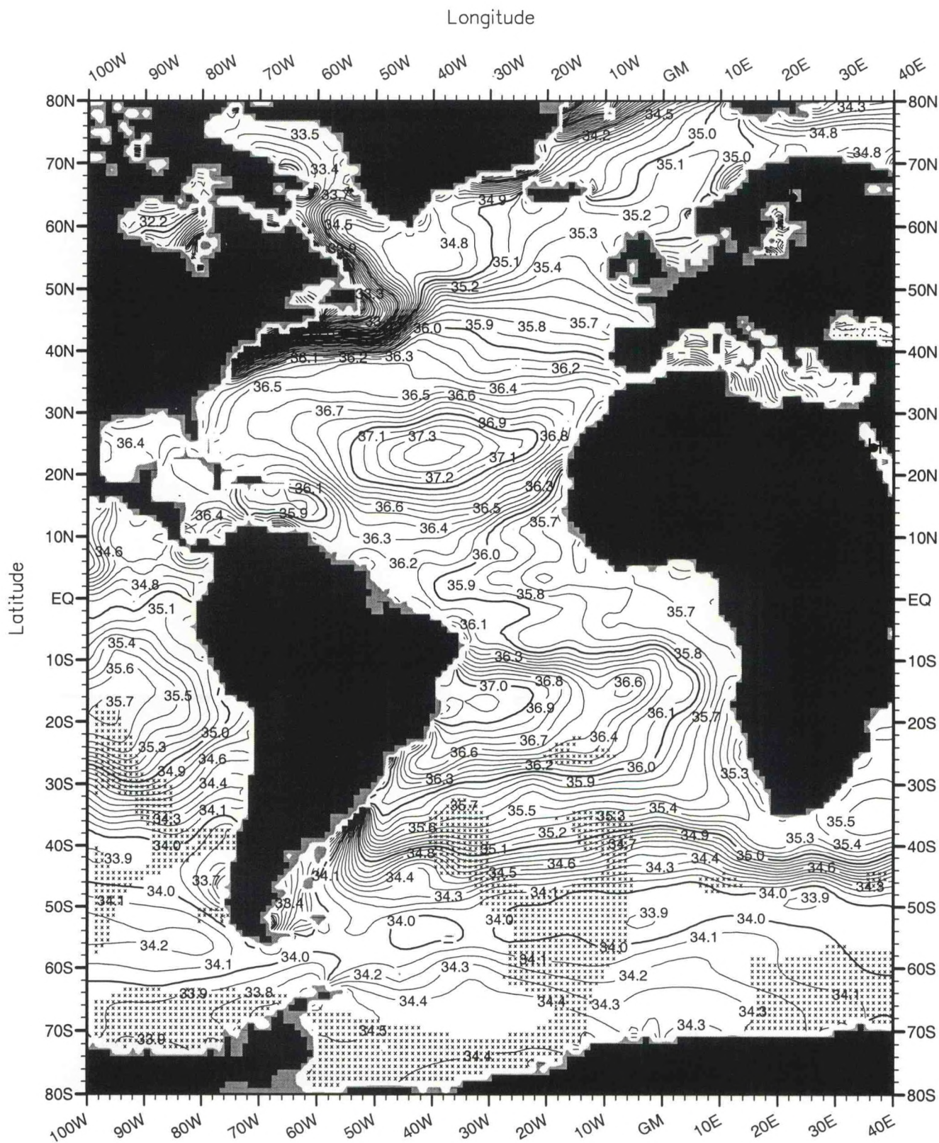
Fig. B51. Summer (Jul.-Sep.) mean salinity (PSS) at 50 m. depth .
