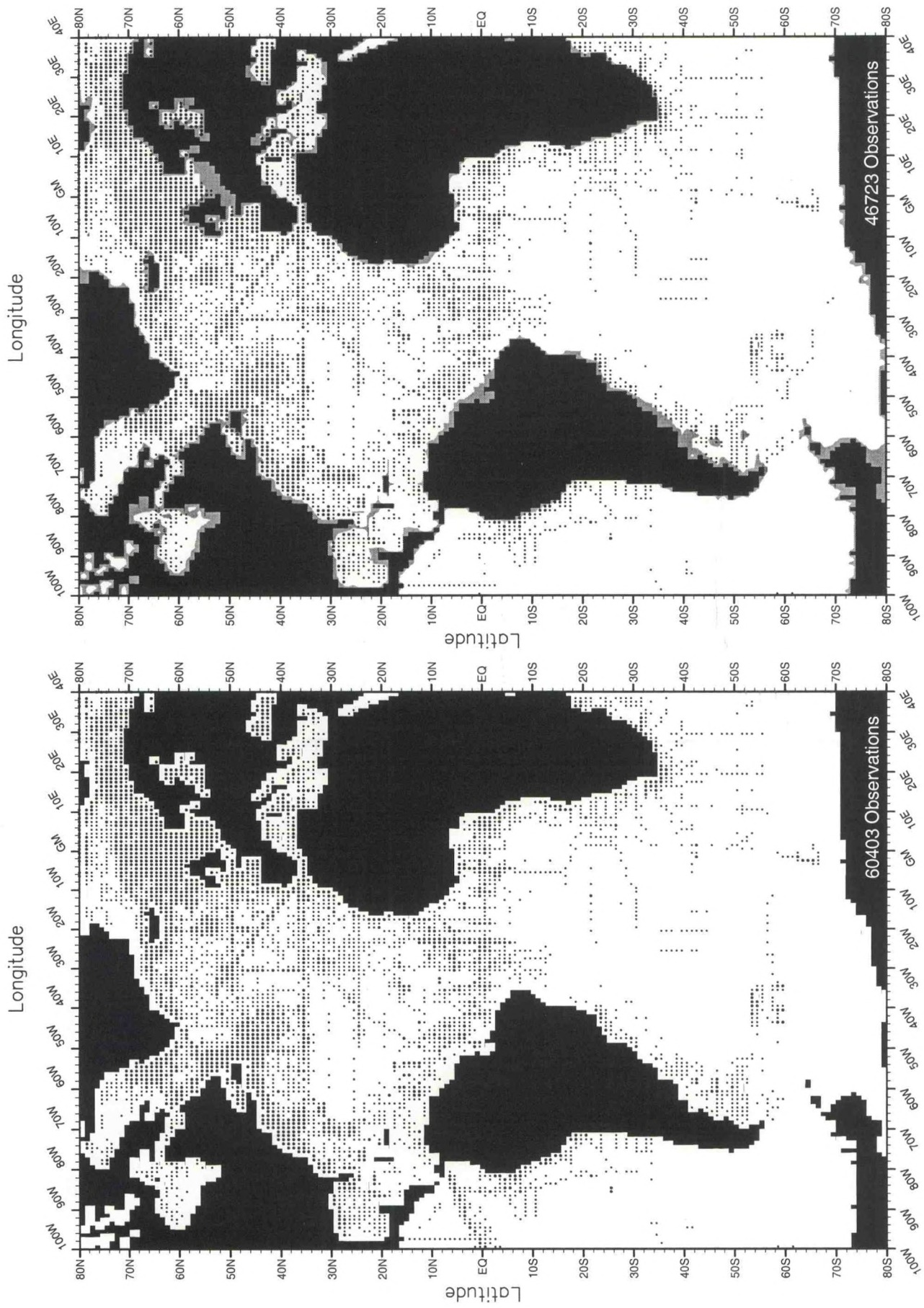
Fig. C13. July salinity observations at the surface .
