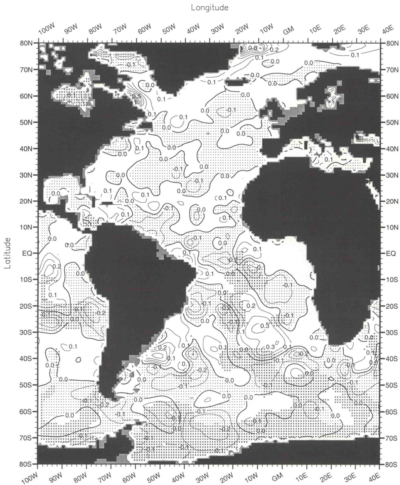
Fig. C44. May minus annual salinity (PSS) at 75 m. depth .
