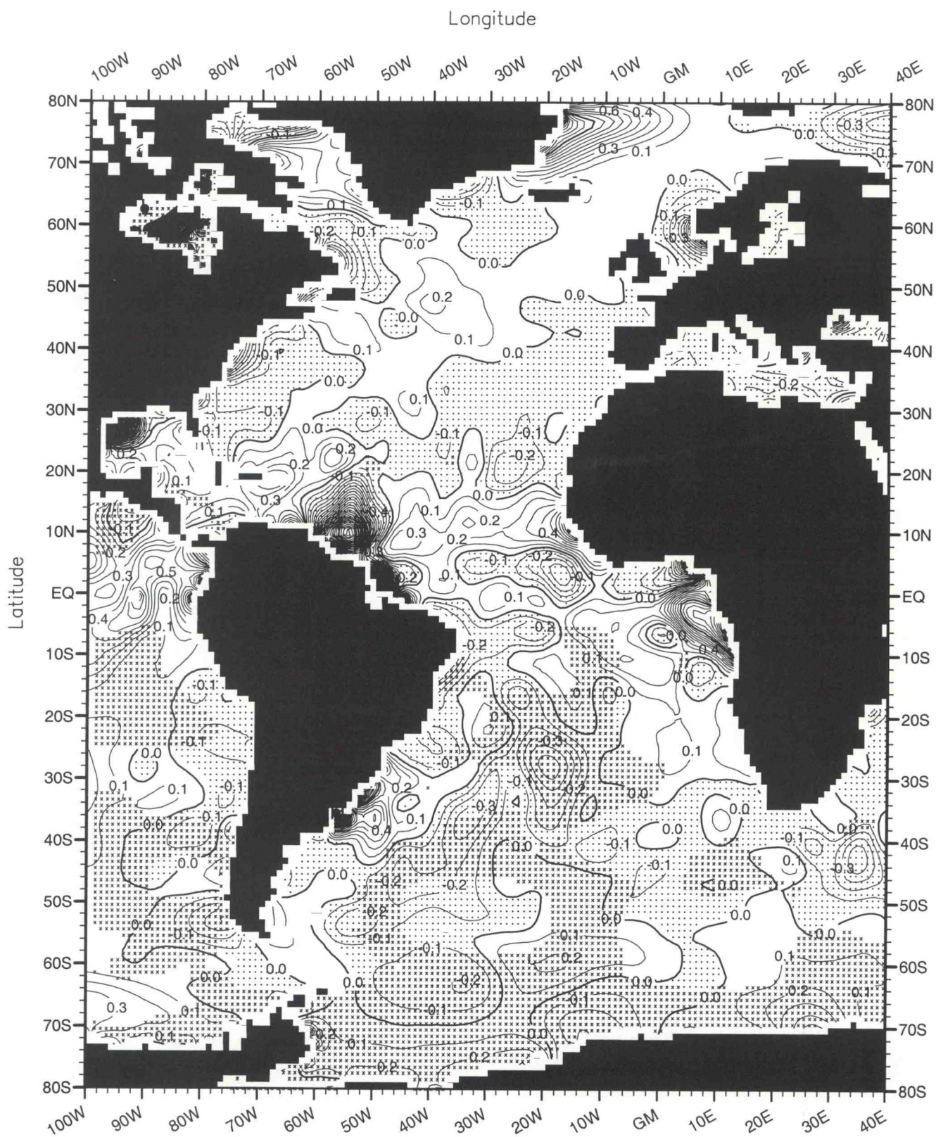
Fig. C46. June minus annual salinity (PSS) at the surface .
