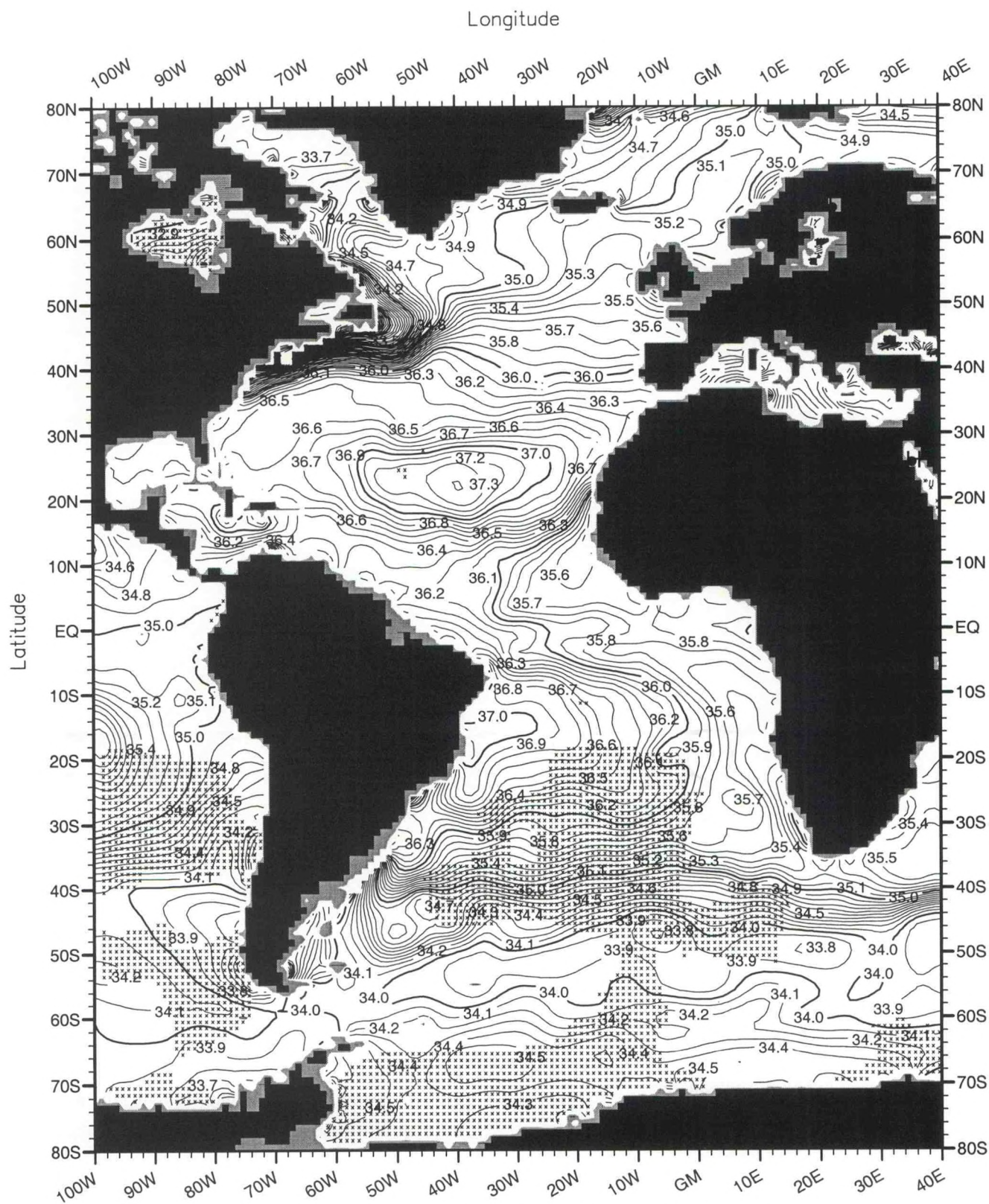
Fig. C39. April mean salinity (PSS) at 75 m. depth .
