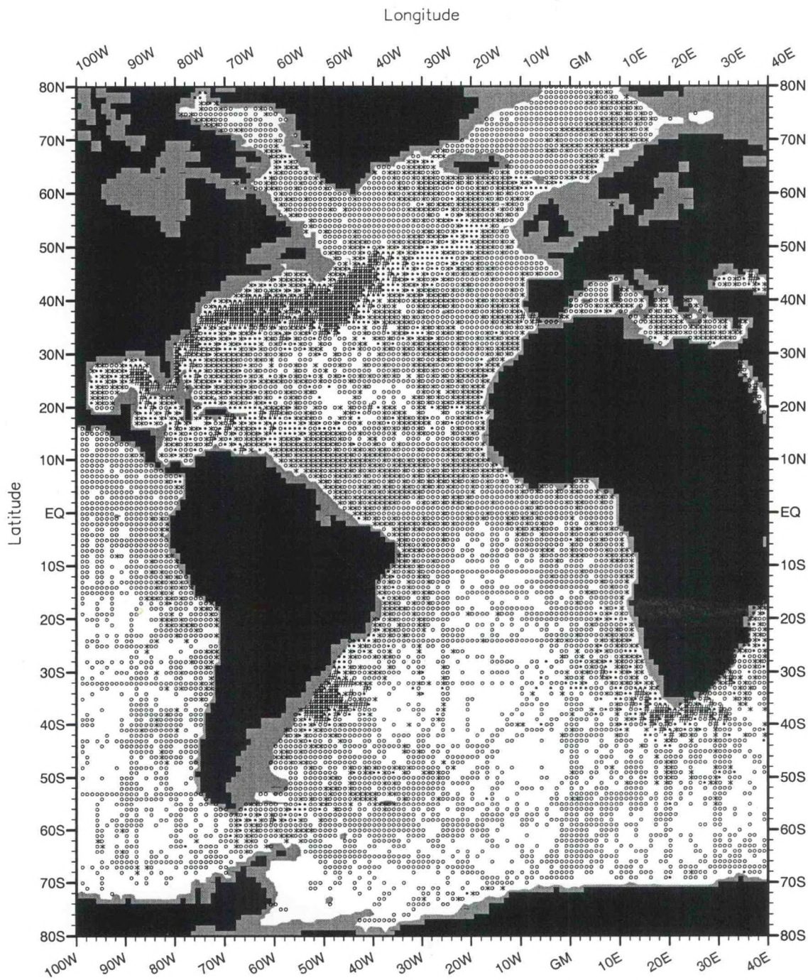
Fig. 1a Annual salinity standard deviation (PSS) at 500 meters depth by one-degree squares.
