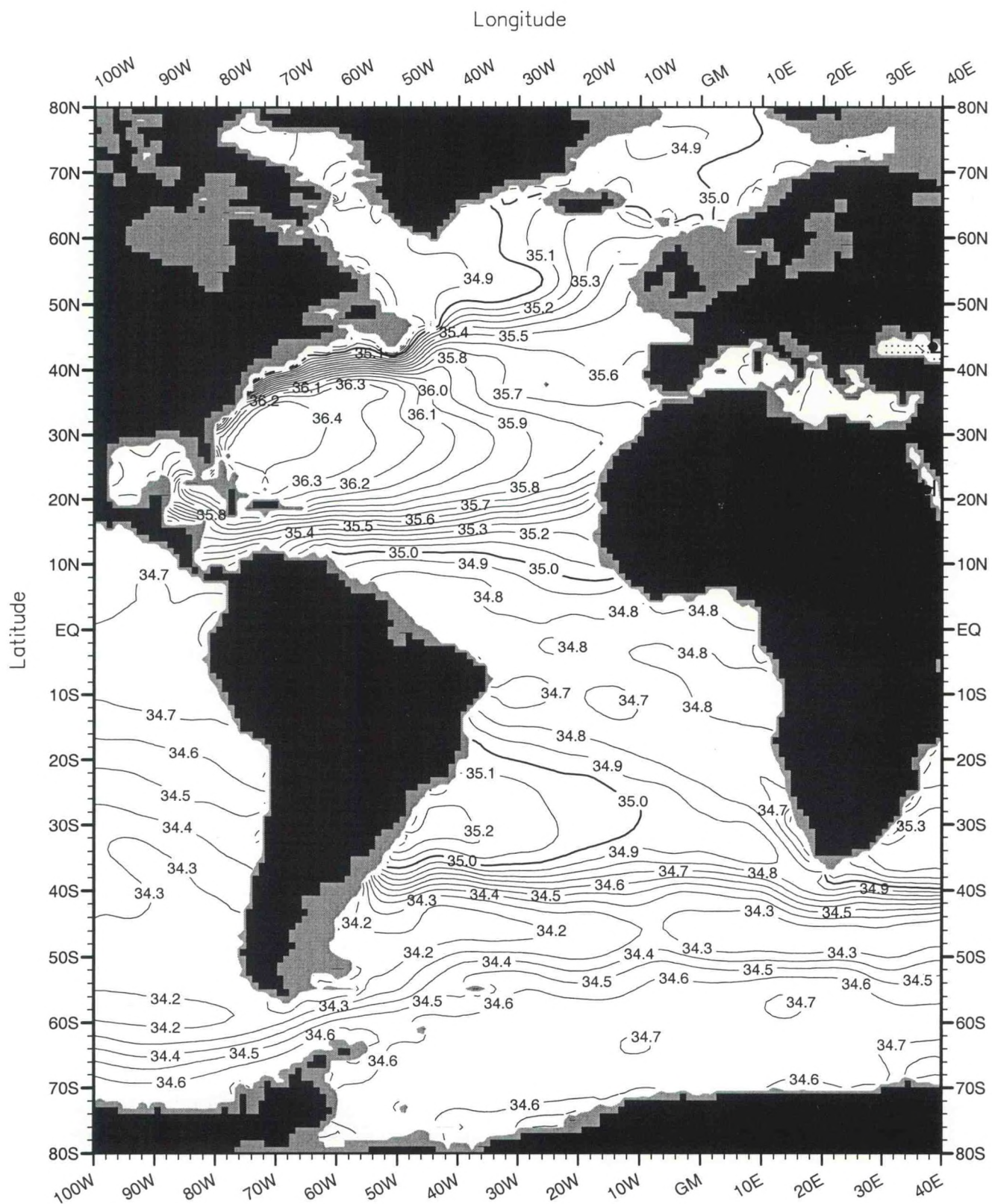
Fig. A24. Annual mean salinity (PSS) at 400 m. depth .
