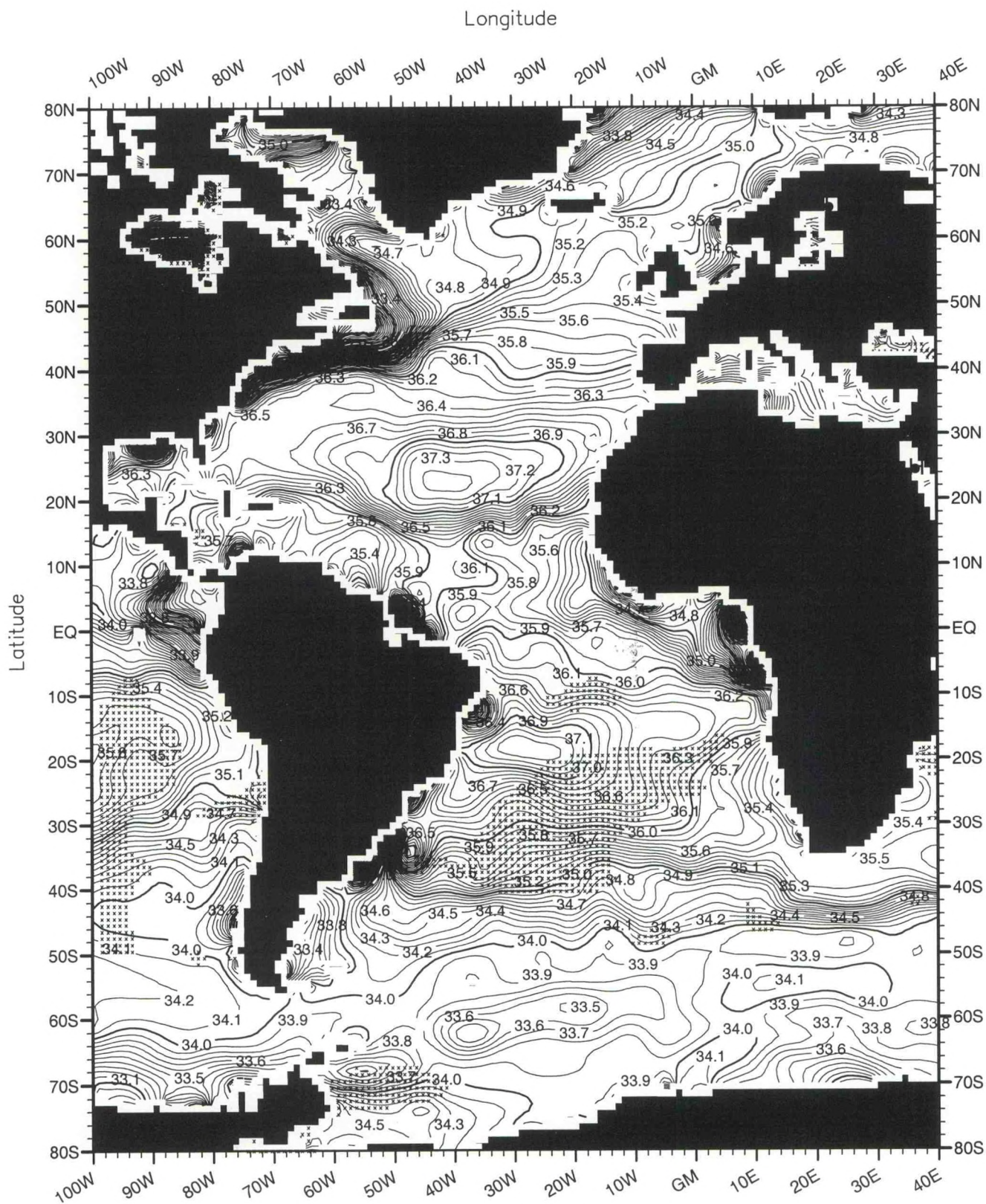
Fig. C25. January mean salinity (PSS) at the surface .
