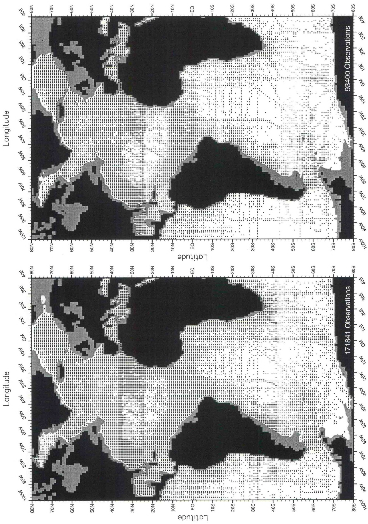
Fig. A9. Annual salinity observations at 500 m. depth .
