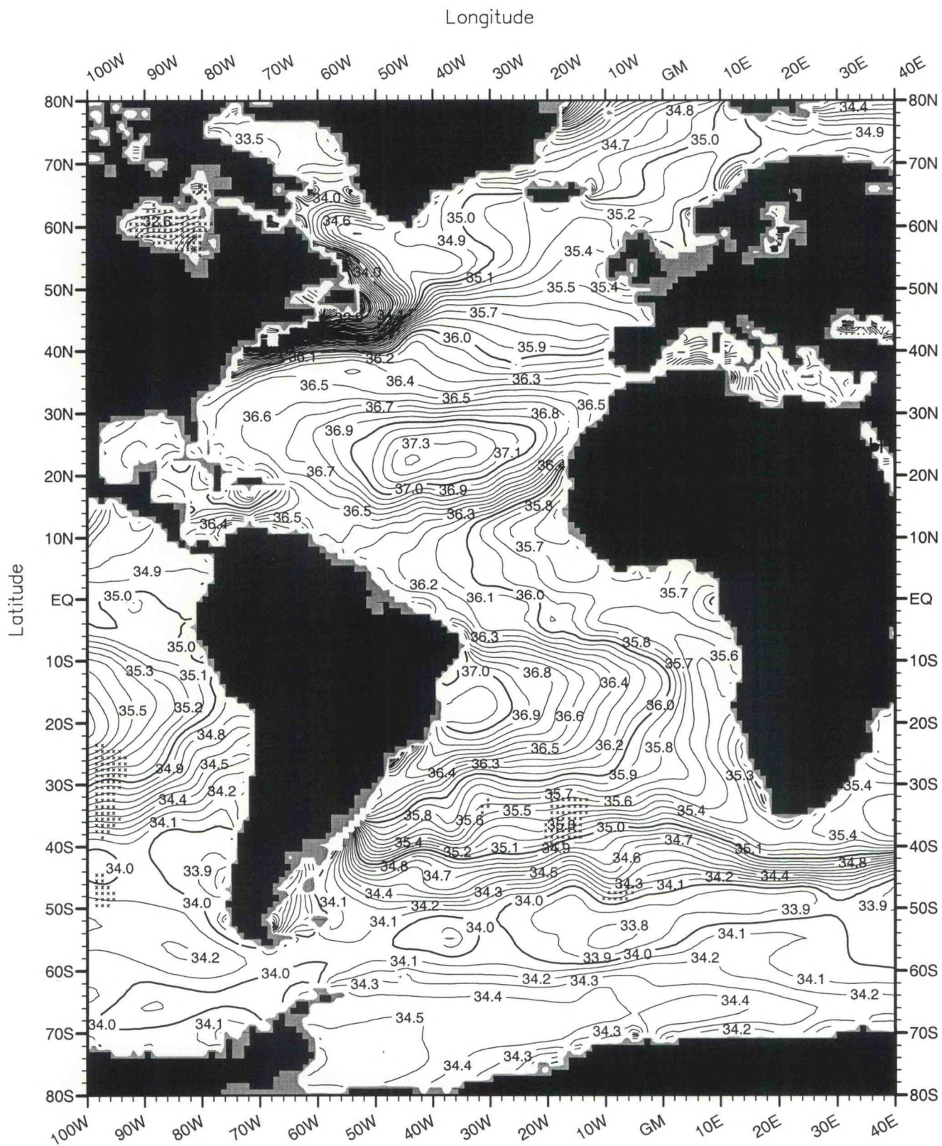
Fig. B29. Winter (Jan.-Mar.) mean salinity (PSS) at 75 m. depth . Minimum Value= 33.5 Maximum Value= 37.3 Contour Interval: 0.10
