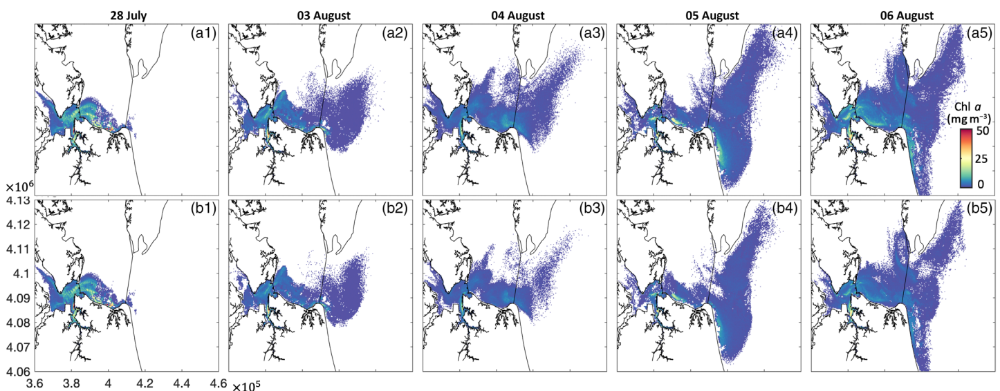
Fig. 4. Simulated Chl a concentrations (depth < 1 m) from sensitivity tests of mixotrophy and algal bloom dynamics with particles released on 28 July 2020, by disabling (a1–a5) heterotrophy and (b1–b5) all growth and biomass loss processes.
