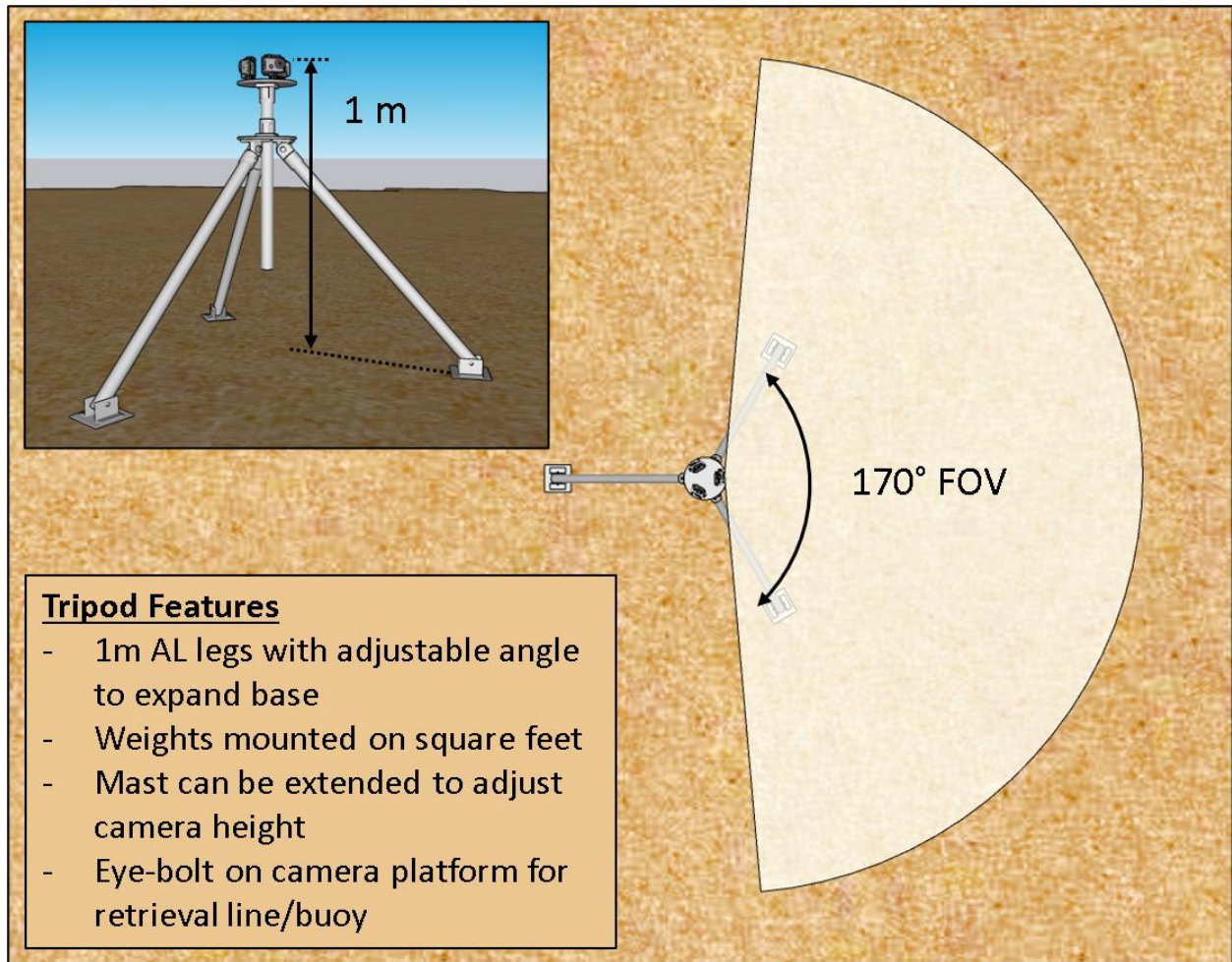
Supplementary Figure – The unbaited remote underwater video system was used to confirm the occurrence of suspected FSAs observed during hydroacoustic surveys. The frame was constructed from aluminum slip-on fencing materials (Speed-Rail®).
