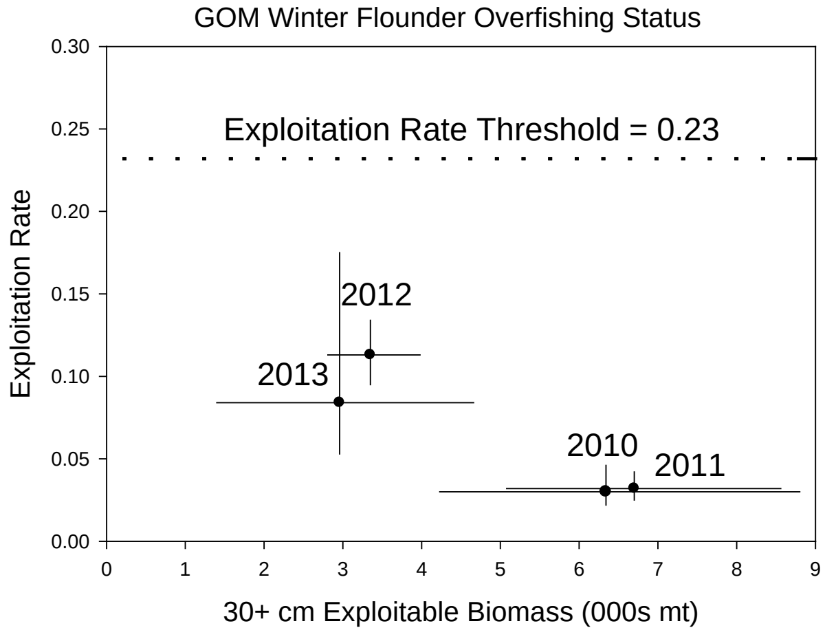
Figure B26. Stock status for Gulf of Maine (GOM) winter flounder ( Pseudopleuronectes americanus ) from 2010 through 2013 with respect to the F_{MSY} proxy. 80% confidence intervals are shown for biomass and exploitation rate from 2010 and 2013. F_{40\%} = 0.31 , which corresponds to an exploitation rate of 0.23.
