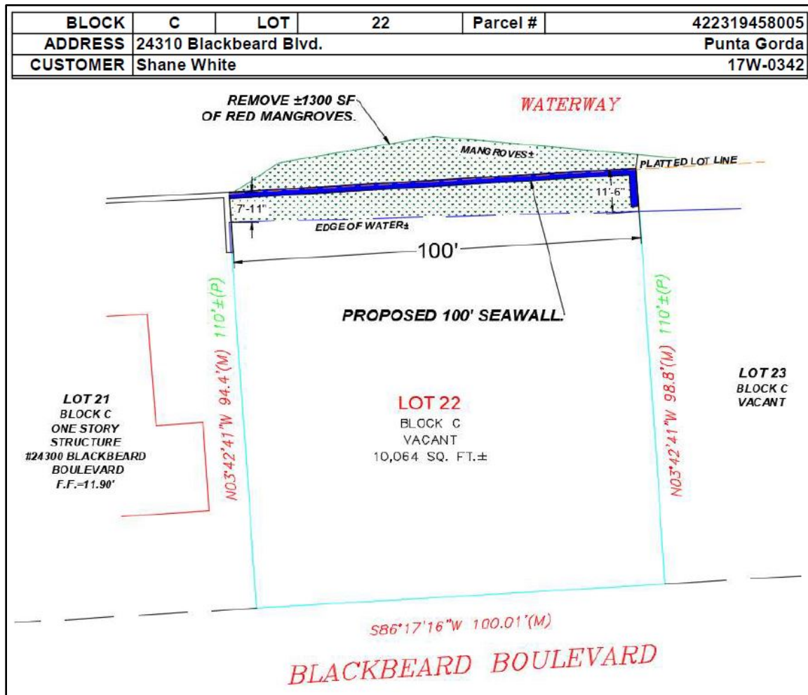
Figure 1. Plans for the proposed action, showing the location of the new 100-lin ft concrete seawall (Image provided by USACE).
