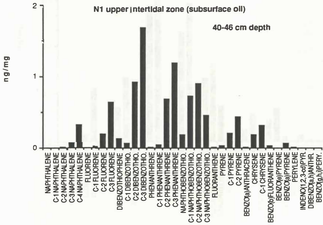
Figure I-31. Comparison of Exxon Valdez cargo oil to subsurface oil at NOAA study station N-1 upper intertidal zone (May 1990). Note the difference in scale of concentration between the plots.
