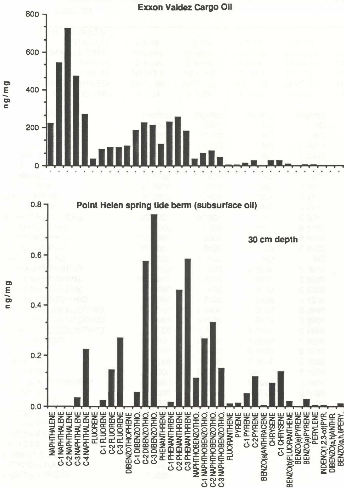
Figure I-32. Comparison of Exxon Valdez cargo oil to subsurface oil in the spring tidal berm at Point Helen (May 1990). Note the differences in scale of concentration between the two plots.
