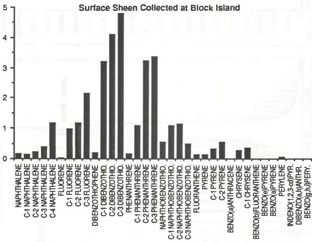
Figure II-8. Comparison of the analysis profiles of Exxon Valdez cargo oil and a sheen collected at Block Island (May 1990).
