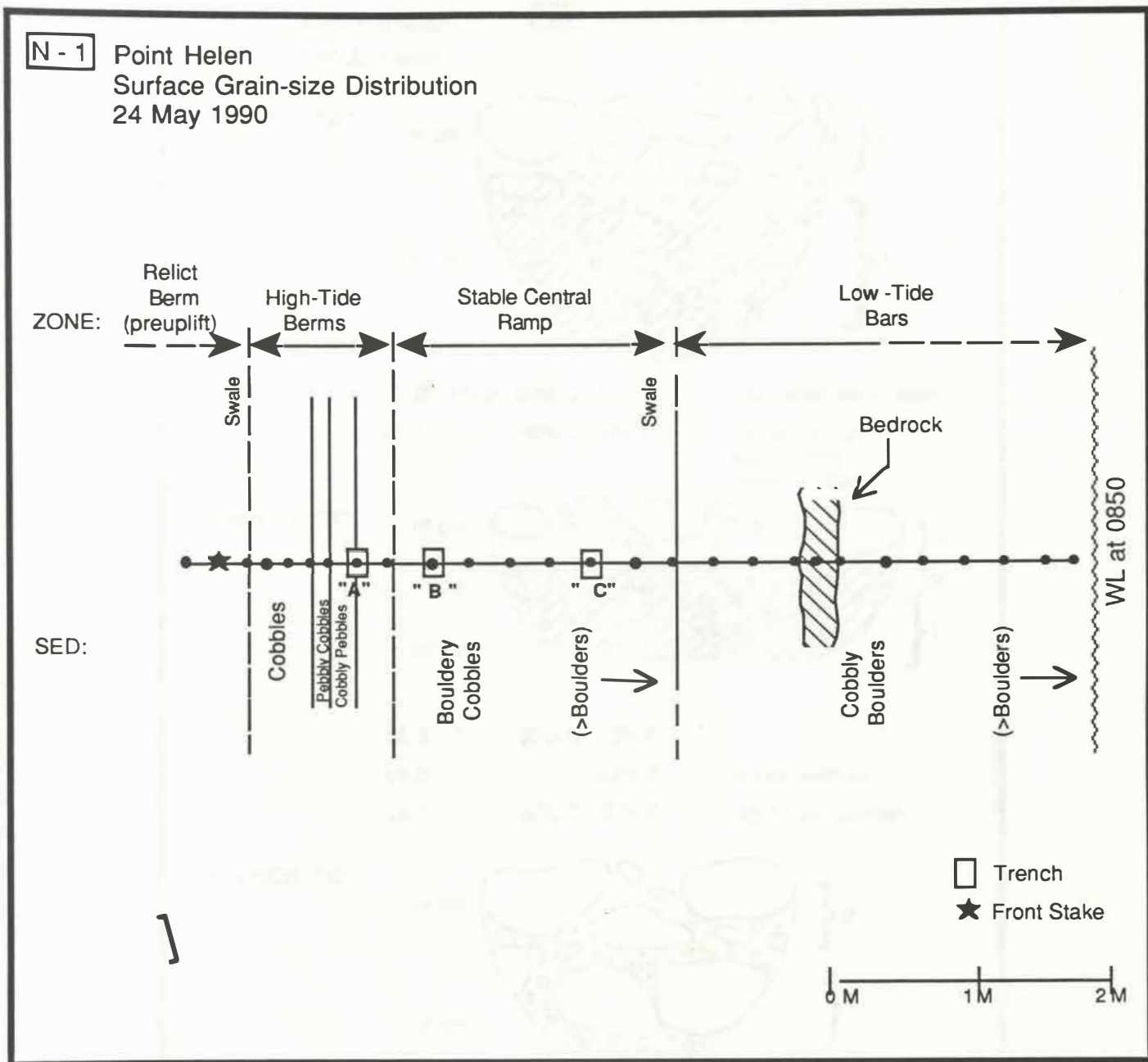
Figure I-7. Distribution of grain size of surface sediments adjacent to NOAA's profile N-1 on 24 May 1990. Dots along profile line indicate points where grain size estimates were made.
