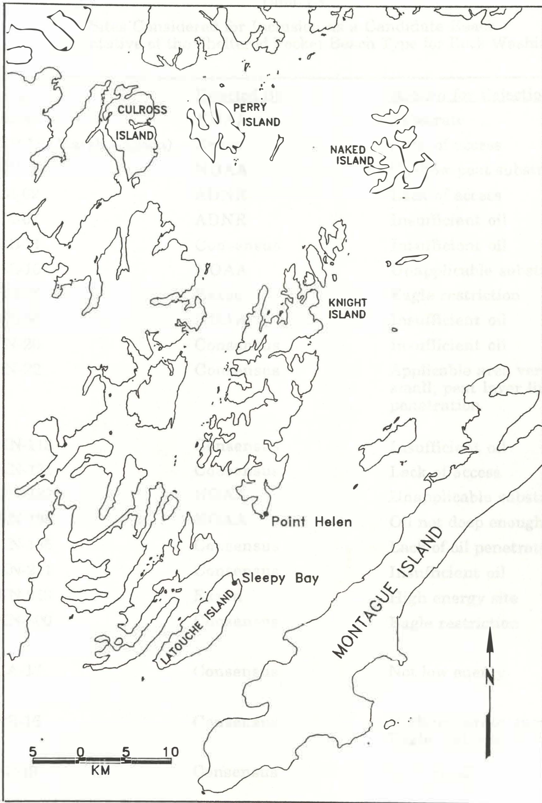
Figure I-3. Location map showing the two candidate beaches at Sleepy Bay and Point Helen.
