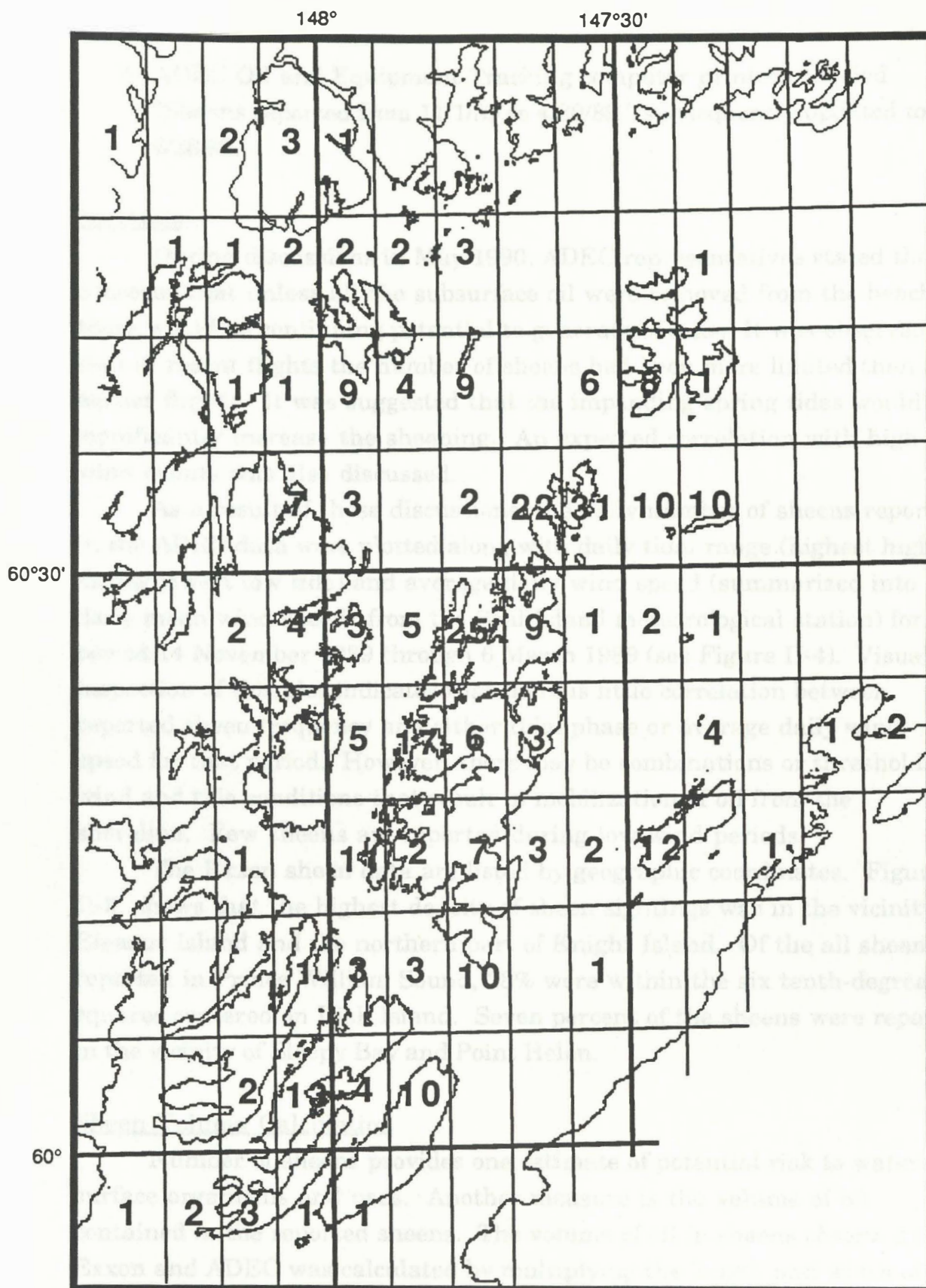
Figure II-3. Sheen sightings reported in 1990 by Exxon crews, through 2 June.
