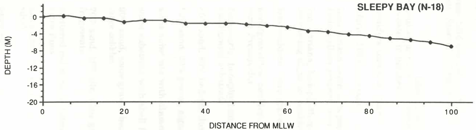
Figure II-12. Subtidal profiles off NOAA stations N-1 (upper) and N-18 (lower) in June 1990.
