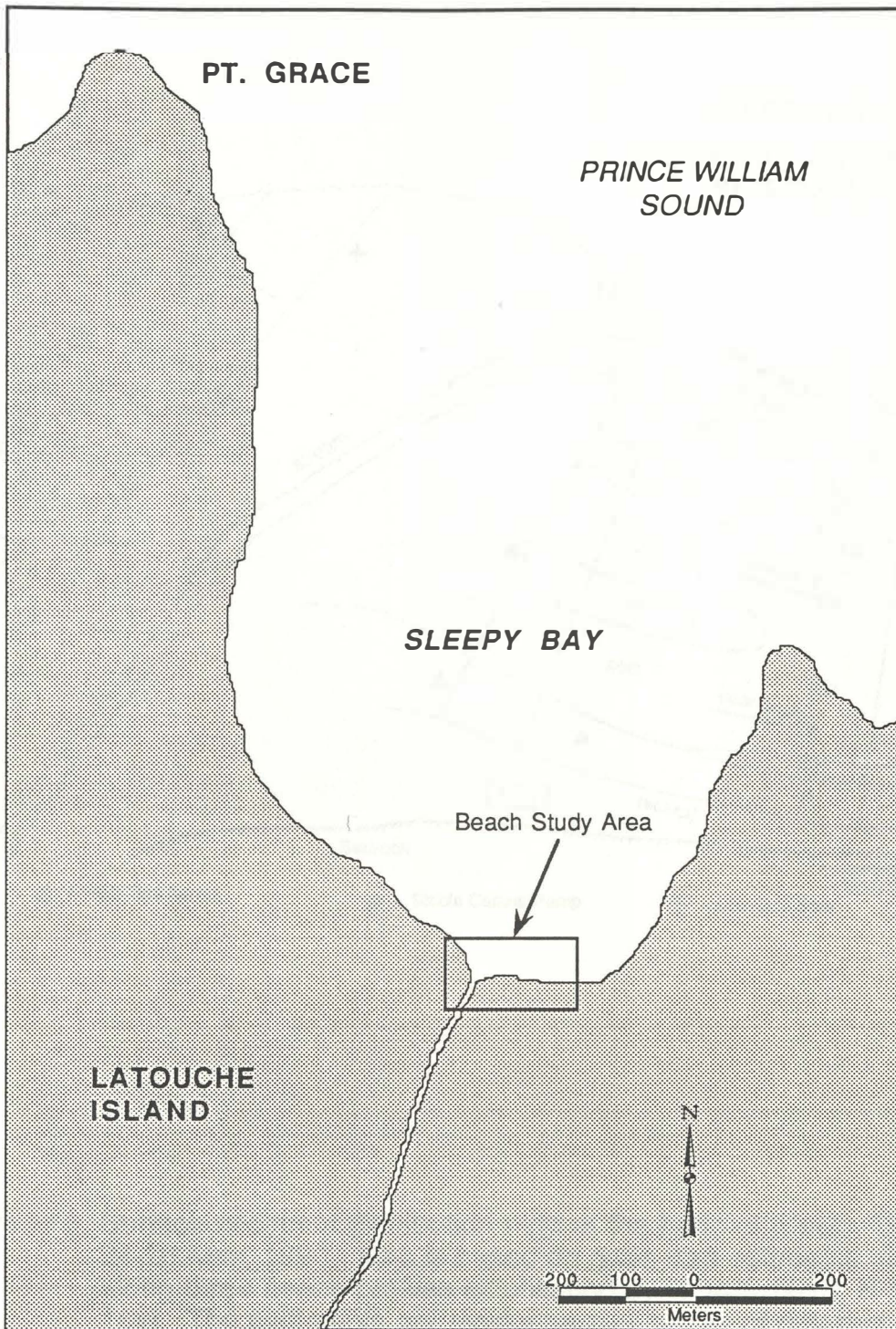
Figure I-12. Map of Sleepy Bay showing the location of the specific section of Sleepy Bay used as a candidate beach for this analysis.
