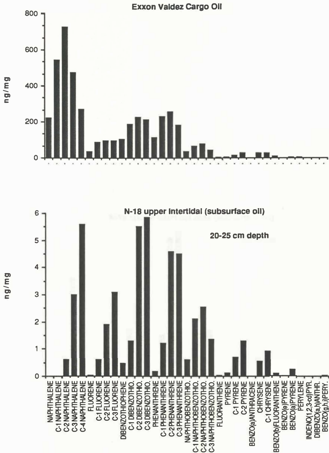
Figure I-28. Comparison of Exxon Valdez cargo oil to subsurface oil of the upper intertidal zone at NOAA study station N-18 (May 1990). Note the difference in scale of concentration between the two plots.
