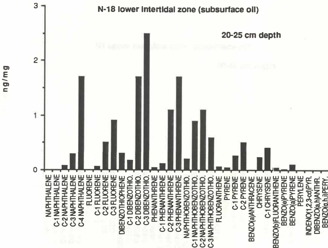
Figure I-30. Comparison of Exxon Valdez cargo oil to subsurface oil of the lower intertidal zone at NOAA study station N-18 (May 1990). Note the difference in scale of concentration between the two plots.
