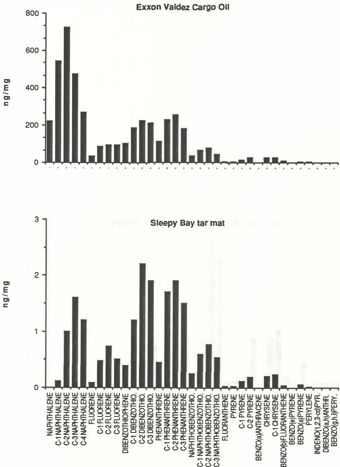
Figure I-25. Comparison of Exxon Valdez cargo oil to oil contained within a tar mat at Sleepy Bay. Note the difference in scale of concentration between the two plots.
