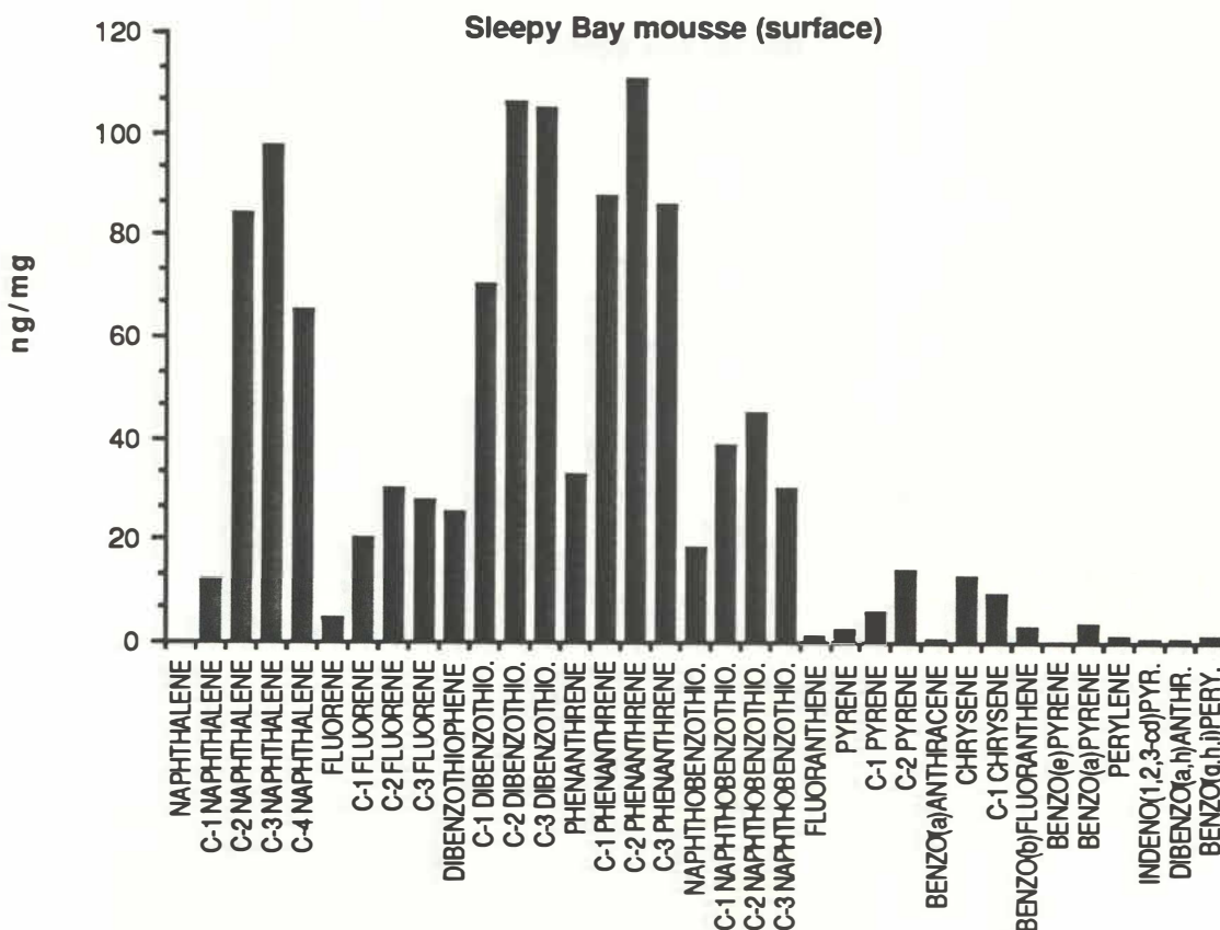
Figure I-24. Comparison of Exxon Valdez cargo oil to mousse collected at Sleepy Bay (May 1990). Note the difference in scale of concentration between the two plots.
