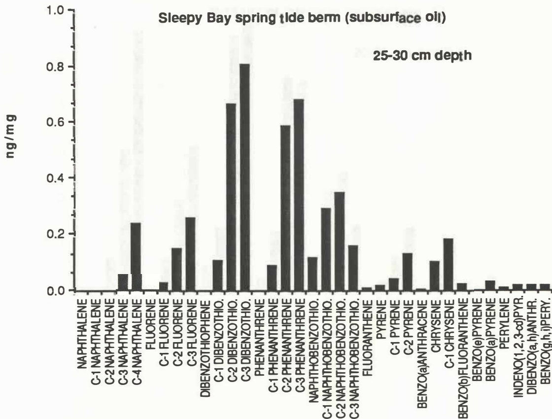
Figure I-27. Comparison of Exxon Valdez cargo oil to subsurface oil buried in the spring tide berm at Sleepy Bay (May 1990). Note the difference in scale of concentration between the two plots.
