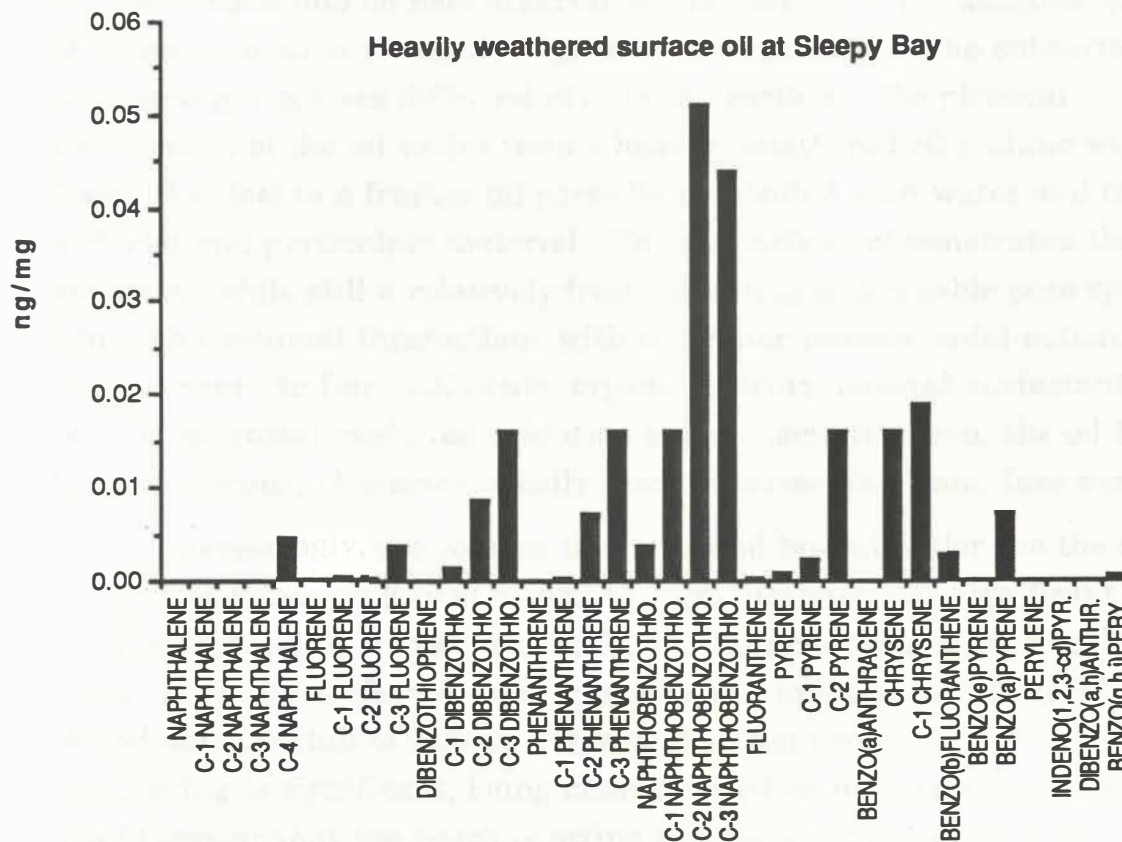
Figure I-26. Comparison of Exxon Valdez cargo oil to a surface sample from Sleepy Bay that is heavily weathered. Note the difference in scale of concentration between the two plots.
