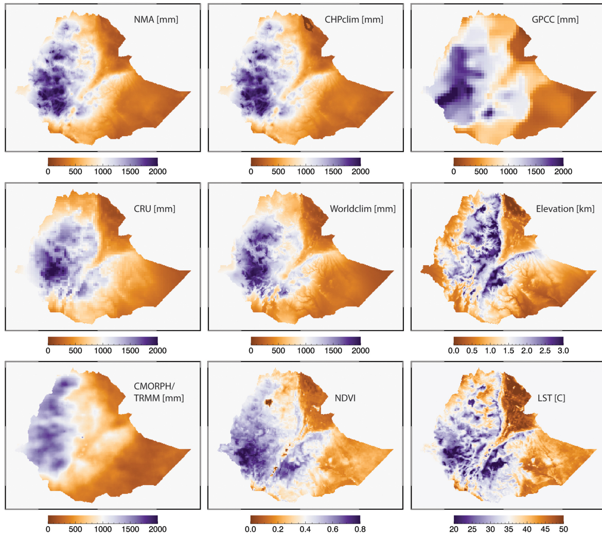
Figure 10. Total annual rainfall, elevation, NDVI and LST for Ethiopia. Rainfall totals are from the Ethiopian National Meteorological Agency (NMA), CHPclim, the GPCCC M V2015 climatology, the CRU CL v2.0, the version 1.4 release 3 Worldclim climatology, and the blended CMORPH/TRMM data used in the CHPclim modeling process.
