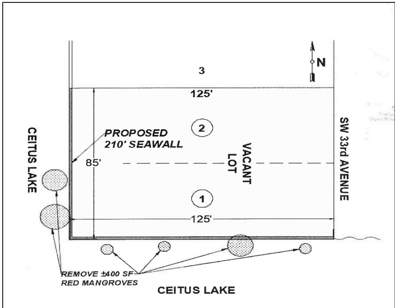
Figure 3. Project drawing showing the 2 perpendicular seawalls proposed and the approximate location of the existing red mangroves (© 2017 Honc Marine Construction, Inc.)
