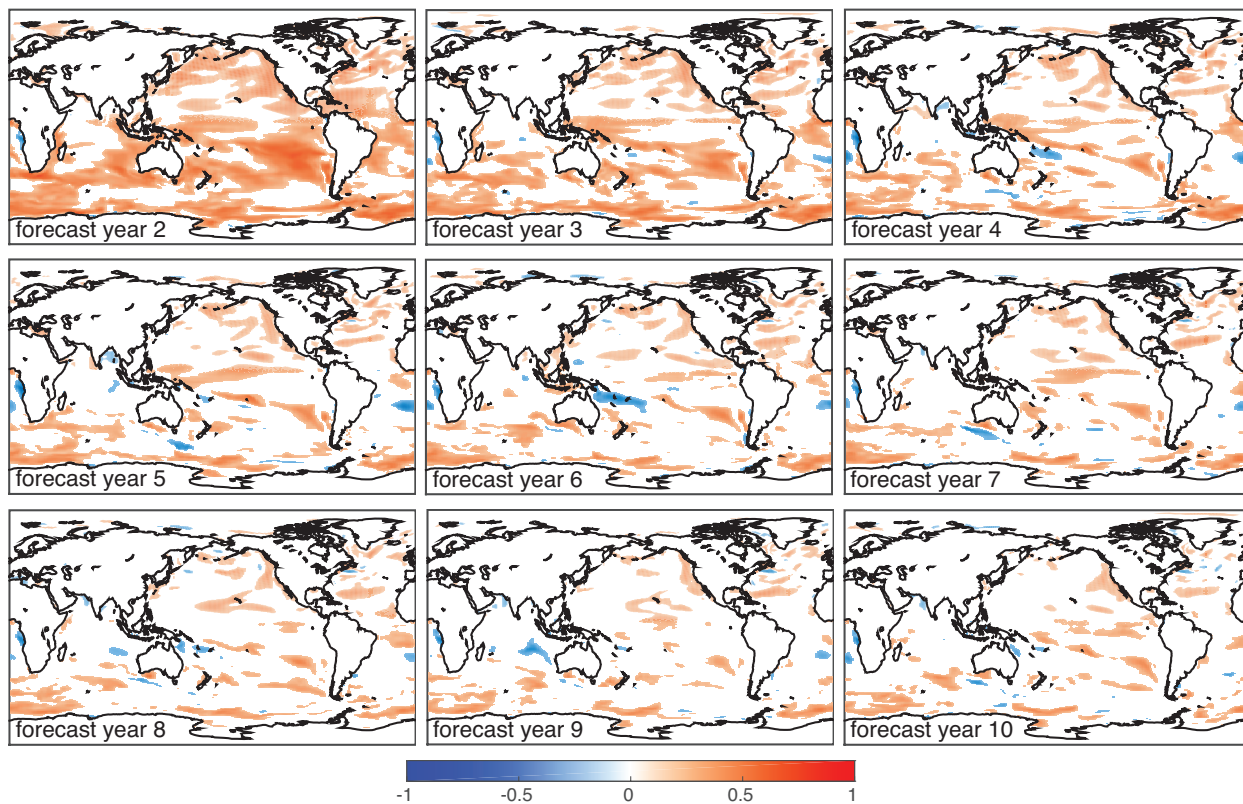
Figure S1. Predictability of air-sea CO 2 flux, as indicated by the correlation coefficient of detrended, air-sea CO 2 flux anomalies from the CESM-DPLE initialized forecast for a range of lead years with the reconstruction. Correlation coefficients that are not statistically significant at the 95% level using a t test are assigned a value of zero.
