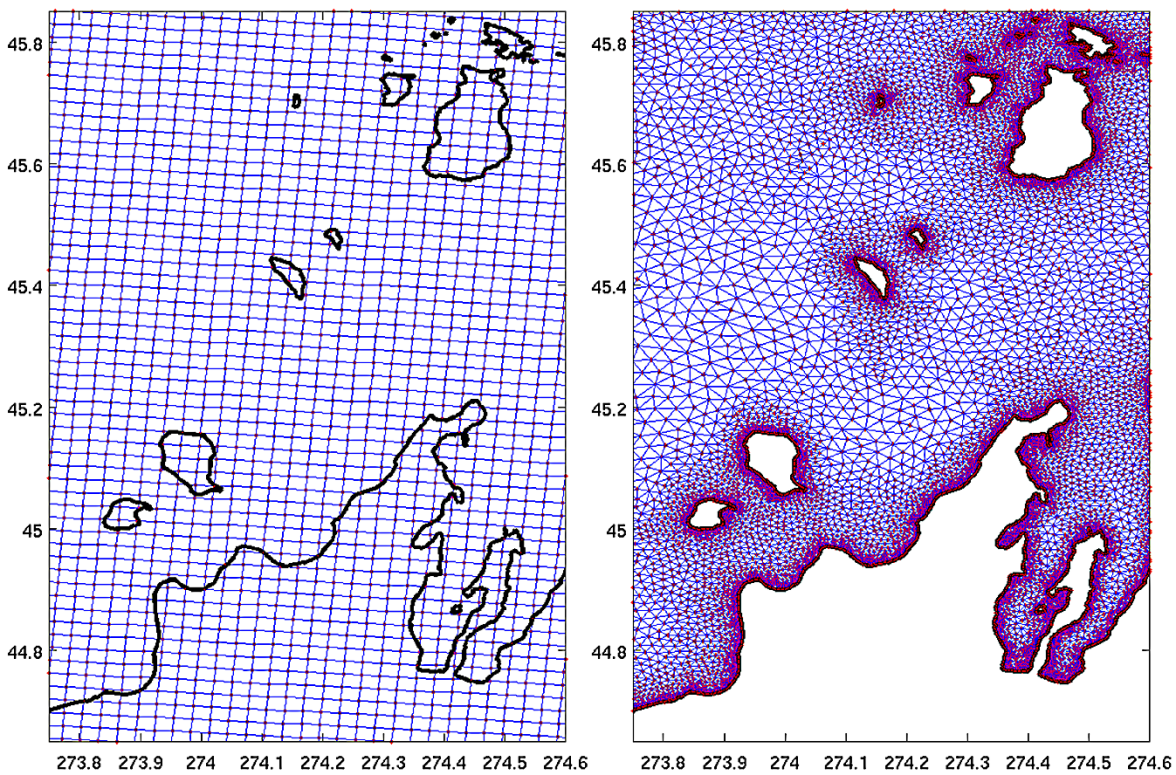
Figure 2 Resolution differences between curvilinear (Lambert conformal) grid at ~2.5km resolution (left panel) and the unstructured mesh at ~2.5km offshore and ~250m at the coast (right panel). Leelanau Peninsula, Beaver and North Manitou Islands, Lake Michigan.
