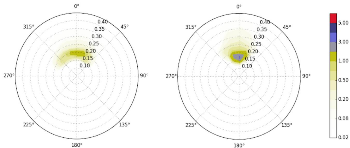
Figure 4 Comparison of wave spectra using the DIA (left) and the GMD (right) at NDBC buoy 45170 in Lake Michigan.
