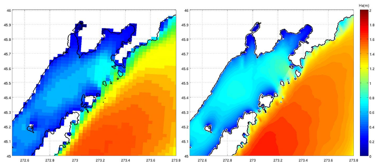
Figure 3 Wave-height pattern resolution near Green Bay, Lake Michigan, illustrating the significant improvement in quality of simulated wave forecasts in the nearshore zone. Original Lambert conformal grid (left panel), Upgraded unstructured mesh (right panel).
