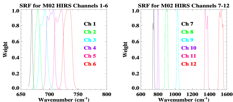
Figure 1. SRFs for MetOp-2 HIRS channels 1–6 (left panel) and 7–12 (right panel).
