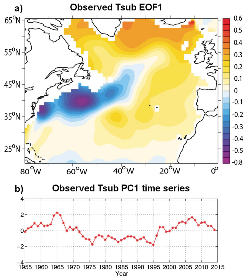
Figure 11. Variability of observed annual mean anomalies of ocean temperature at 400 m ( T_{\text{sub}} ) from an objectively analyzed ocean temperature data set [Levitus et al. , 2005]. (a) The first empirical orthogonal function (EOF1) of observed North Atlantic T_{\text{sub}} (K, 30%) for 1955–2014. (b) First principle component (PC1) time series of observed T_{\text{sub}} during 1955–2014 (normalized). Figure provided by R. Zhang (personal communication, 2015), updated from Zhang [2008].
