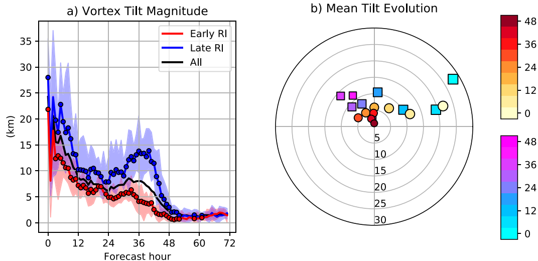
FIG. 10. (a) Composite-mean ensemble forecasts of surface–400-hPa vortex tilt magnitude (km) for early-RI members (red), late-RI members (blue), and all ensemble members (black). Red-shaded regions span the entire distribution of early-RI members, while blue-shaded regions span the distribution of late-RI members. Dotted points denote times where the differences between early and late-RI members are statistically significant at the 95% confidence level. (b) Mean orientation of the surface–400-hPa vortex tilt configuration for early-RI members (circles; warm colors) and late-RI members (squares; cool colors). Vortex tilt is shown in 6-h increments beginning at forecast hour zero and ending at forecast hour 48 (shaded). The vortex tilt is shown with respect to its geographic heading, where north points toward the top of the figure. Radial rings are spaced in 5-km increments.
