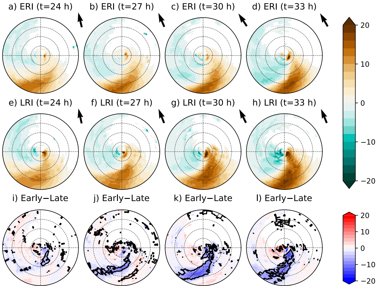
FIG. 6. Storm-centered, 0–200-km, 400-hPa composite-mean radial ventilation ( \Lambda_u ; shaded; \text{kg K m}^{-2} \text{s}^{-1} ) (top) for early-RI members and (middle) late-RI members. Dashed radial rings are spaced in 50-km increments. The 850–200-hPa shear direction is shown by the black vectors. (bottom) As in the top panels, but for the difference between early-RI minus late-RI members. Regions of statistically significant differences are shown by the black contours and hatching. Composites are shown at (a),(e),(i) 24; (b),(f),(j) 27; (c),(g),(k) 30; and (d),(h),(l) 33 h into the simulations.
