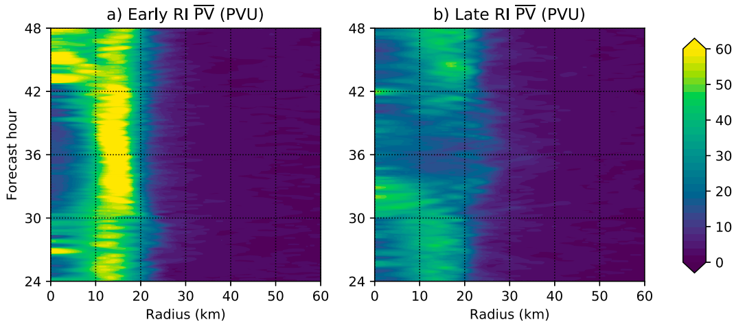
FIG. 11. (a) Time–radius diagram of azimuthally averaged 850-hPa PV (PVU) for the representative early-RI (ERI) ensemble member and (b) late-RI (LRI) ensemble member.
