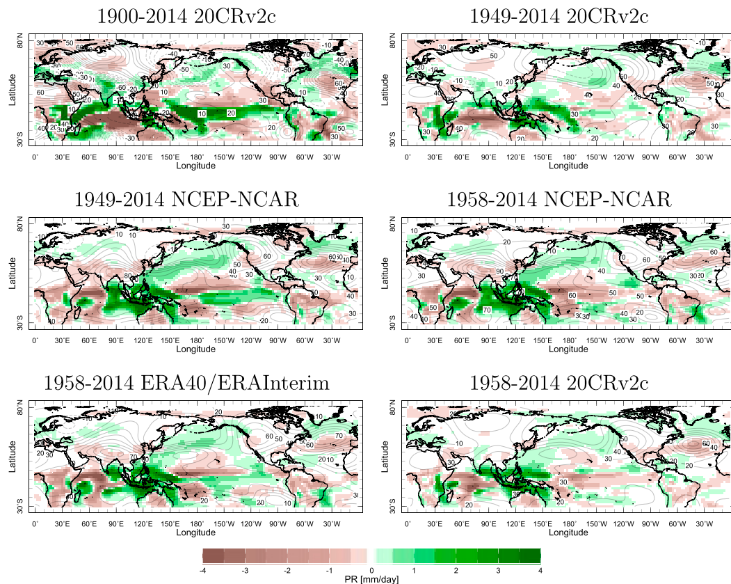
FIG. 14. As in Fig. 14, but for the precipitation response.
