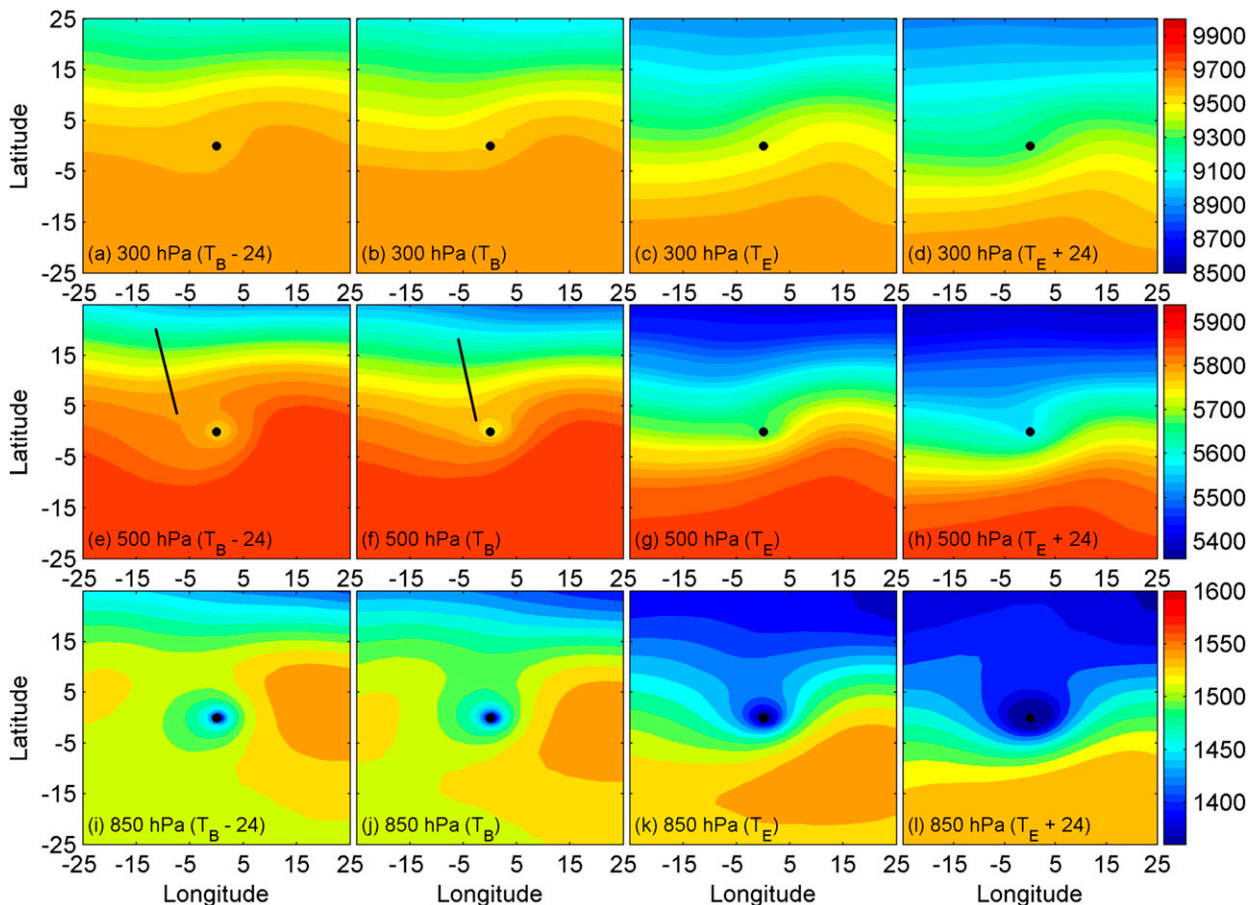
FIG. 8. Storm center-based (a)–(d) 300-, (e)–(h) 500-, and (i)–(l) 850-hPa geopotential height (m) composite from FLOR-FA over 1979–2005. The solid black line indicates the trough axis. The beginning and end time of ET are labeled as T_B and T_E , respectively. The x and y axes are degrees from storm centers. The y axes are in the south–north direction.
