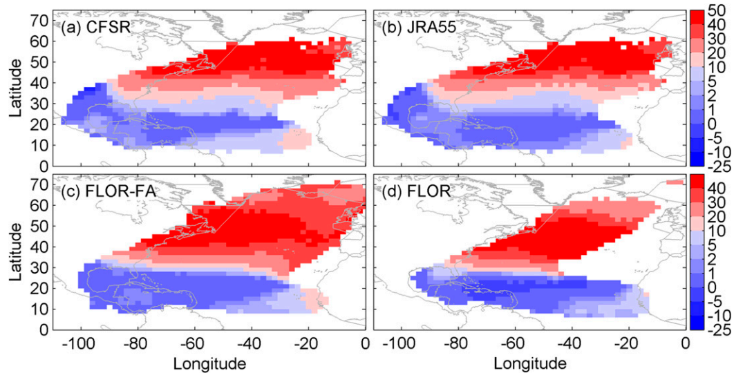
FIG. 4. The mean spatial pattern of B (m) over 1979–2005 from (a) CFSR, (b) JRA-55, (c) FLOR-FA, and (d) FLOR; B is not shown in areas with annual TC density lower than 0.25 TC days. 264 TCs are used for CFSR and JRA-55, and 589 and 983 TCs from all five ensembles for FLOR and FLOR-FA, respectively. The same TC numbers are used for figures hereafter.
