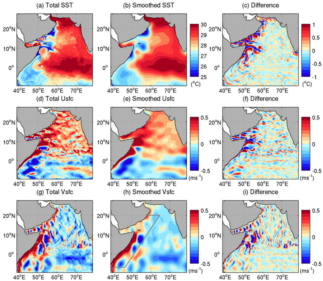
FIG. 3. Example of a 5^\circ low-pass filtering applied to the daily snapshot (1 Aug 2009) of the ocean surface fields, (a)–(c) SST ( ^\circ\text{C} ), (d)–(f) surface zonal current U_{\text{sfc}} ( \text{m s}^{-1} ), and (g)–(i) surface meridional current V_{\text{sfc}} ( \text{m s}^{-1} ). The fields (left) before and (center) after the smoothing; (right) the difference (before minus after). The gray box in (h) denotes the area in which the alongshore averages of the EKE budget terms are calculated for Figs. 8 and 9.
