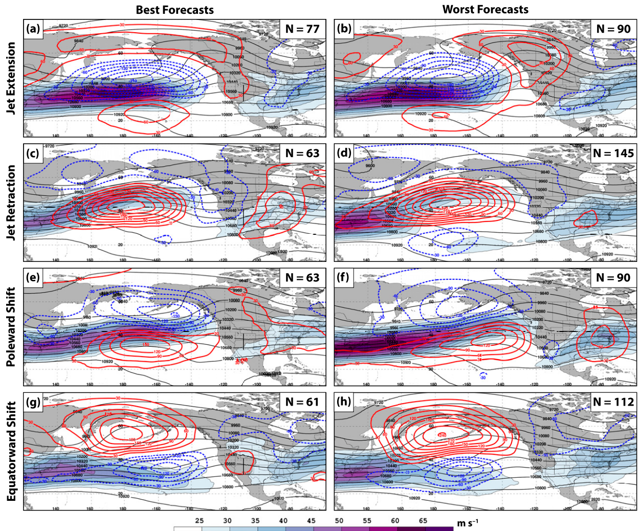
FIG. 12. Composite mean 250-hPa wind speed ( m s^{-1} ) is shaded in the fill pattern, 250-hPa geopotential height is contoured in black every 120 m, and 250-hPa geopotential height anomalies are contoured in solid red and dashed blue every 30 m for positive and negative values, respectively, at the time (a) a best and (b) a worst NPJ phase diagram forecast is initialized during a jet extension. (c),(d) As in (a),(b), but for those forecasts that are initialized during a jet retraction. (e),(f) As in (a),(b), but for those forecasts that are initialized during a poleward shift. (g),(h) As in (a),(b), but for those forecasts that are initialized during an equatorward shift. The quantities in the top-right corner of every panel indicate the number of cases included in each composite.
