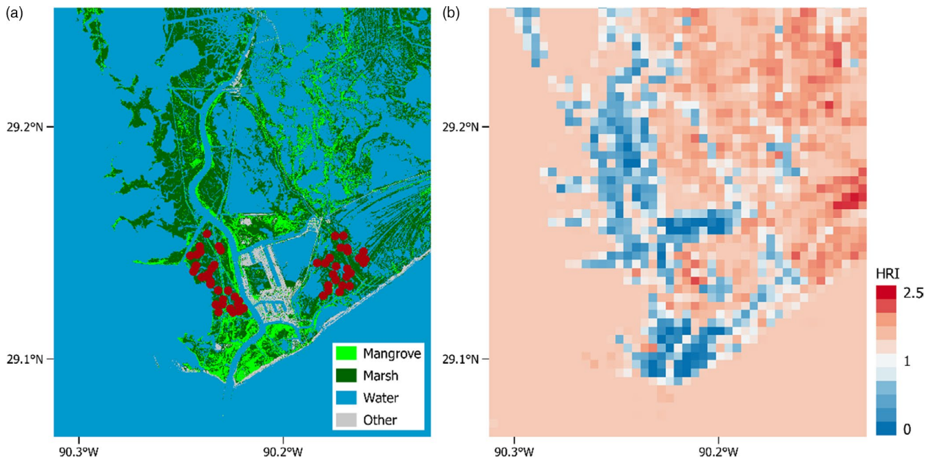
FIGURE 1 The Port Fourchon, LA (a) habitat cover map showing the sampling locations of white shrimp (red points) and (b) the corresponding white shrimp E -scape map. Edge habitat was calculated by measuring the linear distance between the water and vegetation (marsh and mangrove) habitat cover classes and multiplying by 2 m to generate an area. Warmer colours (HRI values > 1) contain more area from habitats producing resources being used by white shrimp, and cooler colours (HRI values < 1) contain less amount of these habitats. The E -scape was generated at a cell size of 400 m × 400 m (similar area to a 200 m radius circle)
