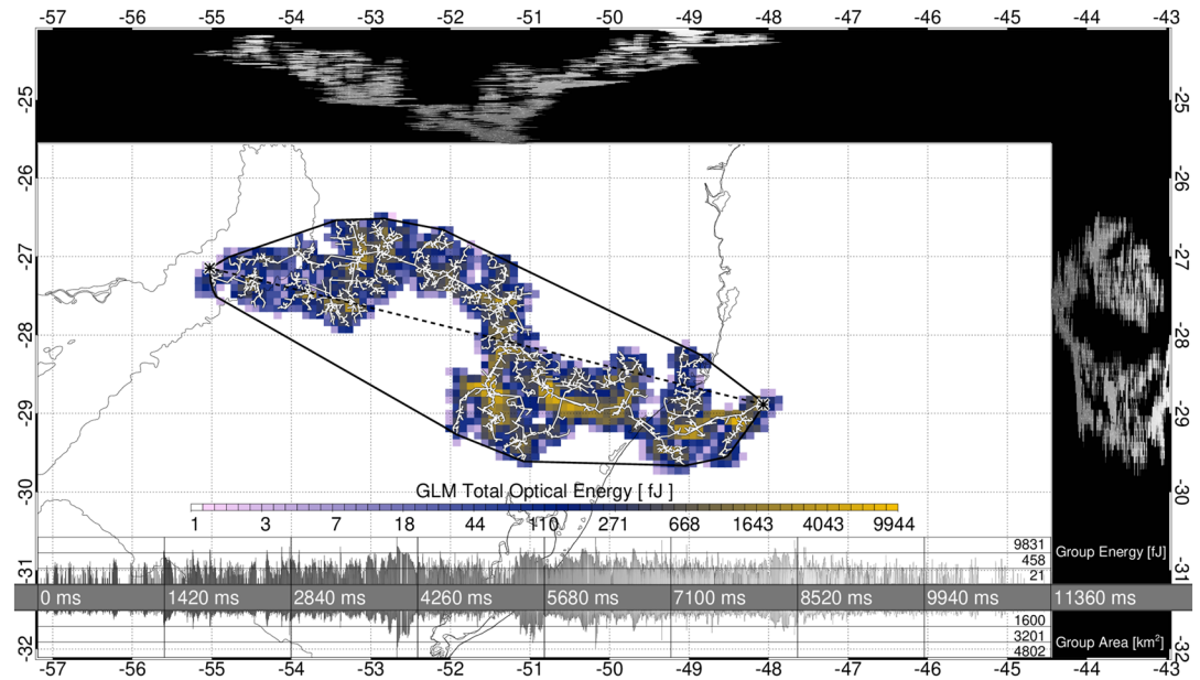
Figure 2. The evolution of the 709 \pm 8 km megaflash over southern Brazil. Incremental flash development is plotted over a total optical energy grid in the central panel. Group extents in longitude (top) and latitude (right) are shown in the outer panels as a function of time-ordered group index starting at the edge of the plan-view plot. Negative longitudes indicate degrees west while negative latitudes indicate degrees south. Timeseries of group energy (above) and group area (below) are shown aligning the bottom of the figure. The dashed line connects the most distant groups (marked with asterisks), while the solid line draws a convex hull around the groups in the flash.
