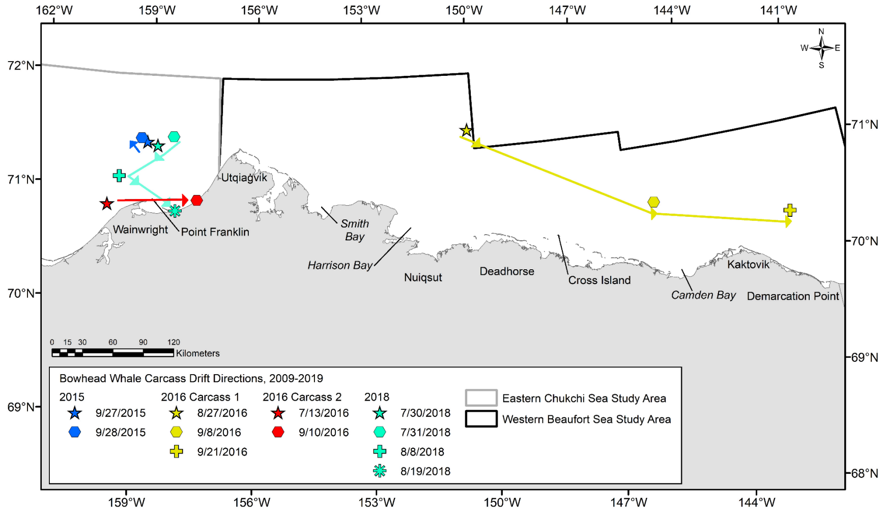
Fig. 3.1 Bowhead whale ( Balaena mysticetus ) carcass drift directions, 2009–2019. Sightings of individual carcasses sighted more than once are color-coded. The star symbol represents the initial sighting, the octagon symbols represent the second sighting, the cross symbols represent the third sighting, and the asterisk symbol represents the four sightings. Lines with triangles depict the drift direction of the carcass with the matching color. The boundary for the eastern Chukchi Sea (EC) study area is indicated in grey and the border for the western Beaufort (WB) Sea study area is shown in black (see Fig. 1 for a full view of the EC and WB study areas)
