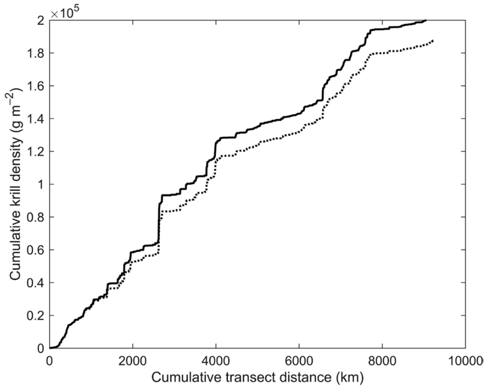
Figure 7. Cumulative krill density obtained from the southwest arms analysis when using a -30 \text{ dB re m}^{-1} (solid line) and -40 \text{ dB re m}^{-1} (dotted line) noise filter S_v threshold.
