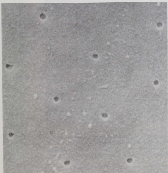
Figure 3-11.—Two scanning electron micrographs (about 10,000 \times ), (a) cod, Gadus callarias , chorion and (b) pollock, Pollachius virens , chorion, are examples of striking pore patterns one expects to find in fish eggs. No such patterns were observable in fourbeard rockling eggs sampled in gasoline spill vicinity 2 d after spill (even though embryo and egg deterioration had not occurred) as demonstrated in Figures 3-9 and 3-10. Compare Figure 3-11 with Figure 3-9 at same magnification.
