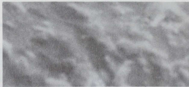
Figure 3-10.—Scanning electron microscope view of a portion of chorion of fourbeard rockling egg. Membrane is deteriorating and no pore structure can be observed. Postspill day 2 (25,000 \times ).
