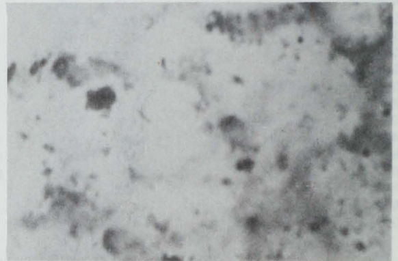
Figure 3-7.—Photographic enlargement of portion of chorion of fourbeard rockling egg showing deterioration and absence of any pore structure ( 100\times oil immersion objective, light microscope). Postspill day 4.
