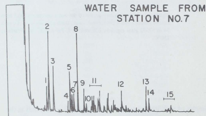
Figure 2-3.—Gas chromatograms of a gasoline standard in hexane, a water-accommodated fraction (WAF) of the gasoline standard, and a water sample from station 7. The standards were run on a 30 m SE-52 glass capillary column. The water sample was run on a 30 m OV-101 column. All analyses: 35°C for 4 min, the 5°/min to 250°C.
