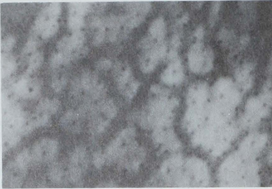
Figure 3-4.—Portion of chorion of fourbeard rockling egg as seen under oil immersion lens ( 100\times ) of light microscope. Chorion has been removed from egg. Postspill day 4.
