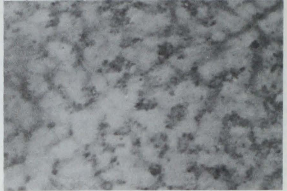
Figure 3-6.—Portion of chorion of fourbeard rockling egg showing deterioration and absence of any pore structure. ( 100\times immersion objective, light microscope). Postspill day 4.
