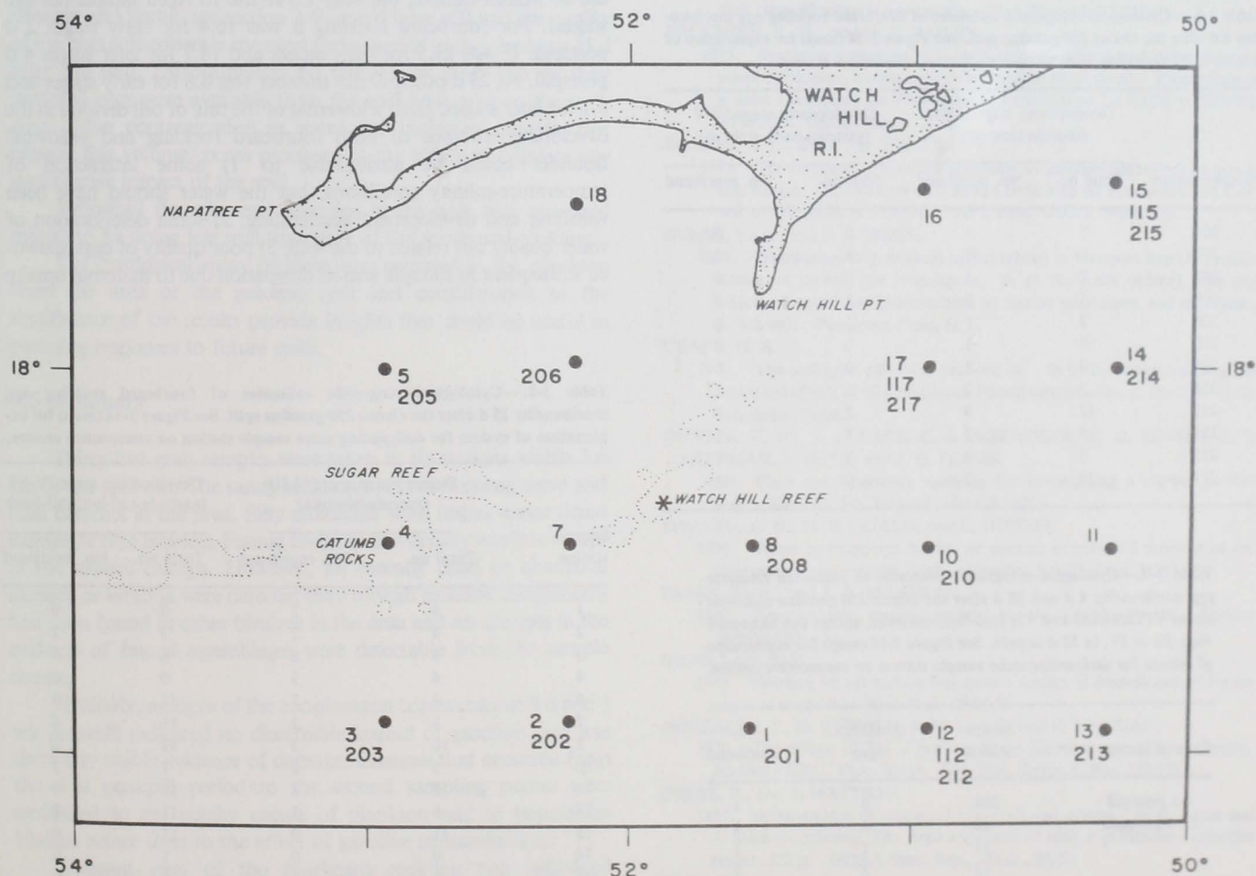
Figure 3-14.—Survey area and station locations for RV Strider cruise 78-01. Asterisk marks the location of grounding of barge Ocean 250 on Watch Hill Reef. The 100 series numbers refer to postspill day 2 samples; the 200 series, to postspill day 4 samples. Numbers 1-18 refer to postspill day 25 samples. Only stations at which fish eggs were sampled are indicated.
