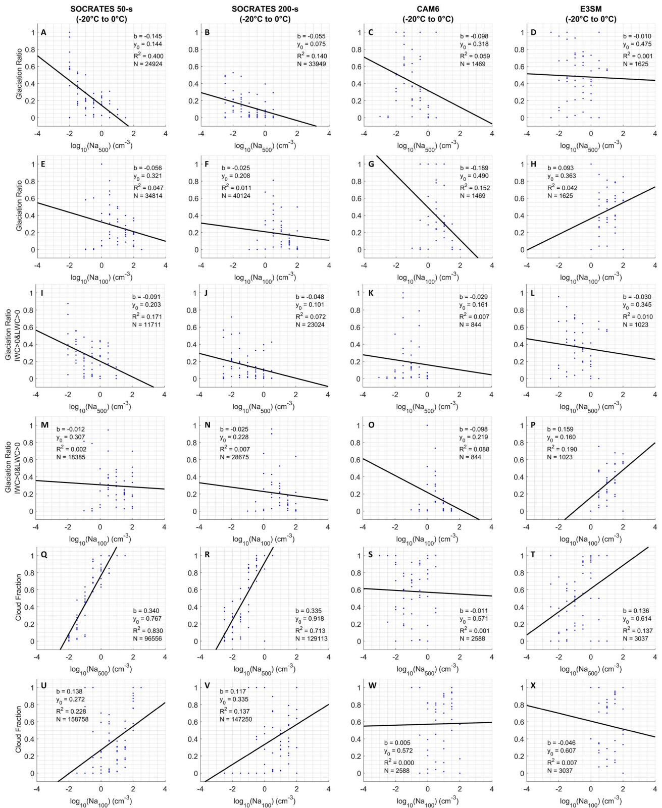
Figure 14. Similar to Figure 13 but for temperatures between -20^{\circ}\text{C} and 0^{\circ}\text{C} .
