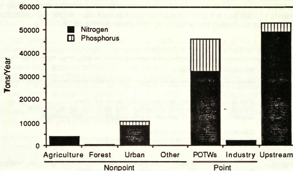
Figure 5. Nutrient discharges by source category for the Northeast
