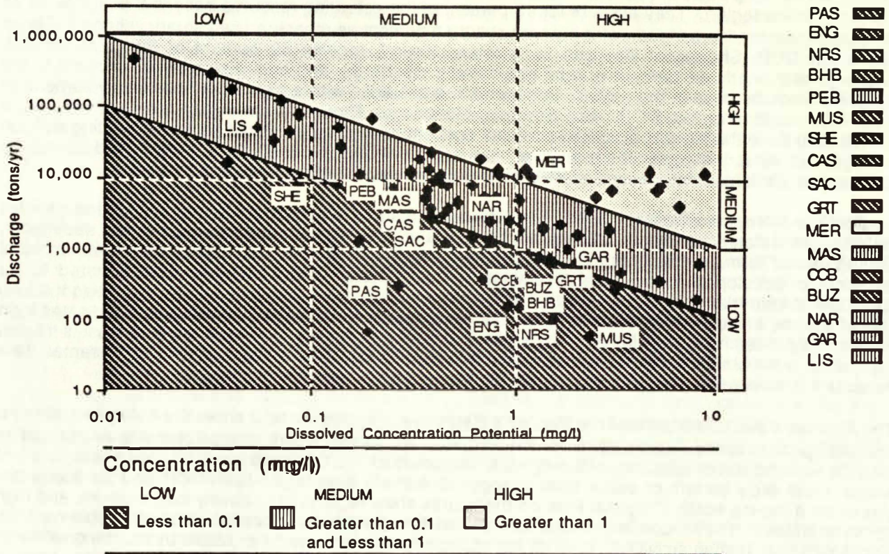
Figure 3. Phosphorus concentration status
