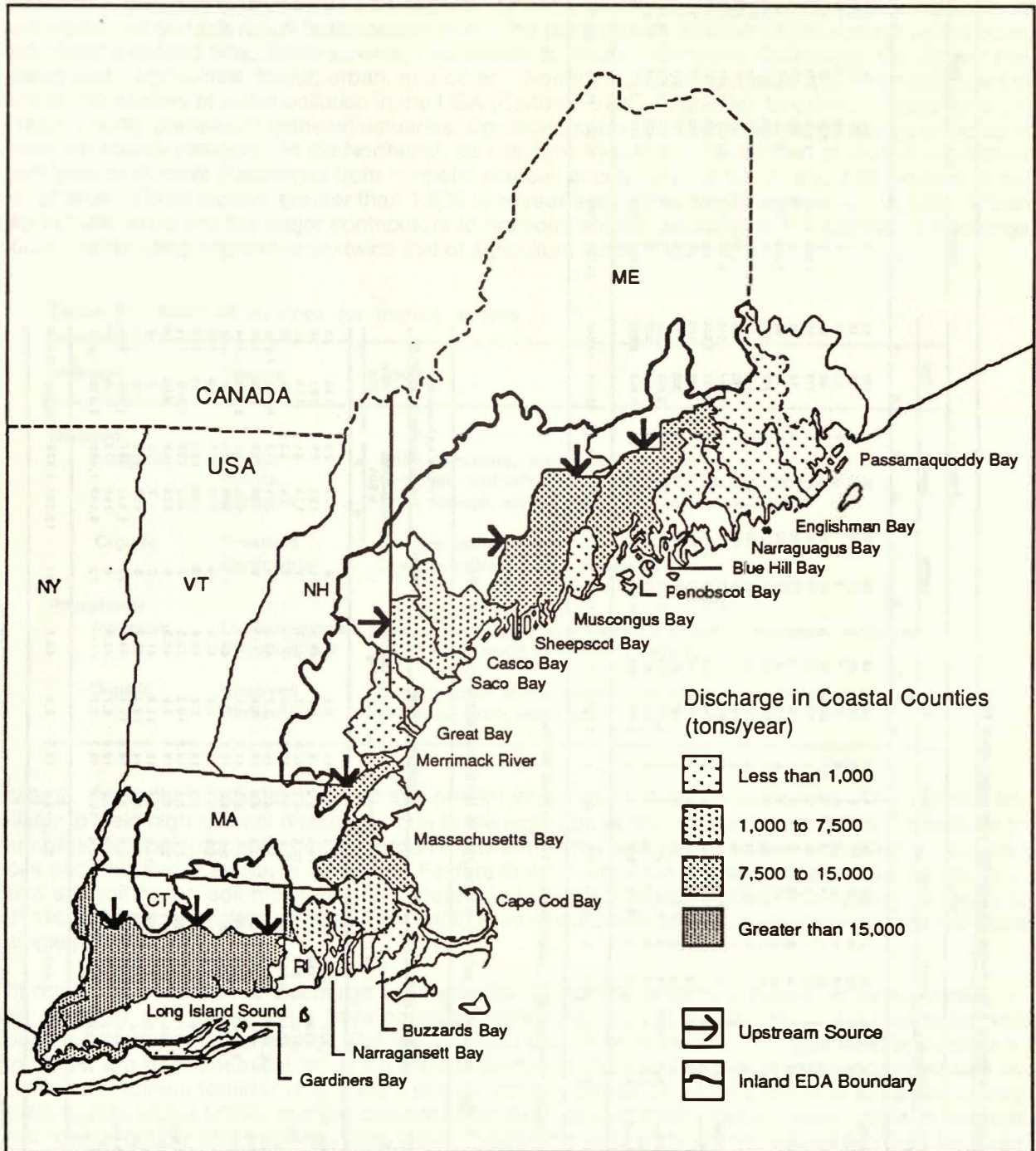
Figure 4. Nitrogen and phosphorus discharge in the coastal county portion of estuarine drainage areas, circa 1982
