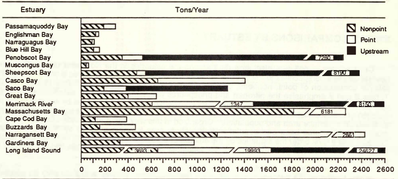
Figure 6. Nitrogen discharges by source by estuary
