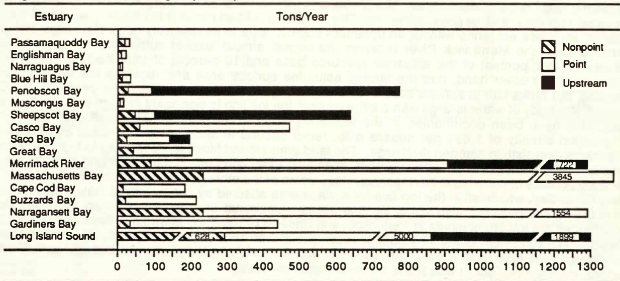
Figure 7. Phosphorus discharges by estuary
