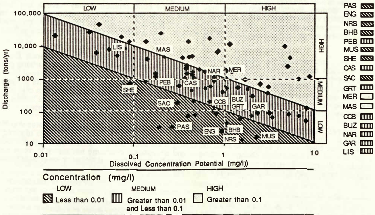
Figure 3. Phosphorus concentration status
