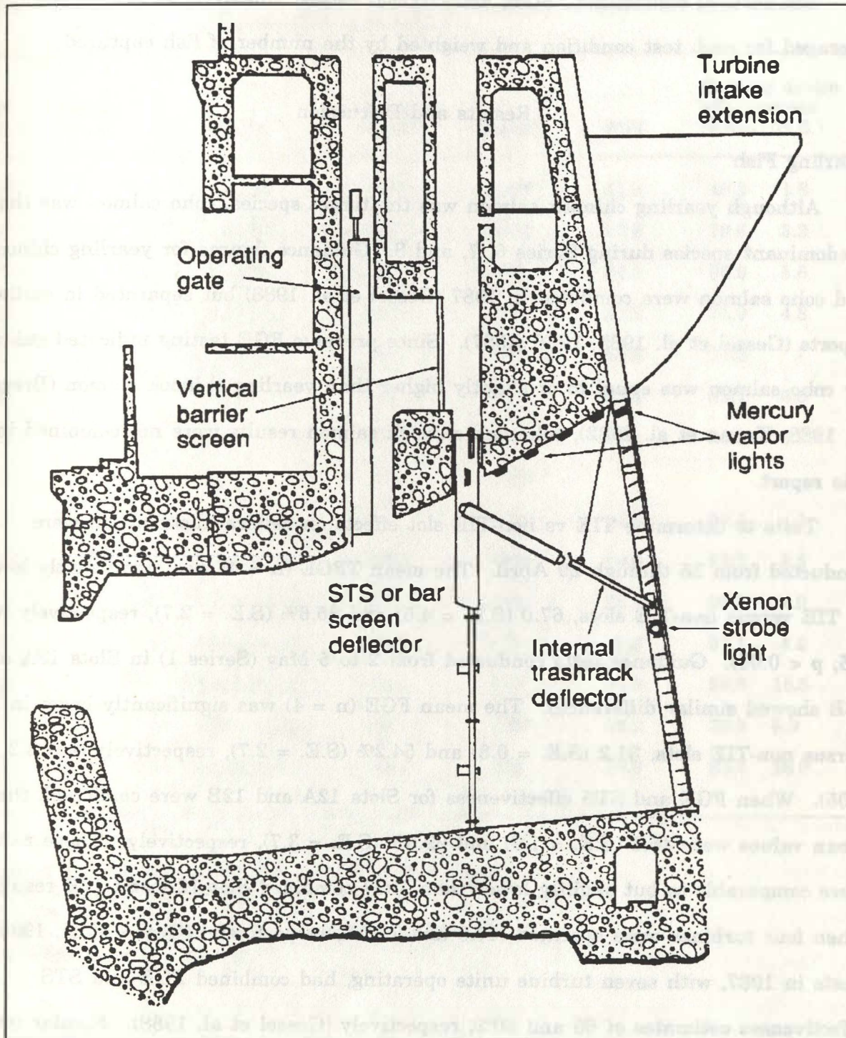
Figure 1.--Cross-sectional view of a turbine intake with turbine intake extension, lights, and internal trashrack deflector tested at Bonneville Dam Second Powerhouse, 1988.
