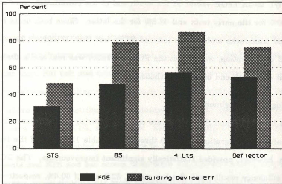
Figure 2.--Spring chinook salmon fish guidance efficiency (FGE) and effectiveness with submersible traveling screen (STS), bar screen (BS), lights (Lts), and internal trash rack deflector at Bonneville Dam Second Powerhouse, 1988.
