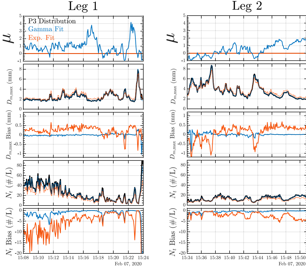
FIG. 7. PSD measurements of D_{m,\max} and N_t computed directly from measured PSDs from the 2DS and HVPS (black lines), gamma distribution fits (blue lines), and exponential distribution fits to the 2DS/HVPS PSDs (orange lines) for (top) \mu , (top middle) D_{m,\max} , (middle) D_{m,\max} bias, (bottom middle) N_t , and (bottom) N_t bias for (left) leg 1 and (right) leg 2; D_{m,\max} and N_t biases represent P3 probe observations subtracted from fits to the P3 probe observations. Fit parameters D_{m,\max} and N_t were calculated over the 2DS and HVPS size range ( 0.10 \leq D_{\max} \leq 30.0 mm) representing the P3-observed PSD.
