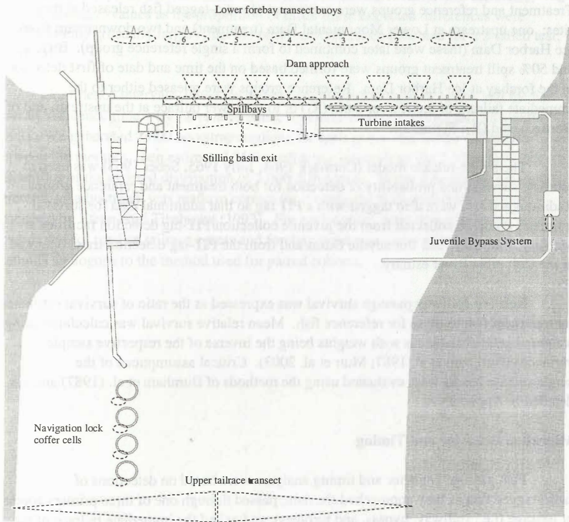
Figure 3. Plan view of Ice Harbor Dam showing approximate radiotelemetry detection zones in 2003. Dashed ovals represent underwater antennas; dashed triangles represent aerial antennas.
