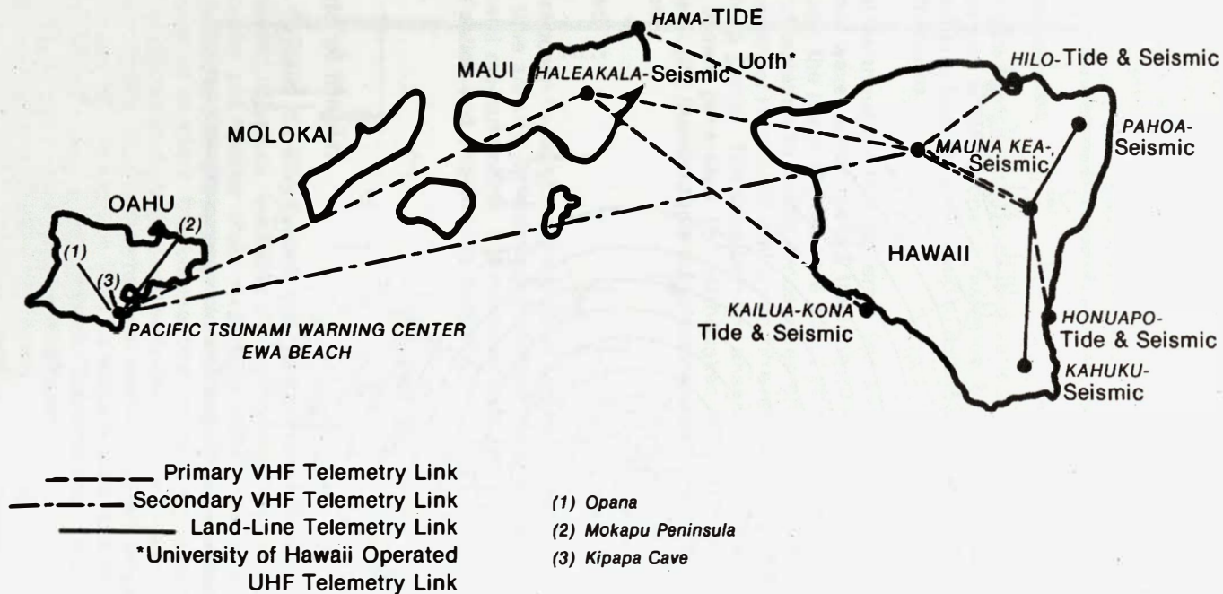
Figure 5 Hawaii Regional Tsunami Warning Network Showing Telemetry Links and Sensor Sites
