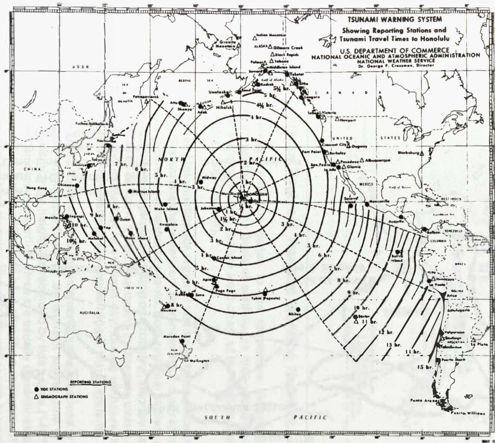
Figure 4 Tsunami Warning System
