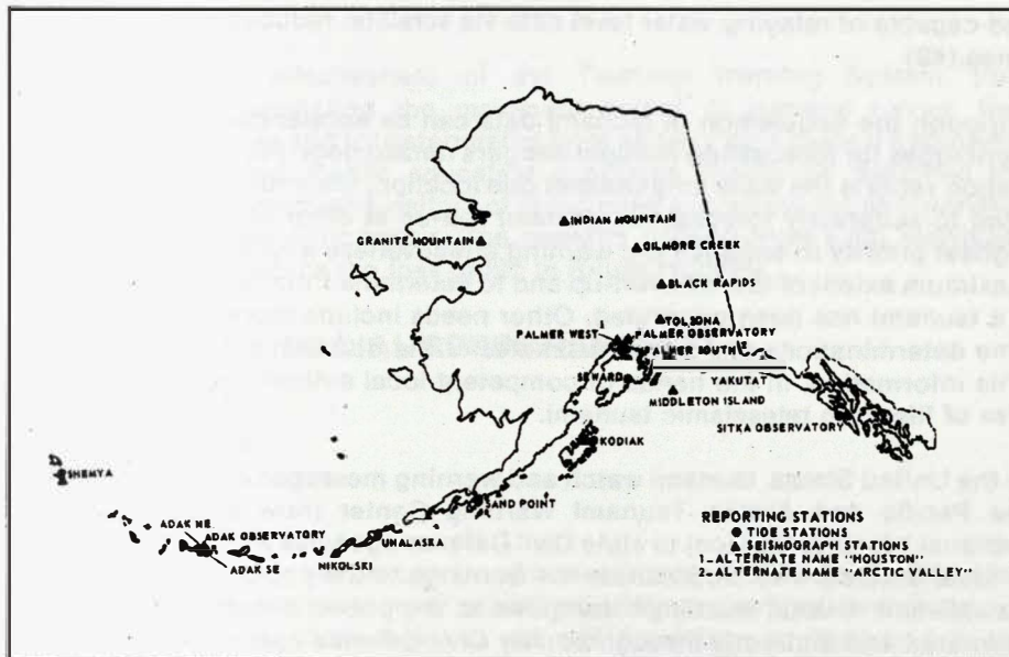
Figure 6 Alaska Regional Tsunami Warning Network
