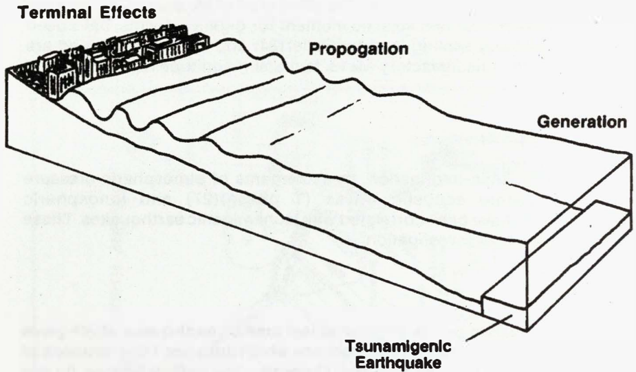
Figure 3 Stages of Tsunami Development
