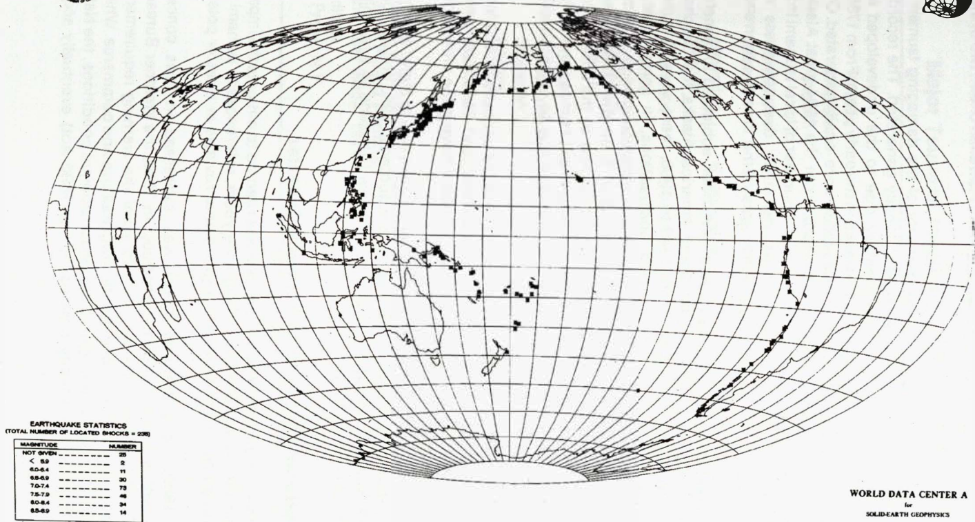
Figure 1 Tsunami Data (1876-1976)
