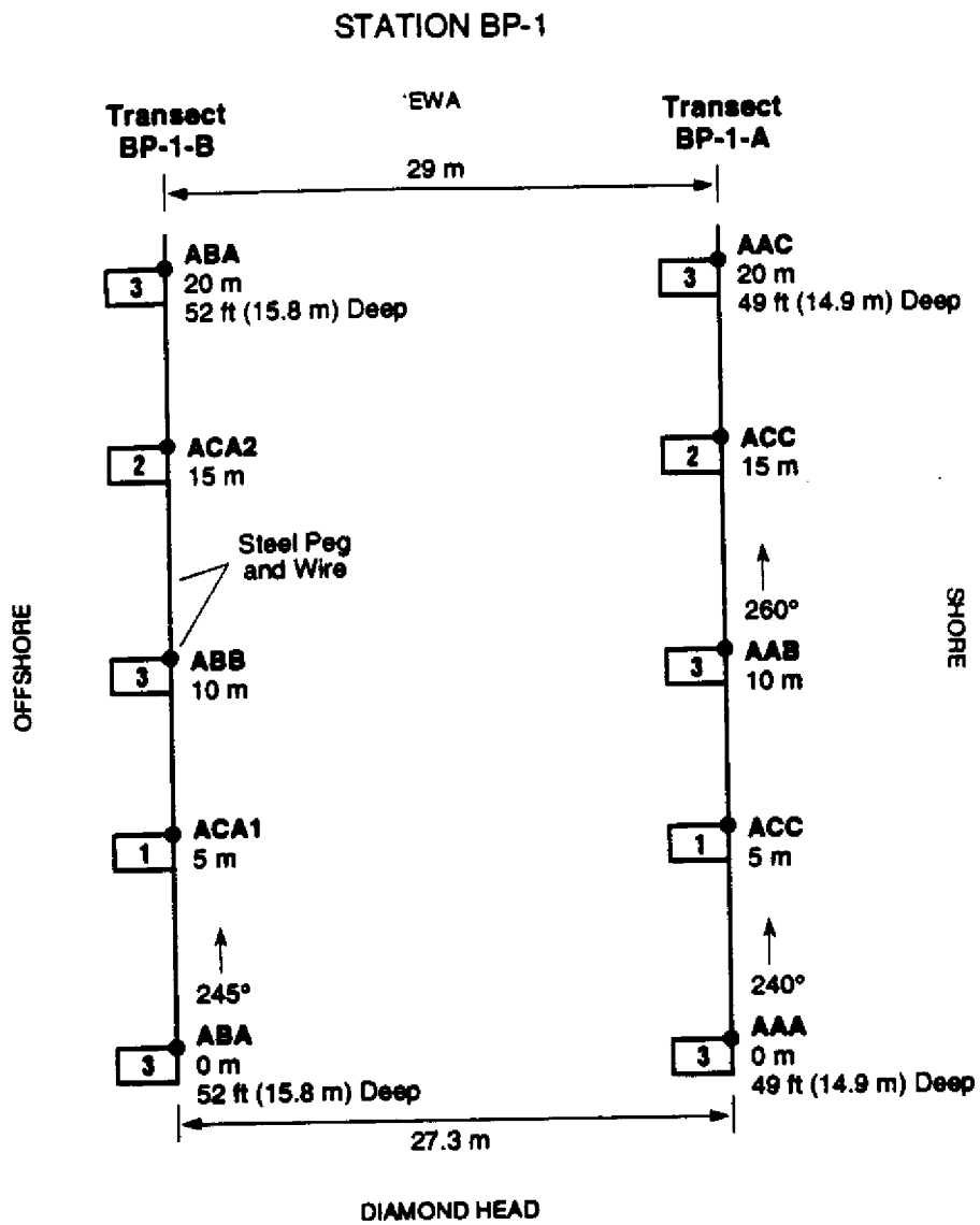
FIGURE 2. Locations of the five photographic quadrats each on Transects BP-1-A and BP-1-B located at the eastern station (BP-1) offshore of 'Ewa Beach, O'ahu, Hawai'i
