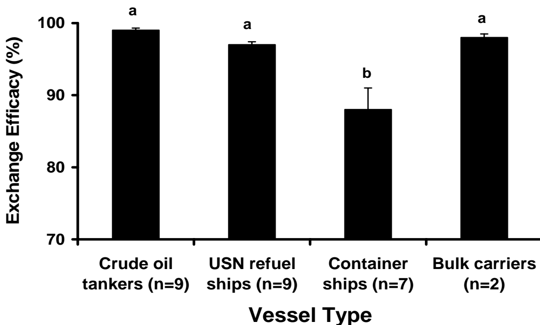
Figure 2-2: BWE Efficacy for Removal of Rhodamine Dye by the Empty-Refill Method. The mean efficacy (+se) is shown for each ship type and sample size, shown on the x-axis.
