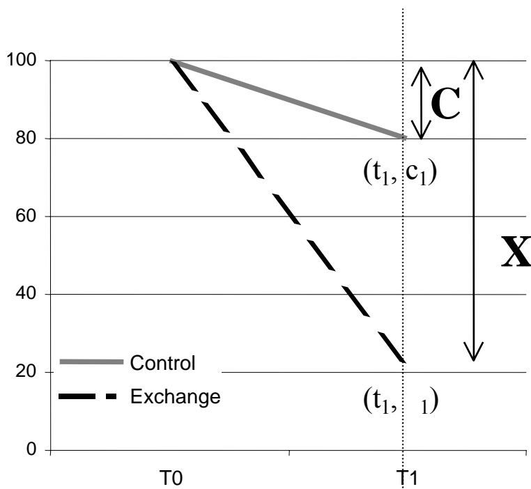
Figure 2-1: Calculation of BWE for Target Zooplankton. Efficacy is estimated as a function of change in concentration over time ( T_0 to T_1 ) in exchanged tank ( X ) relative to those observed in the control tank ( C ). See text for further detail.
