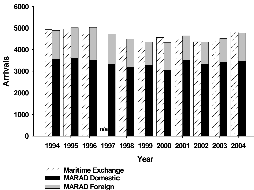
Figure 4-2: Arrivals to Chesapeake Bay based upon reports to the Baltimore and Hampton Roads Maritime Exchanges and to MARAD from 1994 – 2004. MARAD Arrivals were characterized as foreign or domestic arrivals based upon the last port of call. (Note: Arrival records from the Hampton Roads Maritime Exchange were unavailable in 1997).
