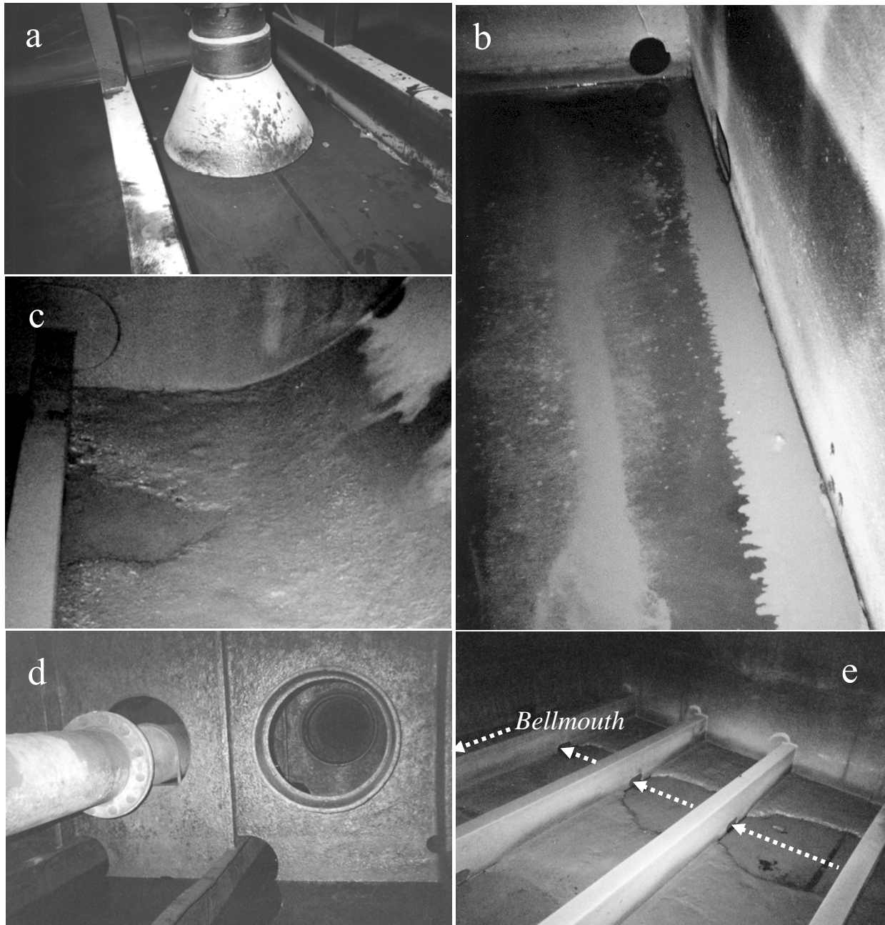
Figure 3-4: a) Area around bellmouth is free of accumulated sediment. Deck plating is clearly visible. b) Longitudinal scour associated with bays aligned with the bellmouth bay. c) Heavy accumulation of sediment along the outer bilge. d) Large holes and slots provide path of least resistance during early stages of deballasting. e) Well-defined paths of transverse sediment scour between drain holes of adjacent stiffeners. (Photos courtesy of the Great Lakes NOBOB Assessment Project).
