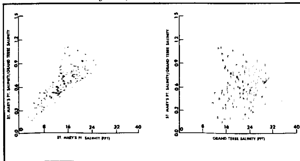
Fig. 8. Salinity vs. salinity ratio comparison.
