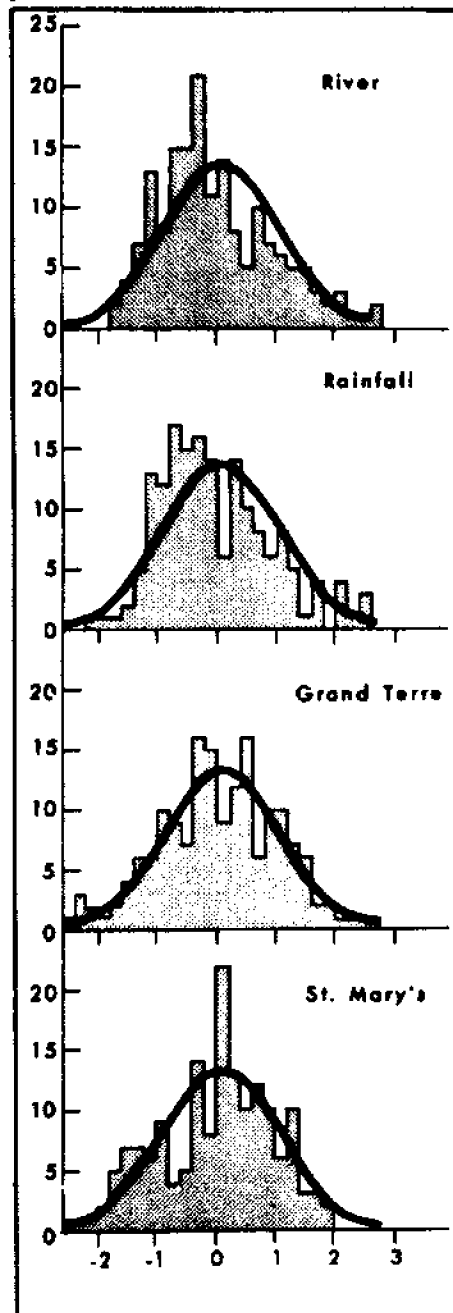
Fig. 7. Histograms of normalized data.
